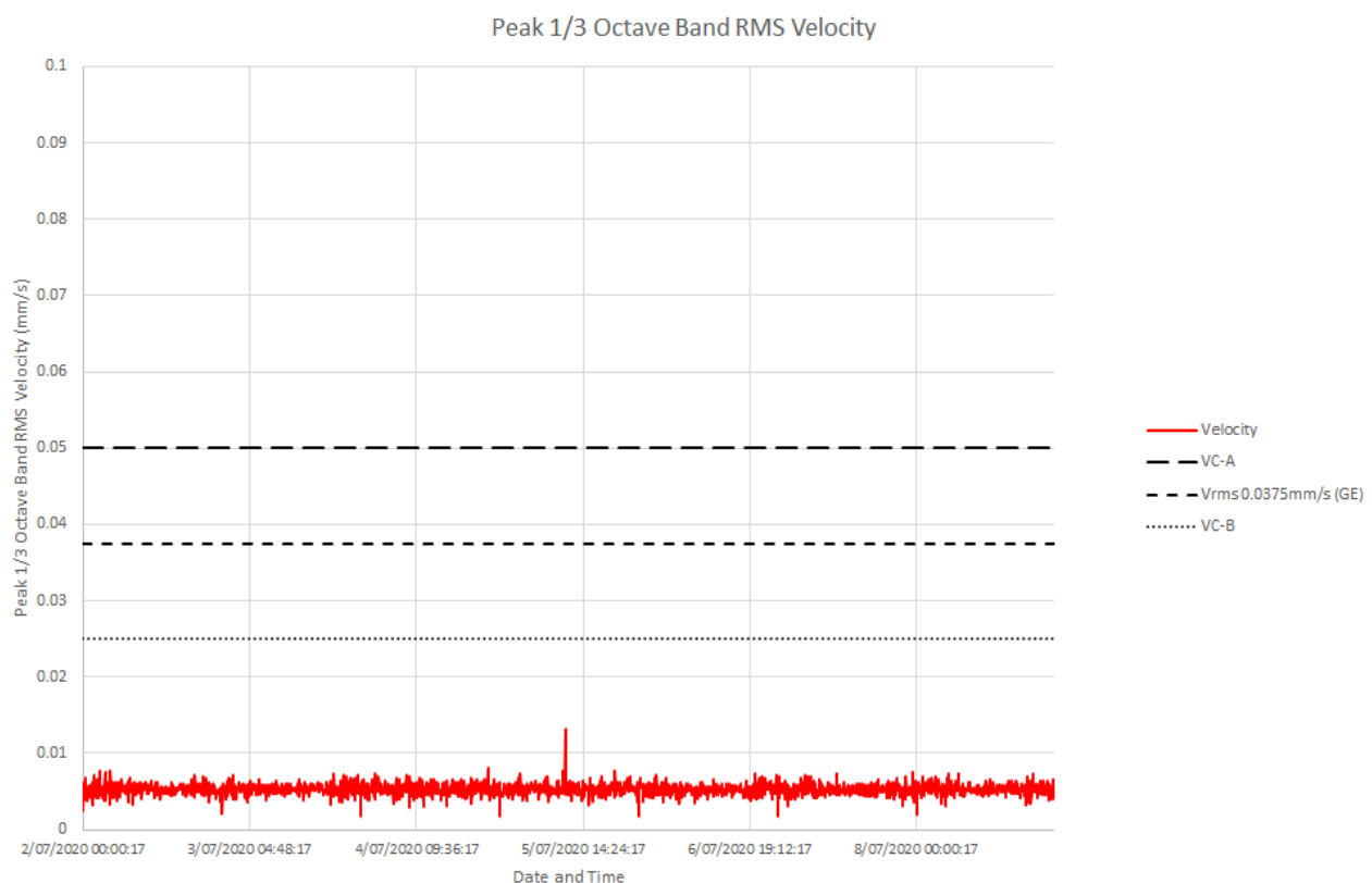
Figure 1: Measured vibration levels for 02/07/2020 to 08/07/2020
