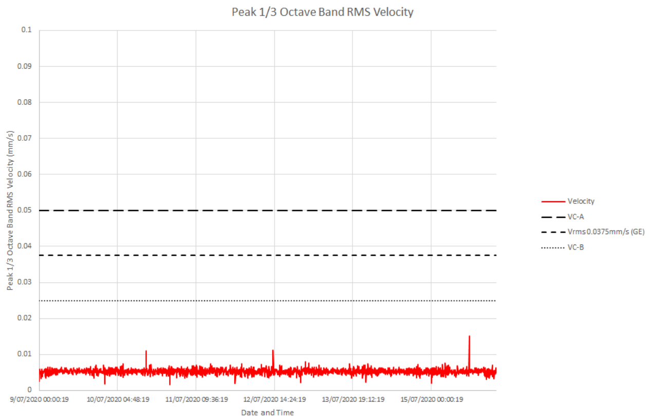
Figure 1: Measured vibration levels for 09/07/2020 to 15/07/2020
