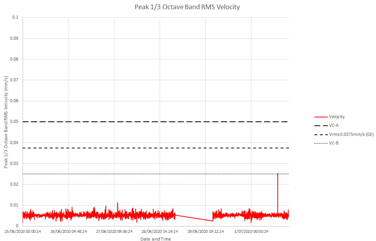
Figure 1: Measured vibration levels for 25/06/2020 to 01/07/2020
