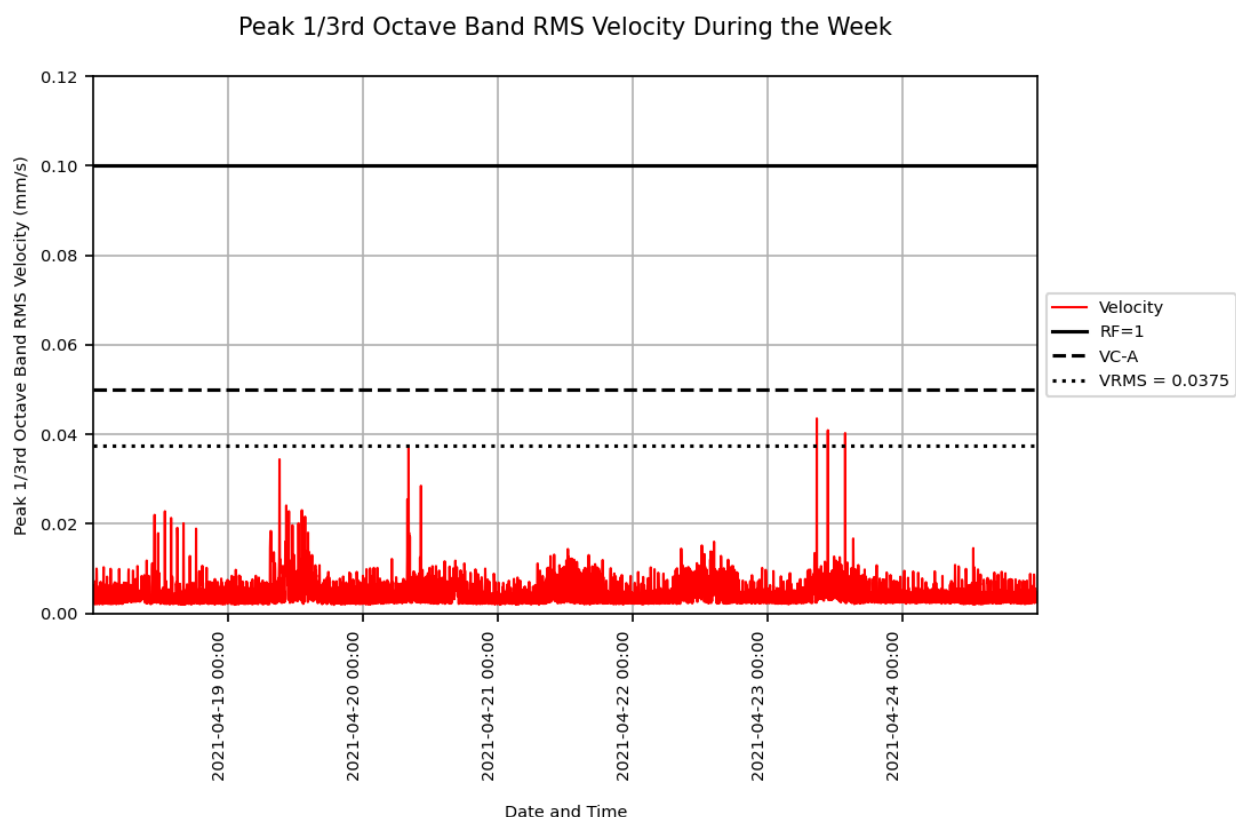
Figure 1: Measured vibration levels for 18/04/2021 to 24/04/2021 at the Medical Imaging Facility
