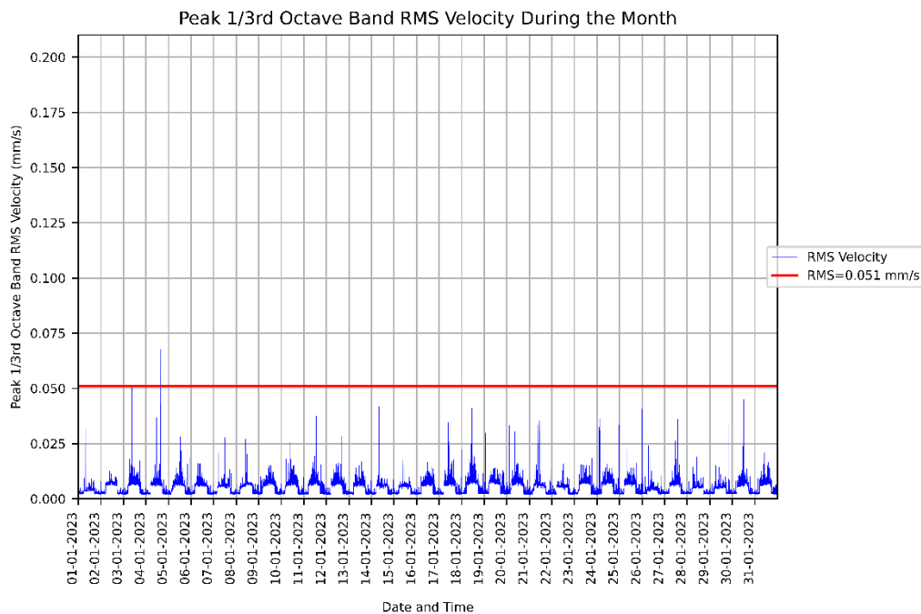
Figure 1: Measured RMSV vibration levels for 01/01/2023 to 31/01/2023 at the KR - L4 Lab 9.
