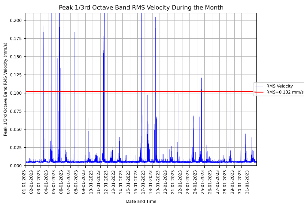
Figure 1: Measured RMSV vibration levels for 01/01/2023 to 31/01/2023 at the CHW - L1 Lab.
