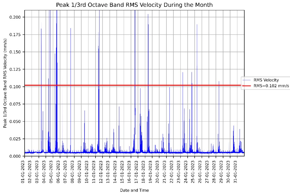
Figure 3: Measured RMSV vibration levels for 01/01/2023 to 31/01/2023 at the CHW - L1 Lab.
