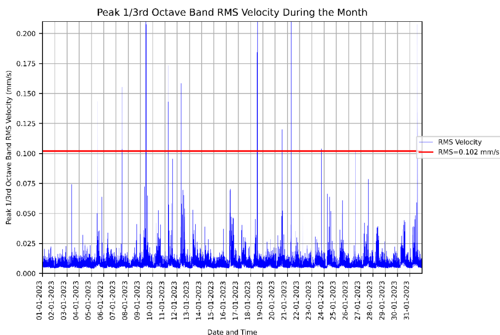
Figure 1: Measured RMSV vibration levels for 01/01/2023 to 31/01/2023 at the CASB level 3 Surgical Suite.
