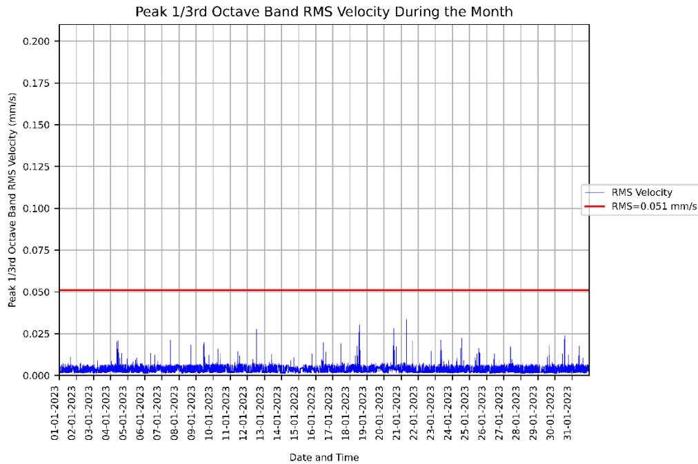
Figure 3: Measured RMSV vibration levels for 01/01/2023 to 31/01/2023 at the CASB Level 2 MRI.
