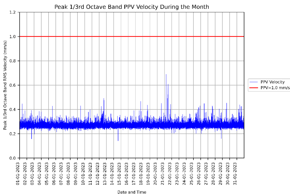
Figure 5: Measured PPV vibration levels for 01/01/2023 to 31/01/2023 at the KR - Animal House.
