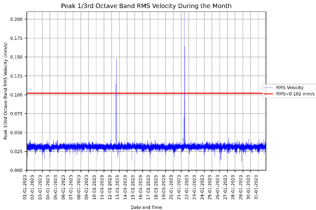
Figure 4: Measured RMSV vibration levels for 01/01/2023 to 31/01/2023 at the KR - Animal House.
