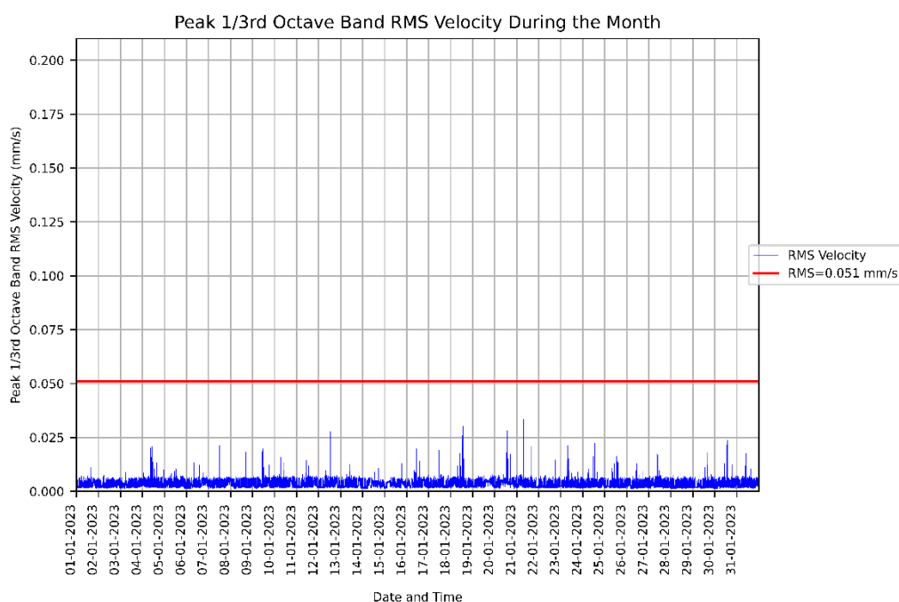
Figure 1: Measured RMSV vibration levels for 01/01/2023 to 31/01/2023 at the CASB Level 2 MRI.
