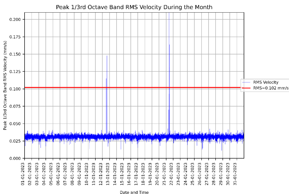
Figure 1: Measured RMSV vibration levels for 01/01/2023 to 31/01/2023 at the KR - Animal House.
