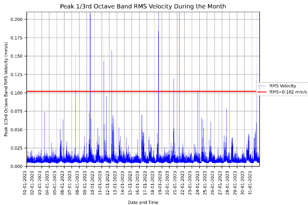
Figure 3: Measured RMSV vibration levels for 01/01/2023 to 31/01/2023 at the CASB level 3 Surgical Suite.
