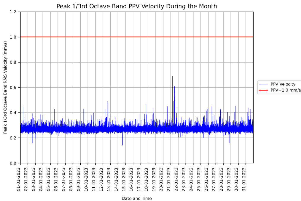
Figure 2: Measured vibration levels for 01/01/2023 to 31/01/2023 at the KR - Animal House.
