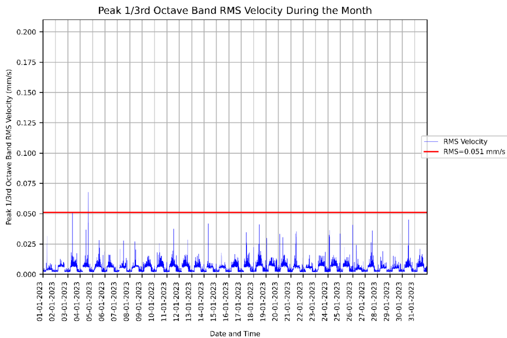
Figure 3: Measured RMSV vibration levels for 01/01/2023 to 31/01/2023 at the KR - L4 Lab 9.
