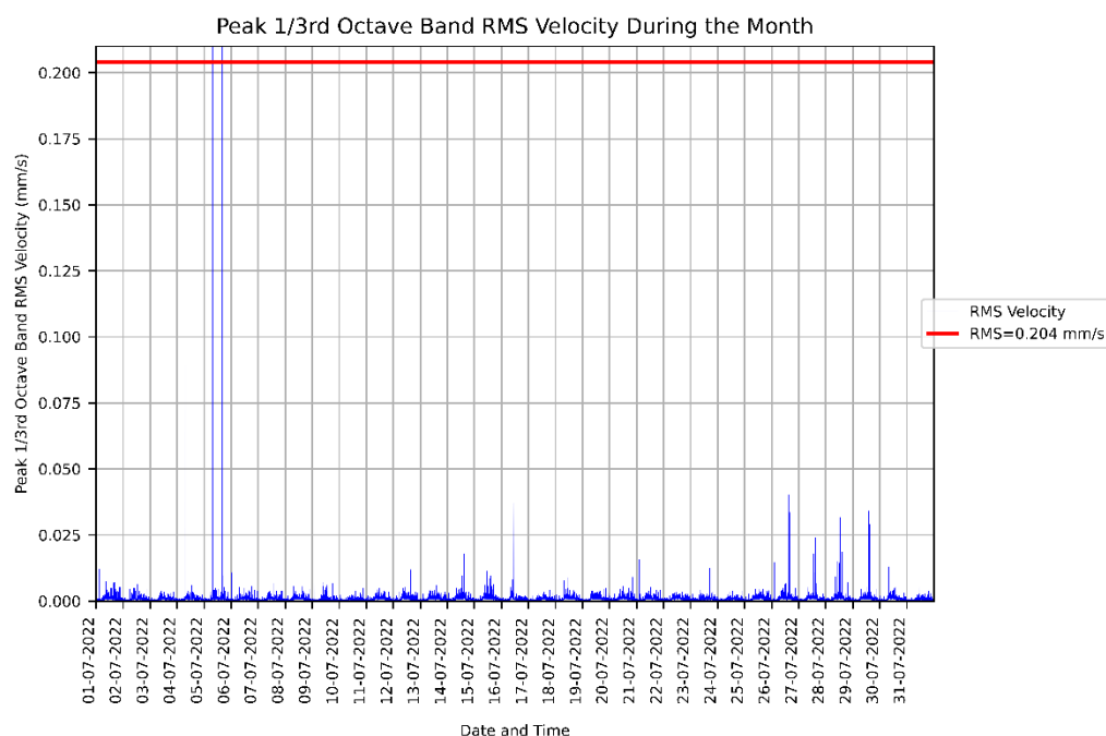
Figure 1: Measured RMSV vibration levels for 01/07/2022 to 31/07/2022 at the CH - Mental Health Utility - Wade Ward.
