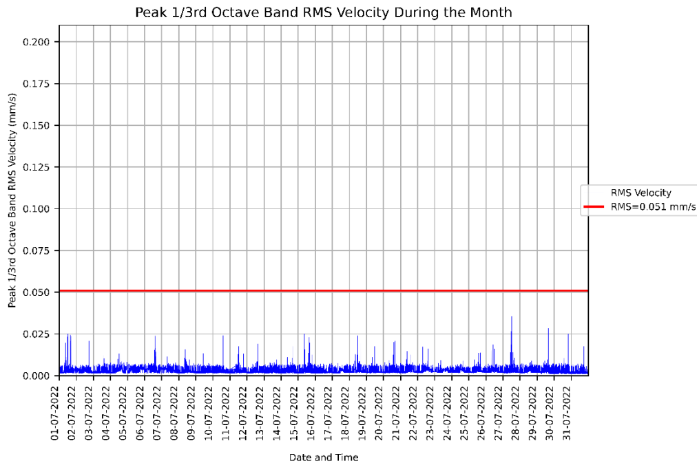
Figure 1: Measured RMSV vibration levels for 01/07/2022 to 31/07/2022 at the CASB Level 2 MRI.
