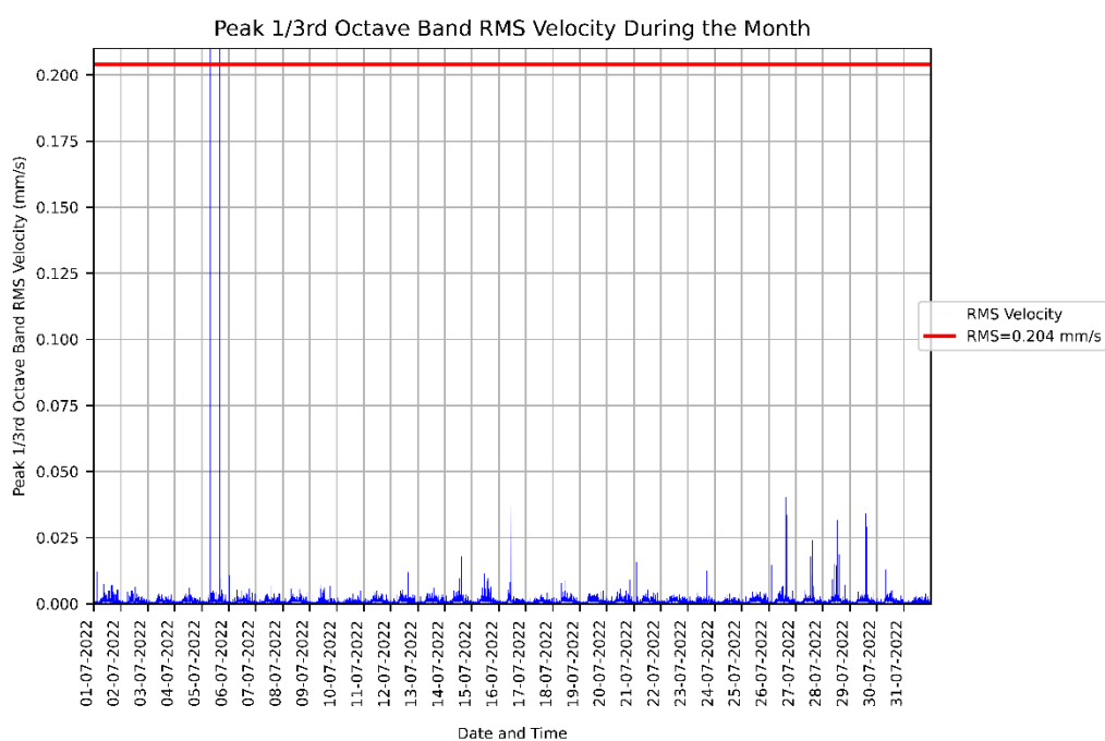
Figure 3: Measured RMSV vibration levels for 01/07/2022 to 31/07/2022 at the CH - Mental Health Utility - Wade Ward.
