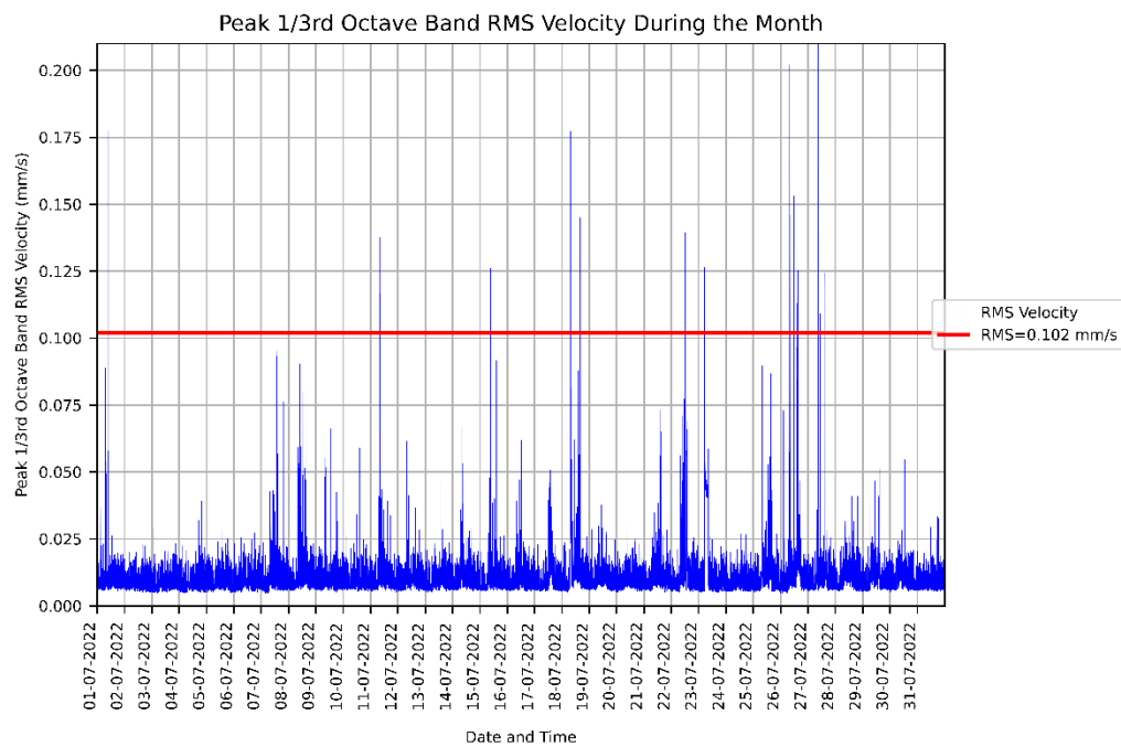
Figure 3: Measured RMSV vibration levels for 01/07/2022 to 31/07/2022 at the CASB level 3 Surgical Suite.
