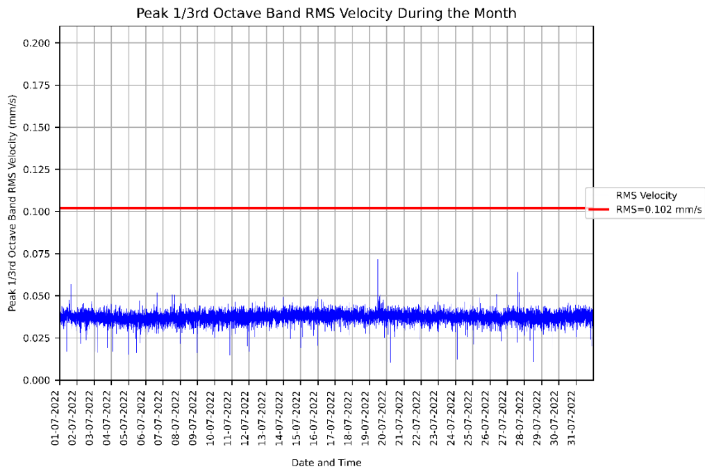
Figure 4: Measured RMSV vibration levels for 01/07/2022 to 31/07/2022 at the KR - Animal House.
