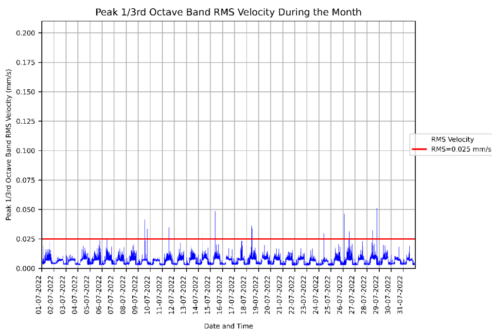
Figure 1: Measured RMSV vibration levels for 01/07/2022 to 31/07/2022 at the KR - L4 Lab 9.
