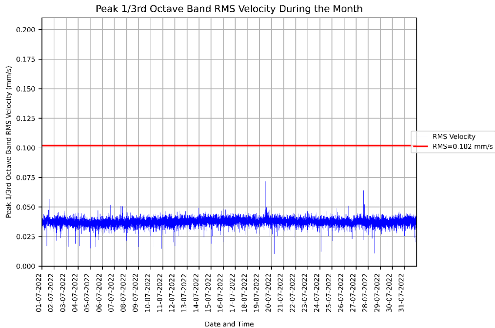
Figure 1: Measured RMSV vibration levels for 01/07/2022 to 31/07/2022 at the KR - Animal House.
