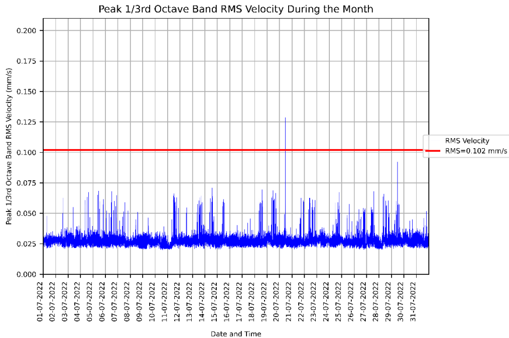
Figure 1: Measured RMSV vibration levels for 01/07/2022 to 31/07/2022 at the CHW - L1 Lab.
