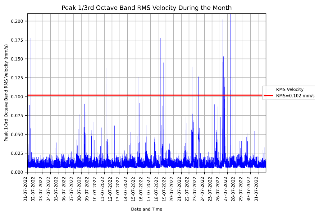
Figure 1: Measured RMSV vibration levels for 01/07/2022 to 31/07/2022 at the CASB level 3 Surgical Suite.
