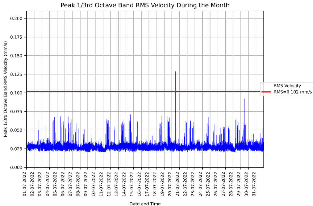
Figure 3: Measured RMSV vibration levels for 01/07/2022 to 31/07/2022 at the CHW - L1 Lab.
