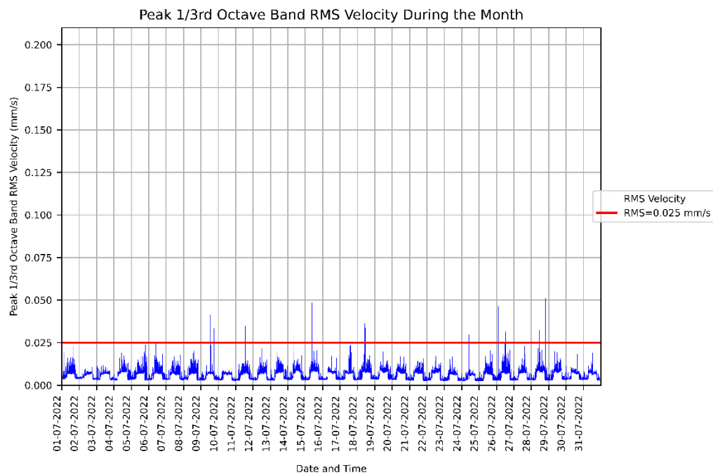
Figure 3: Measured RMSV vibration levels for 01/07/2022 to 31/07/2022 at the KR - L4 Lab 9.
