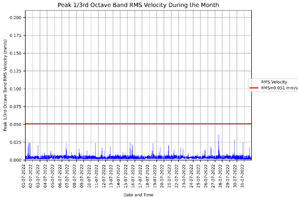
Figure 3: Measured RMSV vibration levels for 01/07/2022 to 31/07/2022 at the CASB Level 2 MRI.
