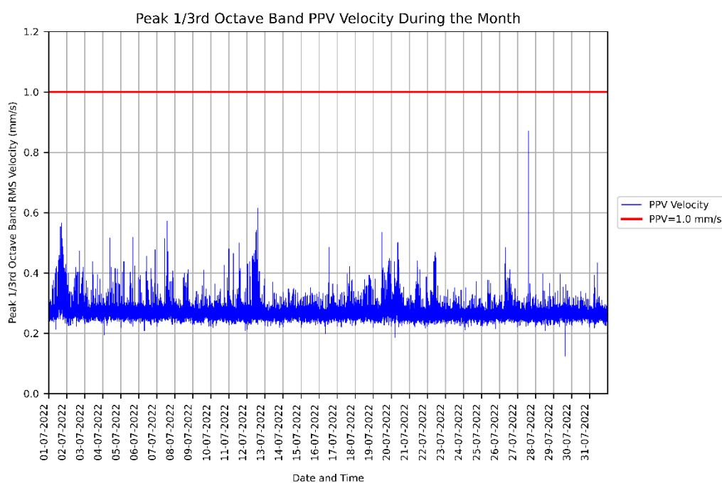
Figure 5: Measured PPV vibration levels for 01/07/2022 to 31/07/2022 at the KR - Animal House.
