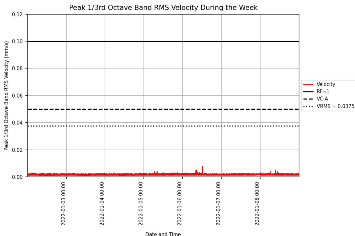
Figure 1: Measured vibration levels for 02/01/2022 to 08/01/2022 at the Medical Imaging Facility.
