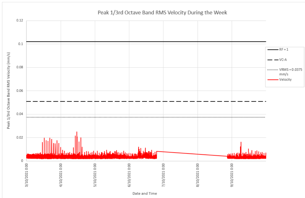
Figure 1: Measured vibration levels for 03/10/2021 to 06/10/2021 at the Medical Imaging Facility
