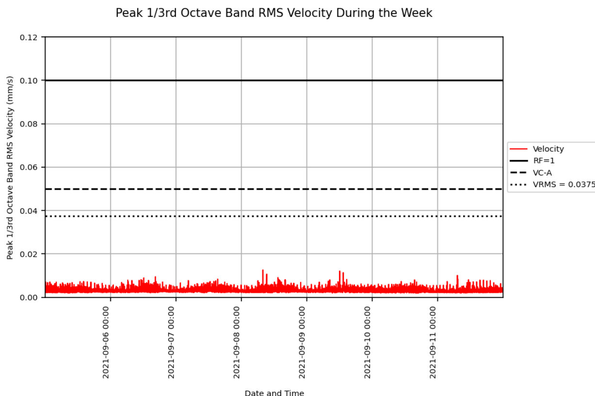
Figure 1: Measured vibration levels for 05/09/2021 to 11/09/2021 at the Medical Imaging Facility
