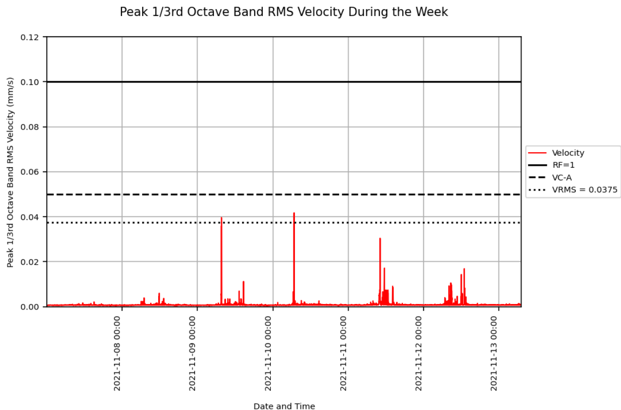
Figure 1: Measured vibration levels for 07/11/2021 to 13/11/2021 at the Medical Imaging Facility
