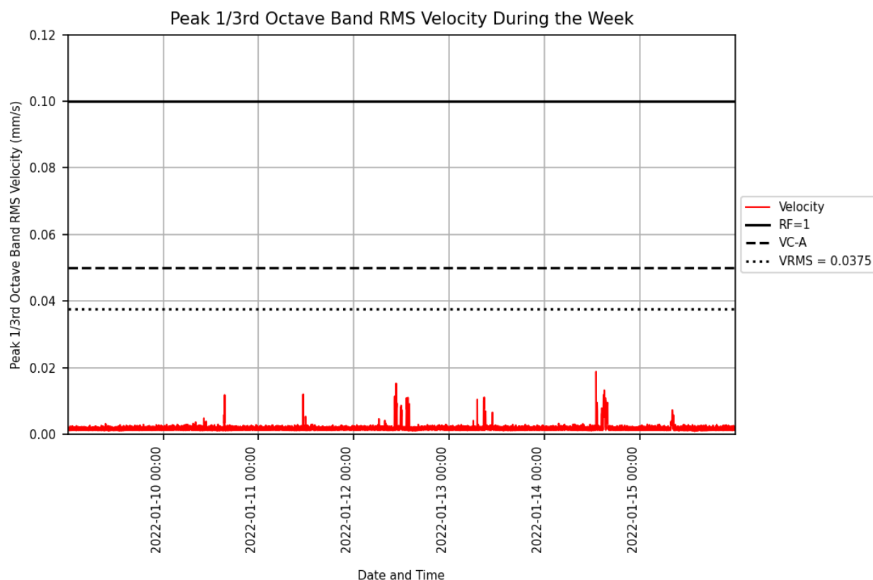
Figure 1: Measured vibration levels for 09/01/2022 to 15/01/2022 at the Medical Imaging Facility.
