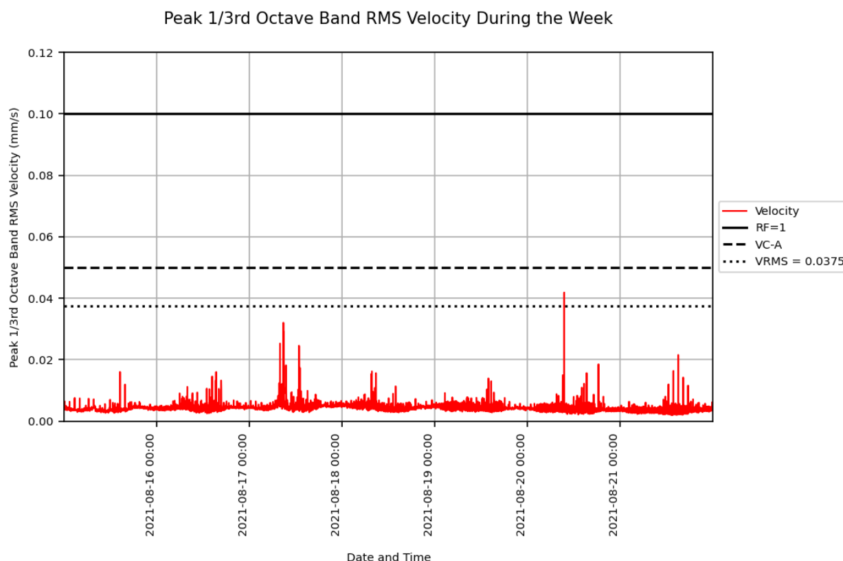
Figure 1: Measured vibration levels for 15/08/2021 to 21/08/2021 at the Medical Imaging Facility
