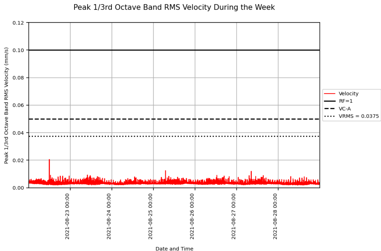
Figure 1: Measured vibration levels for 22/08/2021 to 28/08/2021 at the Medical Imaging Facility
