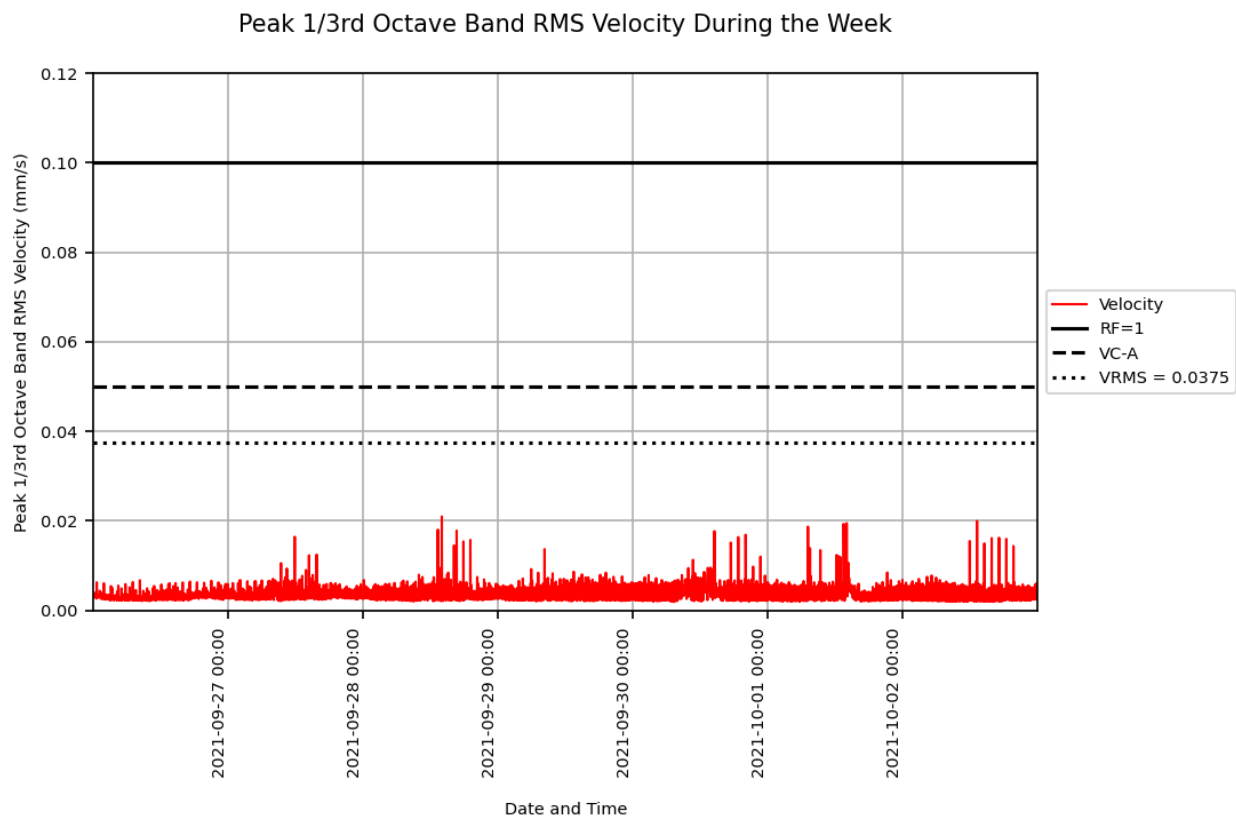
Figure 1: Measured vibration levels for 26/09/2021 to 02/10/2021 at the Medical Imaging Facility
