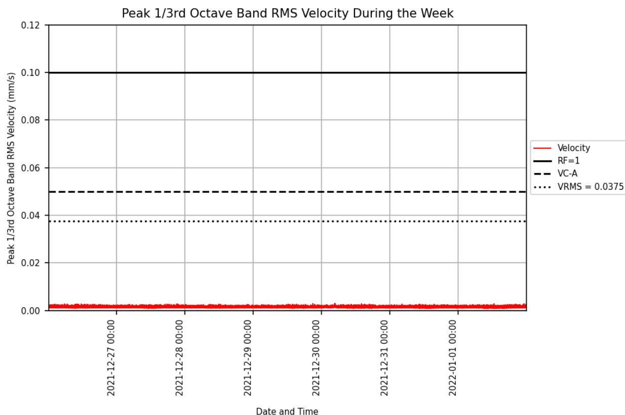
Figure 1: Measured vibration levels for 26/12/2021 to 01/01/2022 at the Medical Imaging Facility.
