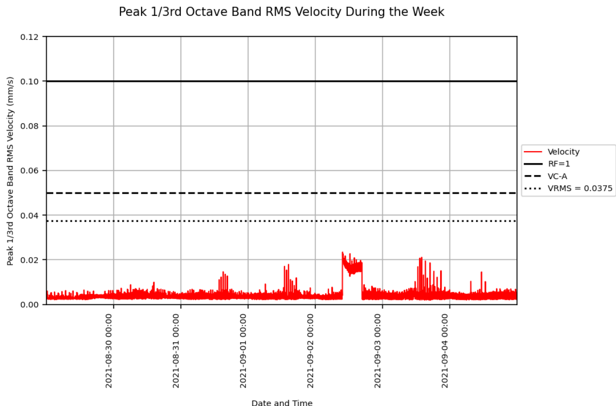
Figure 1: Measured vibration levels for 29/08/2021 to 04/09/2021 at the Medical Imaging Facility
