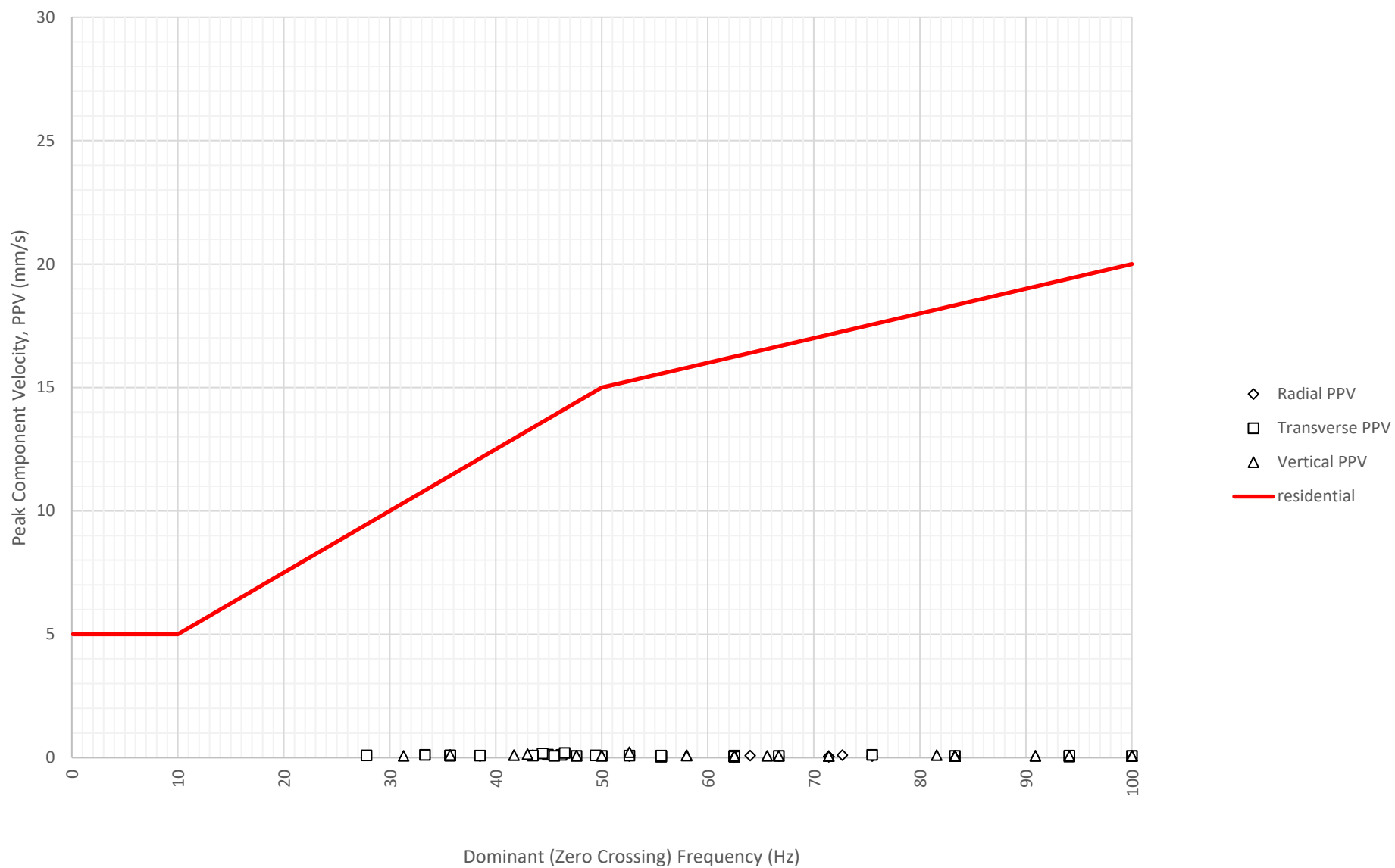
Frequency Content of Vibration Levels at East Boundary Opposite Shoalhaven Street (ETM7326) on 31-07-2024
