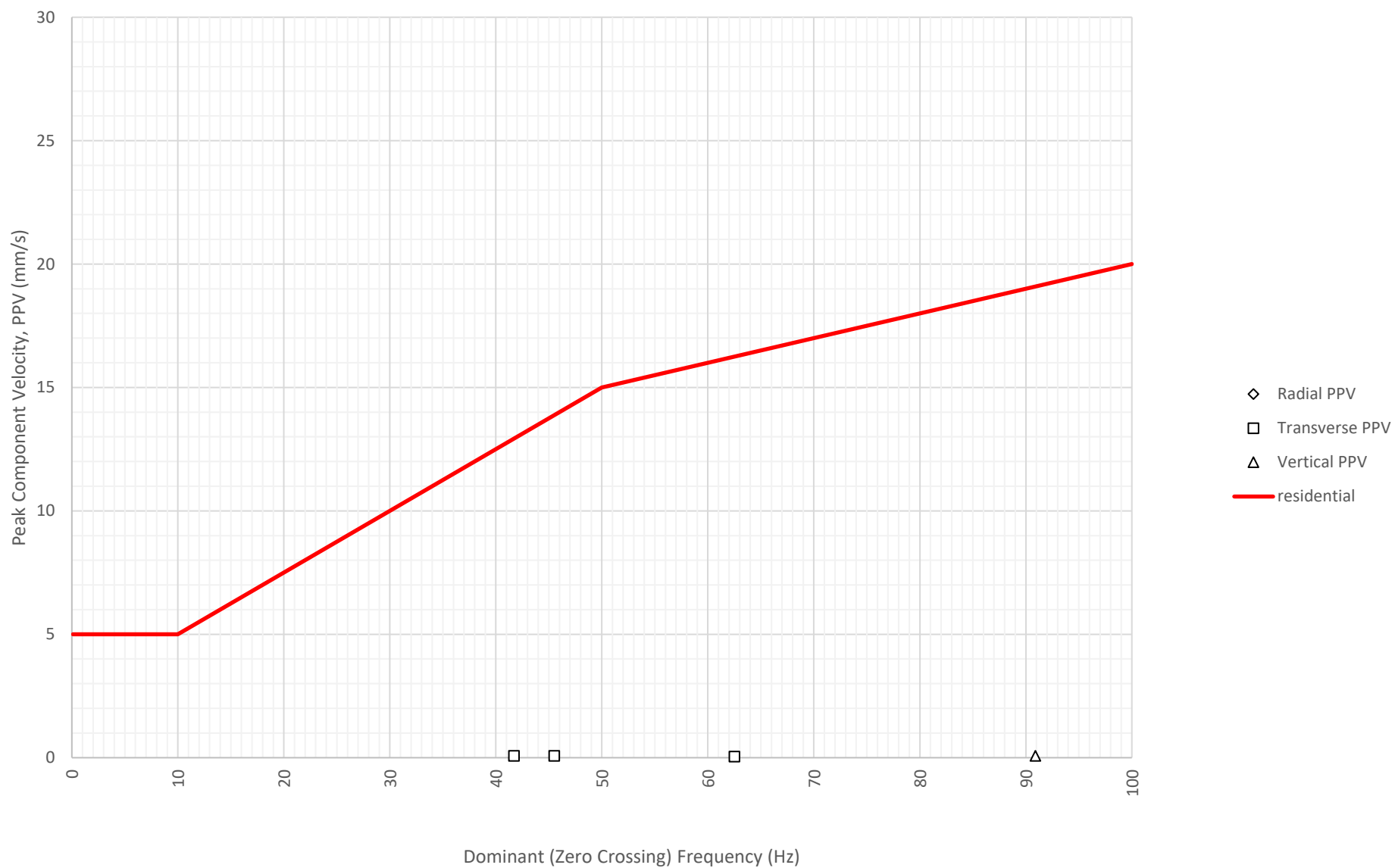
Frequency Content of Vibration Levels at East Boundary Opposite Shoalhaven Street (ETM7326) on 14-07-2024
