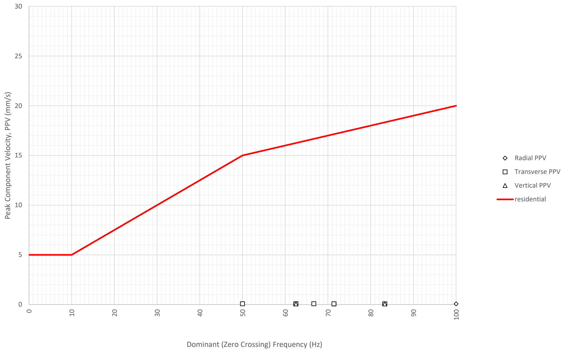
Frequency Content of Vibration Levels at North Boundary Near Block A and B (ETM7687) on 2-07-2024
