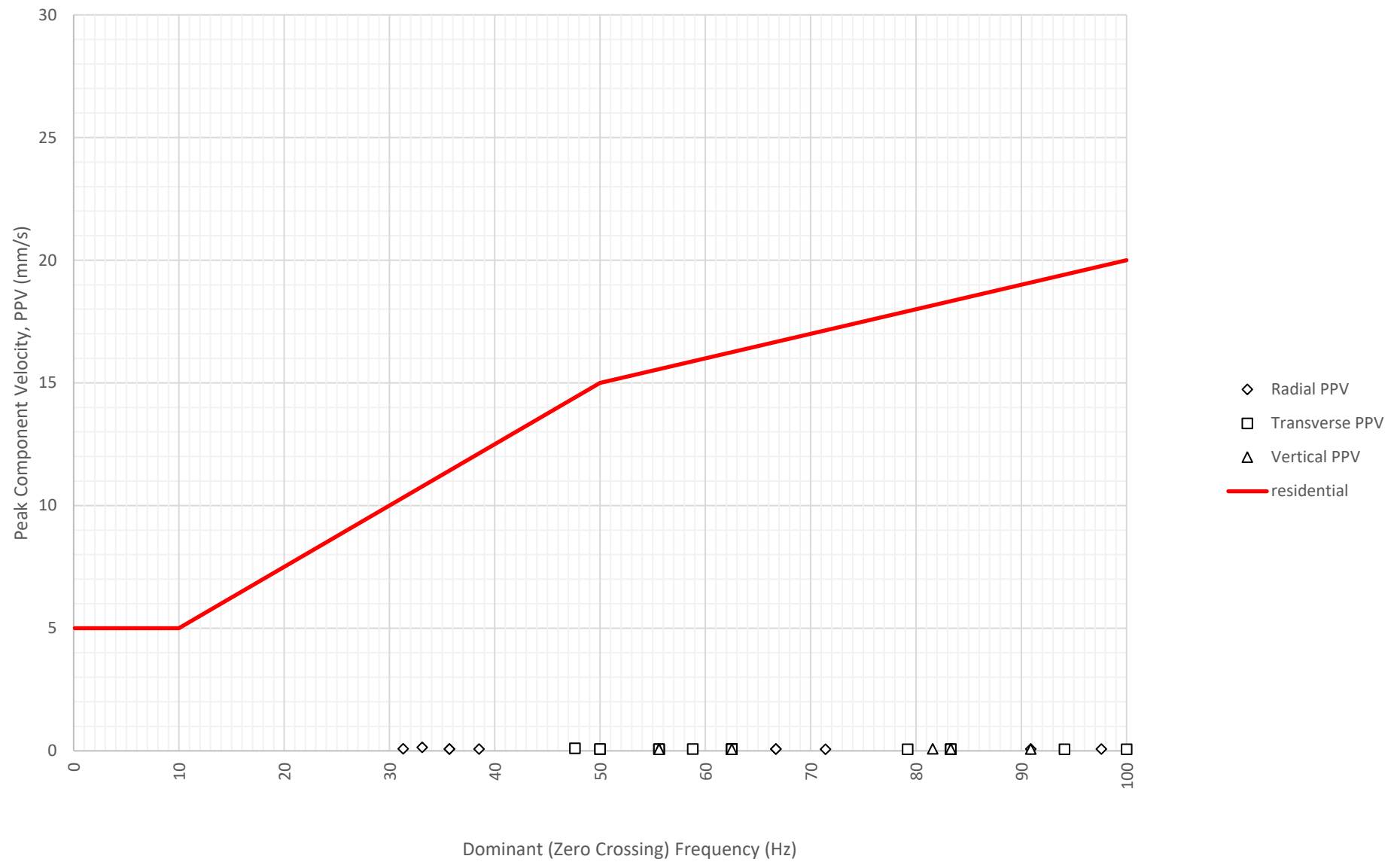
Frequency Content of Vibration Levels at North Boundary Near Block A and B (ETM7687) on 30-07-2024
