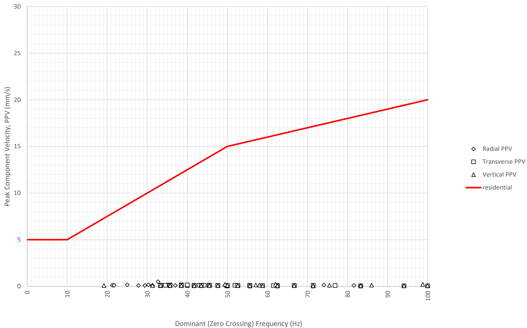
Frequency Content of Vibration Levels at East Boundary Opposite Shoalhaven Street (ETM7326) on 15-07-2024
