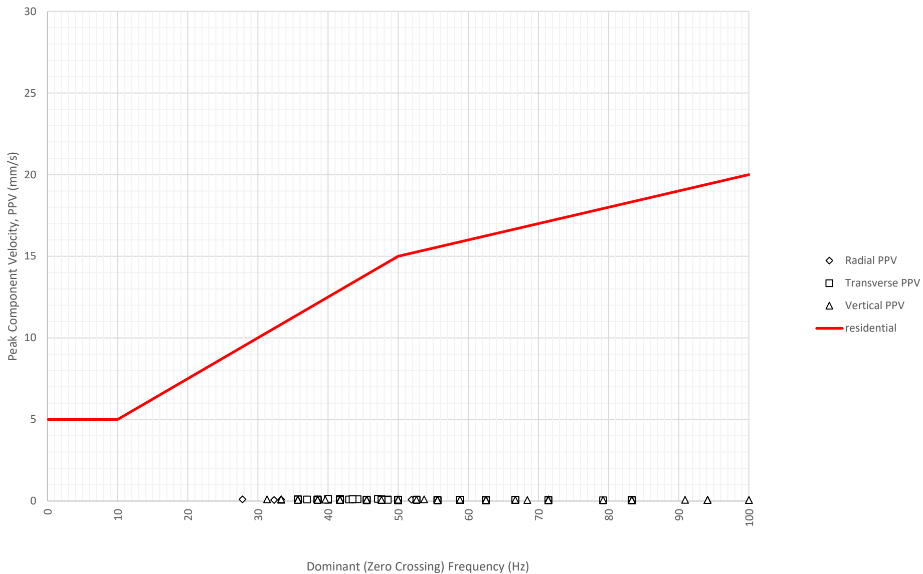
Frequency Content of Vibration Levels at East Boundary Opposite Shoalhaven Street (ETM7326) on 27-07-2024
