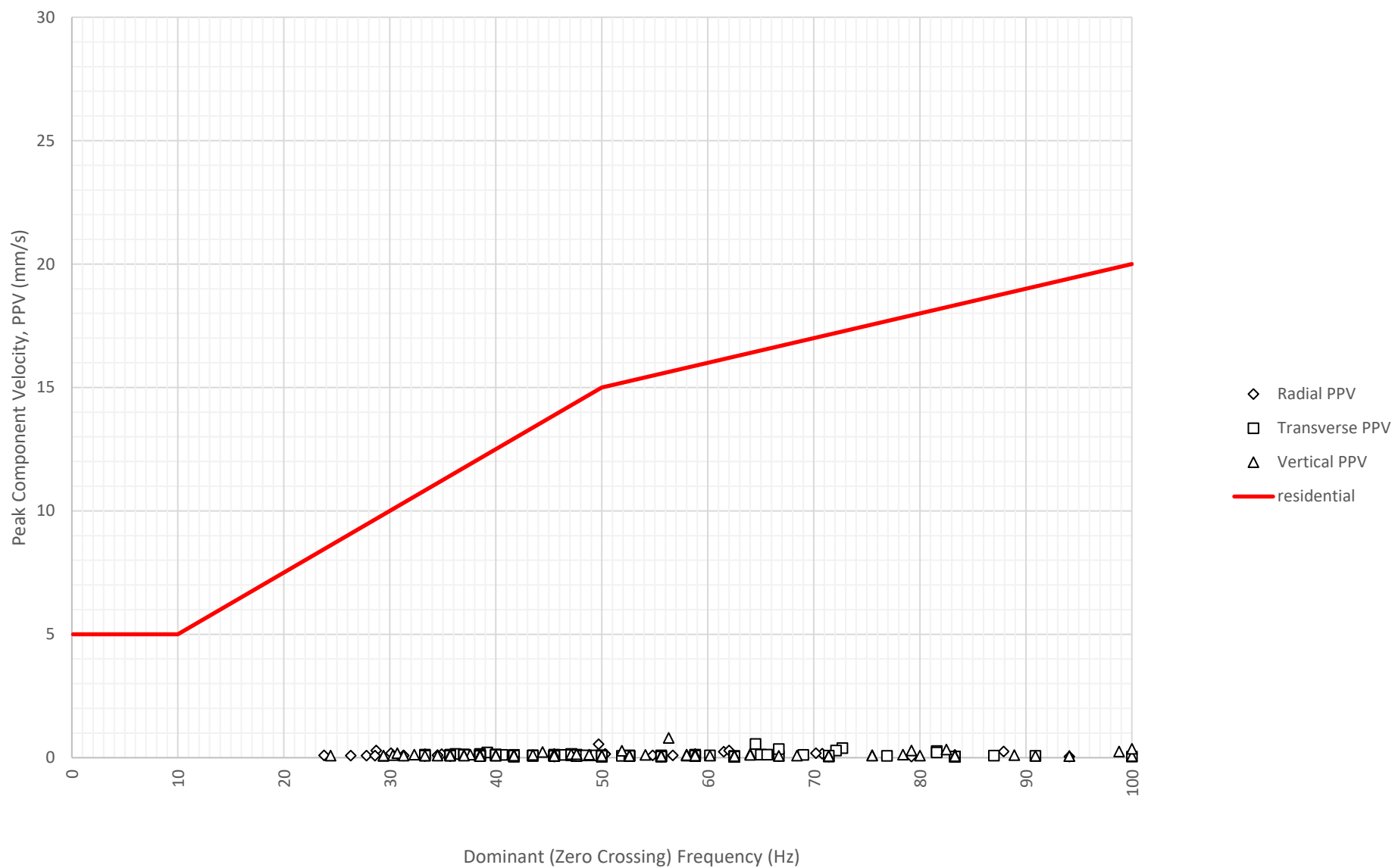
Frequency Content of Vibration Levels at East Boundary Opposite Shoalhaven Street (ETM7326) on 29-07-2024
