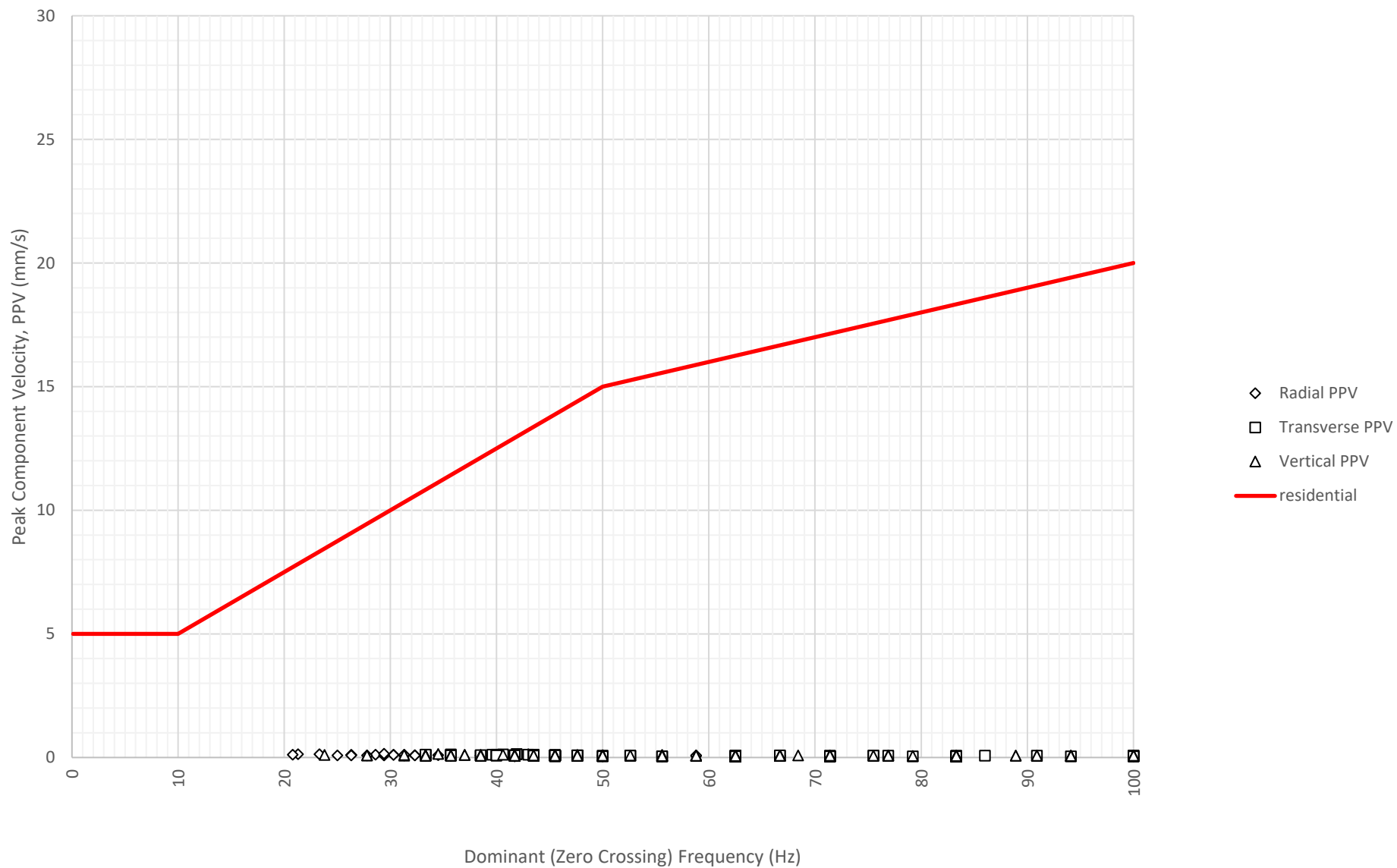
Frequency Content of Vibration Levels at East Boundary Opposite Shoalhaven Street (ETM7326) on 2-07-2024
