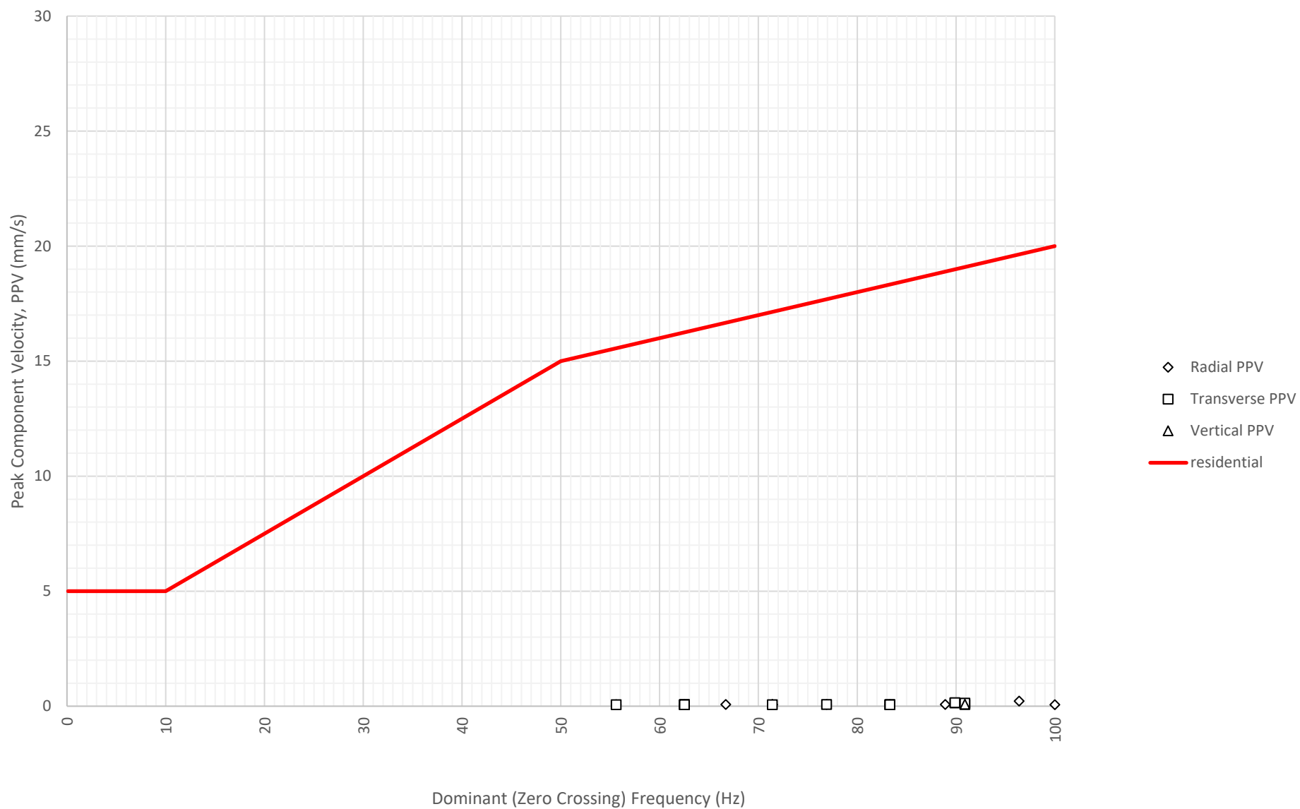
Frequency Content of Vibration Levels at North Boundary Near Block A and B (ETM7687) on 11-07-2024
