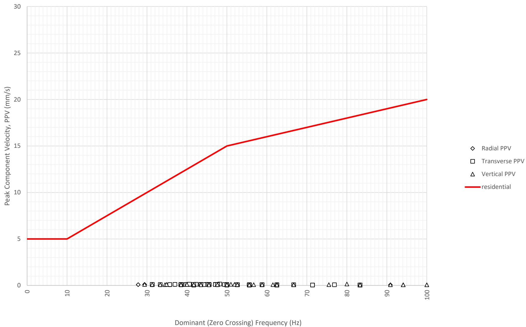
Frequency Content of Vibration Levels at East Boundary Opposite Shoalhaven Street (ETM7326) on 19-07-2024
