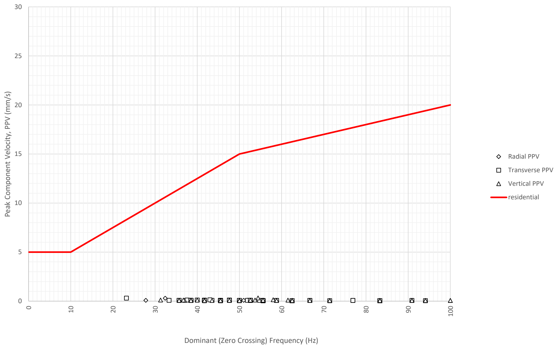
Frequency Content of Vibration Levels at East Boundary Opposite Shoalhaven Street (ETM7326) on 20-07-2024
