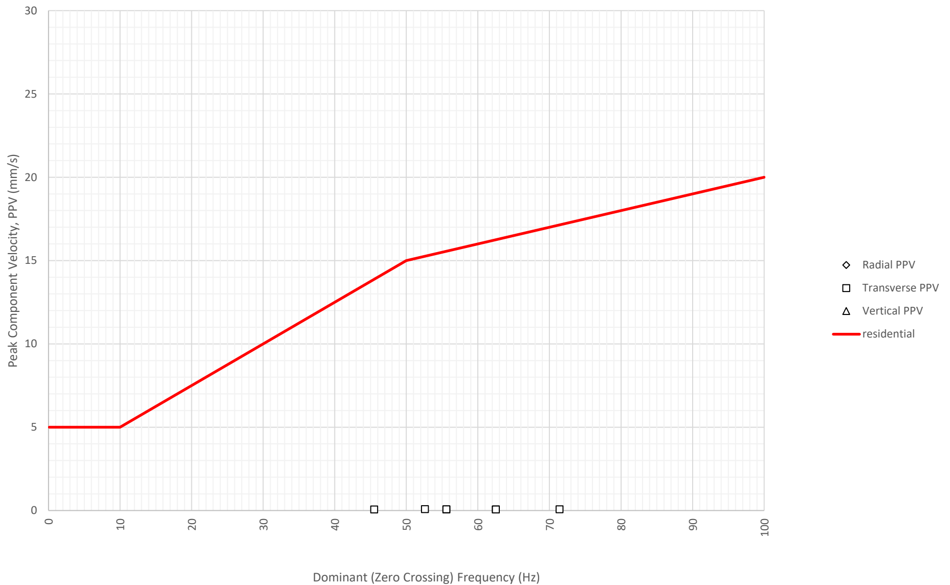
Frequency Content of Vibration Levels at North Boundary Near Block A and B (ETM7687) on 3-07-2024
