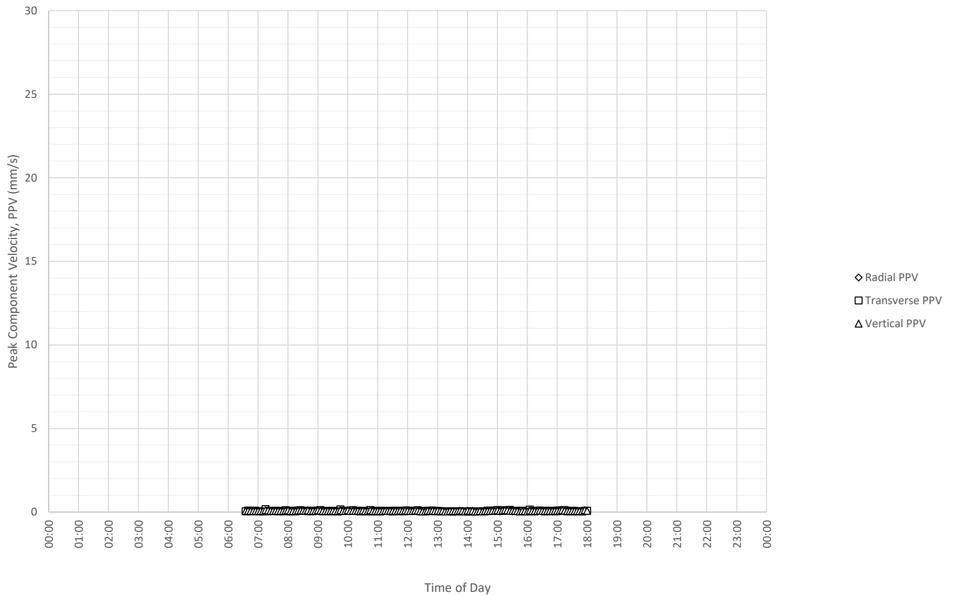
Daily Monitored Vibration Levels at East Boundary Opposite Shoalhaven Street (ETM7326) on 26-07-2024
