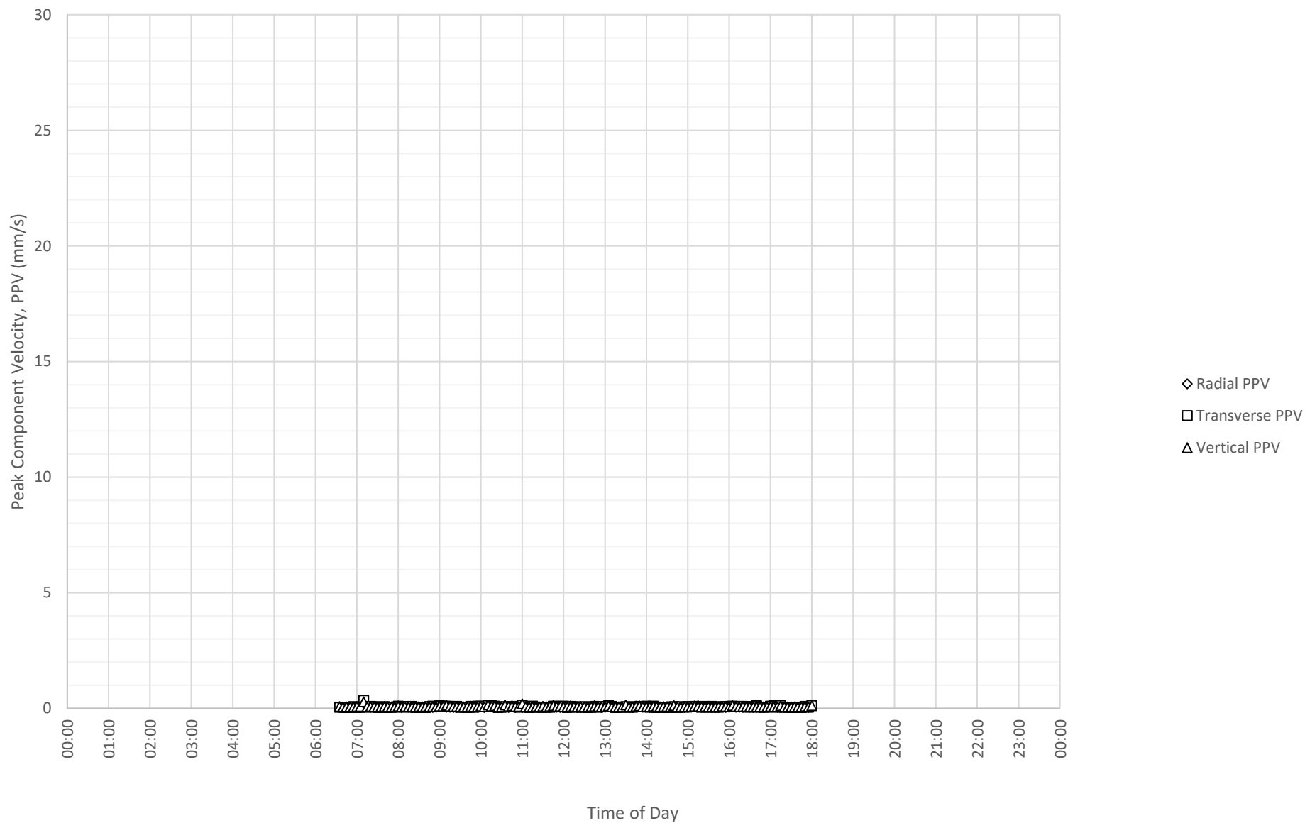
Daily Monitored Vibration Levels at East Boundary Opposite Shoalhaven Street (ETM7326) on 11-07-2024
