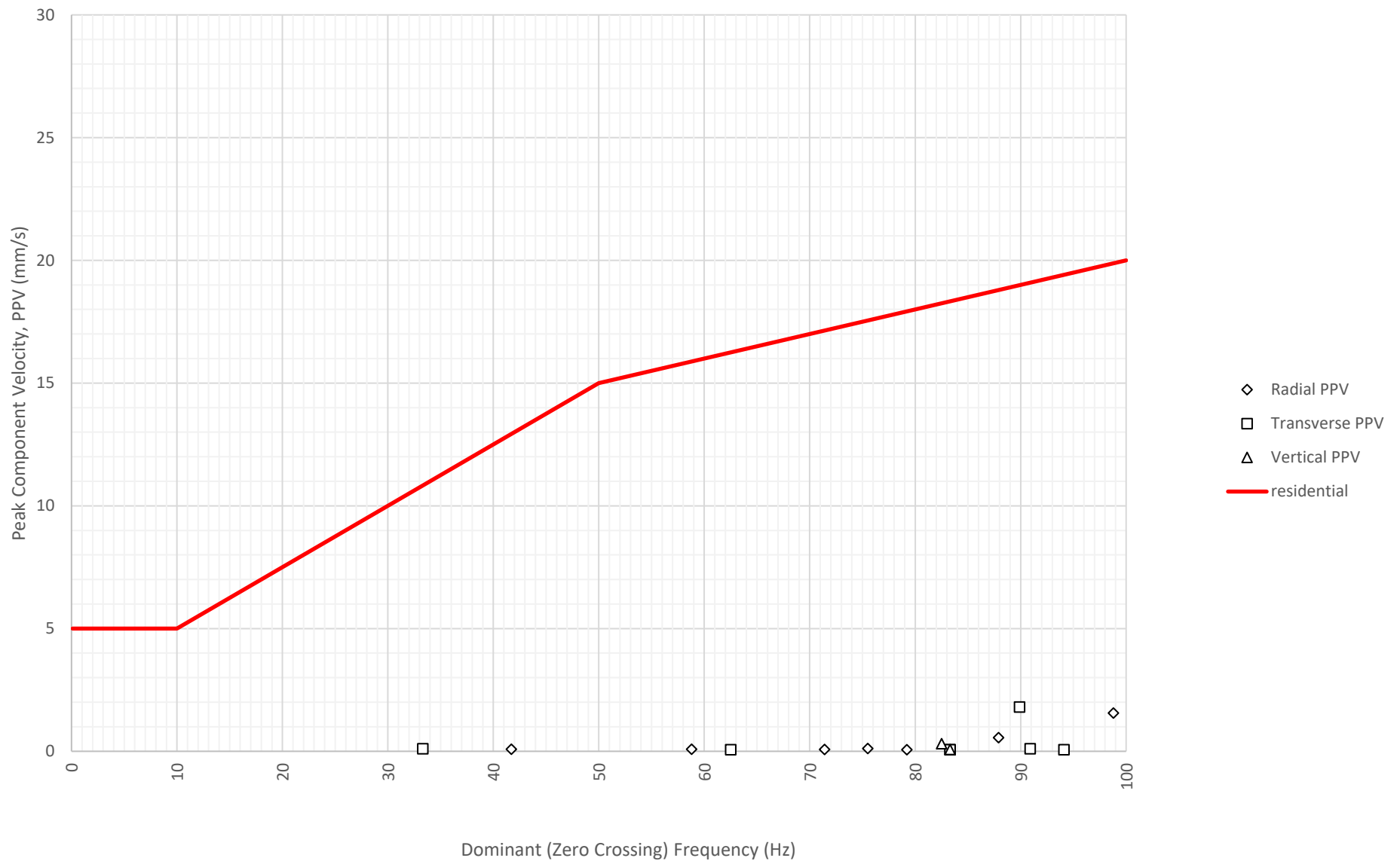
Frequency Content of Vibration Levels at North Boundary Near Block A and B (ETM7687) on 15-07-2024
