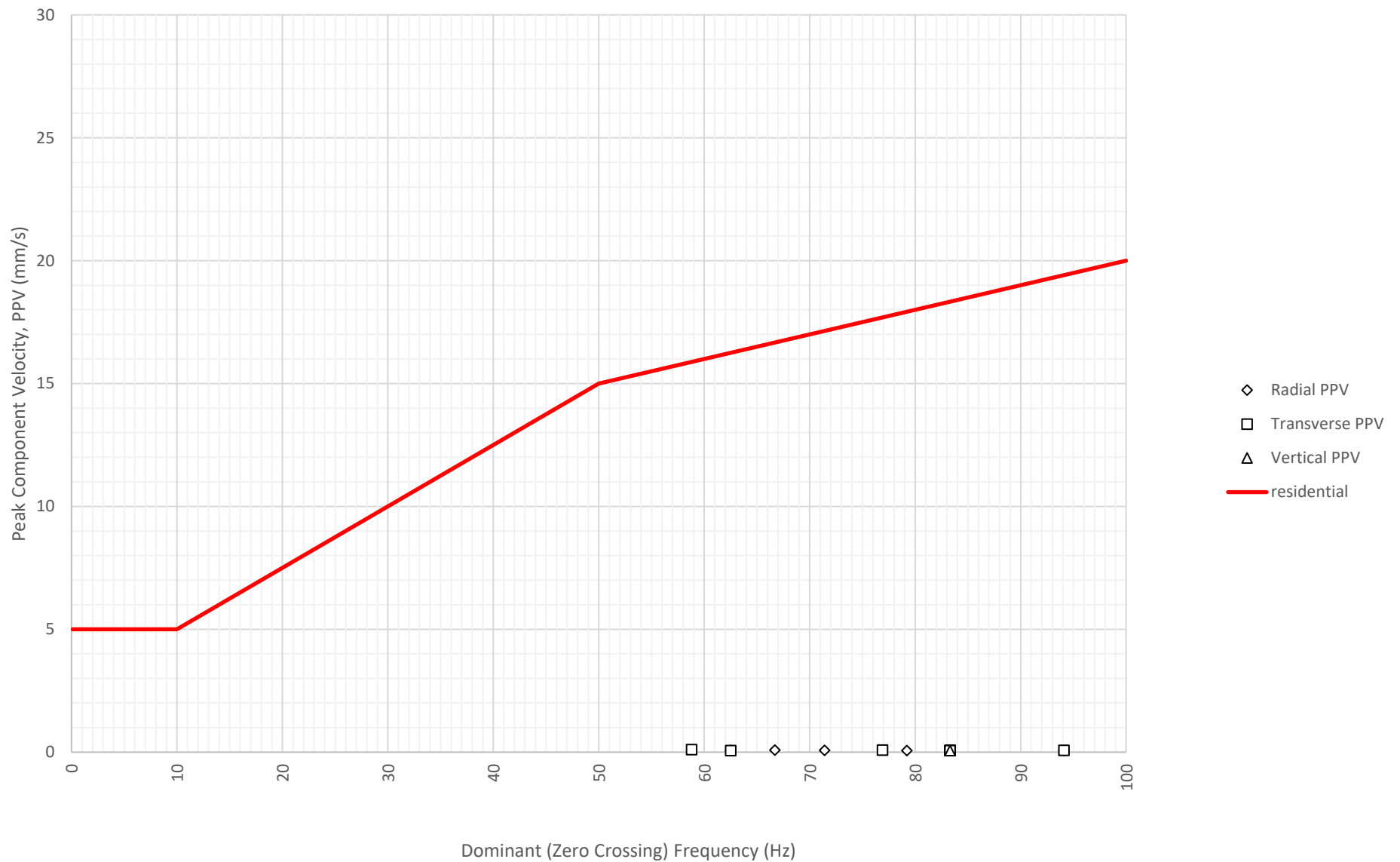
Frequency Content of Vibration Levels at North Boundary Near Block A and B (ETM7687) on 12-07-2024
