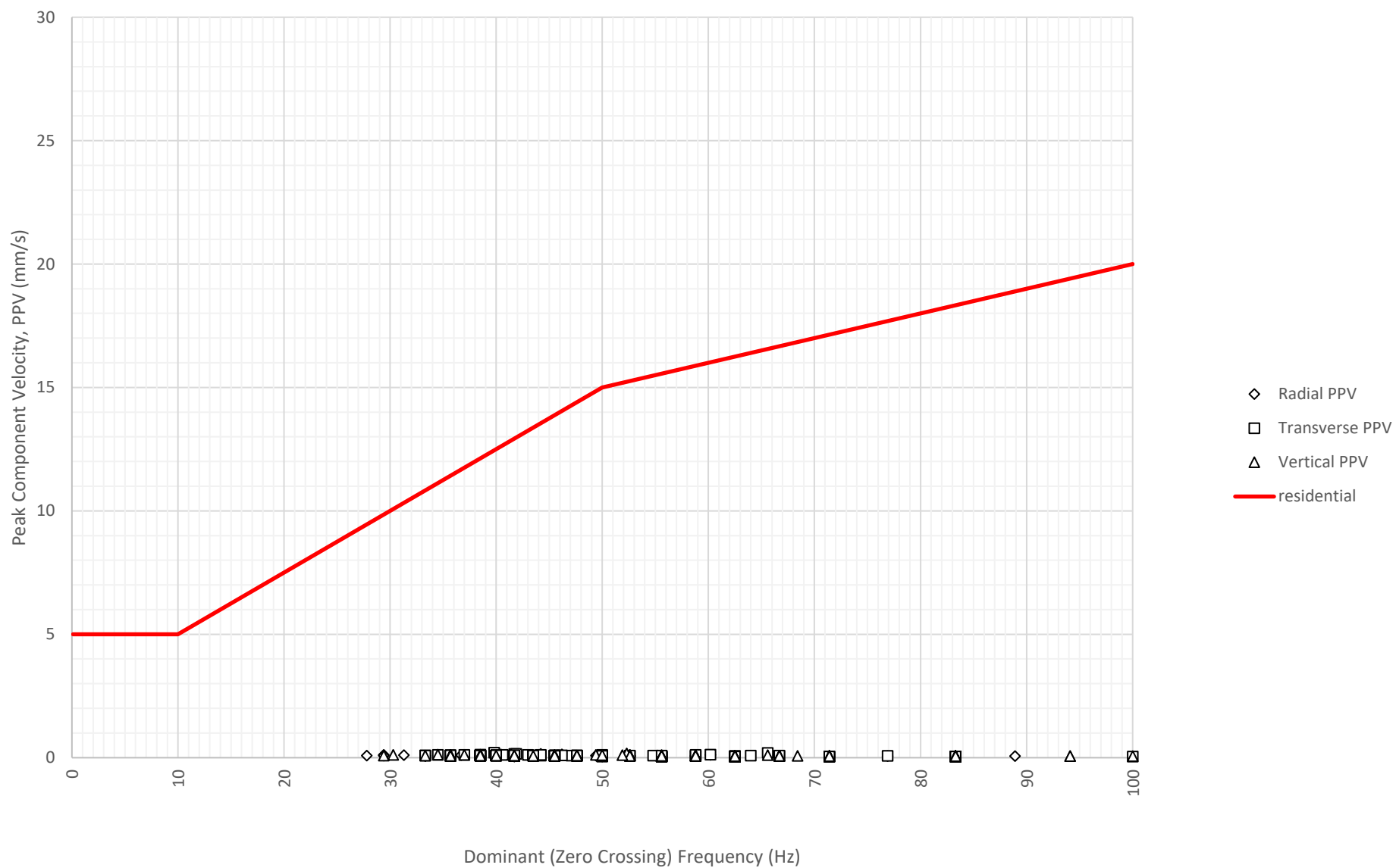
Frequency Content of Vibration Levels at East Boundary Opposite Shoalhaven Street (ETM7326) on 25-07-2024
