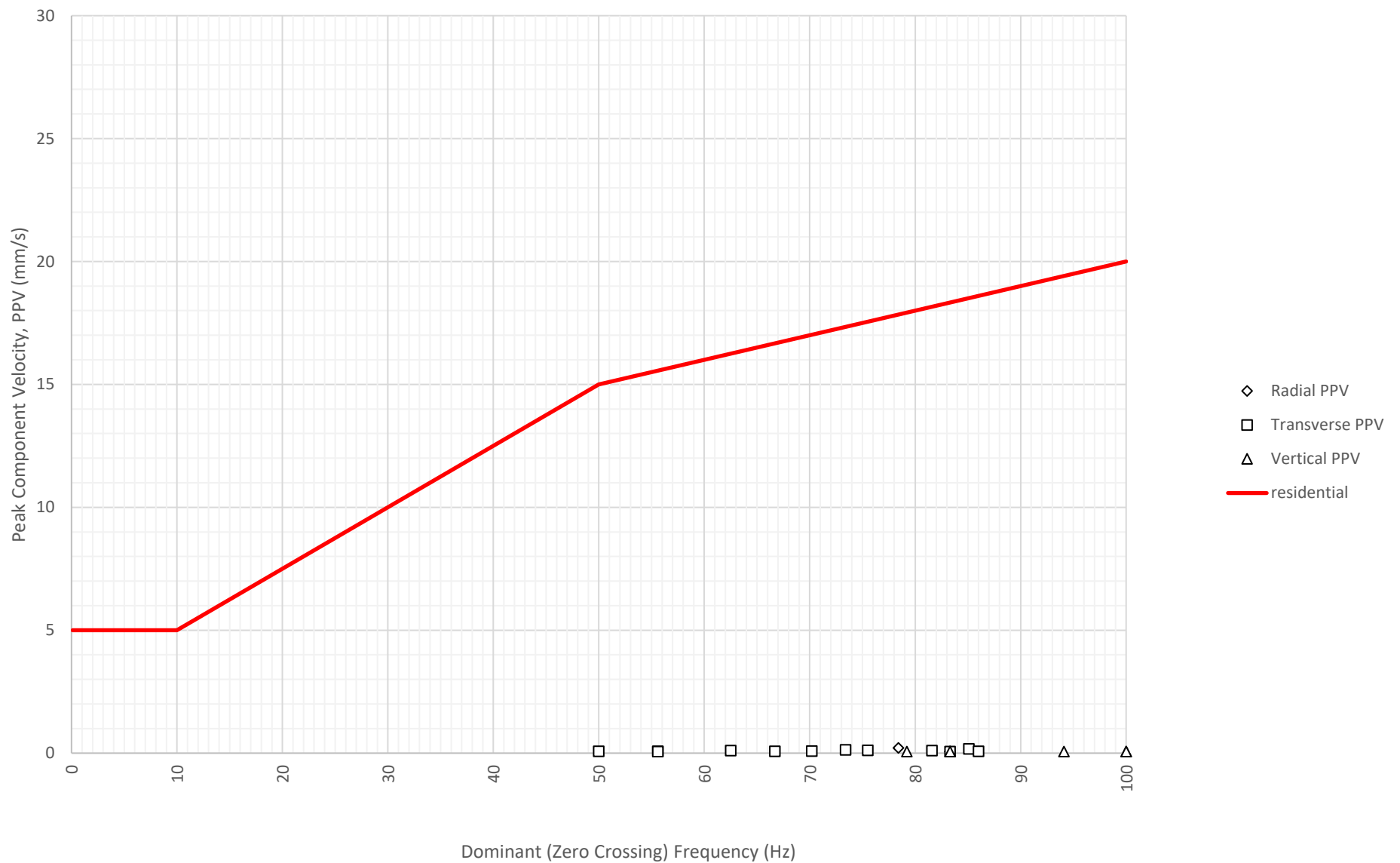
Frequency Content of Vibration Levels at North Boundary Near Block A and B (ETM7687) on 1-07-2024
