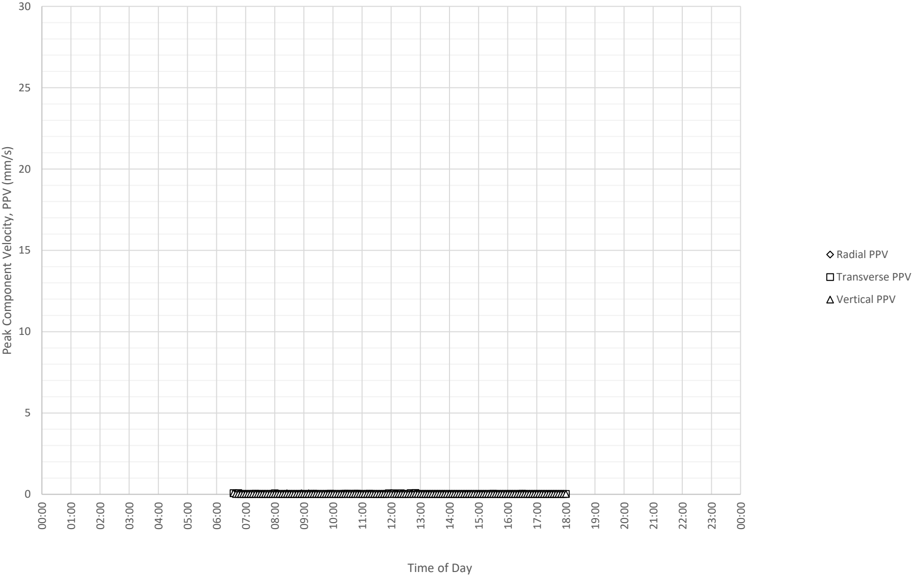
Daily Monitored Vibration Levels at North Boundary Near Block A and B (ETM7687) on 3-07-2024
