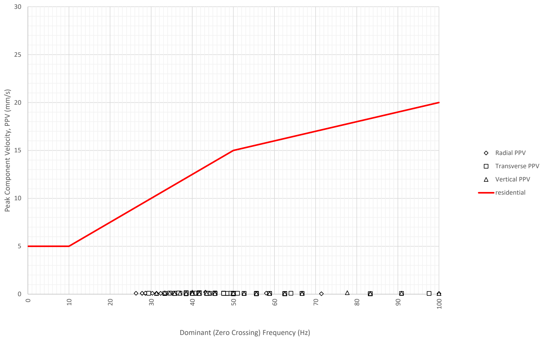
Frequency Content of Vibration Levels at East Boundary Opposite Shoalhaven Street (ETM7326) on 18-07-2024
