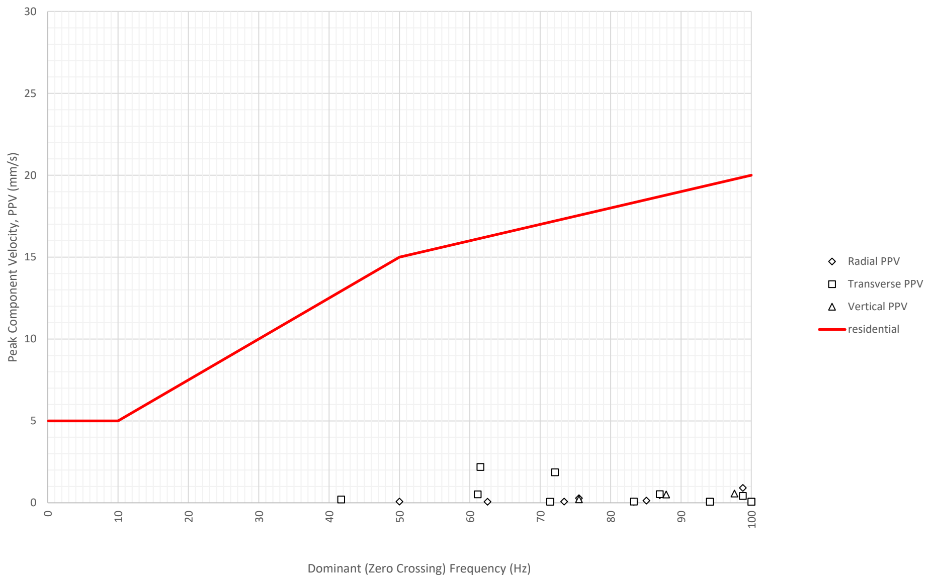
Frequency Content of Vibration Levels at North Boundary Near Block A and B (ETM7687) on 17-07-2024
