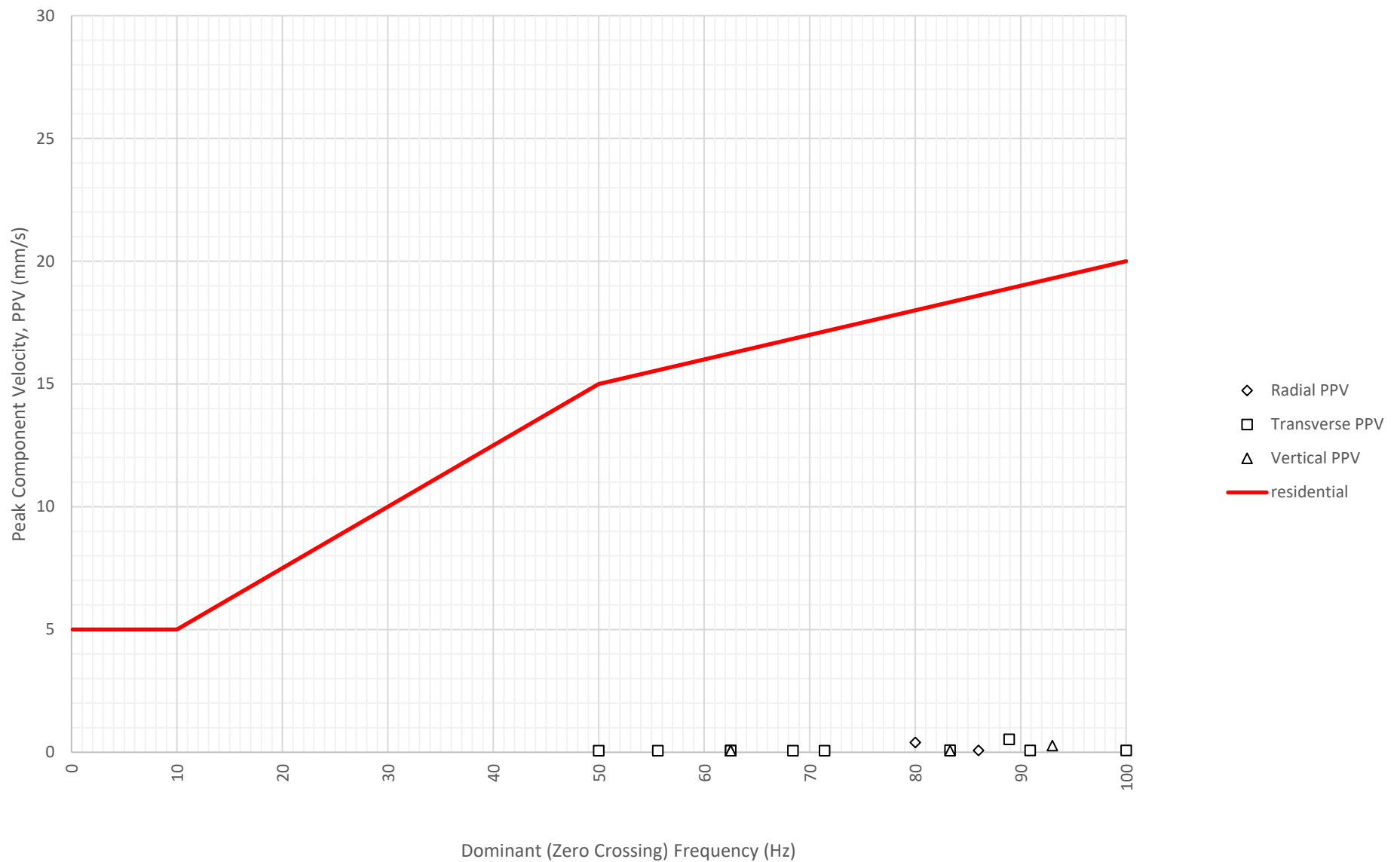
Frequency Content of Vibration Levels at North Boundary Near Block A and B (ETM7687) on 8-07-2024
