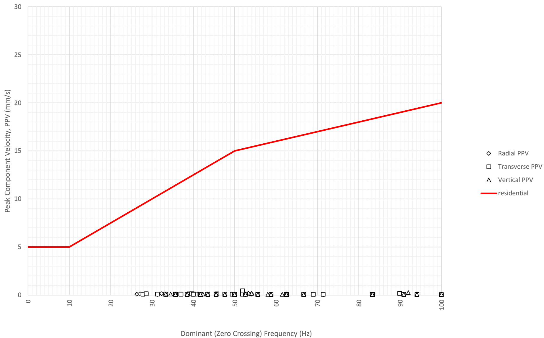
Frequency Content of Vibration Levels at East Boundary Opposite Shoalhaven Street (ETM7326) on 17-07-2024
