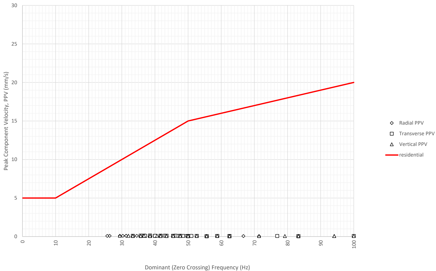
Frequency Content of Vibration Levels at East Boundary Opposite Shoalhaven Street (ETM7326) on 13-07-2024
