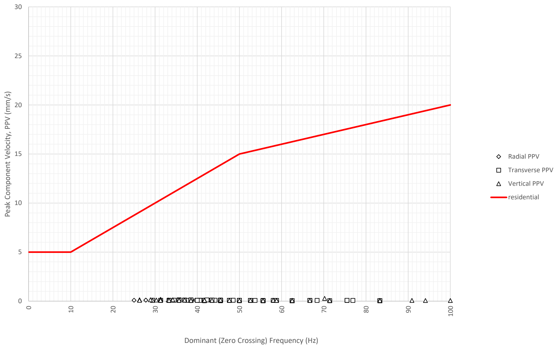
Frequency Content of Vibration Levels at East Boundary Opposite Shoalhaven Street (ETM7326) on 11-07-2024
