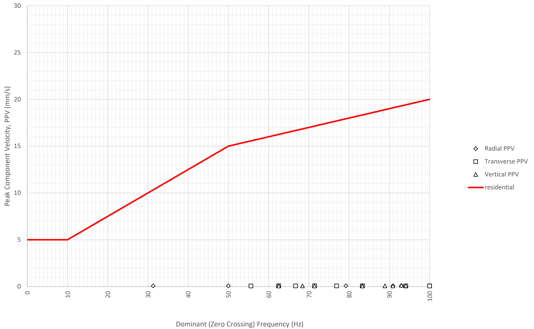
Frequency Content of Vibration Levels at North Boundary Near Block A and B (ETM7687) on 29-07-2024
