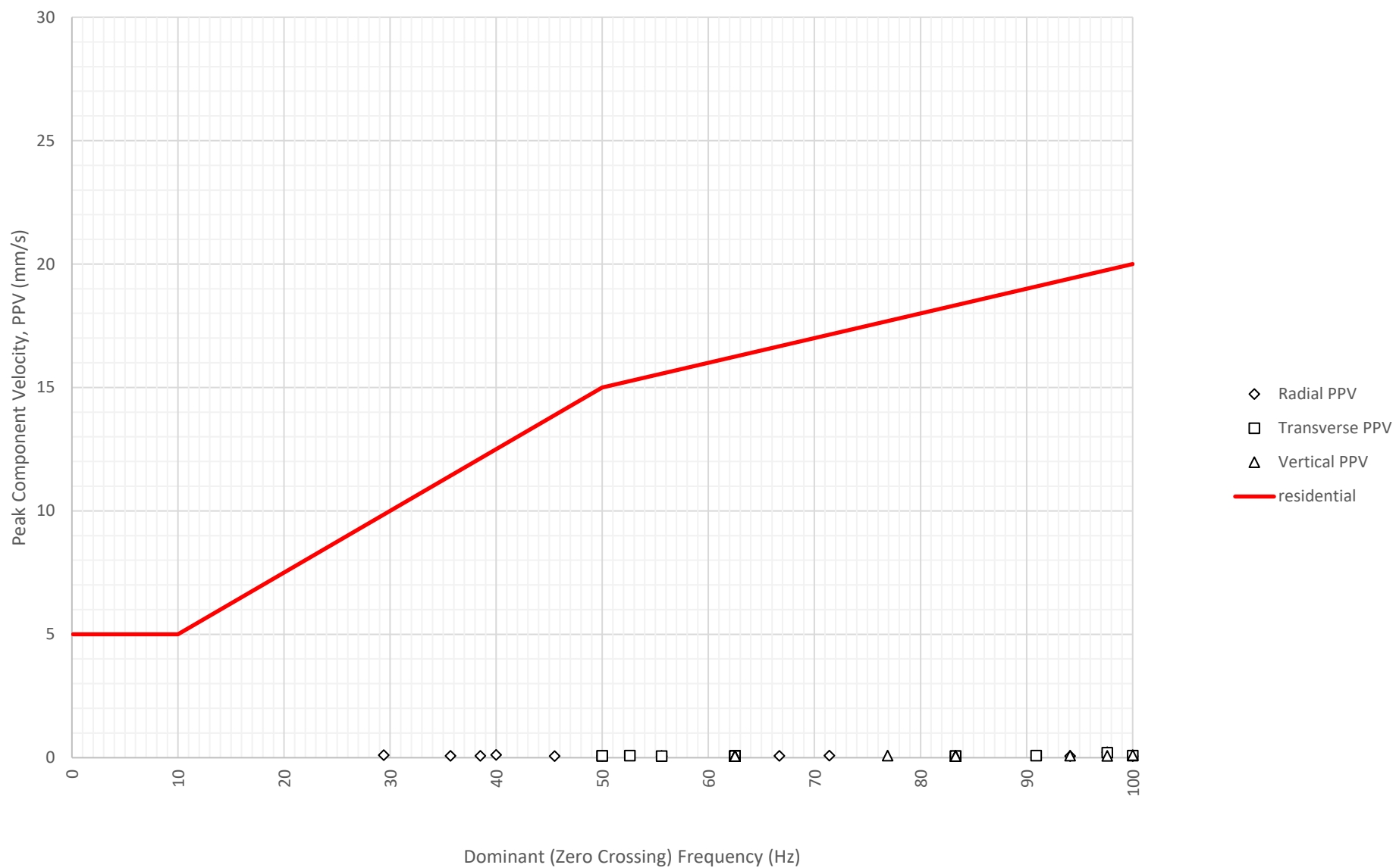
Frequency Content of Vibration Levels at North Boundary Near Block A and B (ETM7687) on 23-07-2024
