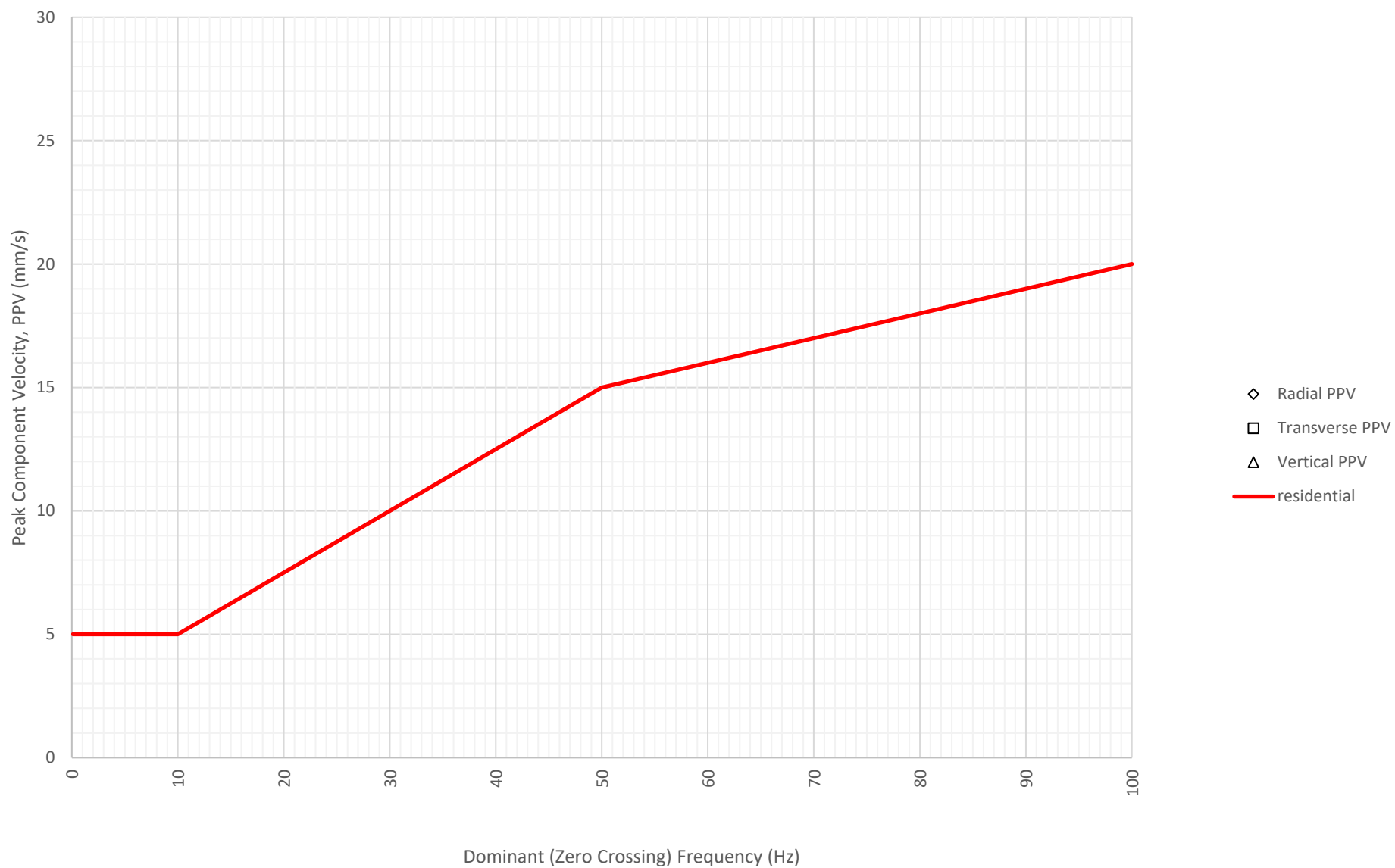
Frequency Content of Vibration Levels at North Boundary Near Block A and B (ETM7687) on 13-07-2024
