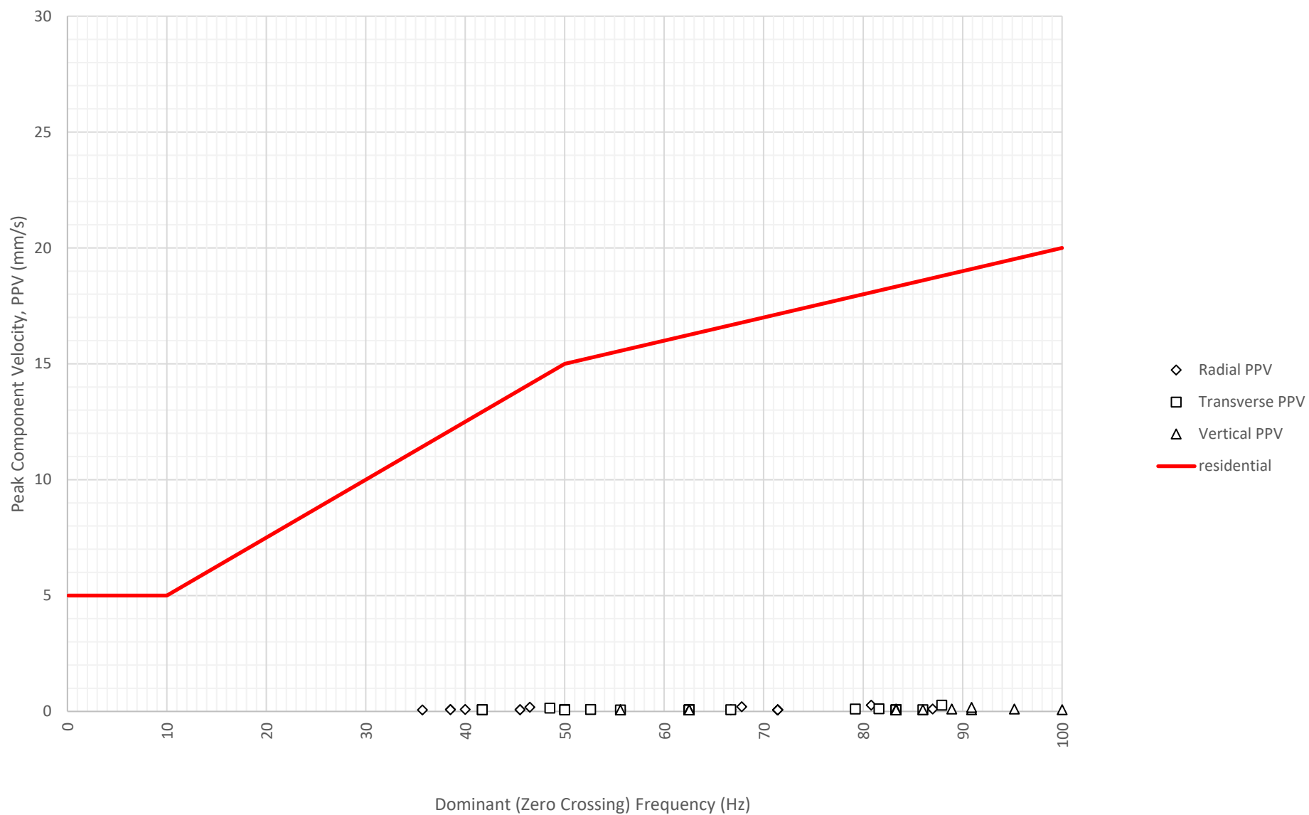
Frequency Content of Vibration Levels at North Boundary Near Block A and B (ETM7687) on 31-07-2024
