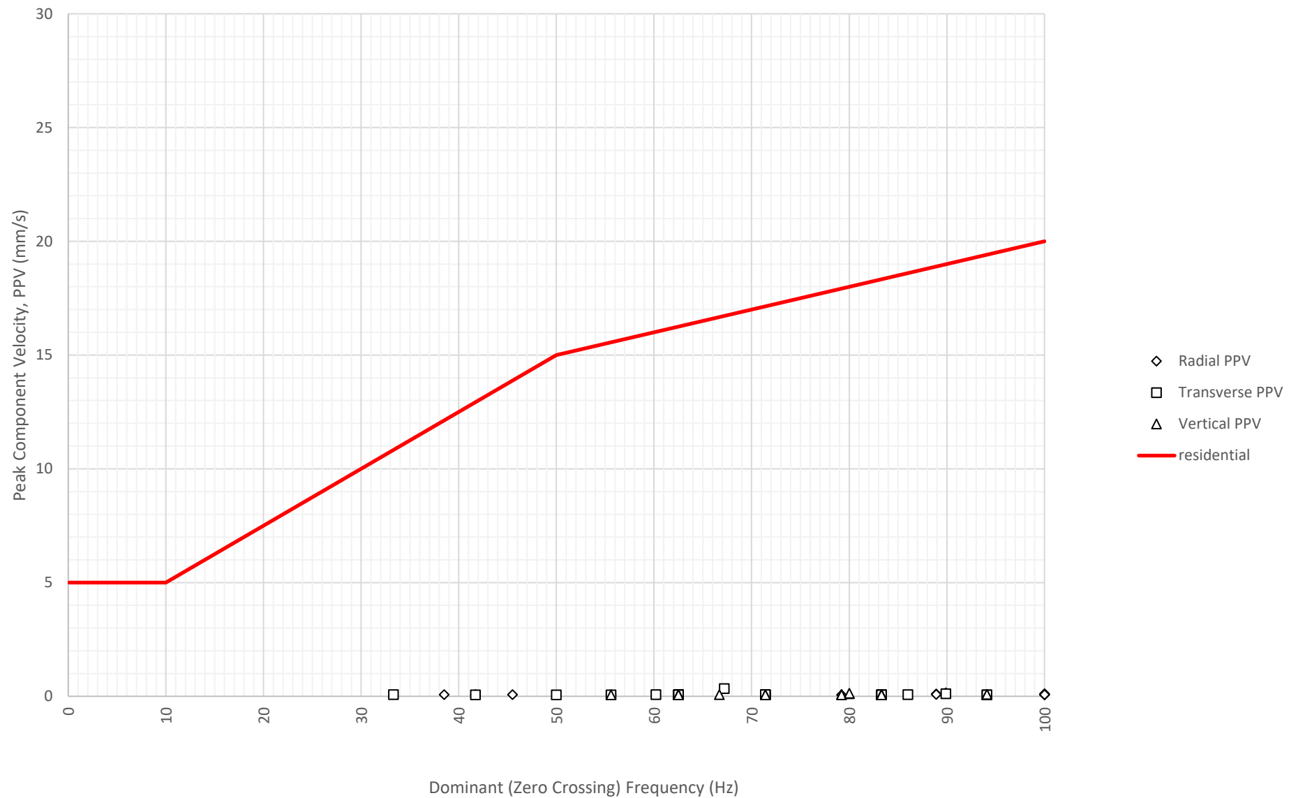
Frequency Content of Vibration Levels at North Boundary Near Block A and B (ETM7687) on 26-07-2024
