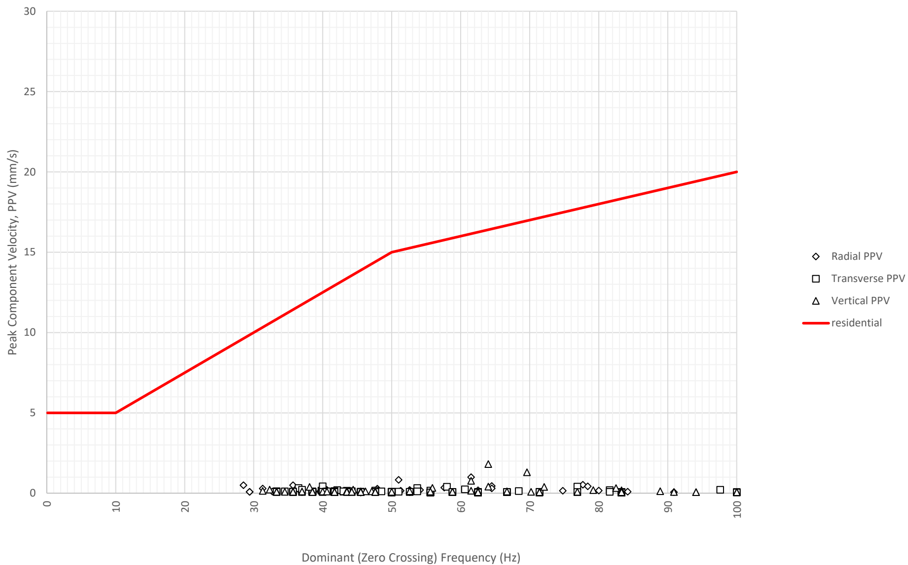
Frequency Content of Vibration Levels at East Boundary Opposite Shoalhaven Street (ETM7326) on 22-07-2024
