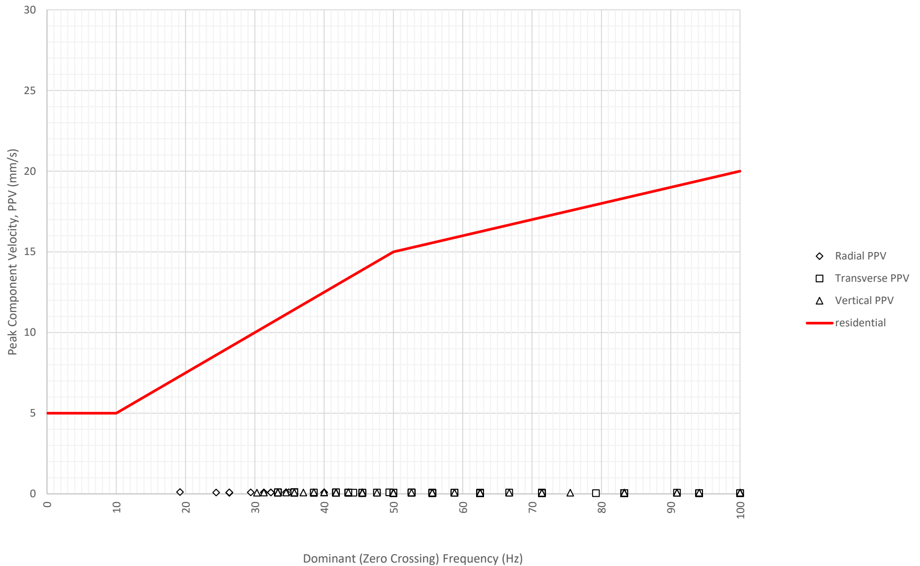
Frequency Content of Vibration Levels at East Boundary Opposite Shoalhaven Street (ETM7326) on 6-07-2024
