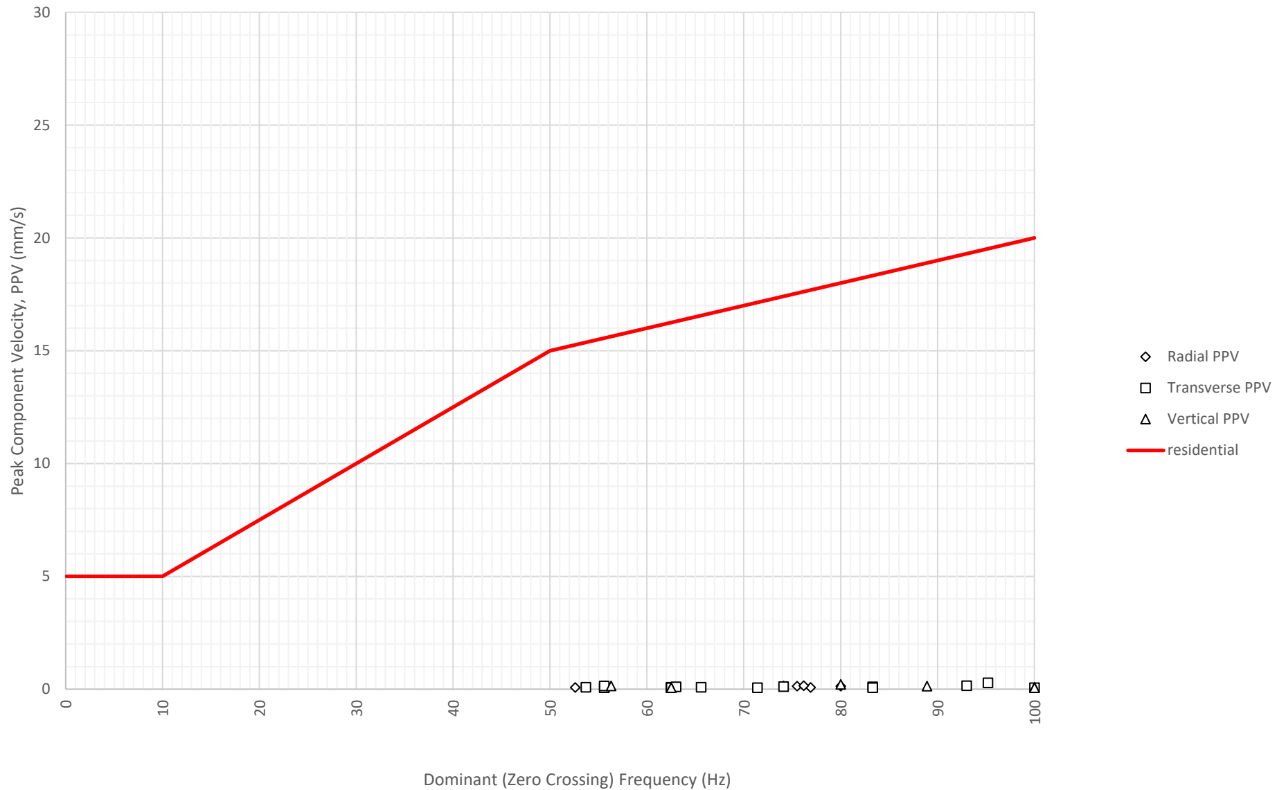
Frequency Content of Vibration Levels at North Boundary Near Block A and B (ETM7687) on 4-07-2024
