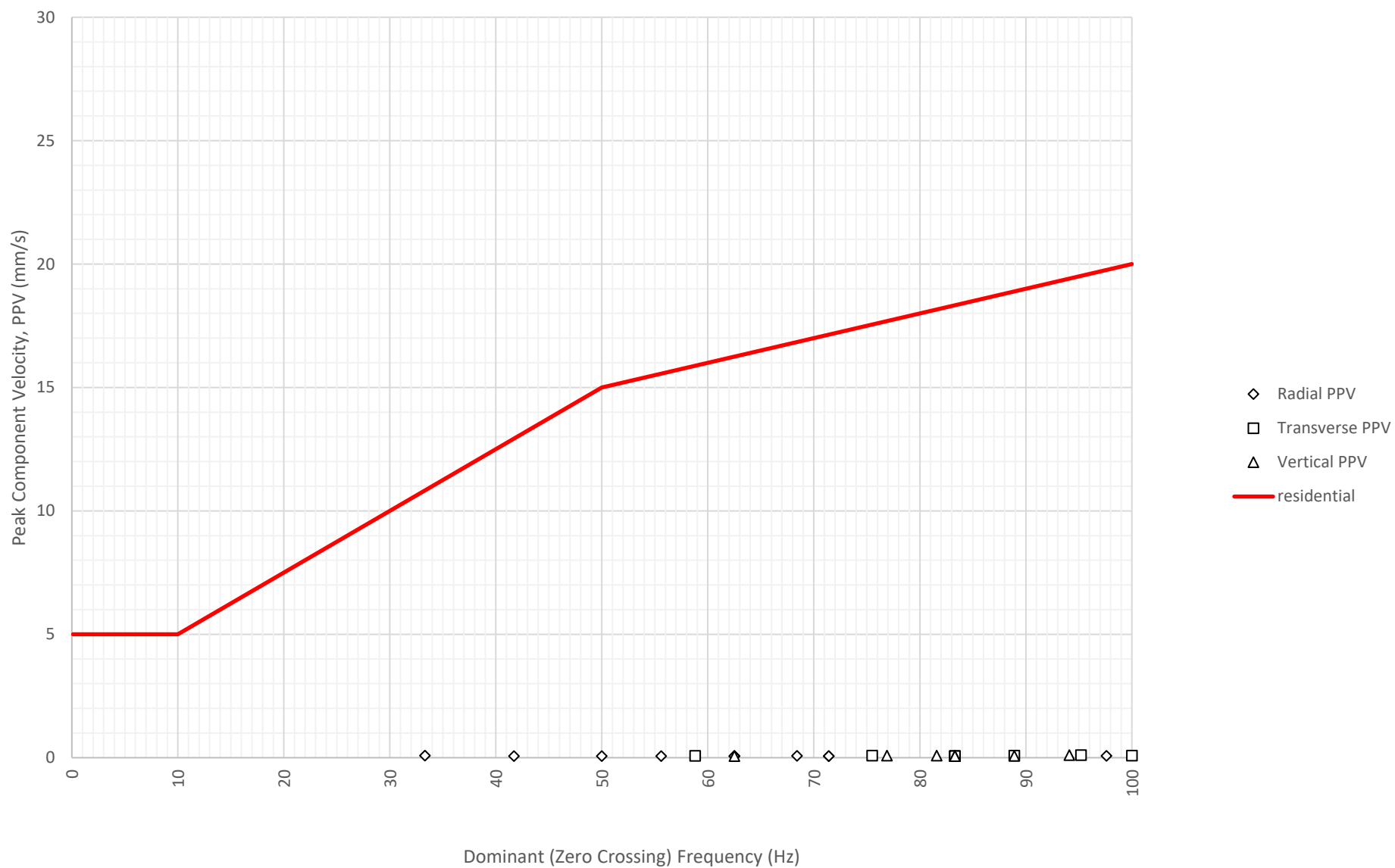
Frequency Content of Vibration Levels at North Boundary Near Block A and B (ETM7687) on 19-07-2024
