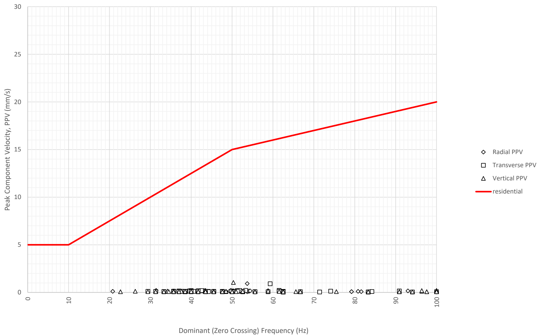
Frequency Content of Vibration Levels at East Boundary Opposite Shoalhaven Street (ETM7326) on 30-07-2024
