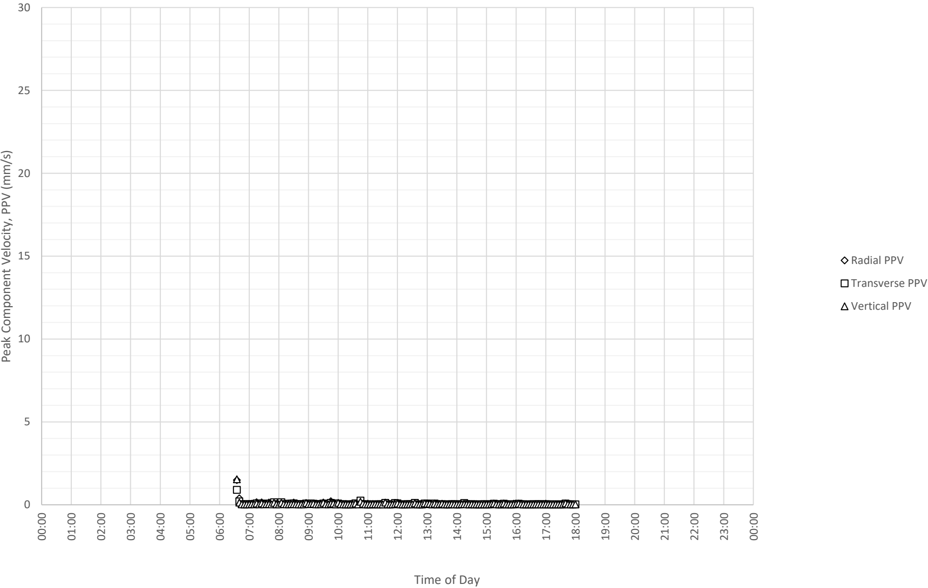
Daily Monitored Vibration Levels at North Boundary Near Block A and B (ETM7687) on 18-07-2024
