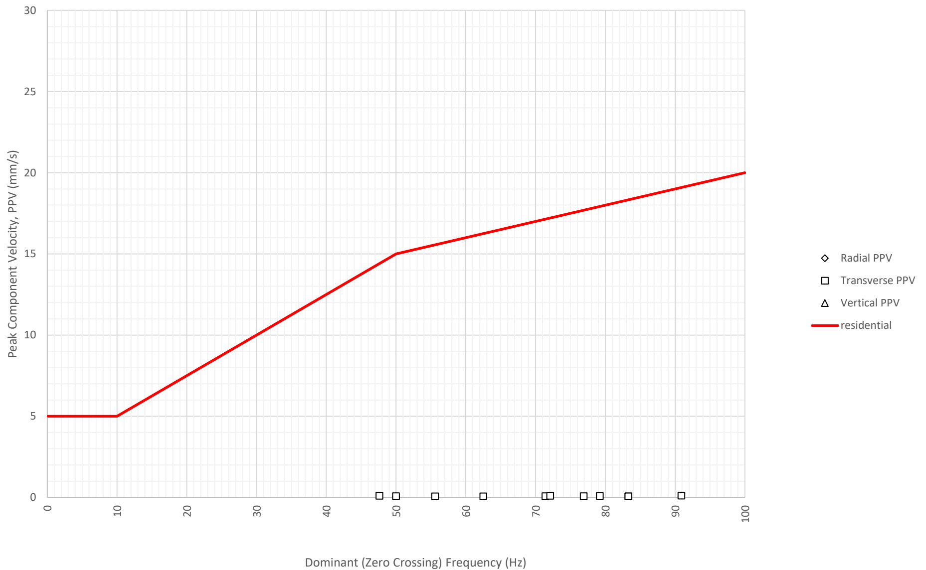
Frequency Content of Vibration Levels at North Boundary Near Block A and B (ETM7687) on 5-07-2024
