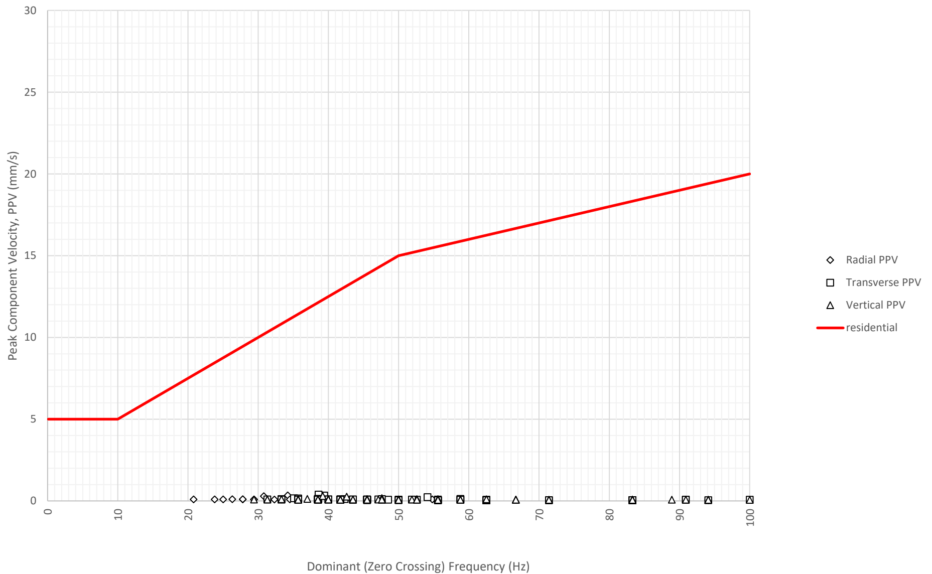
Frequency Content of Vibration Levels at East Boundary Opposite Shoalhaven Street (ETM7326) on 16-07-2024
