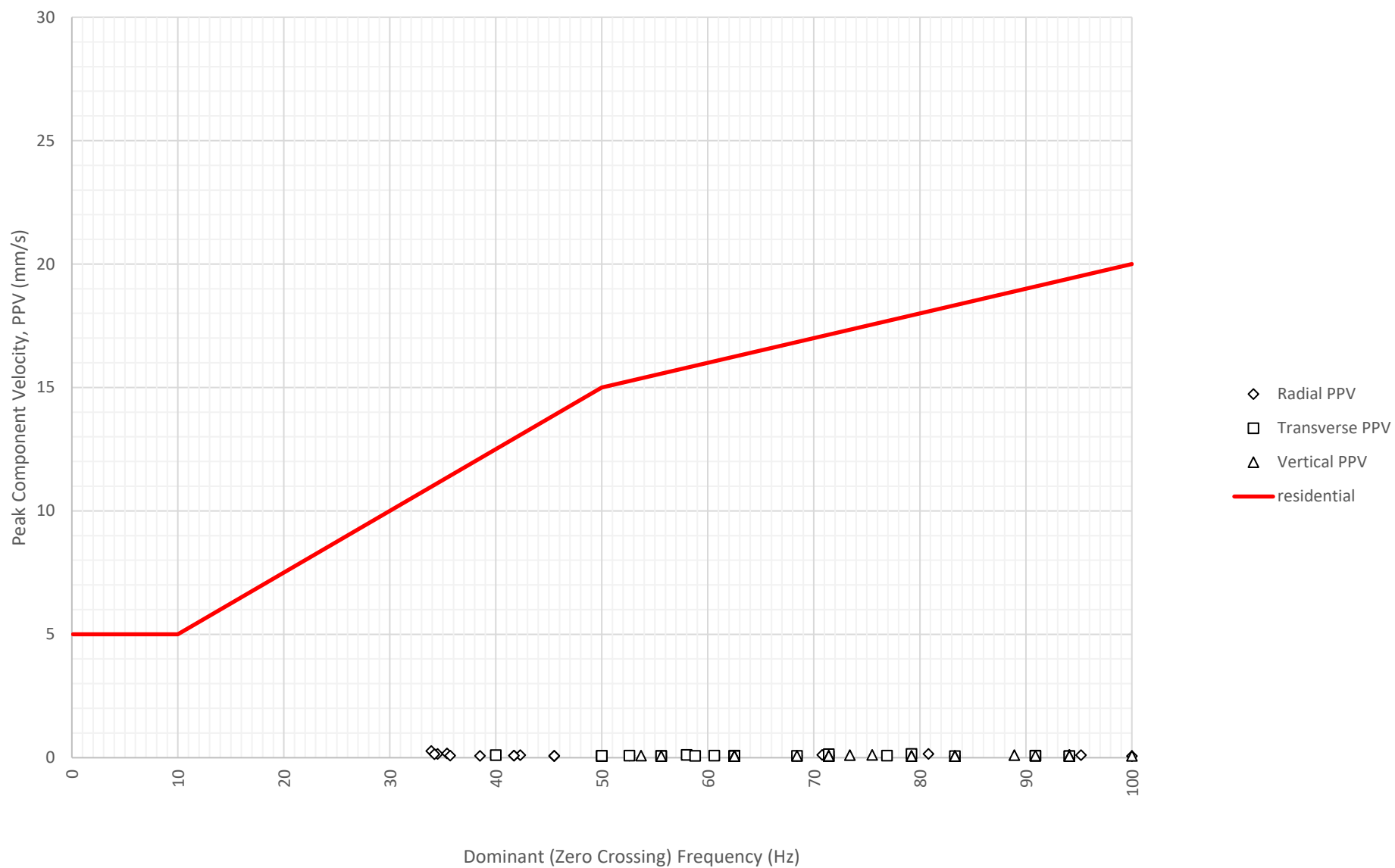
Frequency Content of Vibration Levels at North Boundary Near Block A and B (ETM7687) on 25-07-2024
