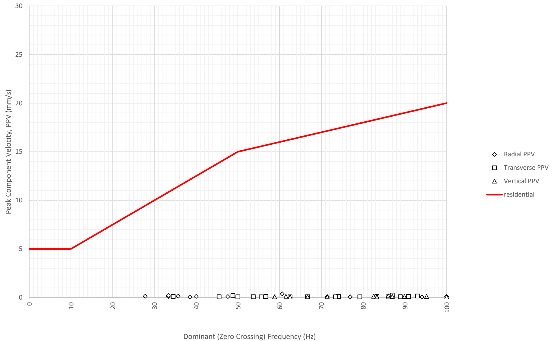
Frequency Content of Vibration Levels at North Boundary Near Block A and B (ETM7687) on 18-07-2024
