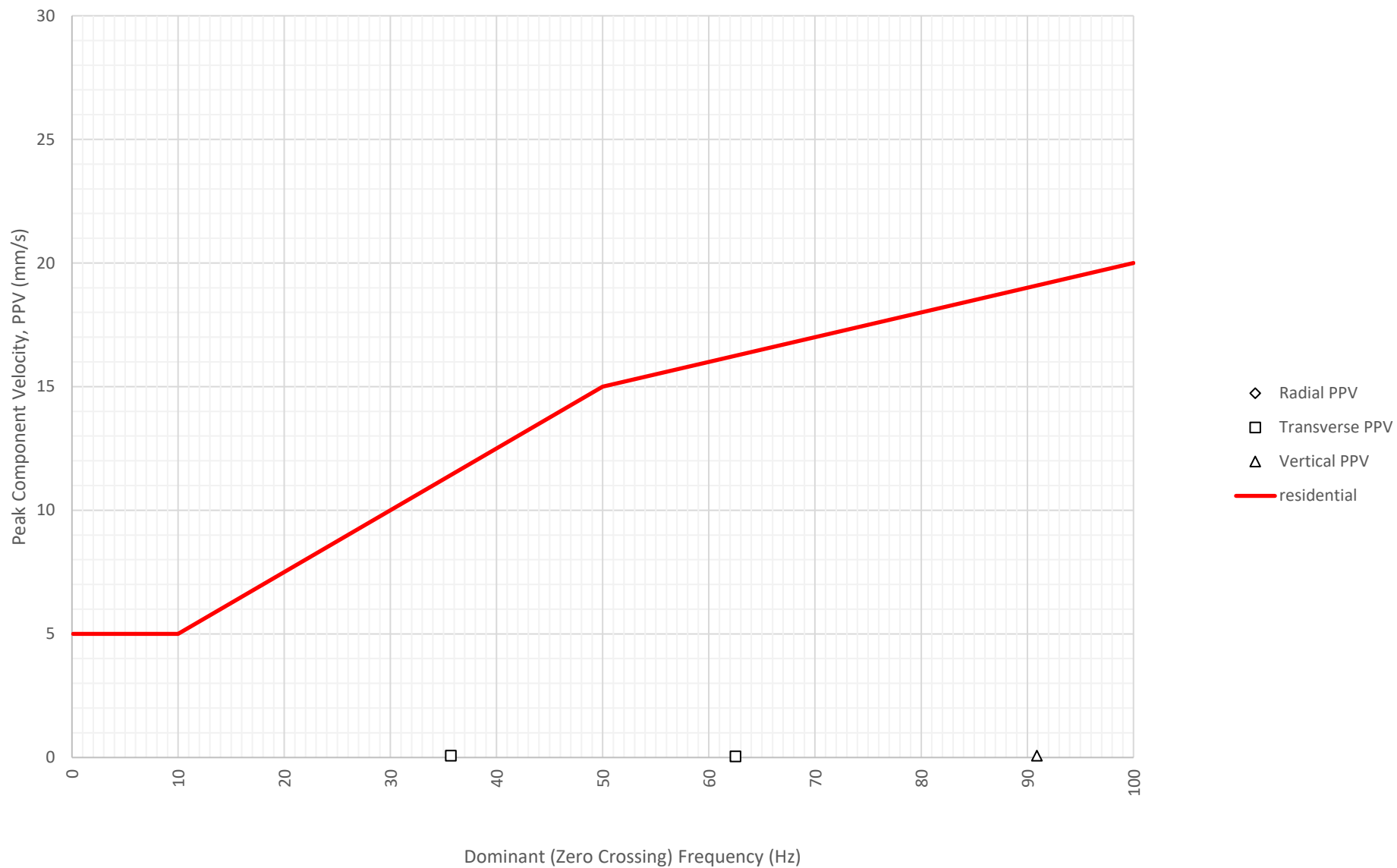
Frequency Content of Vibration Levels at East Boundary Opposite Shoalhaven Street (ETM7326) on 7-07-2024
