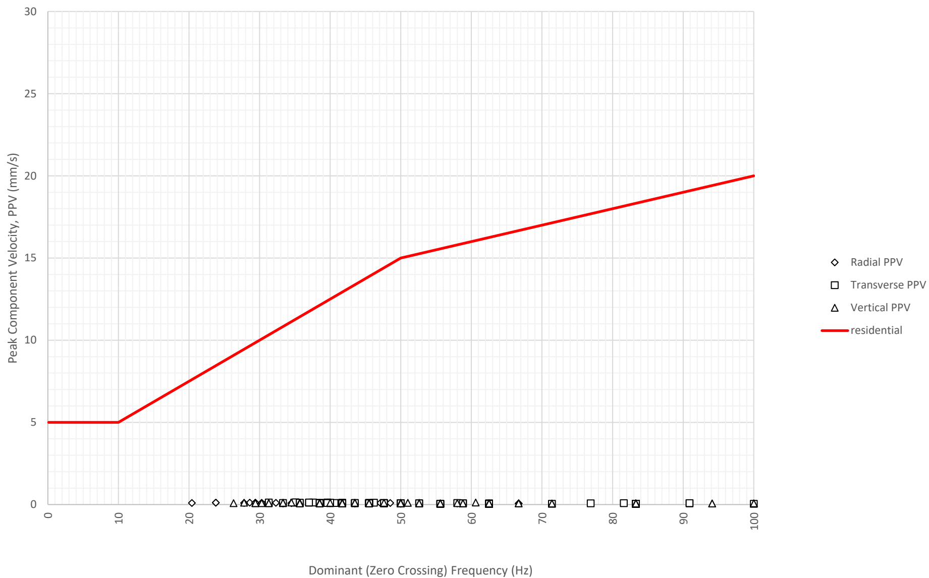
Frequency Content of Vibration Levels at East Boundary Opposite Shoalhaven Street (ETM7326) on 12-07-2024
