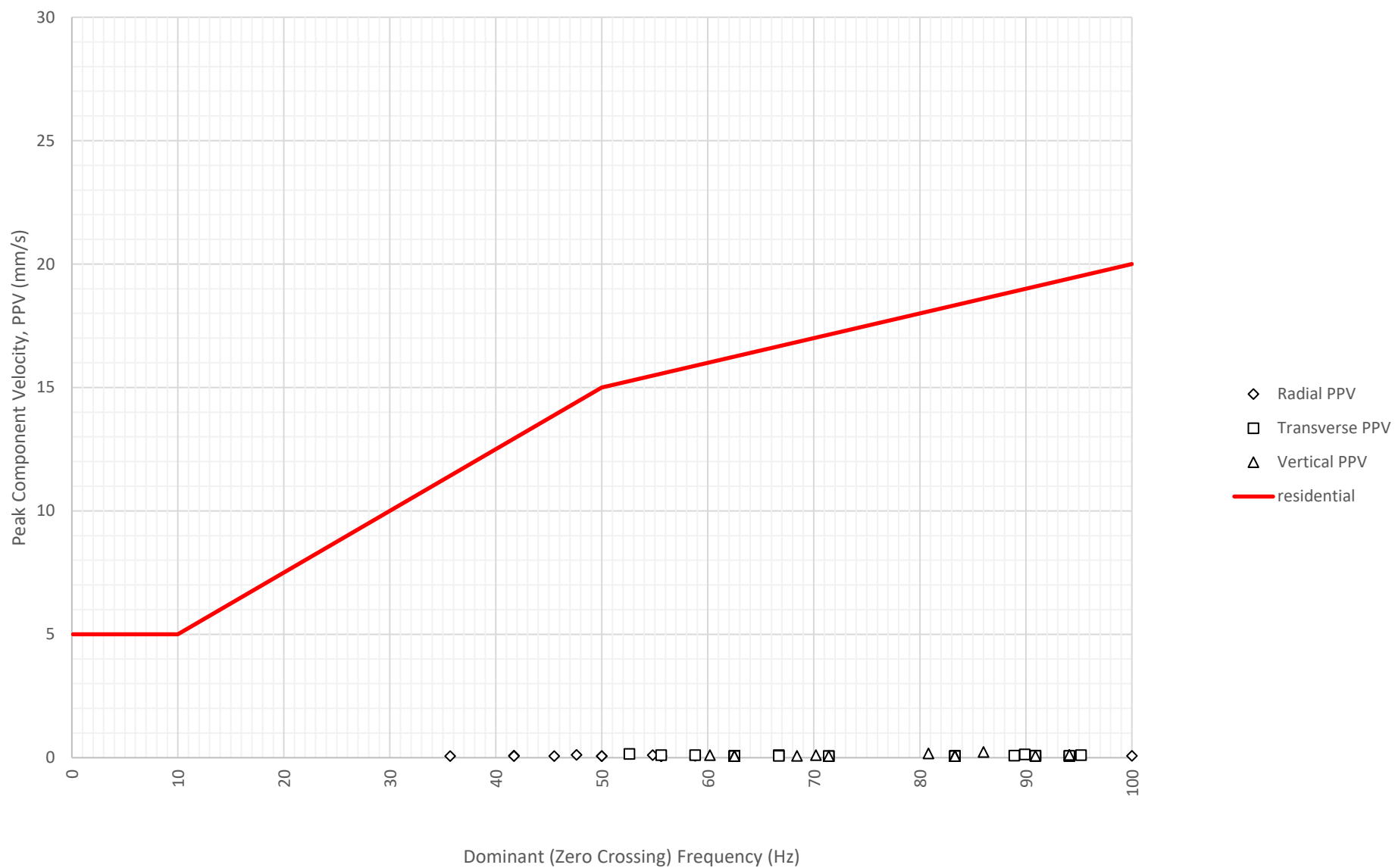
Frequency Content of Vibration Levels at North Boundary Near Block A and B (ETM7687) on 24-07-2024
