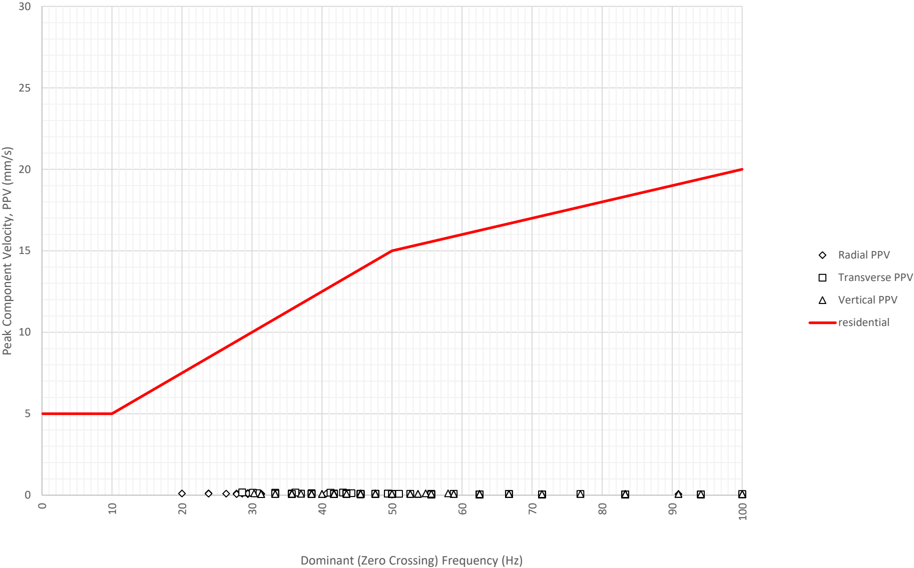
Frequency Content of Vibration Levels at East Boundary Opposite Shoalhaven Street (ETM7326) on 1-07-2024
