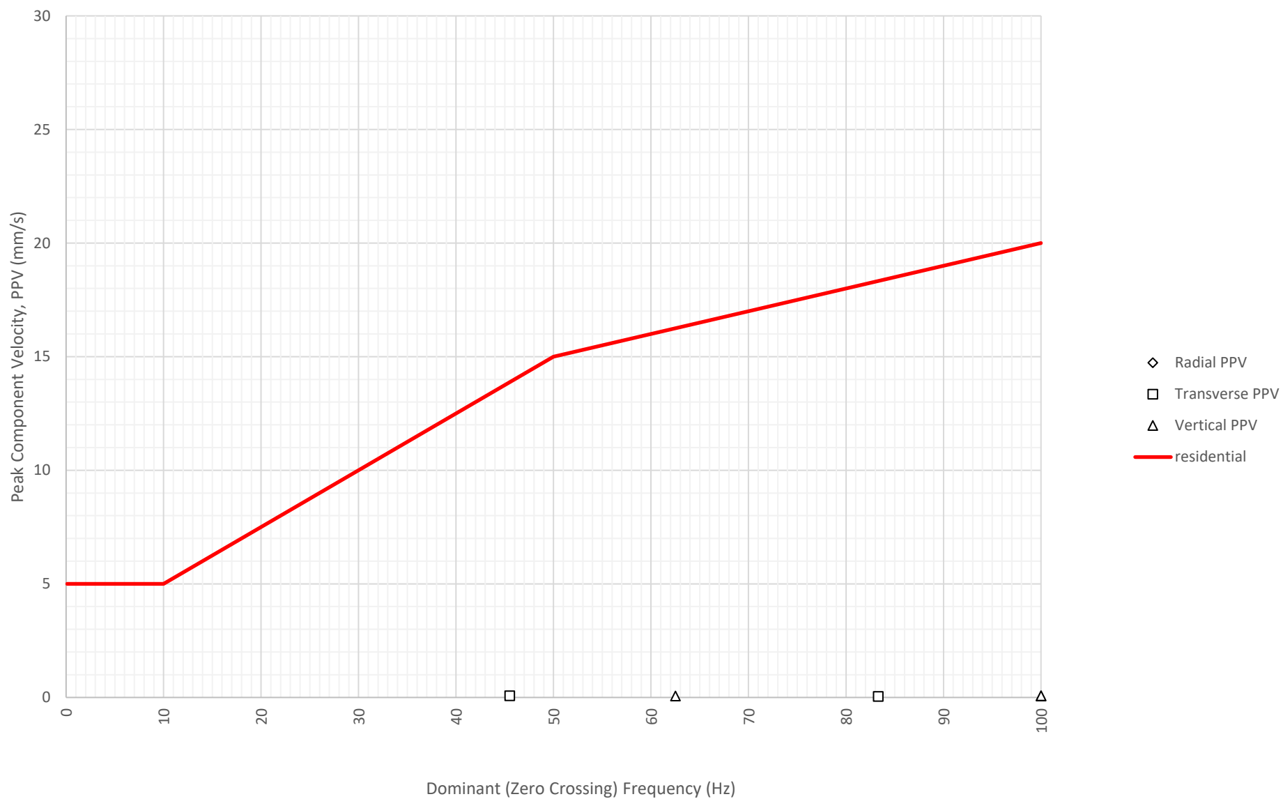
Frequency Content of Vibration Levels at East Boundary Opposite Shoalhaven Street (ETM7326) on 28-07-2024
