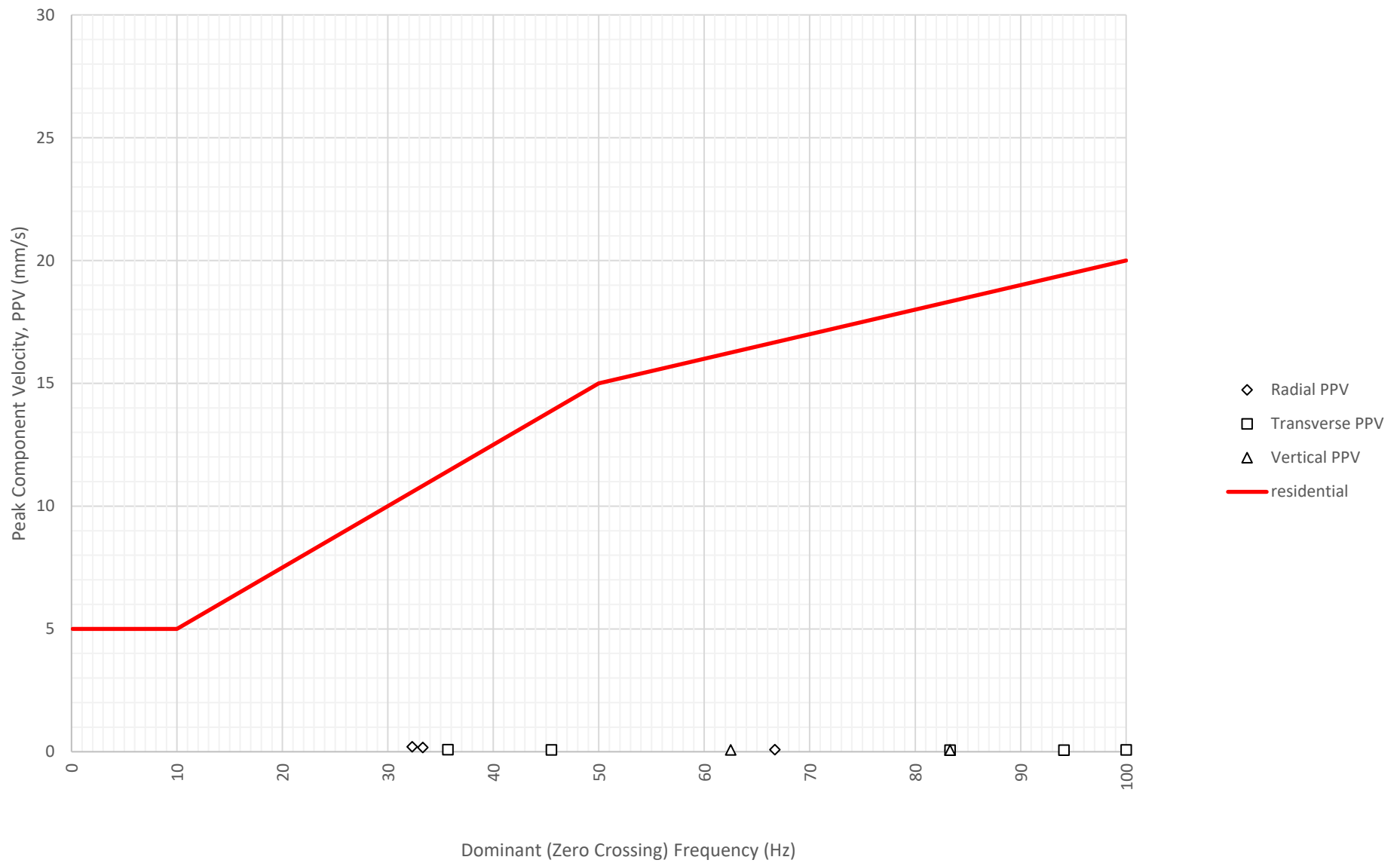
Frequency Content of Vibration Levels at North Boundary Near Block A and B (ETM7687) on 27-07-2024
