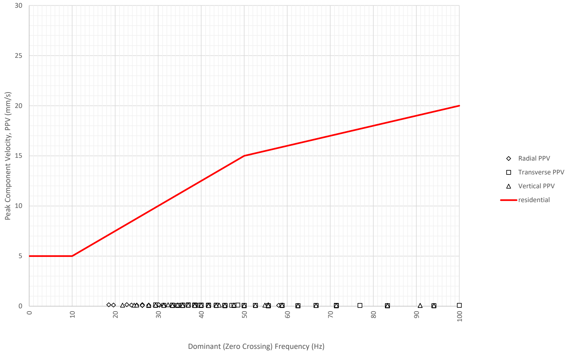
Frequency Content of Vibration Levels at East Boundary Opposite Shoalhaven Street (ETM7326) on 9-07-2024
