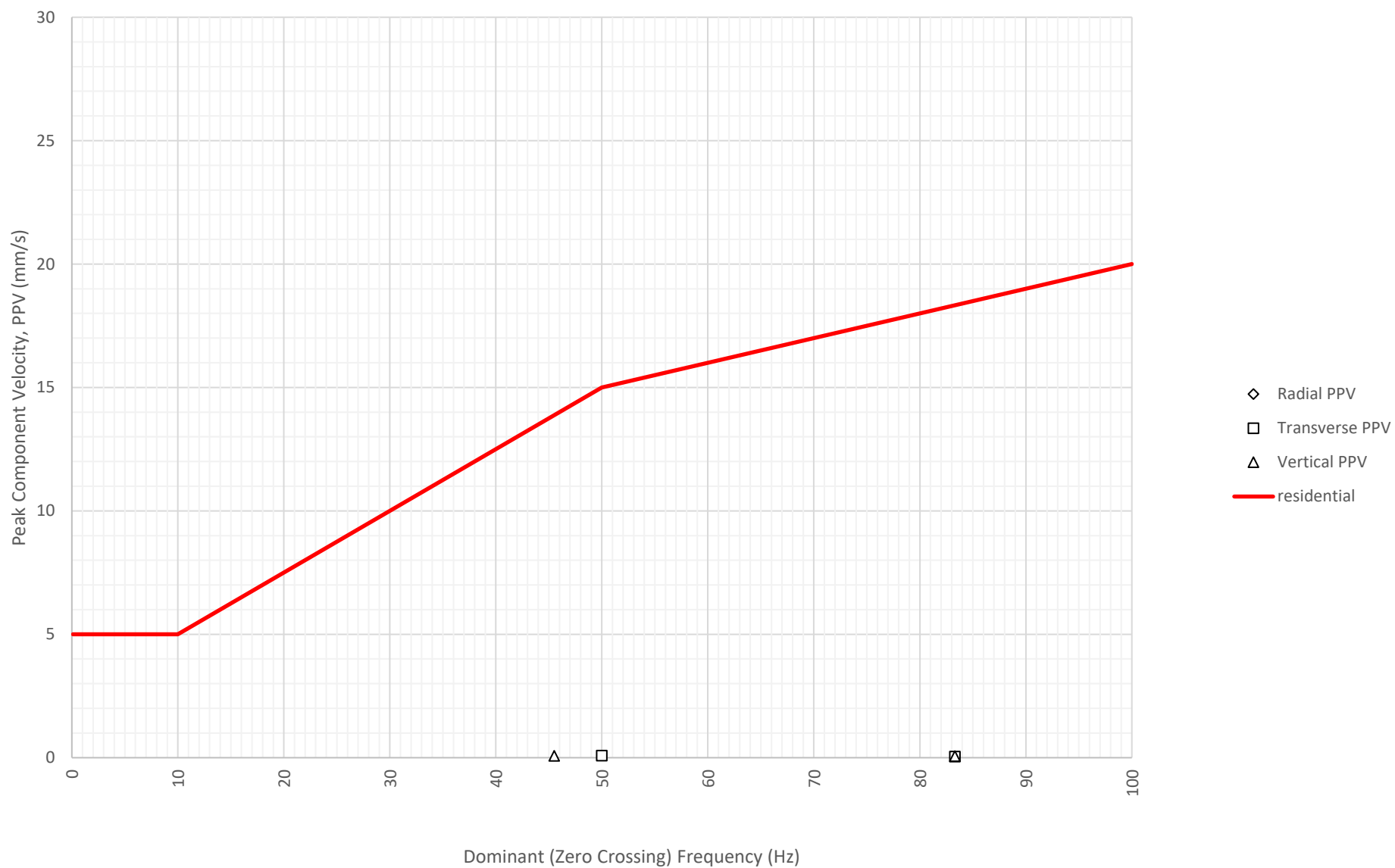
Frequency Content of Vibration Levels at East Boundary Opposite Shoalhaven Street (ETM7326) on 21-07-2024
