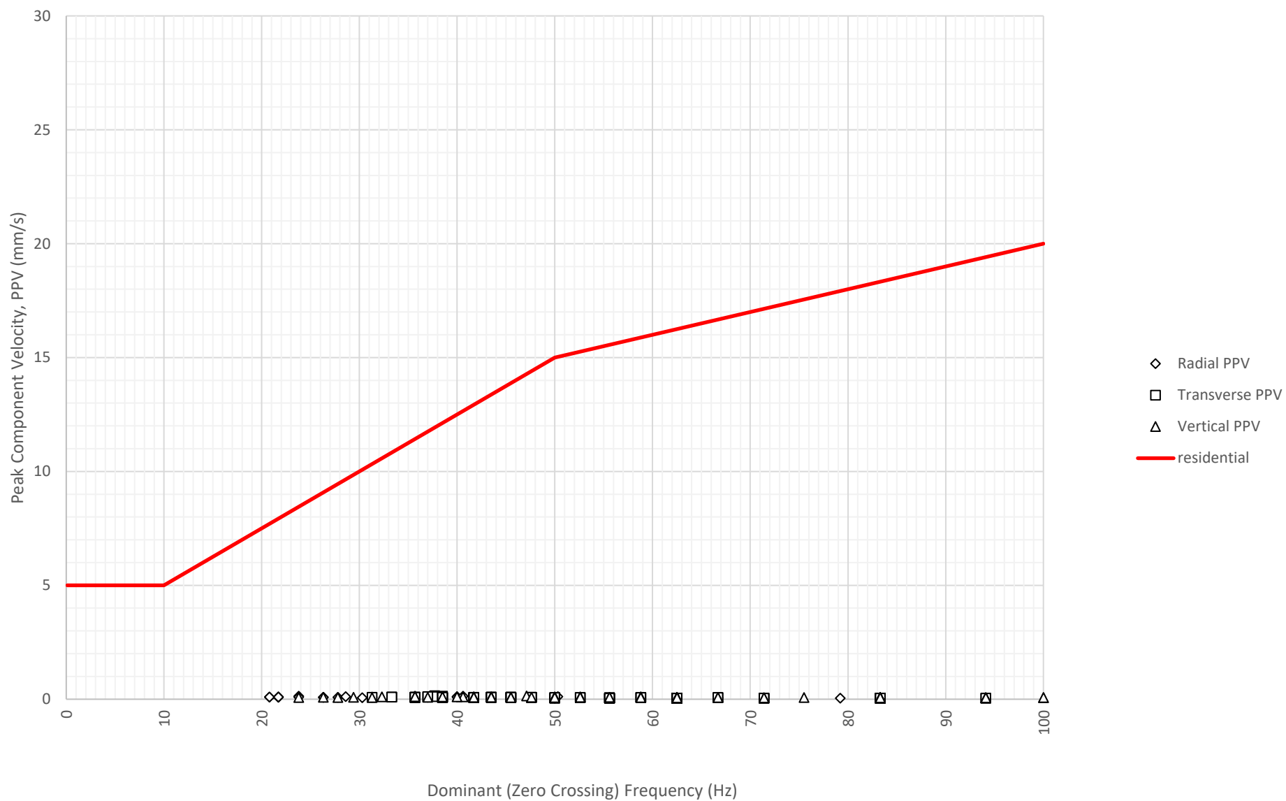
Frequency Content of Vibration Levels at East Boundary Opposite Shoalhaven Street (ETM7326) on 10-07-2024
