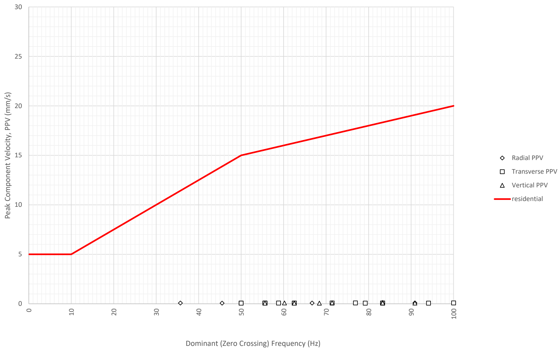
Frequency Content of Vibration Levels at North Boundary Near Block A and B (ETM7687) on 22-07-2024
