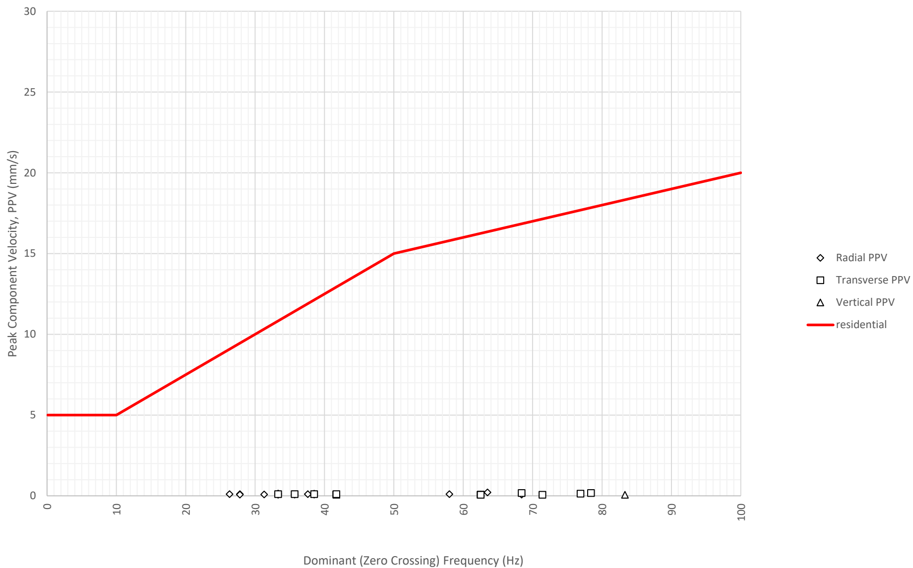
Frequency Content of Vibration Levels at North Boundary Near Block A and B (ETM7687) on 20-07-2024
