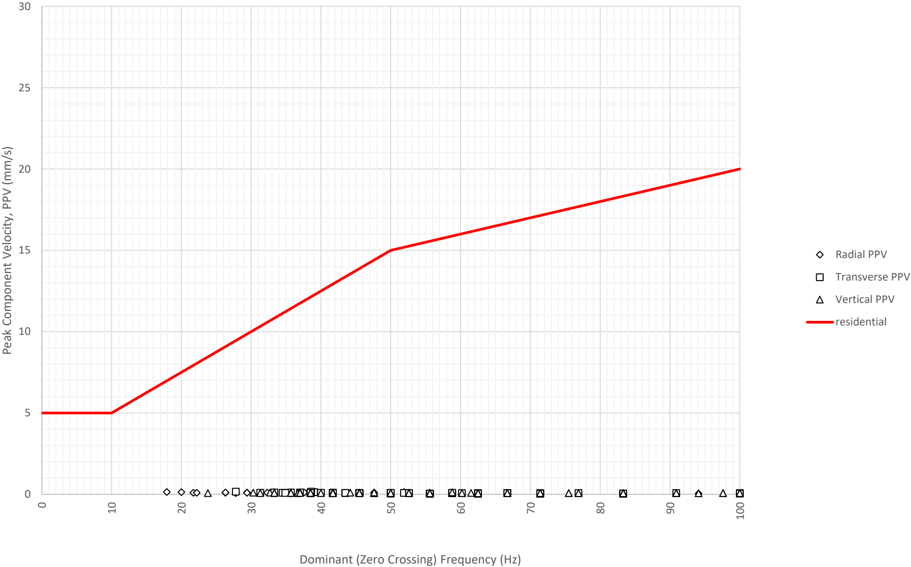
Frequency Content of Vibration Levels at East Boundary Opposite Shoalhaven Street (ETM7326) on 4-07-2024
