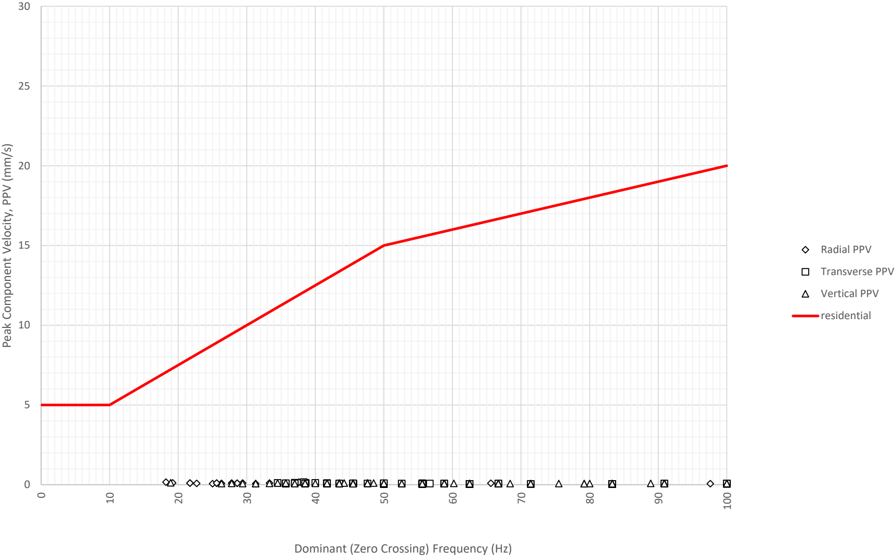
Frequency Content of Vibration Levels at East Boundary Opposite Shoalhaven Street (ETM7326) on 5-07-2024
