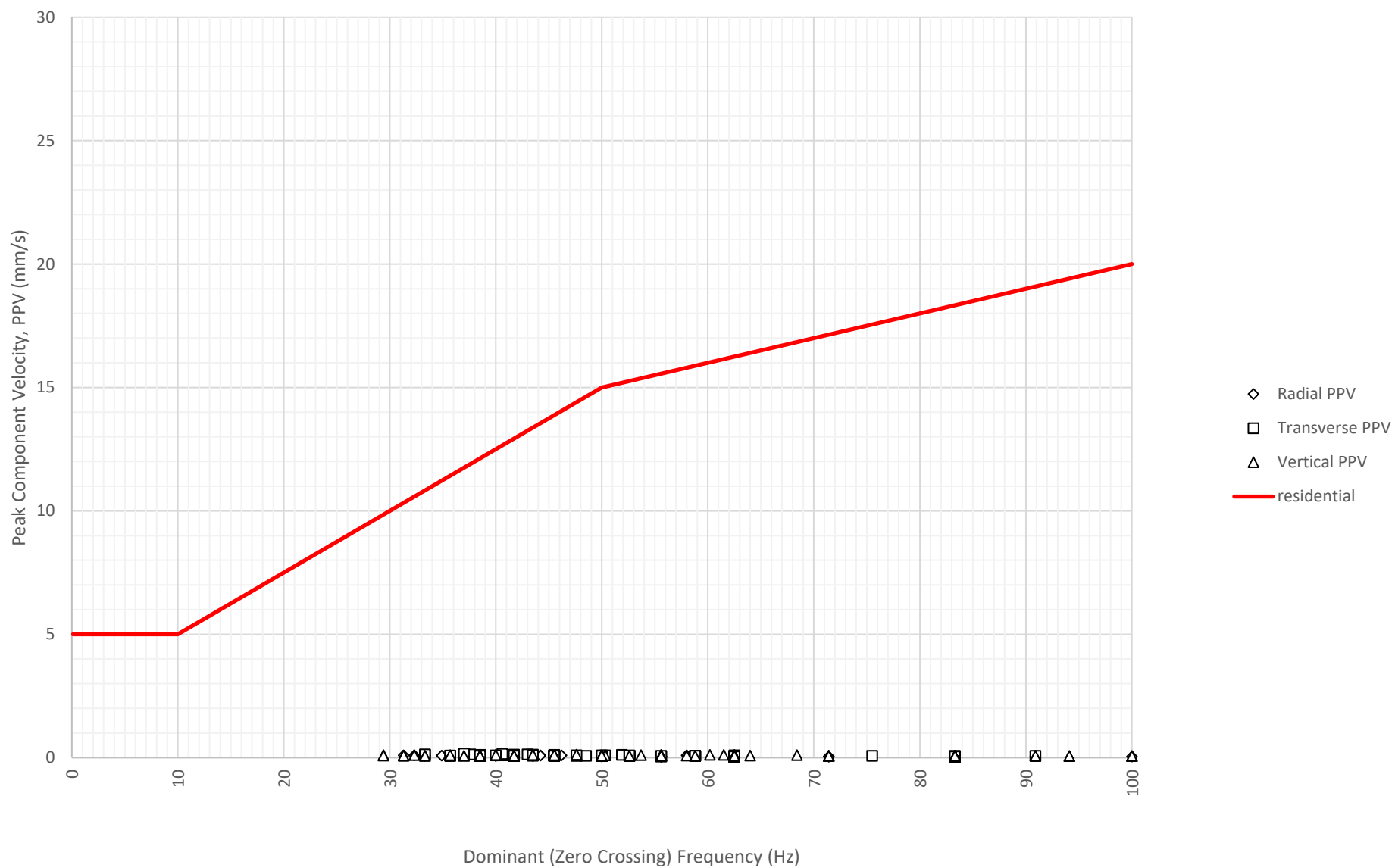
Frequency Content of Vibration Levels at East Boundary Opposite Shoalhaven Street (ETM7326) on 24-07-2024
