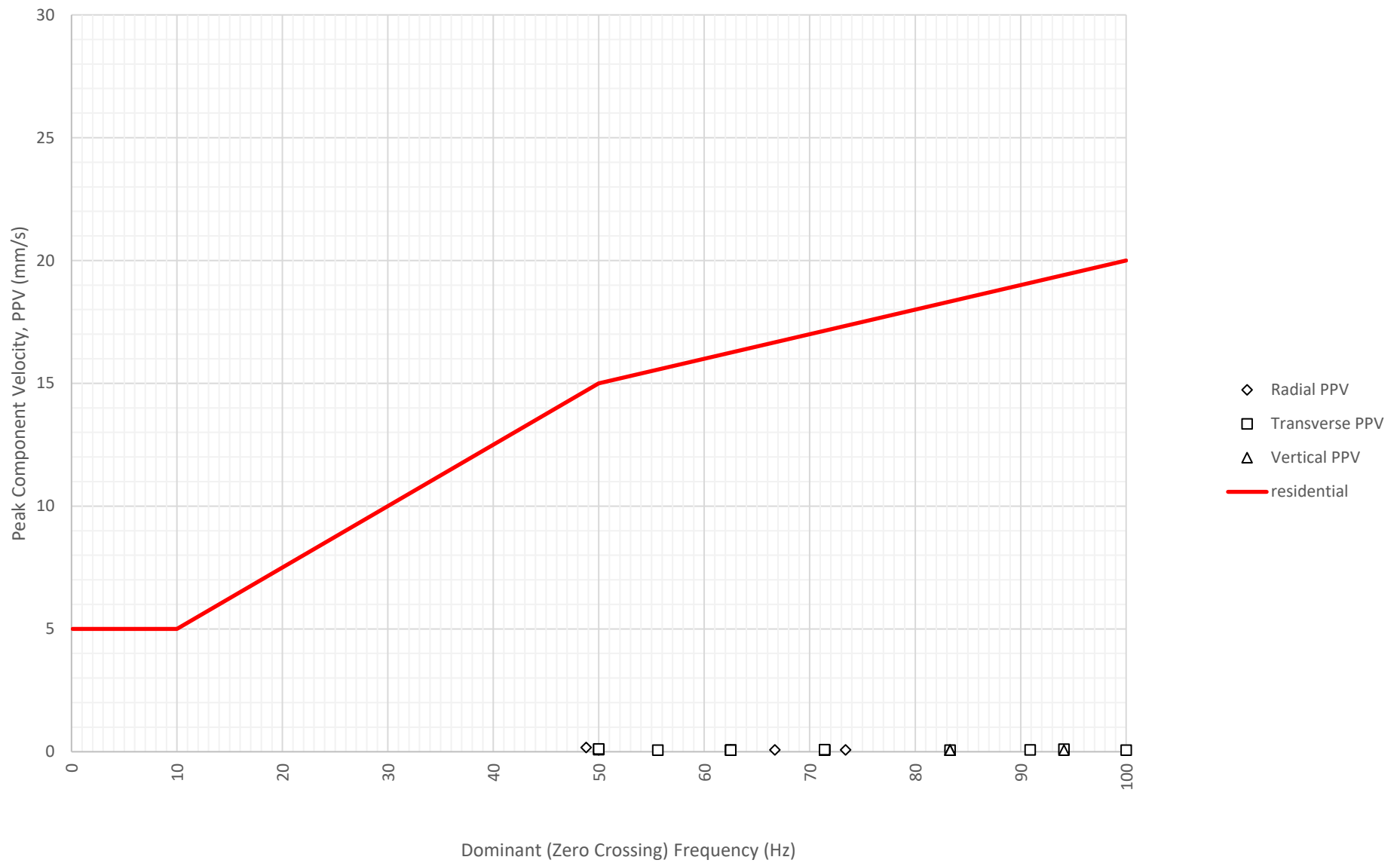
Frequency Content of Vibration Levels at North Boundary Near Block A and B (ETM7687) on 9-07-2024
