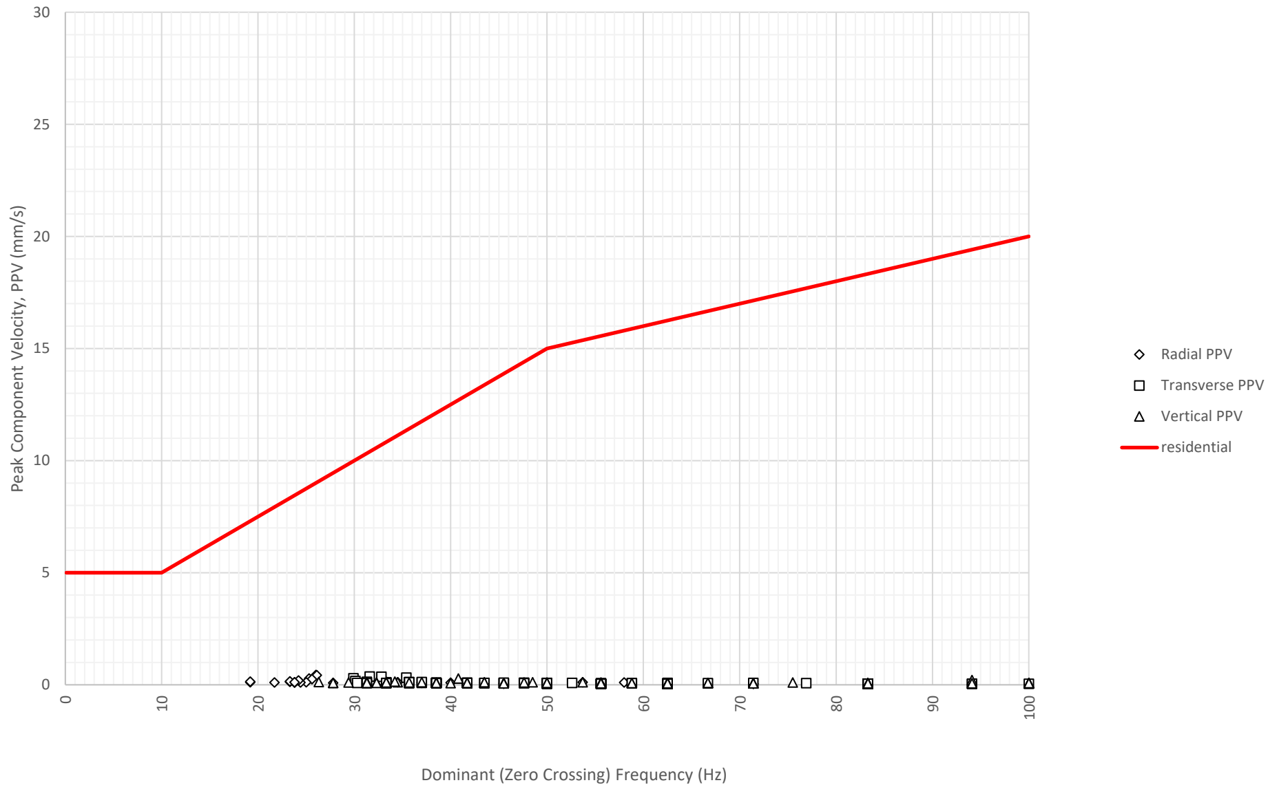
Frequency Content of Vibration Levels at East Boundary Opposite Shoalhaven Street (ETM7326) on 8-07-2024
