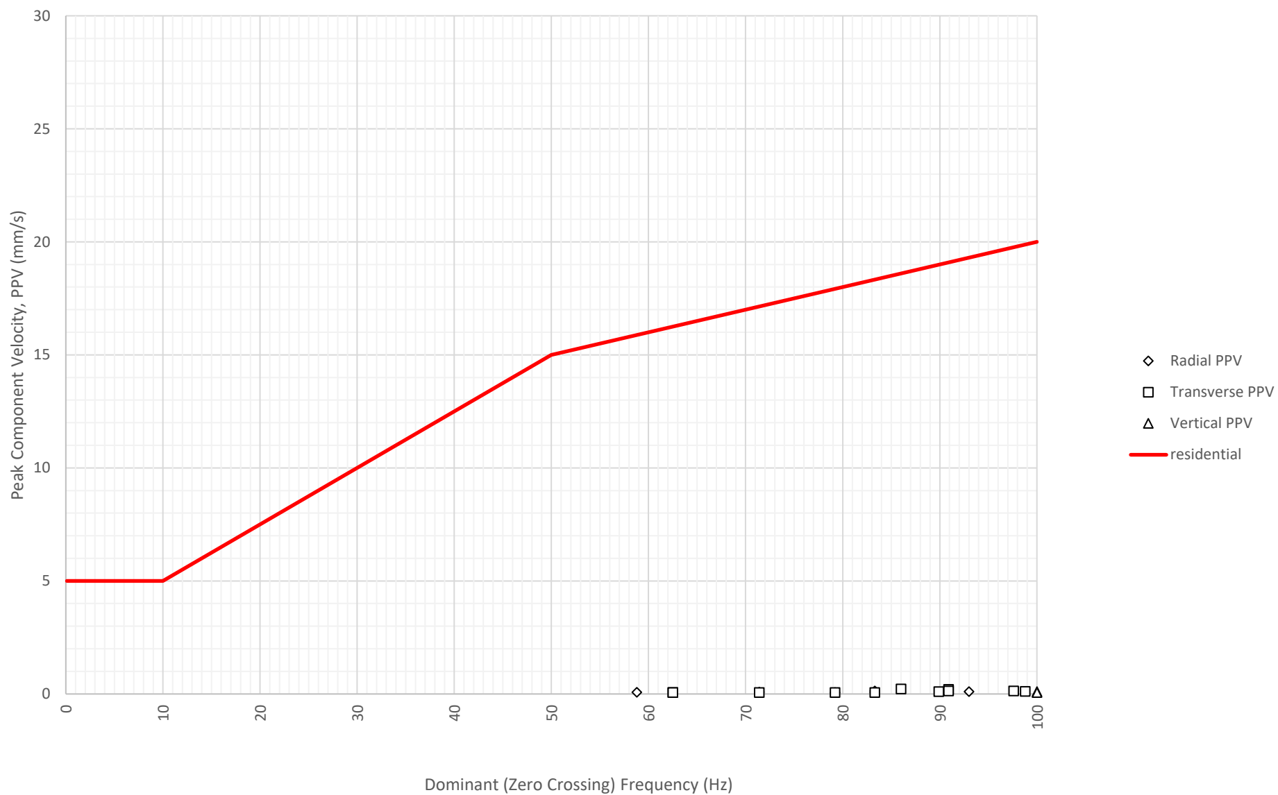
Frequency Content of Vibration Levels at North Boundary Near Block A and B (ETM7687) on 10-07-2024
