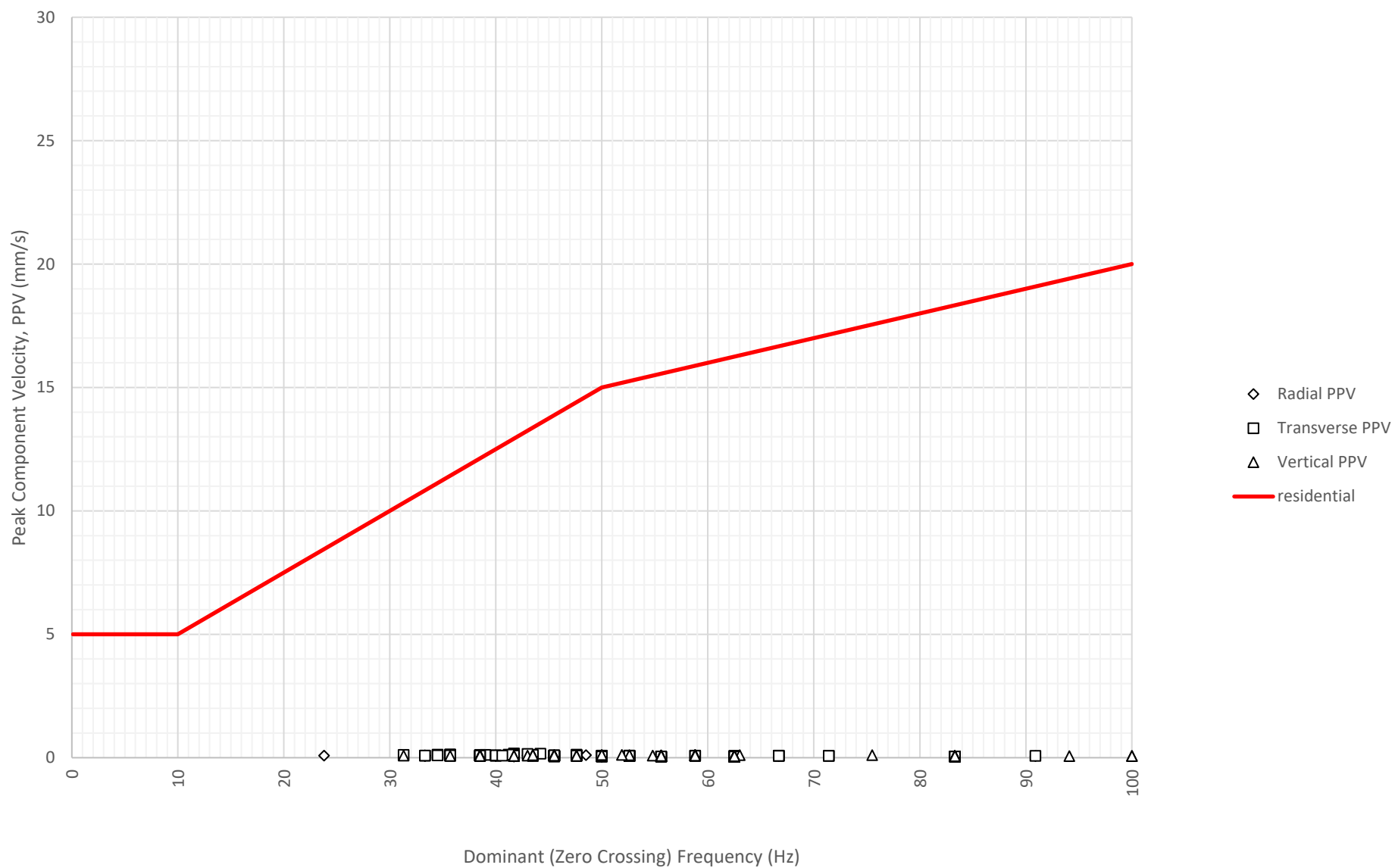
Frequency Content of Vibration Levels at East Boundary Opposite Shoalhaven Street (ETM7326) on 26-07-2024
