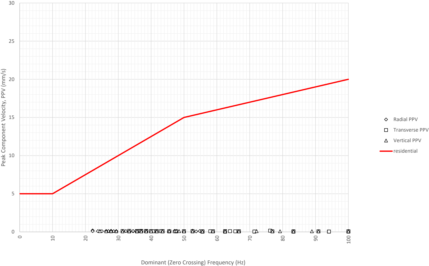
Frequency Content of Vibration Levels at East Boundary Opposite Shoalhaven Street (ETM7326) on 3-07-2024
