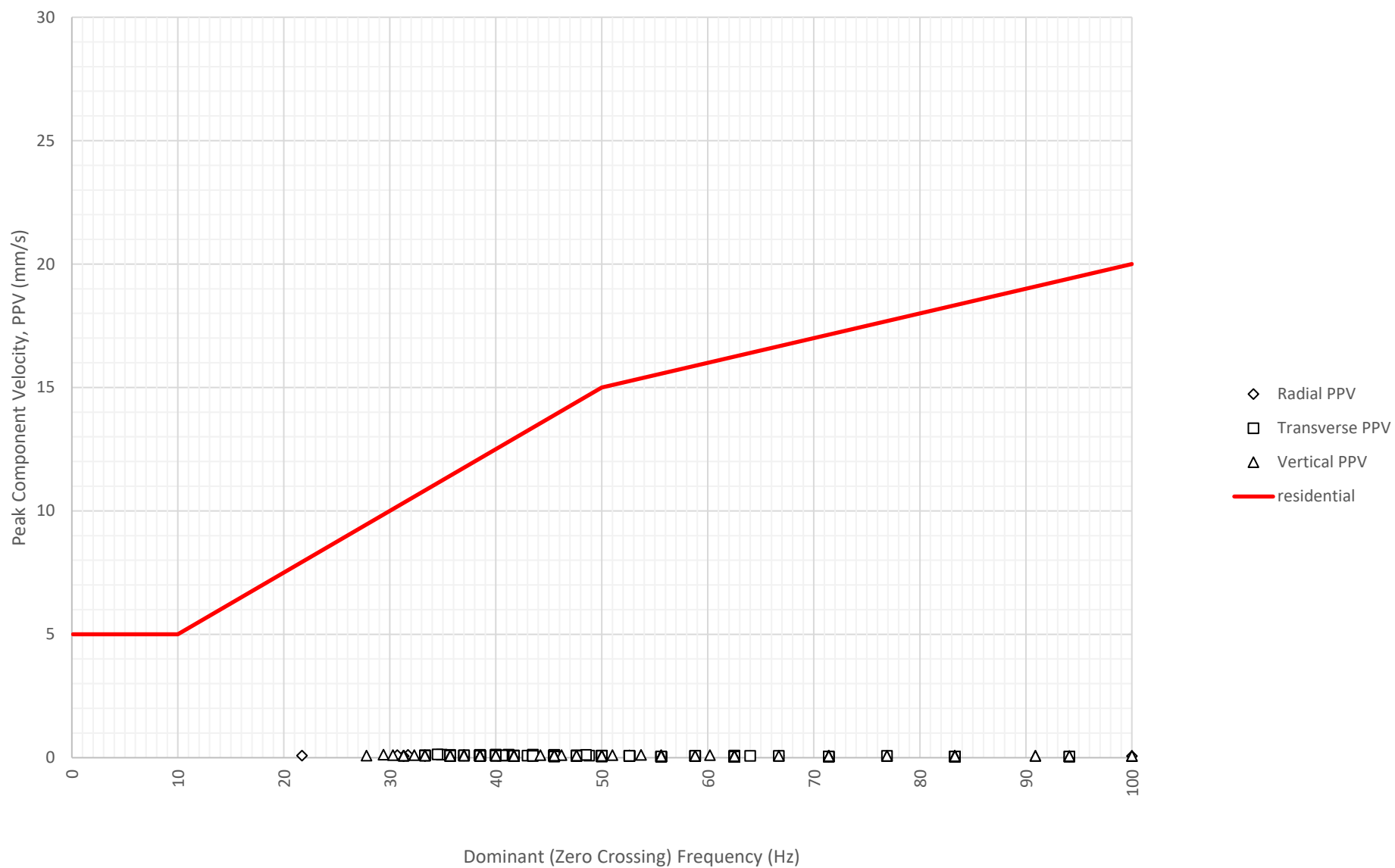
Frequency Content of Vibration Levels at East Boundary Opposite Shoalhaven Street (ETM7326) on 23-07-2024
