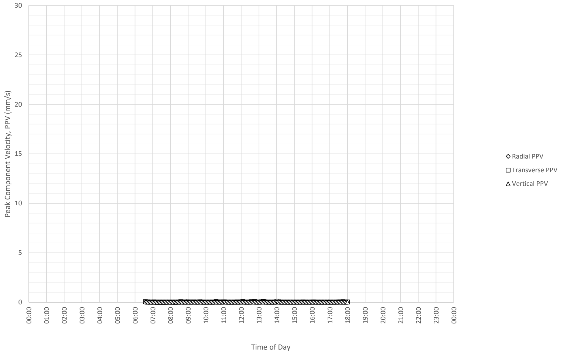
Daily Monitored Vibration Levels at North Boundary Near Block A and B (ETM7687) on 5-07-2024
