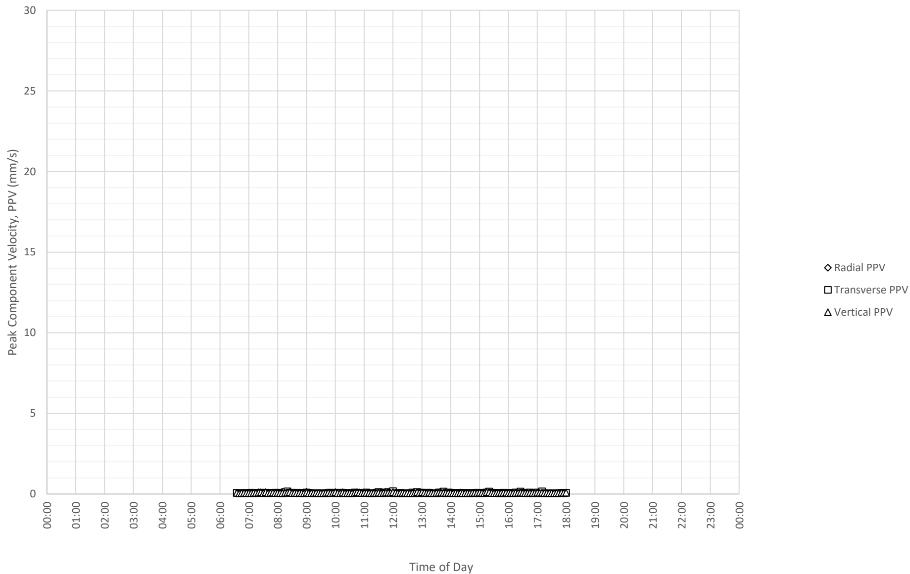
Daily Monitored Vibration Levels at East Boundary Opposite Shoalhaven Street (ETM7326) on 1-07-2024
