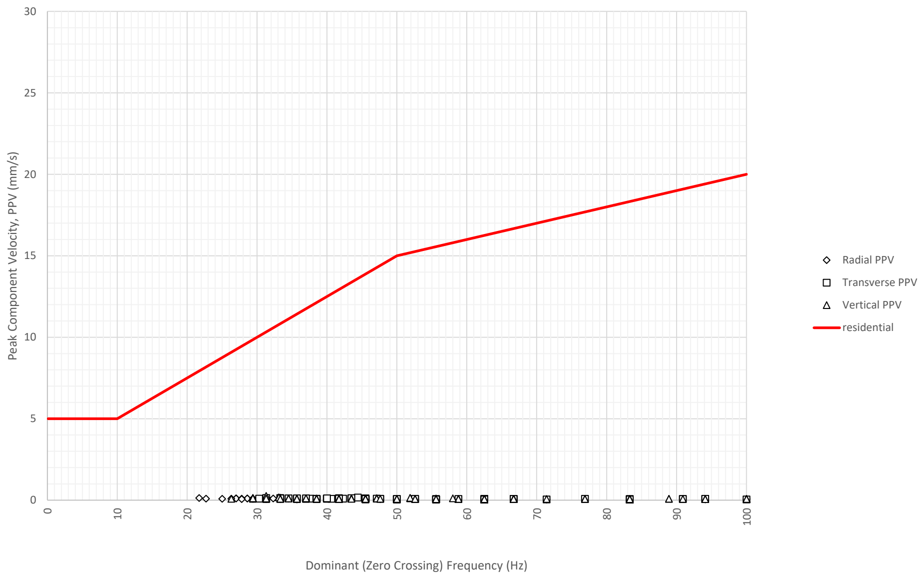
Frequency Content of Vibration Levels at East Boundary Opposite Shoalhaven Street (ETM7326) on 21-06-2024
