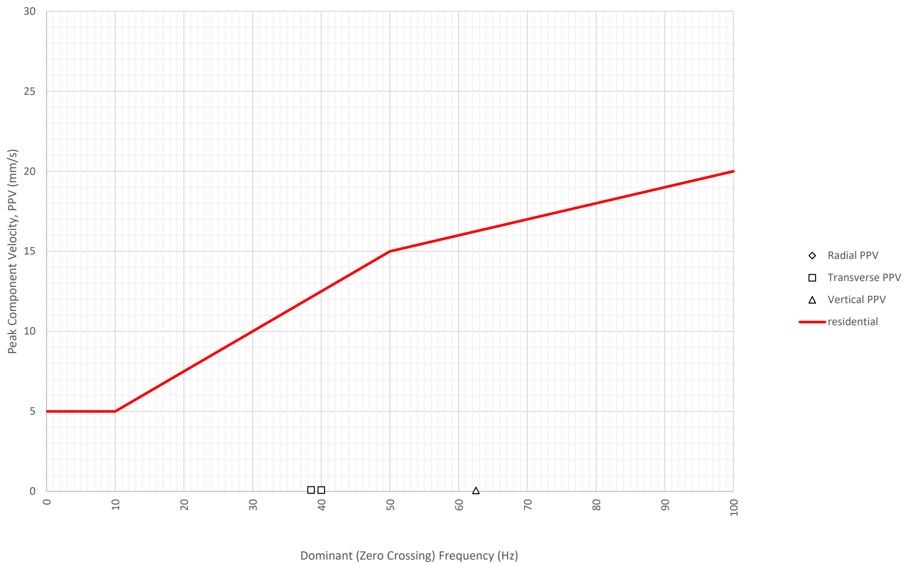
Frequency Content of Vibration Levels at East Boundary Opposite Shoalhaven Street (ETM7326) on 23-06-2024
