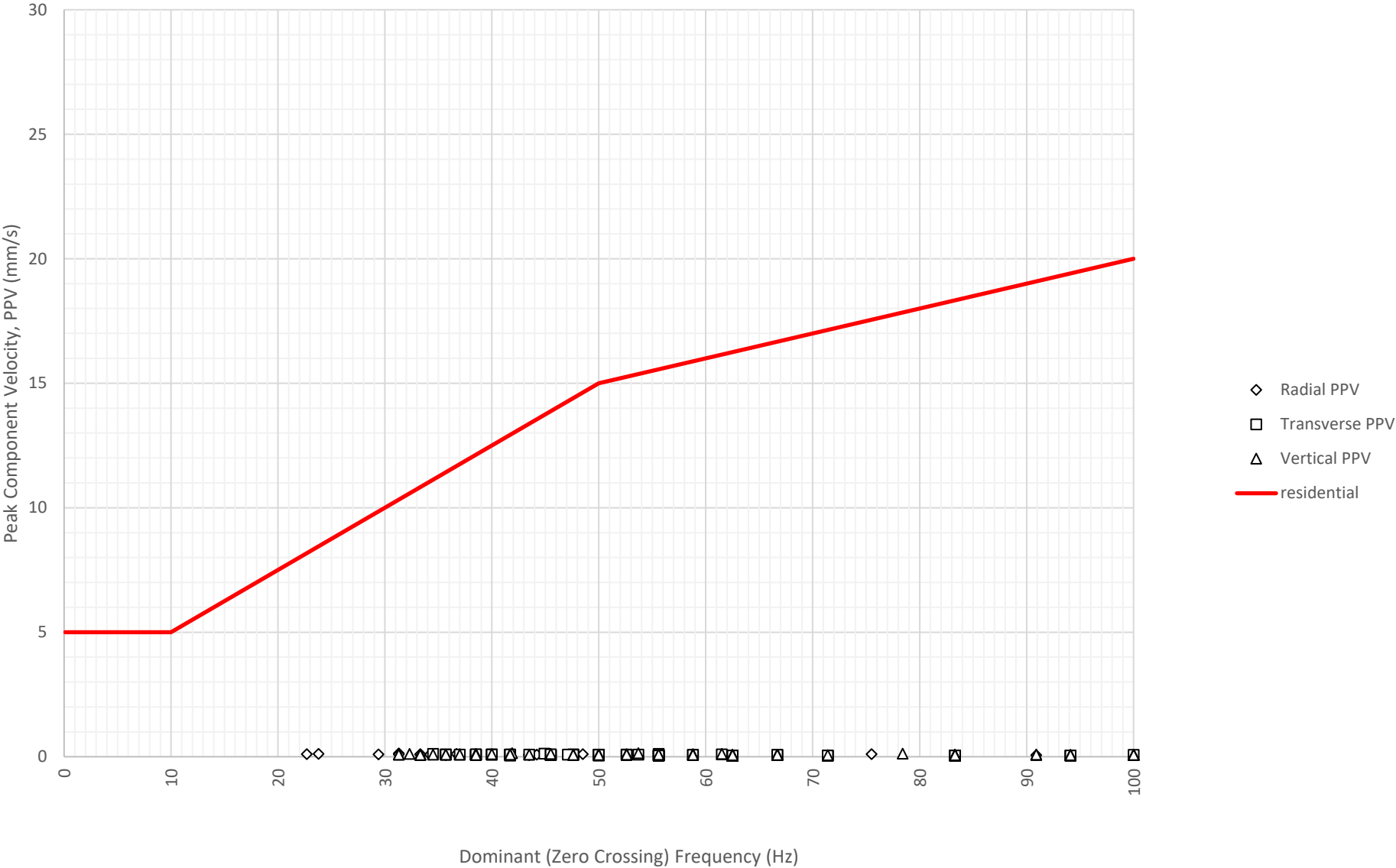
Frequency Content of Vibration Levels at East Boundary Opposite Shoalhaven Street (ETM7326) on 3-06-2024
