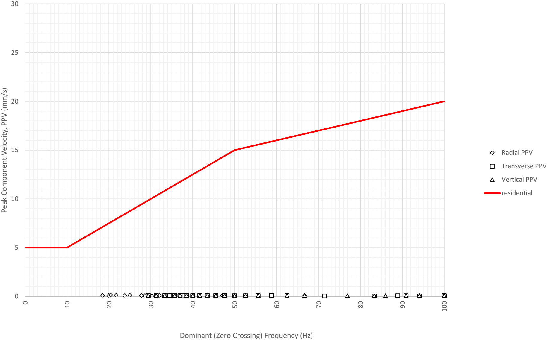
Frequency Content of Vibration Levels at East Boundary Opposite Shoalhaven Street (ETM7326) on 7-06-2024
