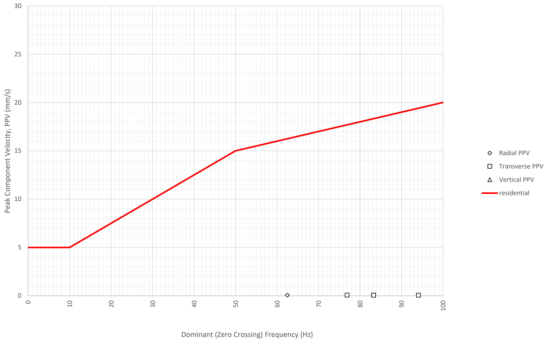
Frequency Content of Vibration Levels at North Boundary Near Block A and B (ETM7687) on 28-06-2024
