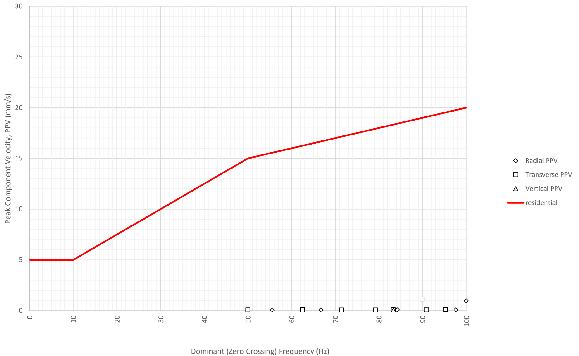
Frequency Content of Vibration Levels at North Boundary Near Block A and B (ETM7687) on 12-06-2024
