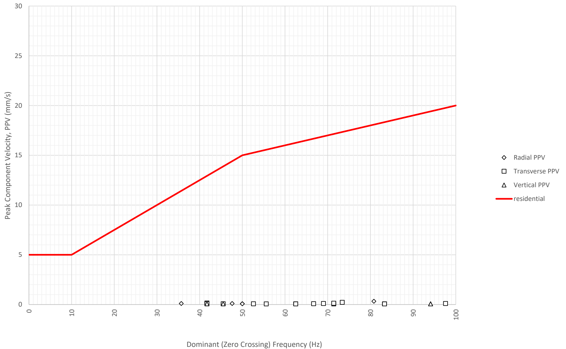
Frequency Content of Vibration Levels at North Boundary Near Block A and B (ETM7687) on 19-06-2024
