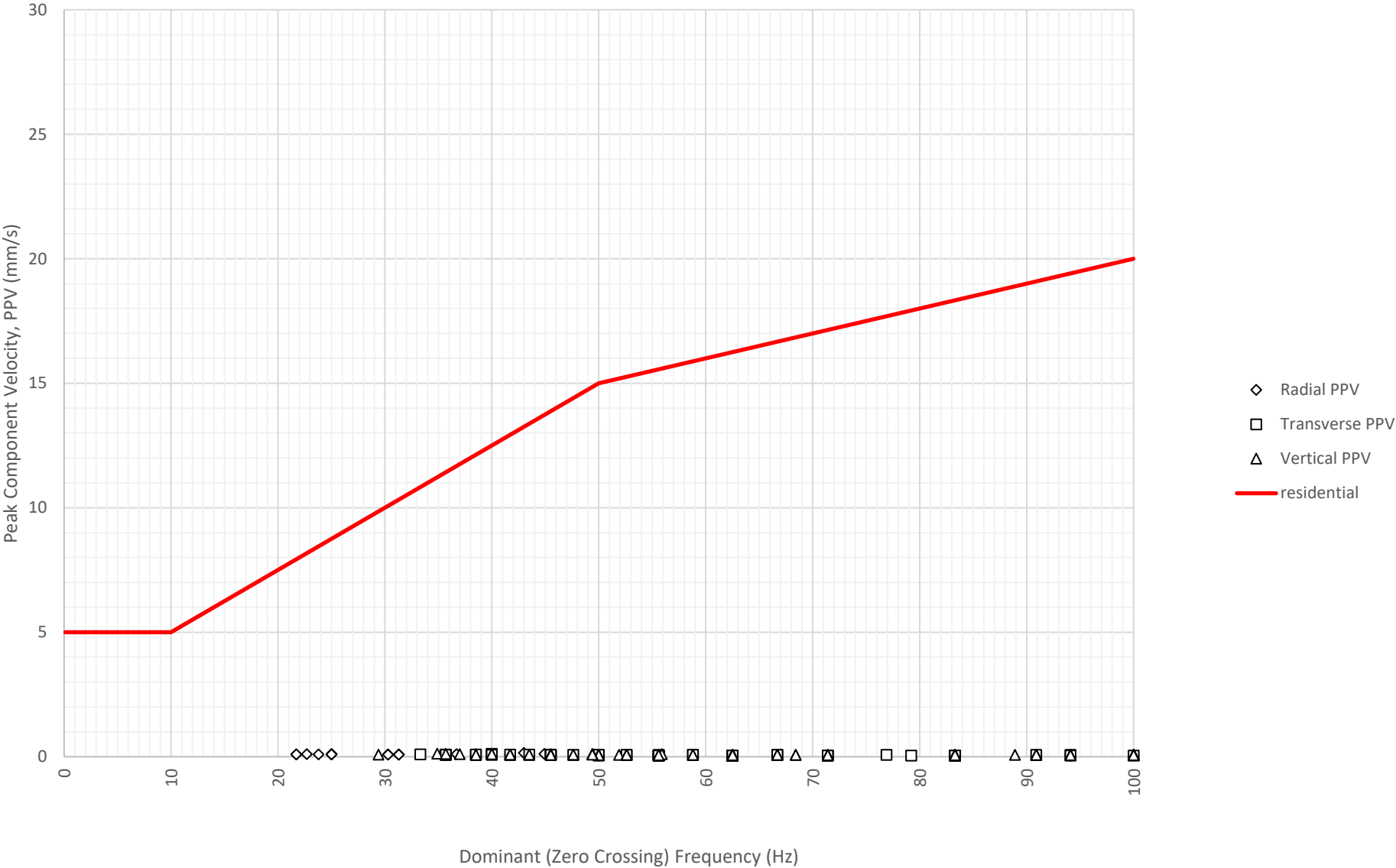
Frequency Content of Vibration Levels at East Boundary Opposite Shoalhaven Street (ETM7326) on 8-06-2024
