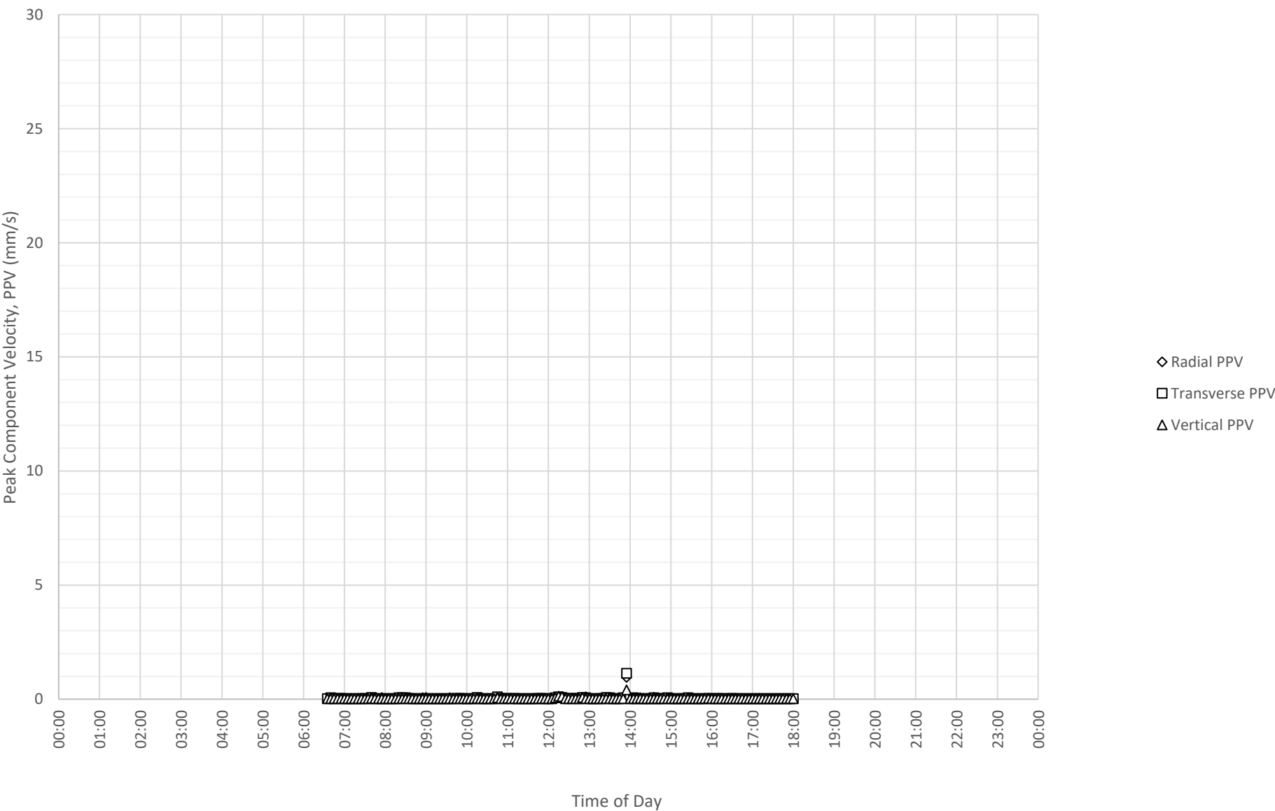
Daily Monitored Vibration Levels at North Boundary Near Block A and B (ETM7687) on 12-06-2024
