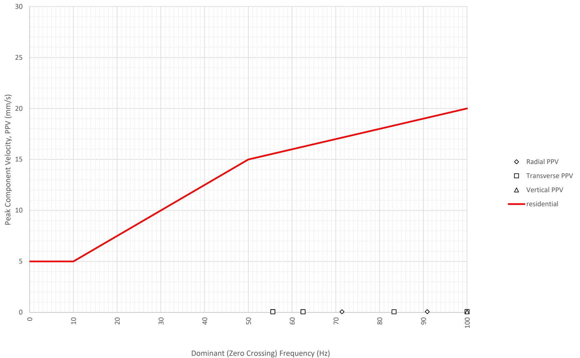
Frequency Content of Vibration Levels at North Boundary Near Block A and B (ETM7687) on 27-06-2024
