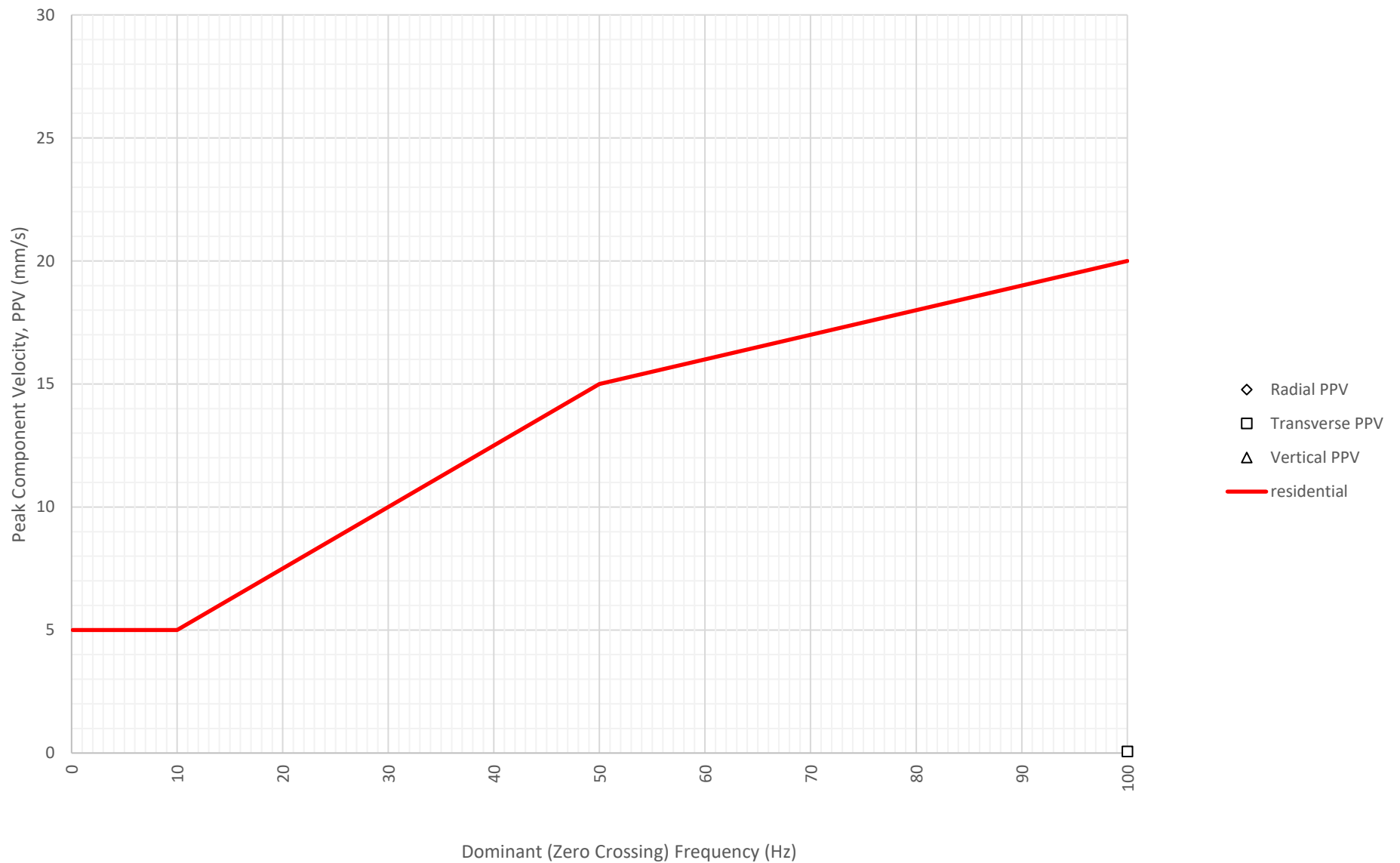
Frequency Content of Vibration Levels at North Boundary Near Block A and B (ETM7687) on 29-06-2024
