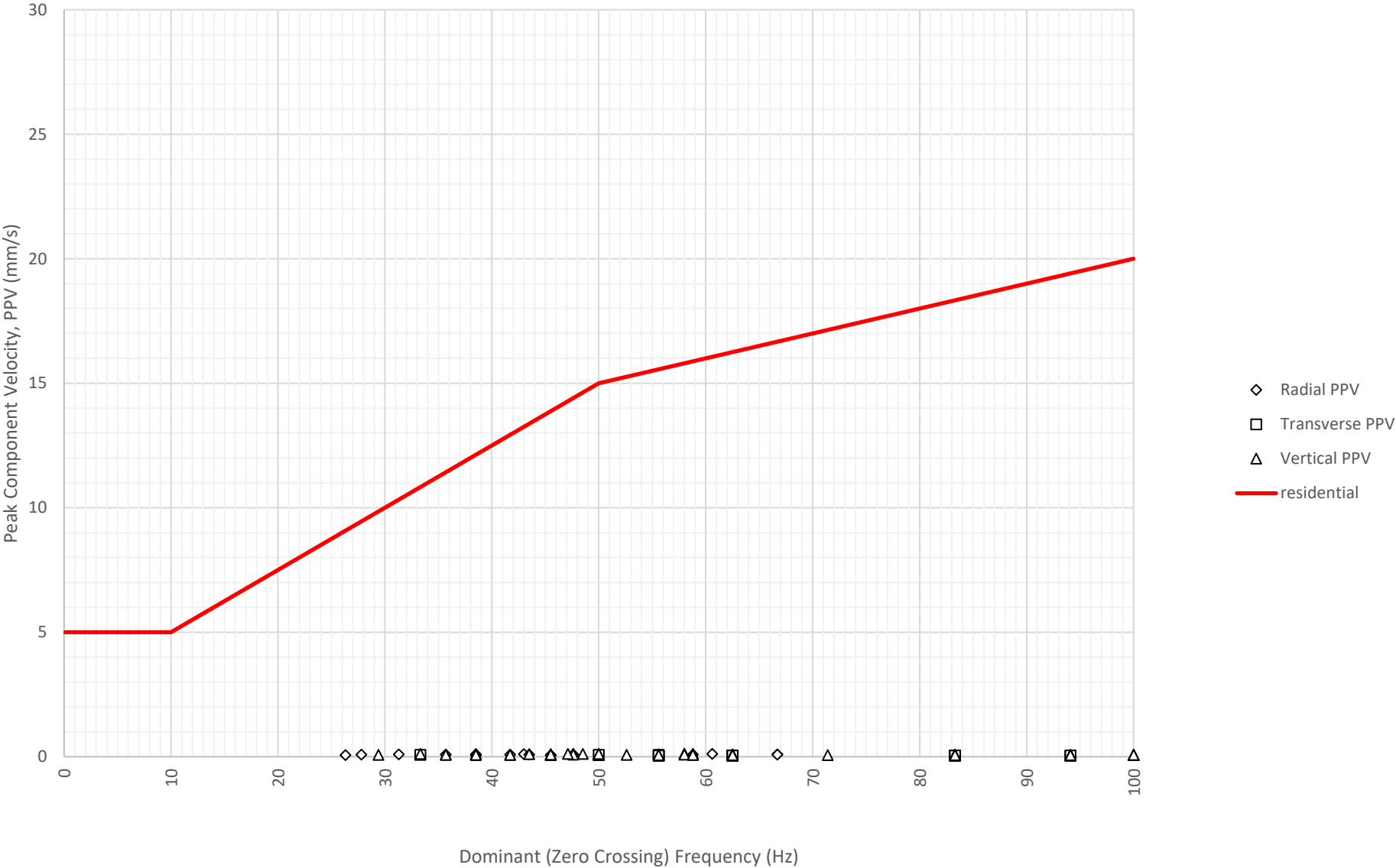
Frequency Content of Vibration Levels at East Boundary Opposite Shoalhaven Street (ETM7326) on 1-06-2024
