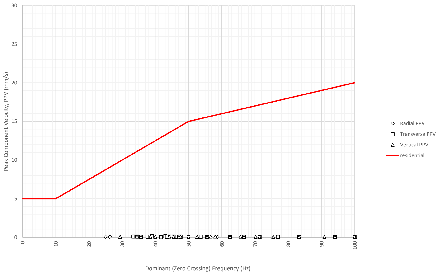
Frequency Content of Vibration Levels at East Boundary Opposite Shoalhaven Street (ETM7326) on 29-06-2024
