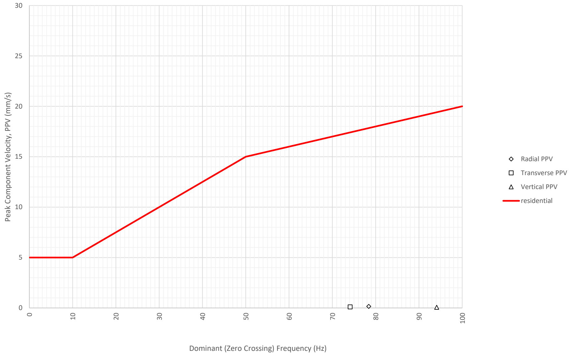
Frequency Content of Vibration Levels at North Boundary Near Block A and B (ETM7687) on 1-06-2024
