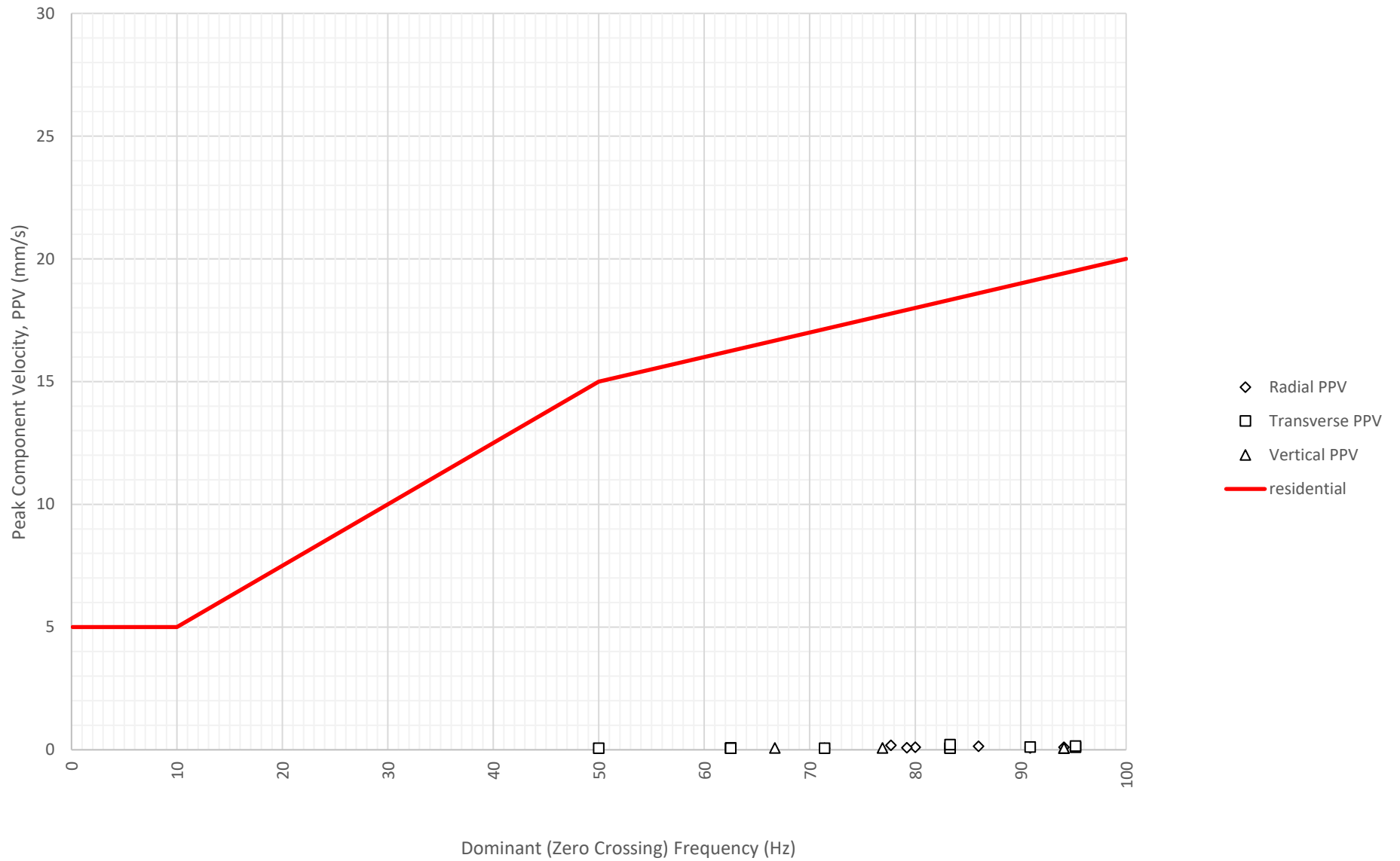
Frequency Content of Vibration Levels at North Boundary Near Block A and B (ETM7687) on 5-06-2024
