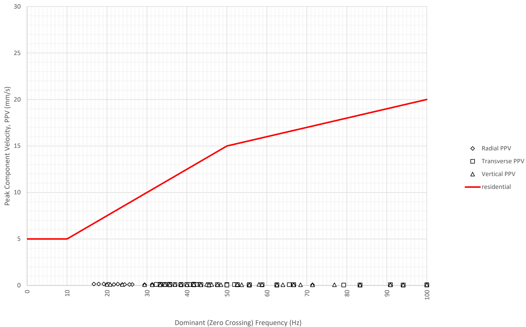
Frequency Content of Vibration Levels at East Boundary Opposite Shoalhaven Street (ETM7326) on 11-06-2024
