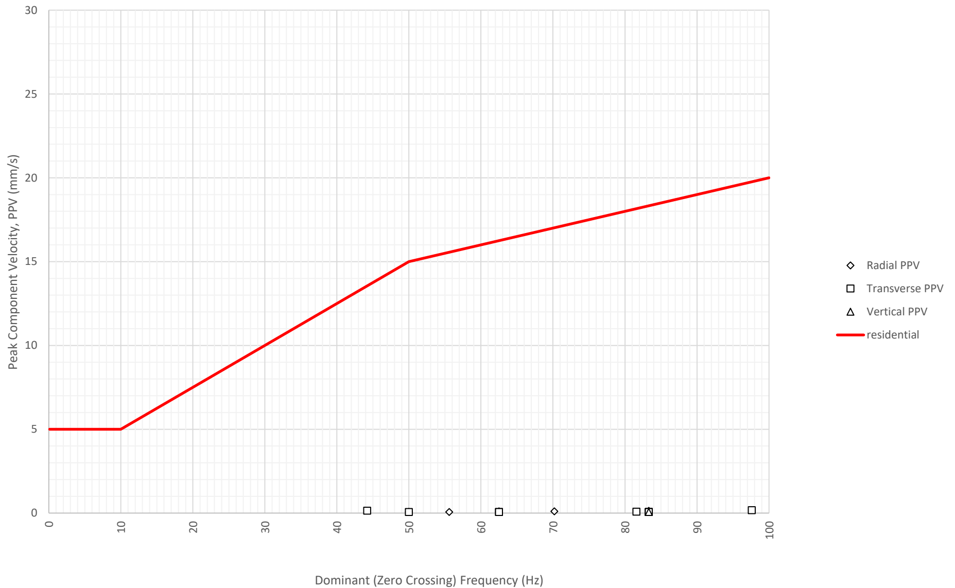
Frequency Content of Vibration Levels at North Boundary Near Block A and B (ETM7687) on 21-06-2024
