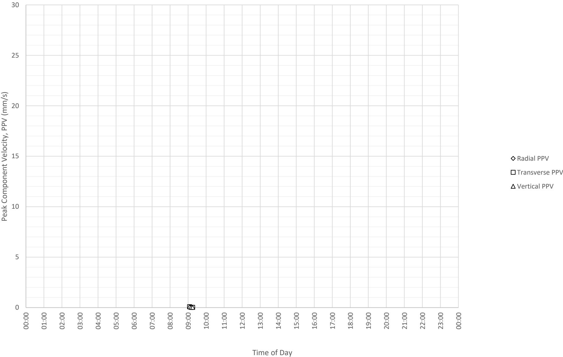
Daily Monitored Vibration Levels at North Boundary Near Block A and B (ETM7687) on 30-06-2024
