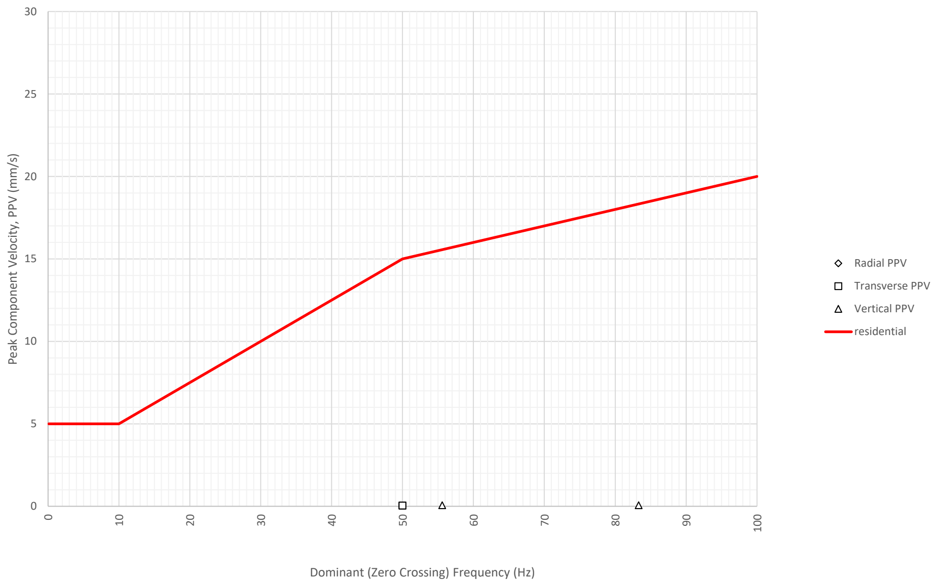
Frequency Content of Vibration Levels at East Boundary Opposite Shoalhaven Street (ETM7326) on 30-06-2024
