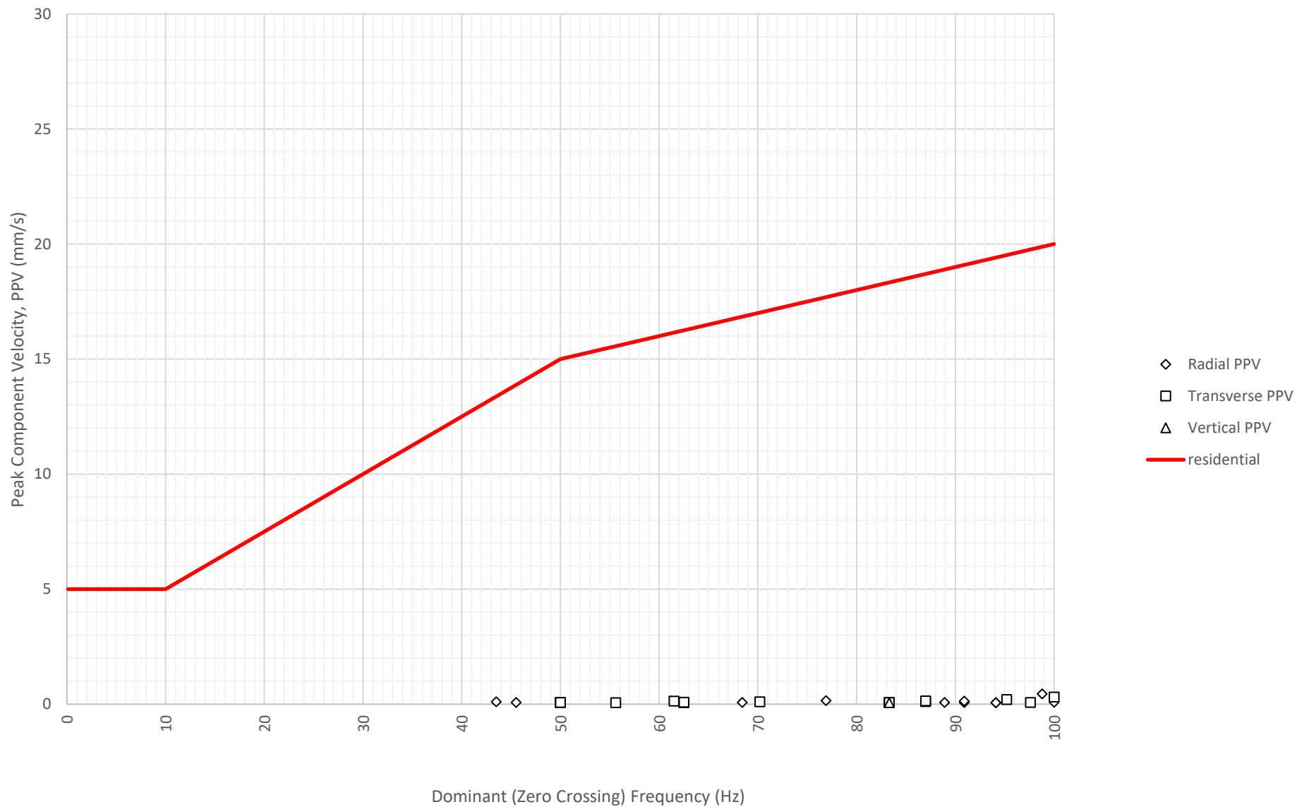
Frequency Content of Vibration Levels at North Boundary Near Block A and B (ETM7687) on 25-06-2024
