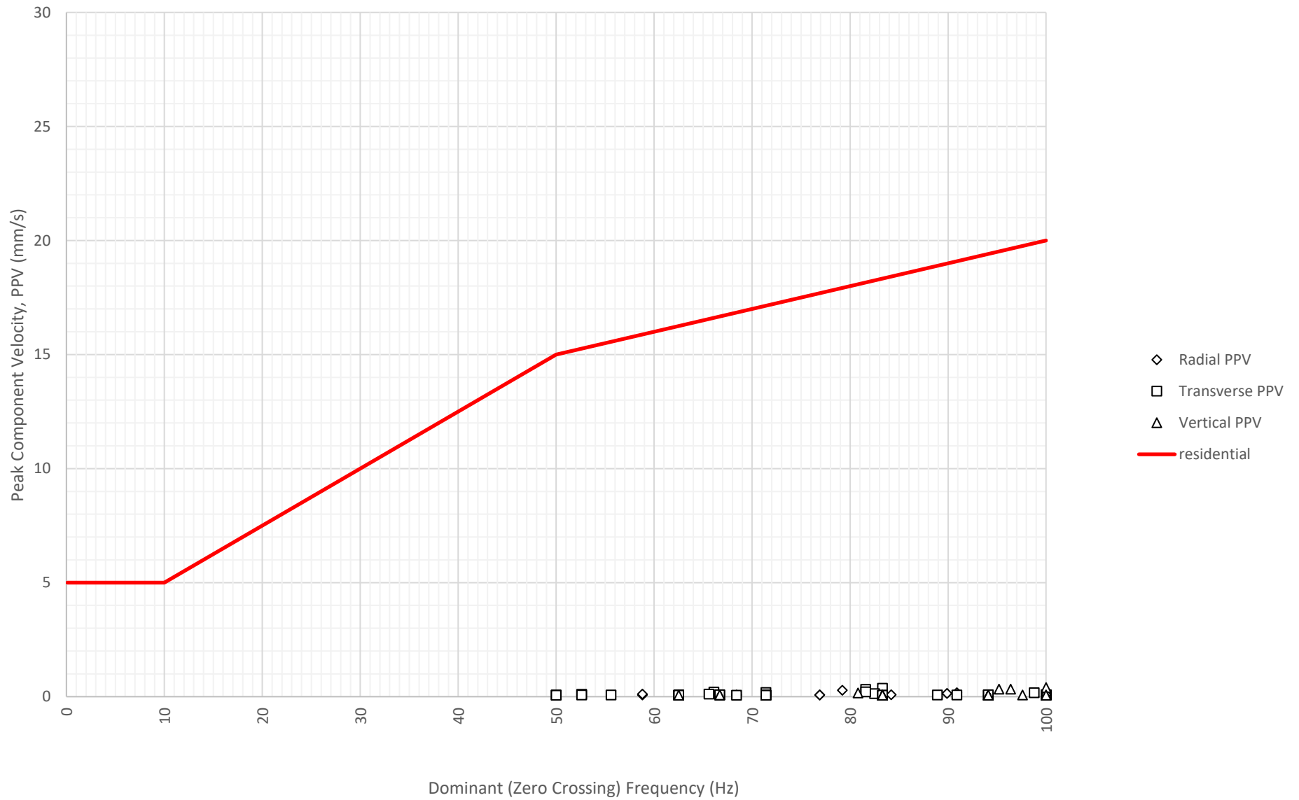
Frequency Content of Vibration Levels at North Boundary Near Block A and B (ETM7687) on 6-06-2024
