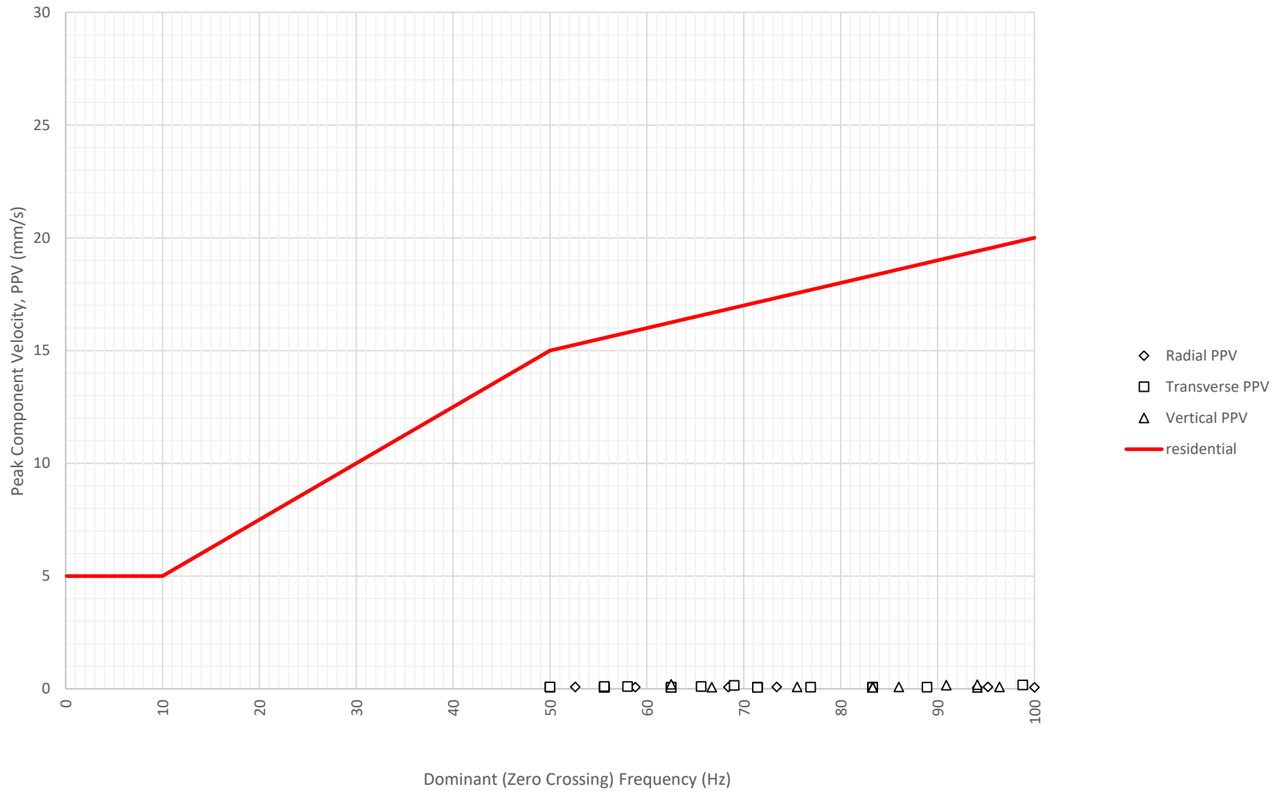
Frequency Content of Vibration Levels at North Boundary Near Block A and B (ETM7687) on 7-06-2024
