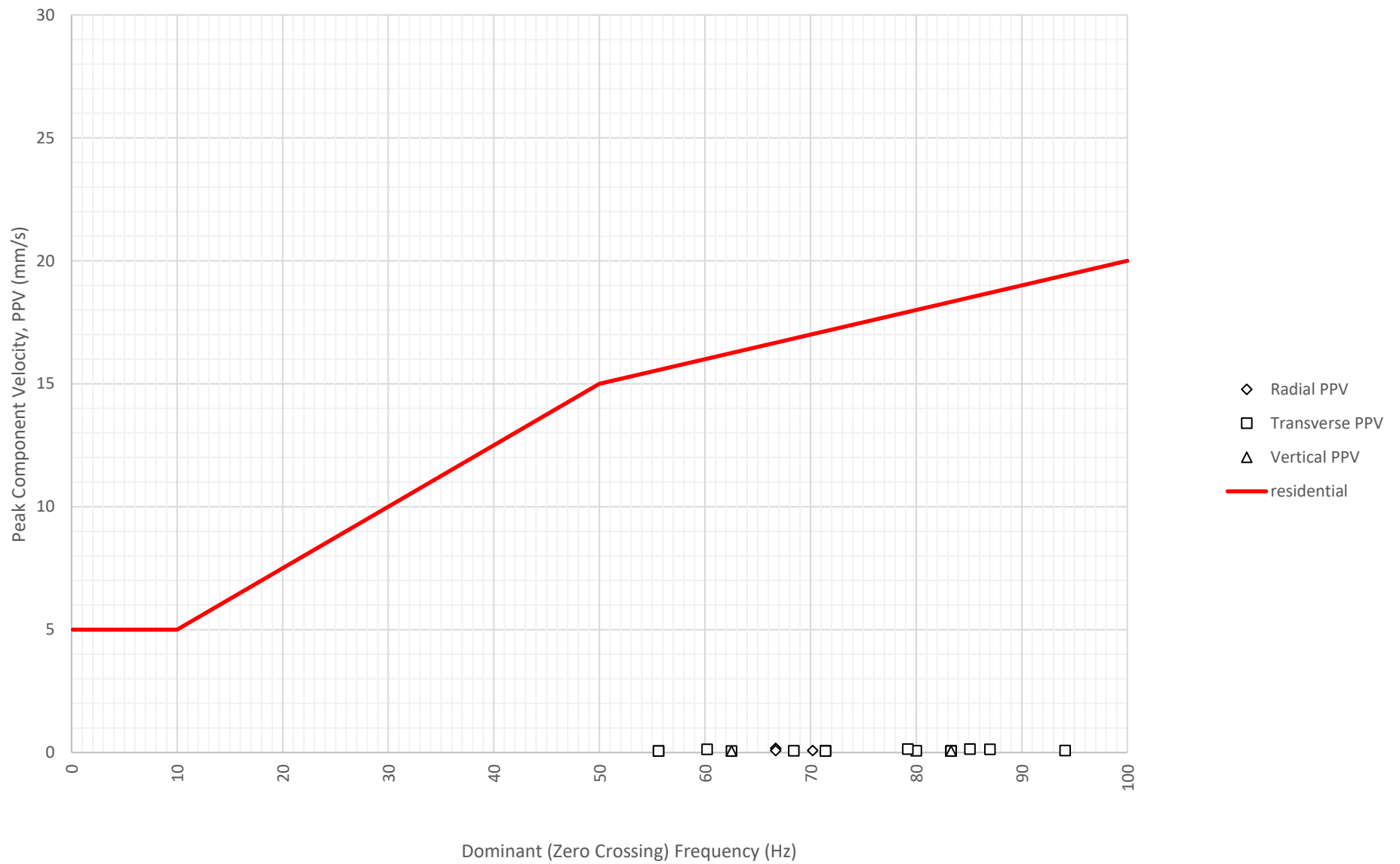
Frequency Content of Vibration Levels at North Boundary Near Block A and B (ETM7687) on 17-06-2024
