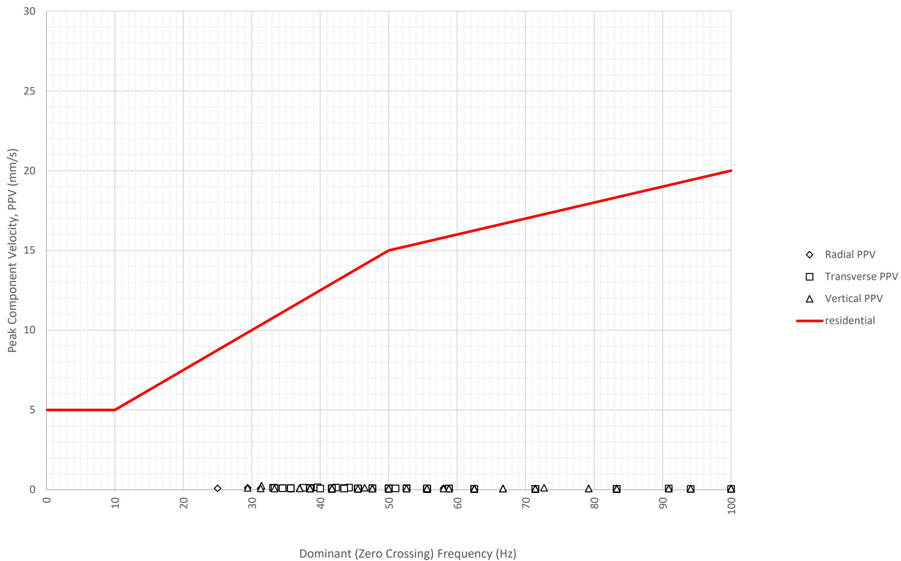
Frequency Content of Vibration Levels at East Boundary Opposite Shoalhaven Street (ETM7326) on 22-06-2024
