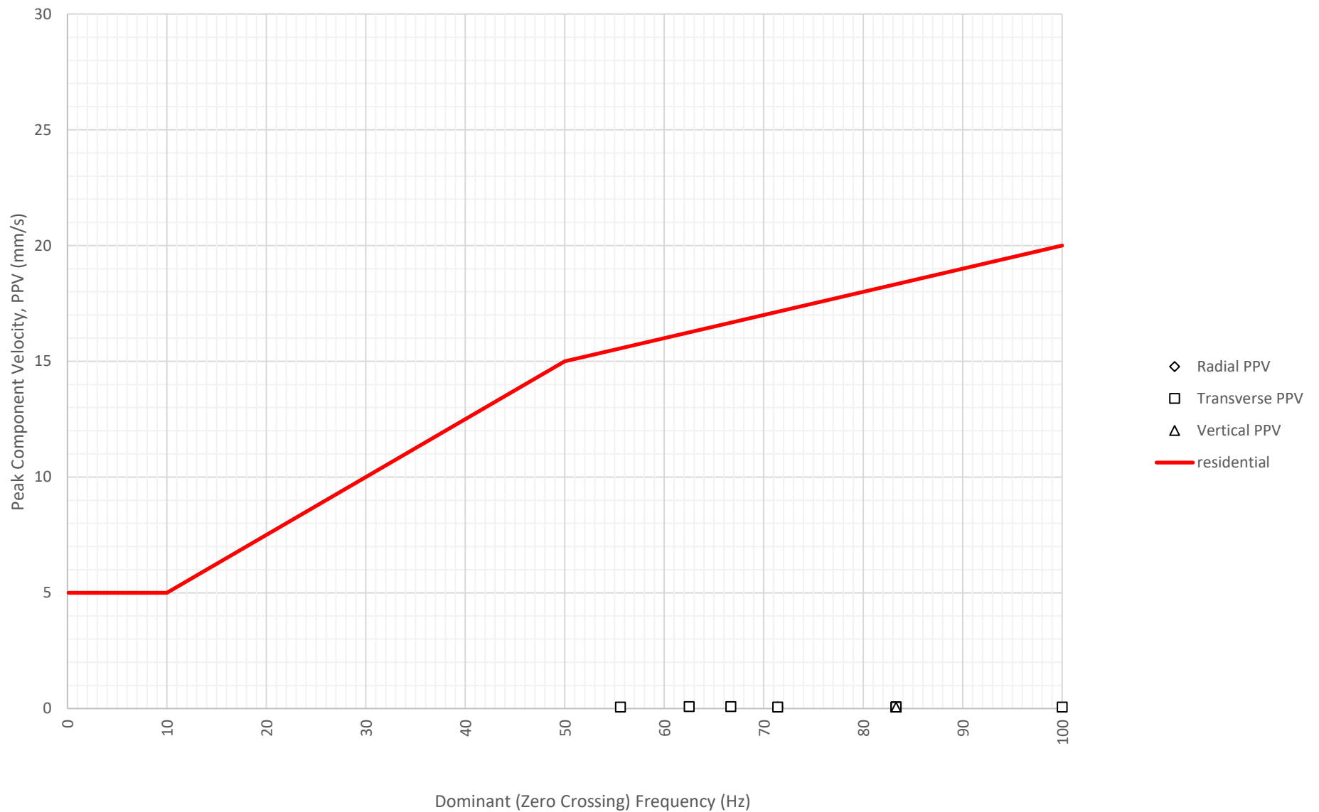
Frequency Content of Vibration Levels at North Boundary Near Block A and B (ETM7687) on 11-06-2024
