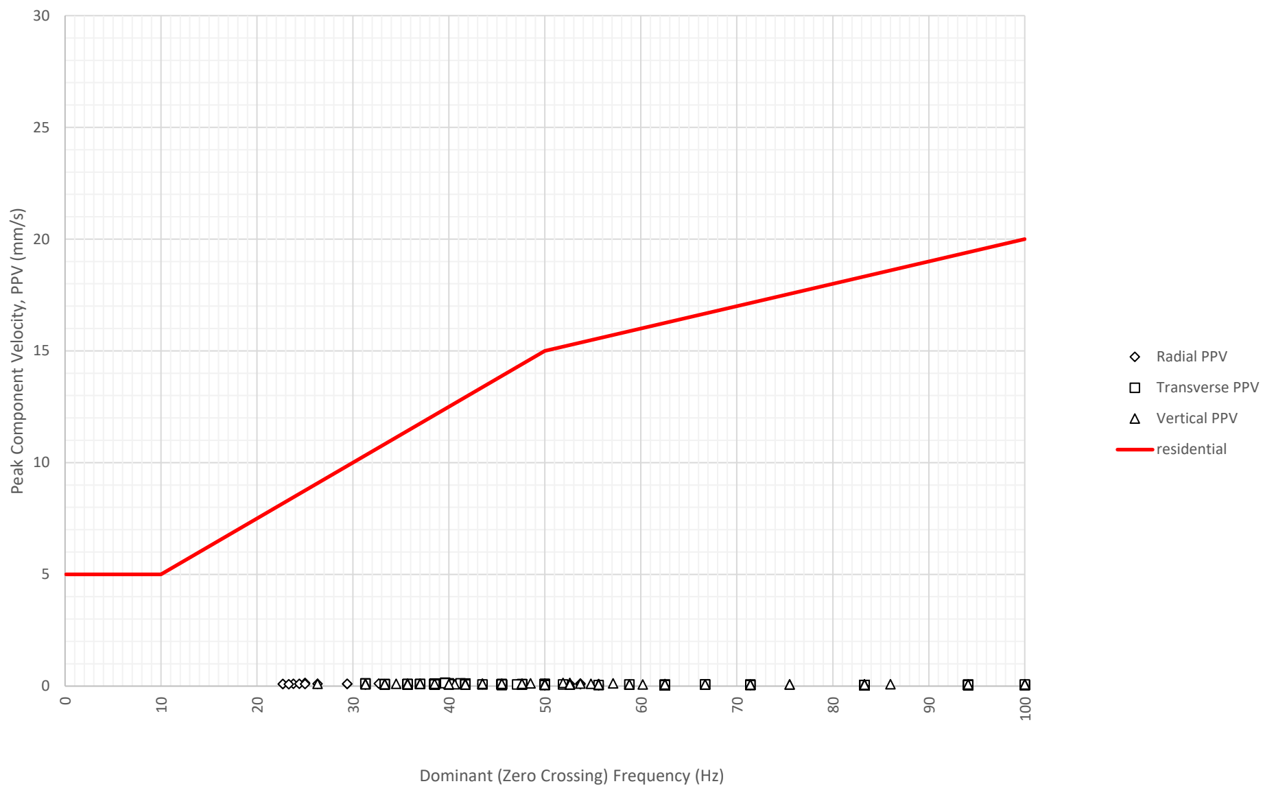
Frequency Content of Vibration Levels at East Boundary Opposite Shoalhaven Street (ETM7326) on 24-06-2024
