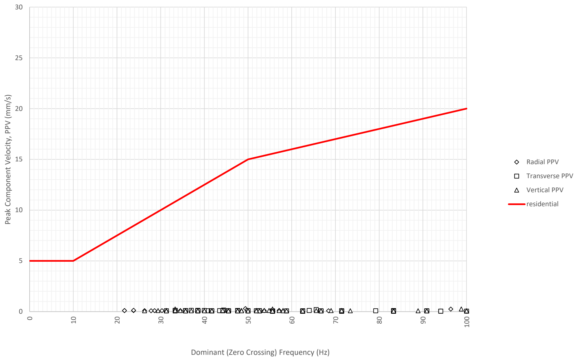
Frequency Content of Vibration Levels at East Boundary Opposite Shoalhaven Street (ETM7326) on 19-06-2024
