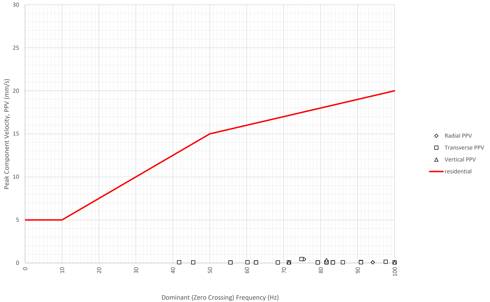
Frequency Content of Vibration Levels at North Boundary Near Block A and B (ETM7687) on 4-06-2024
