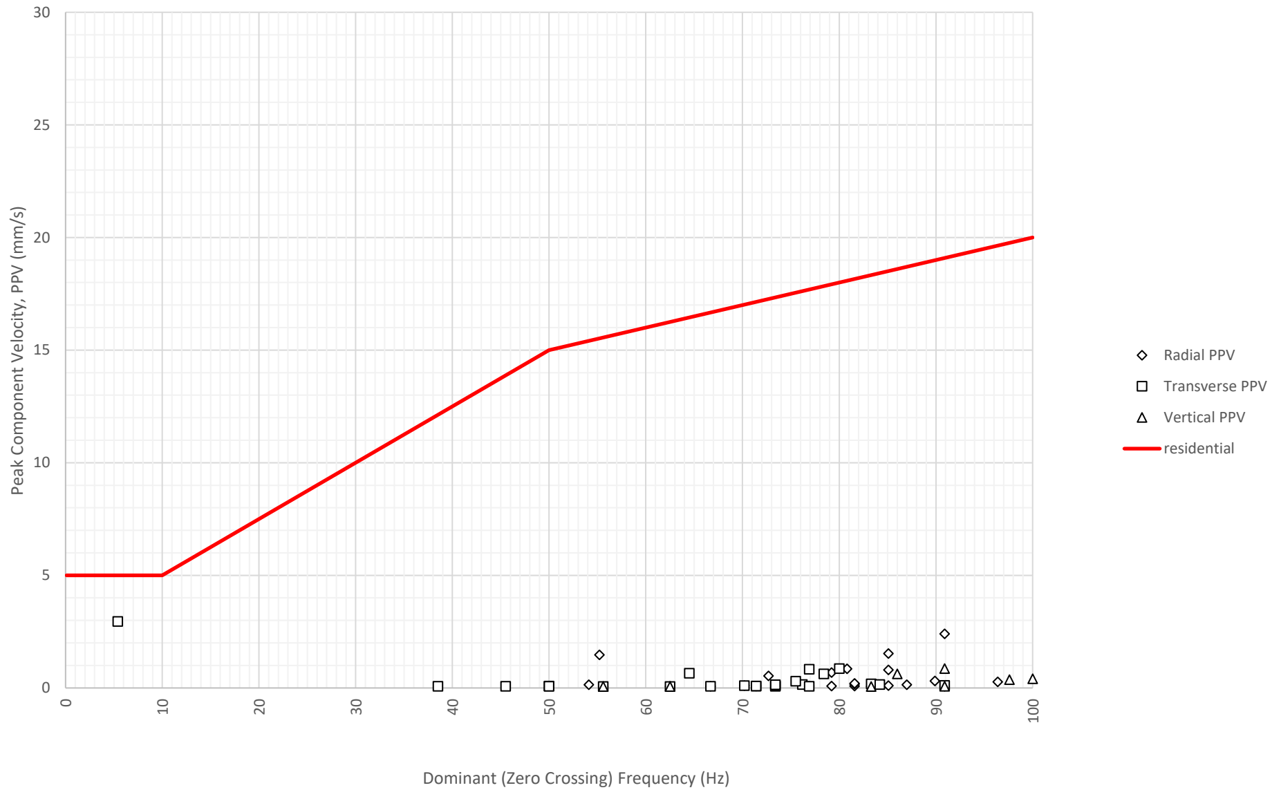
Frequency Content of Vibration Levels at North Boundary Near Block A and B (ETM7687) on 13-06-2024
