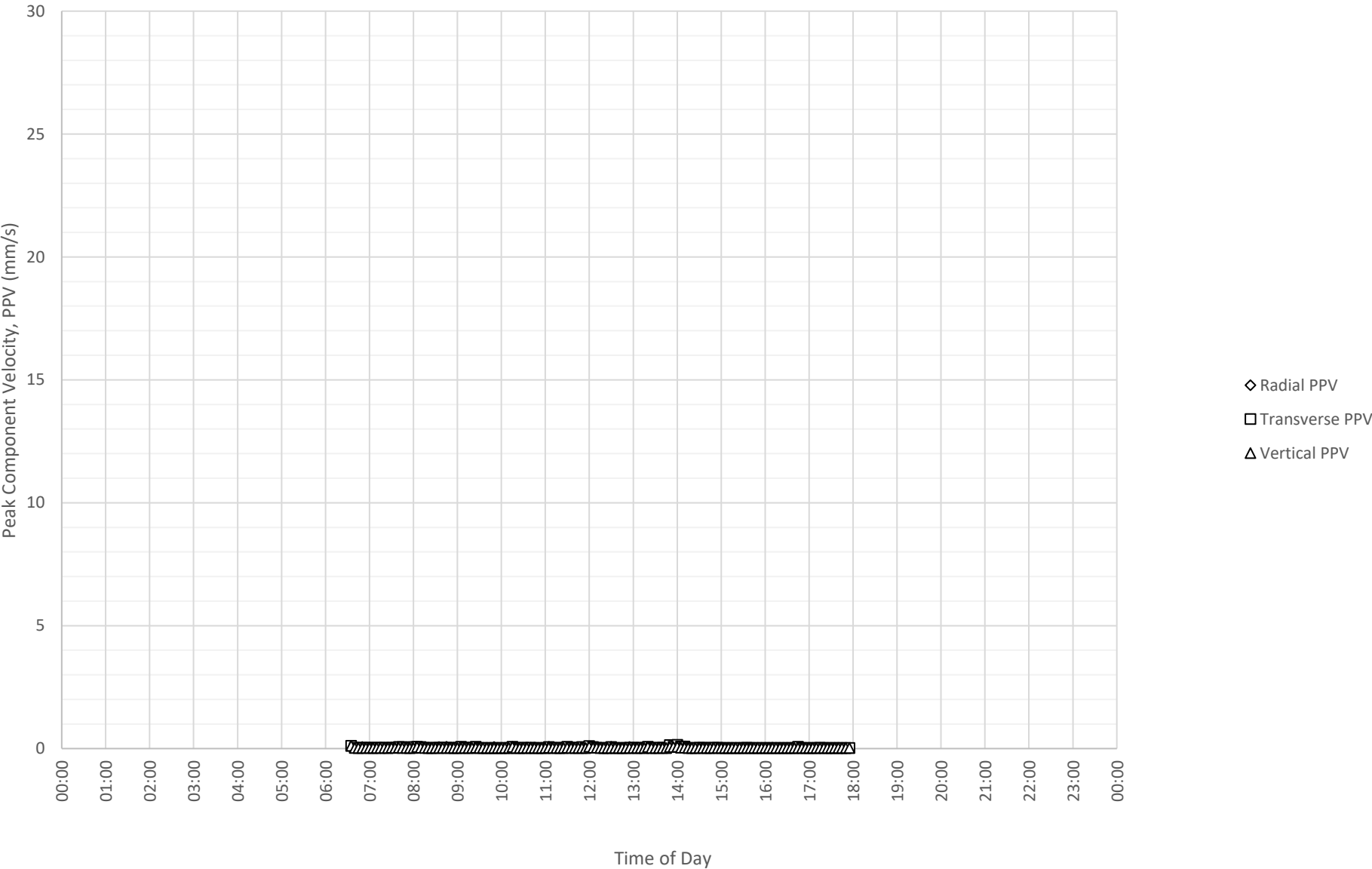
Daily Monitored Vibration Levels at North Boundary Near Block A and B (ETM7687) on 3-06-2024
