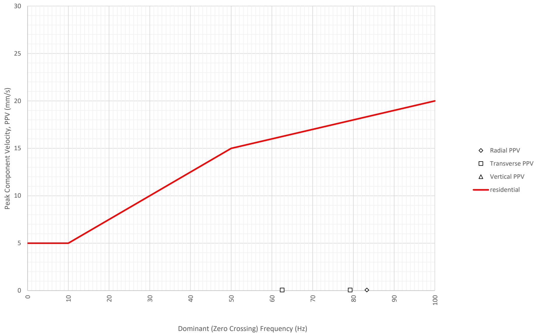
Frequency Content of Vibration Levels at North Boundary Near Block A and B (ETM7687) on 10-06-2024
