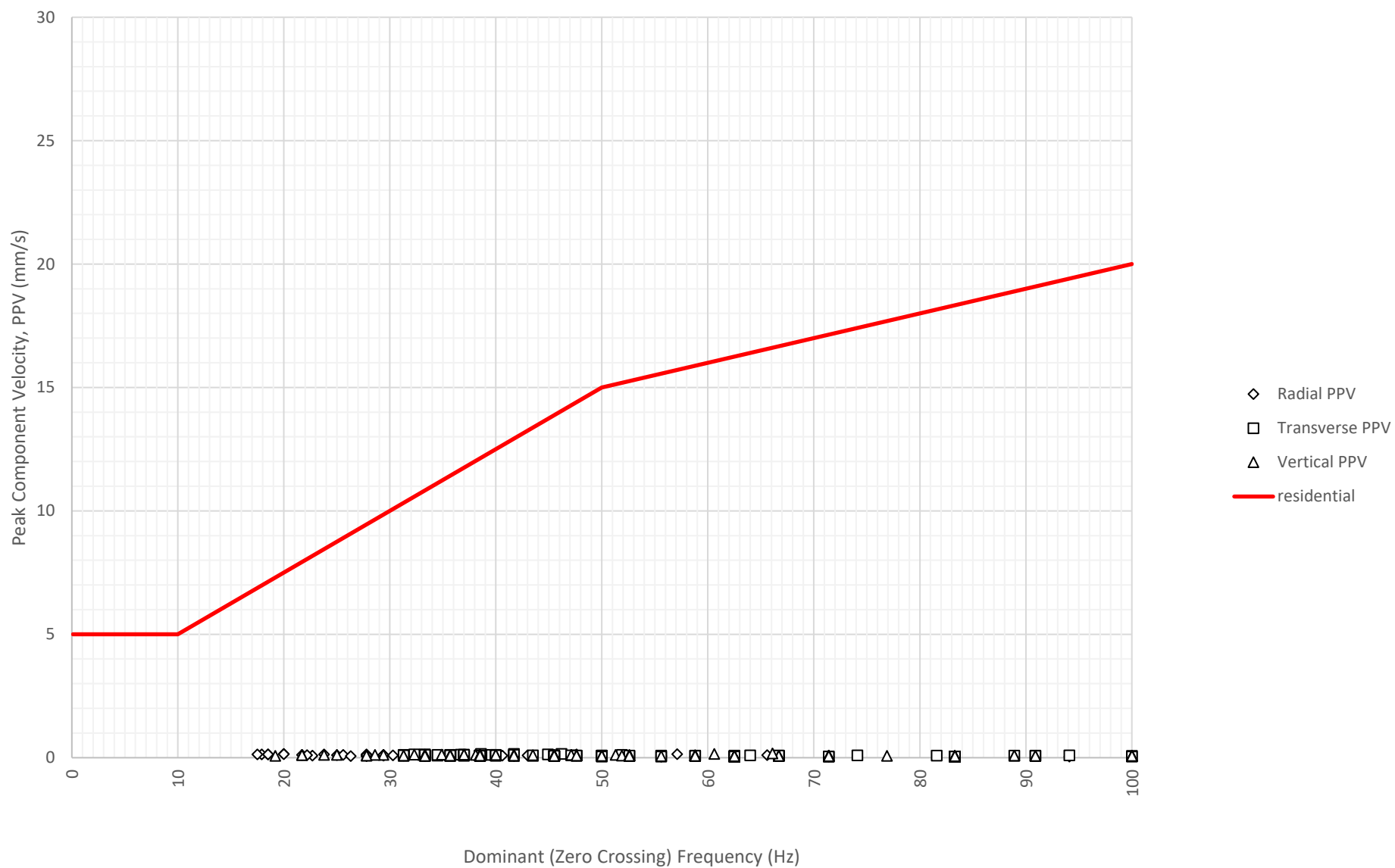
Frequency Content of Vibration Levels at East Boundary Opposite Shoalhaven Street (ETM7326) on 17-06-2024
