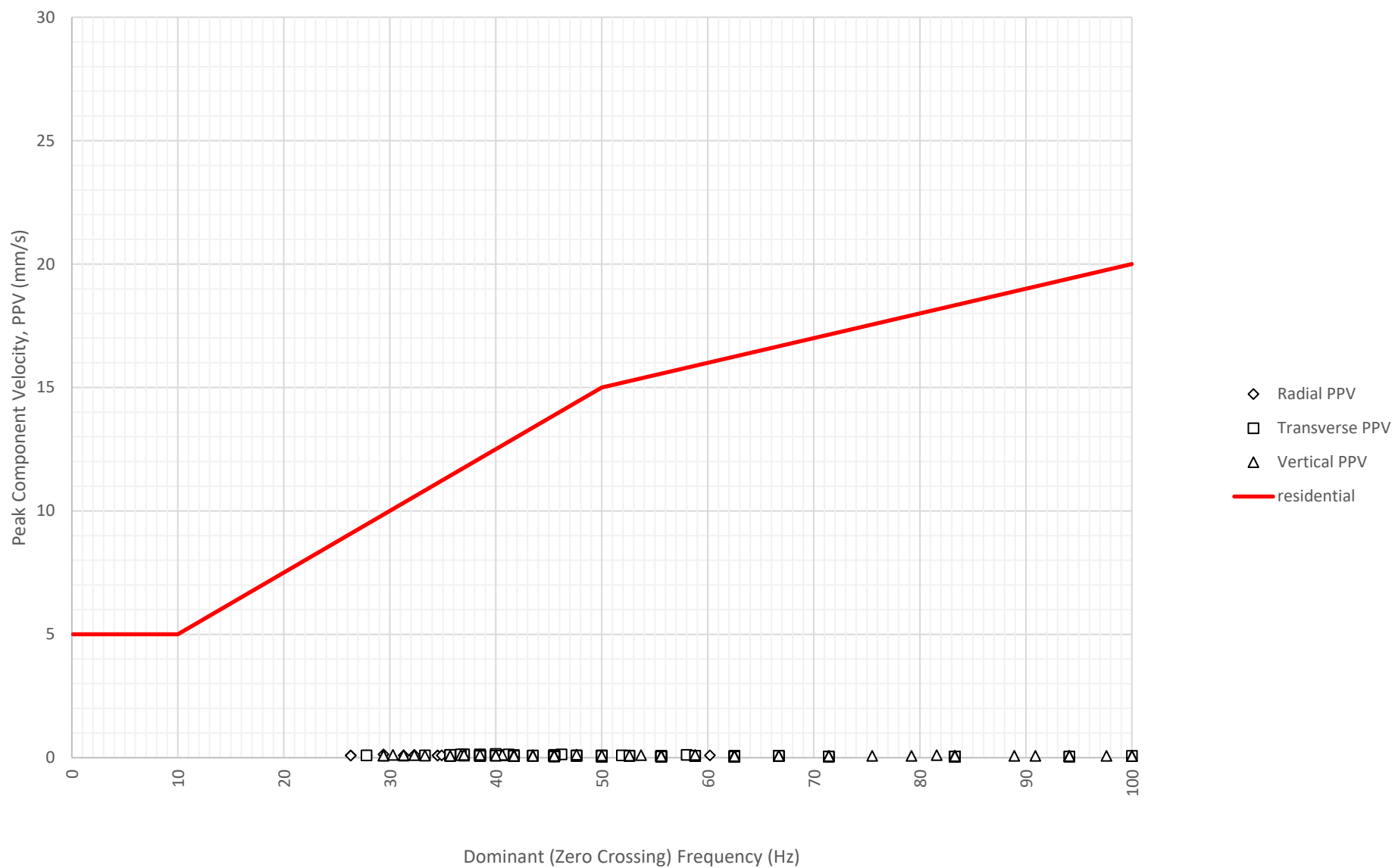
Frequency Content of Vibration Levels at East Boundary Opposite Shoalhaven Street (ETM7326) on 28-06-2024
