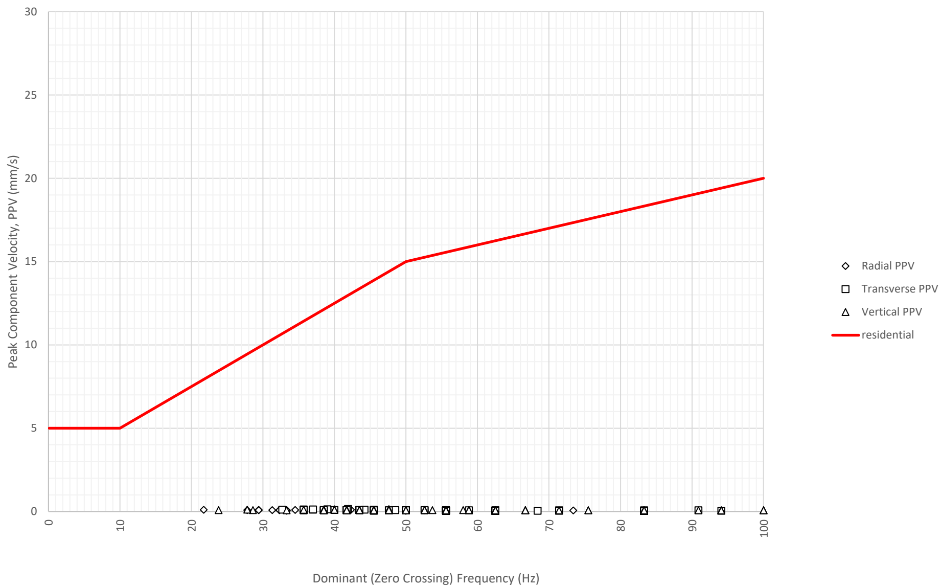
Frequency Content of Vibration Levels at East Boundary Opposite Shoalhaven Street (ETM7326) on 27-06-2024
