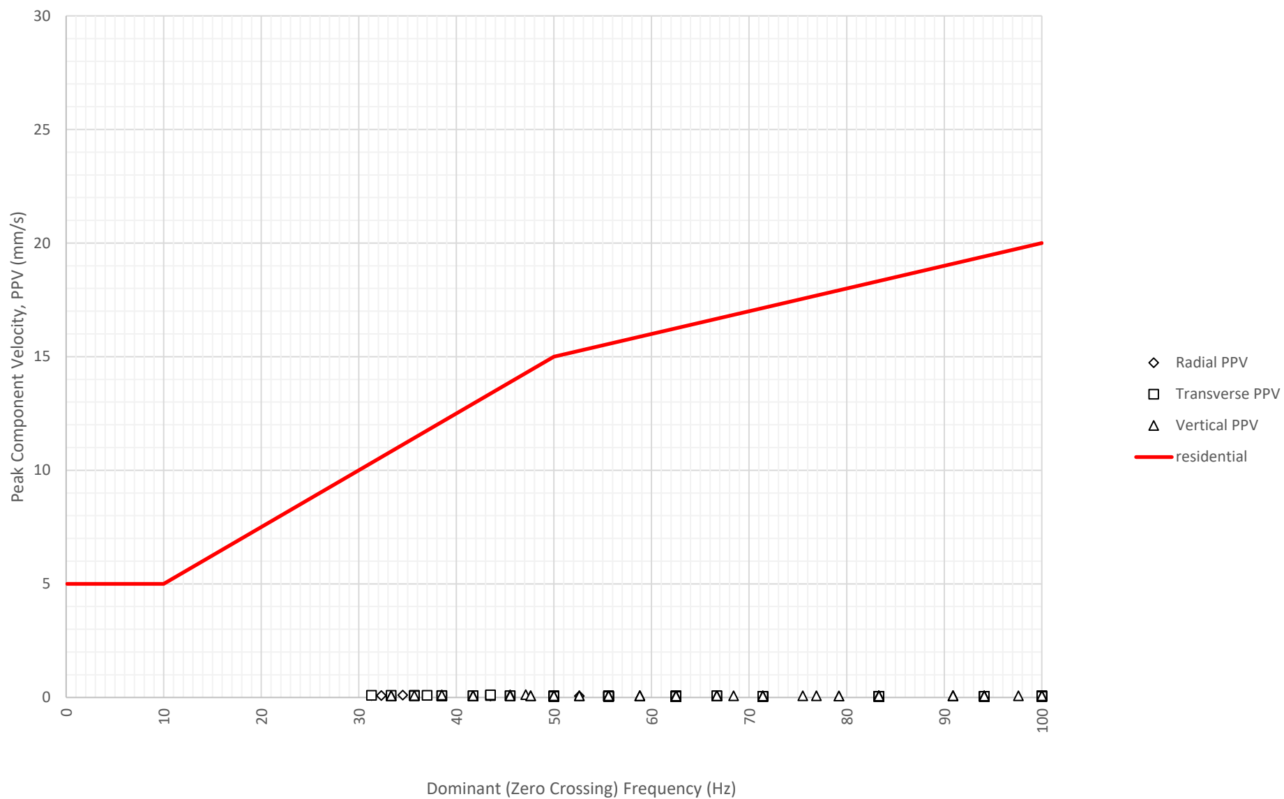
Frequency Content of Vibration Levels at East Boundary Opposite Shoalhaven Street (ETM7326) on 10-06-2024
