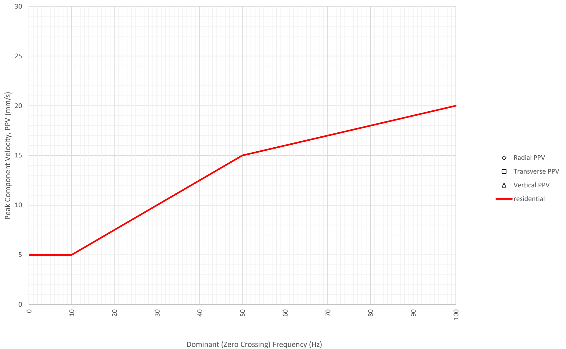
Frequency Content of Vibration Levels at North Boundary Near Block A and B (ETM7687) on 23-06-2024
