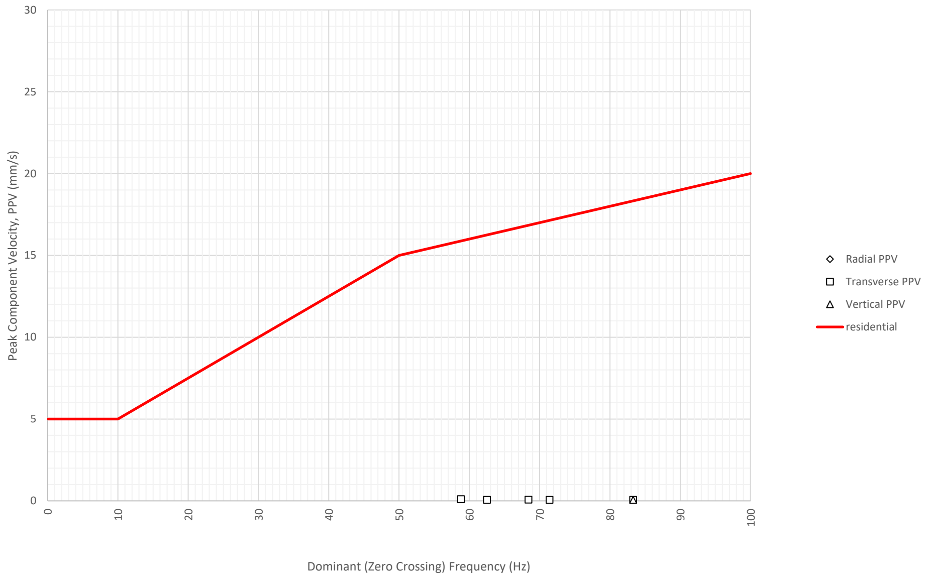
Frequency Content of Vibration Levels at North Boundary Near Block A and B (ETM7687) on 15-06-2024
