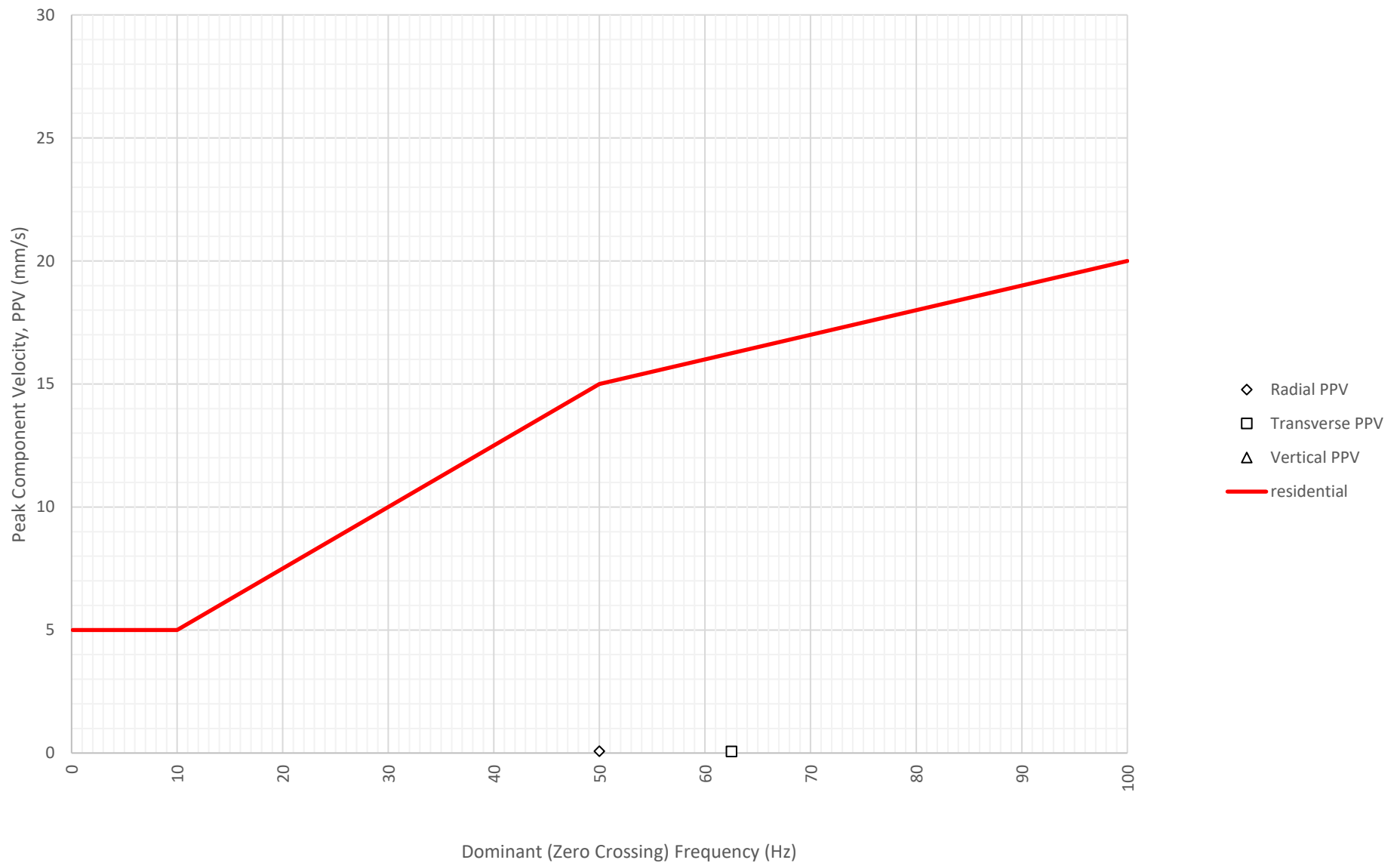
Frequency Content of Vibration Levels at North Boundary Near Block A and B (ETM7687) on 22-06-2024
