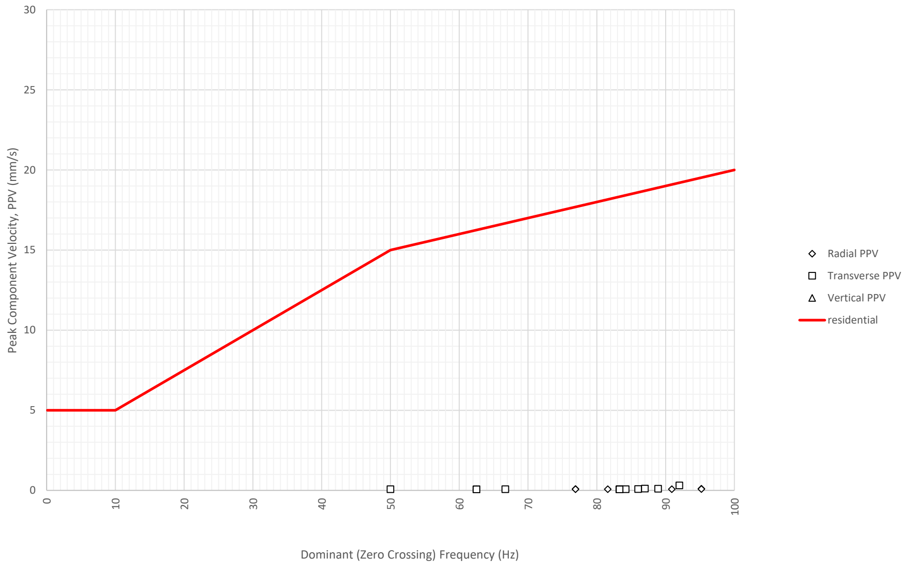
Frequency Content of Vibration Levels at North Boundary Near Block A and B (ETM7687) on 14-06-2024
