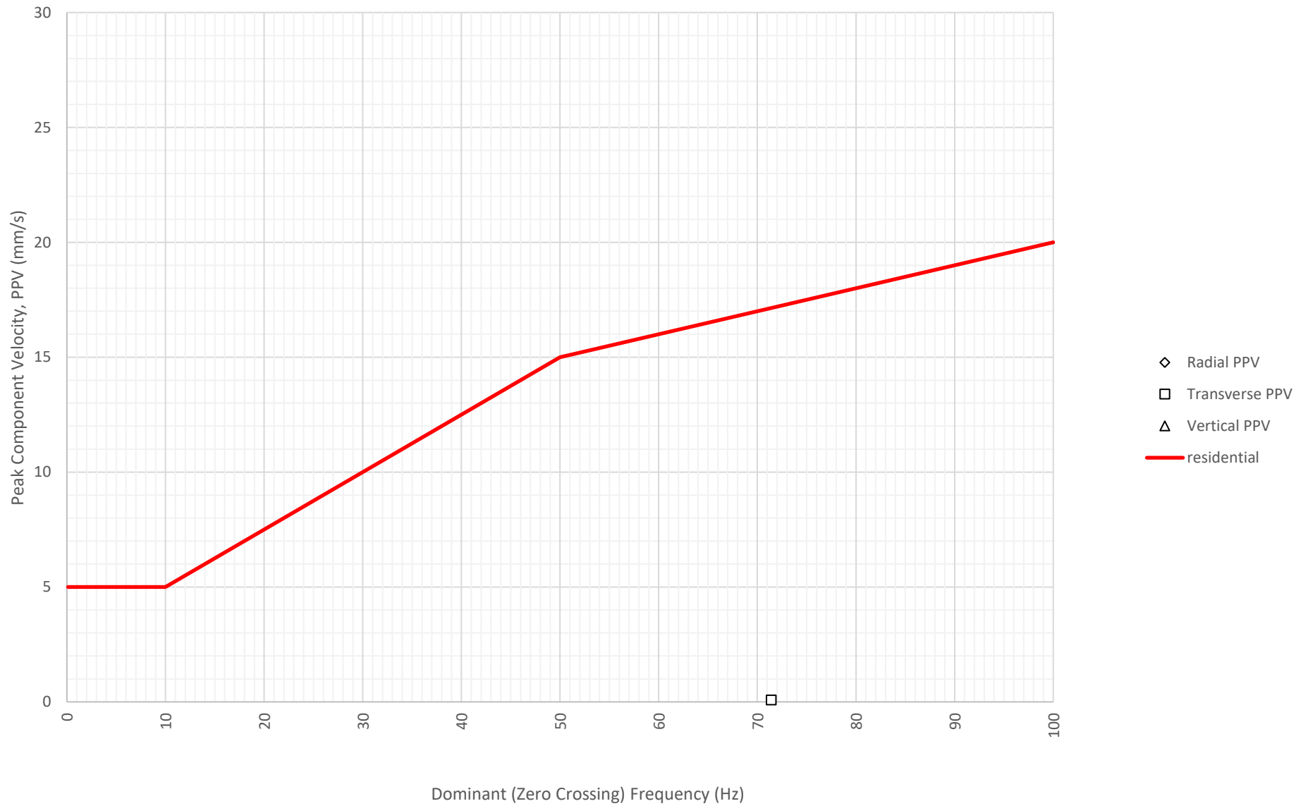
Frequency Content of Vibration Levels at North Boundary Near Block A and B (ETM7687) on 8-06-2024
