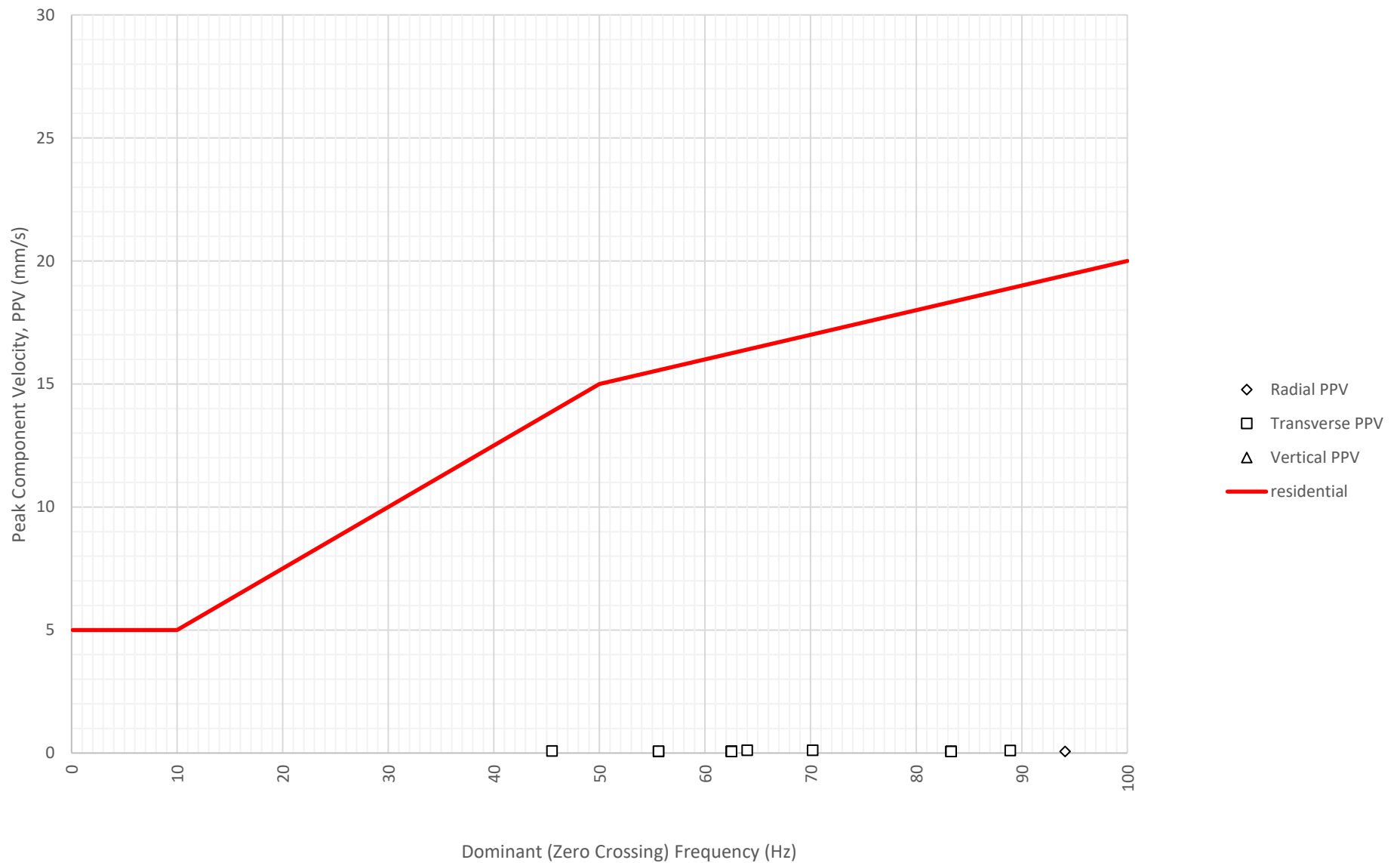
Frequency Content of Vibration Levels at North Boundary Near Block A and B (ETM7687) on 20-06-2024
