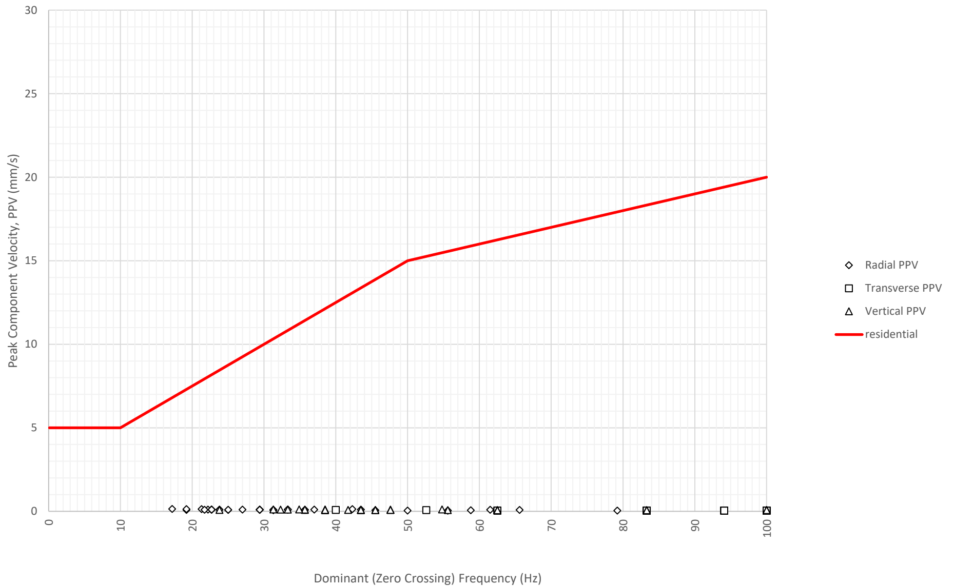
Frequency Content of Vibration Levels at East Boundary Opposite Shoalhaven Street (ETM7326) on 6-06-2024
