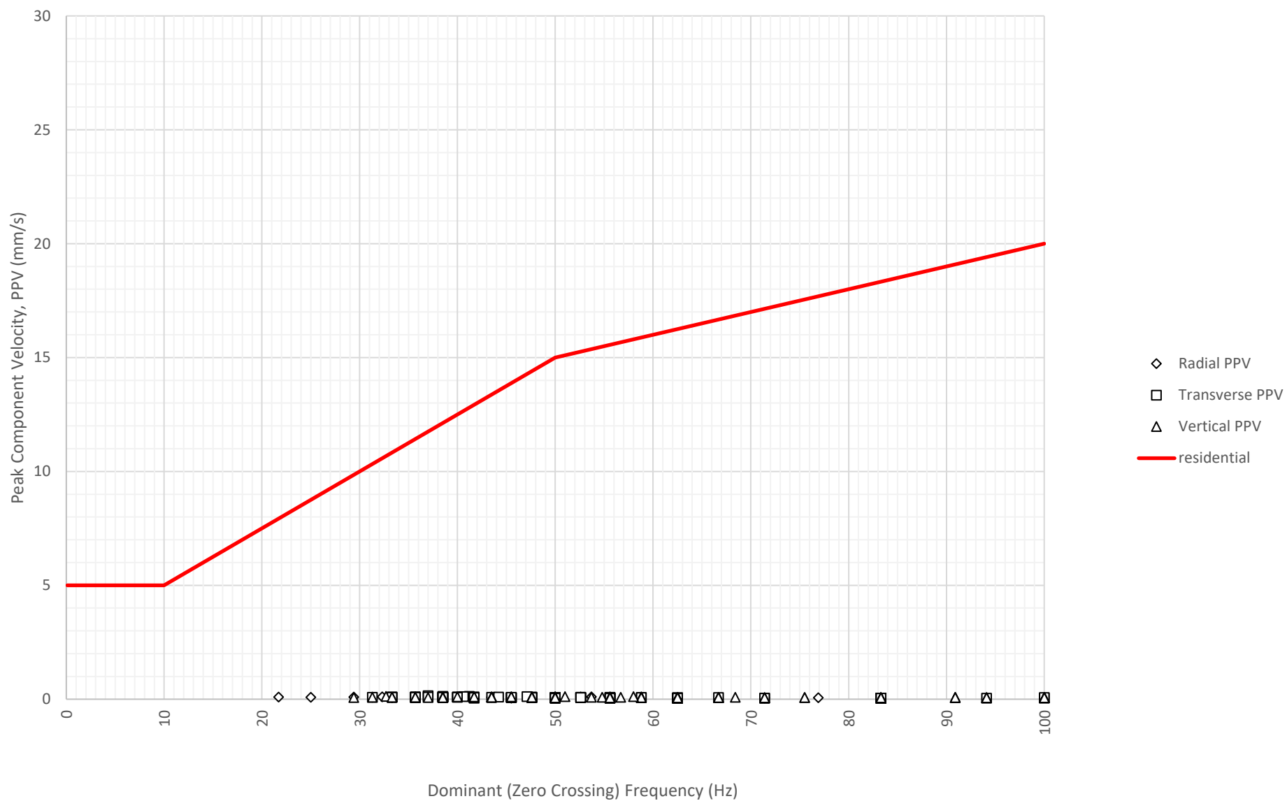
Frequency Content of Vibration Levels at East Boundary Opposite Shoalhaven Street (ETM7326) on 26-06-2024
