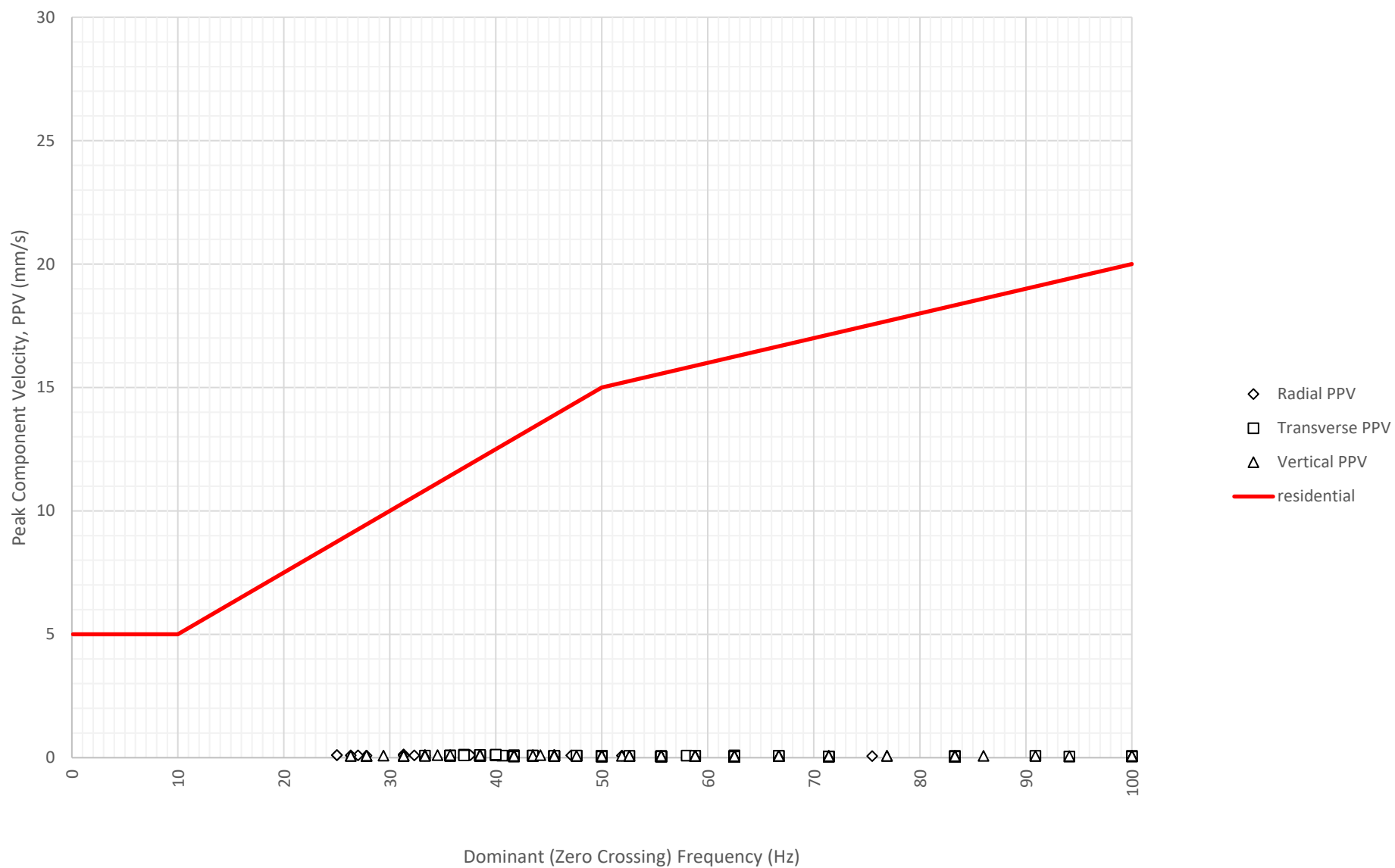
Frequency Content of Vibration Levels at East Boundary Opposite Shoalhaven Street (ETM7326) on 15-06-2024
