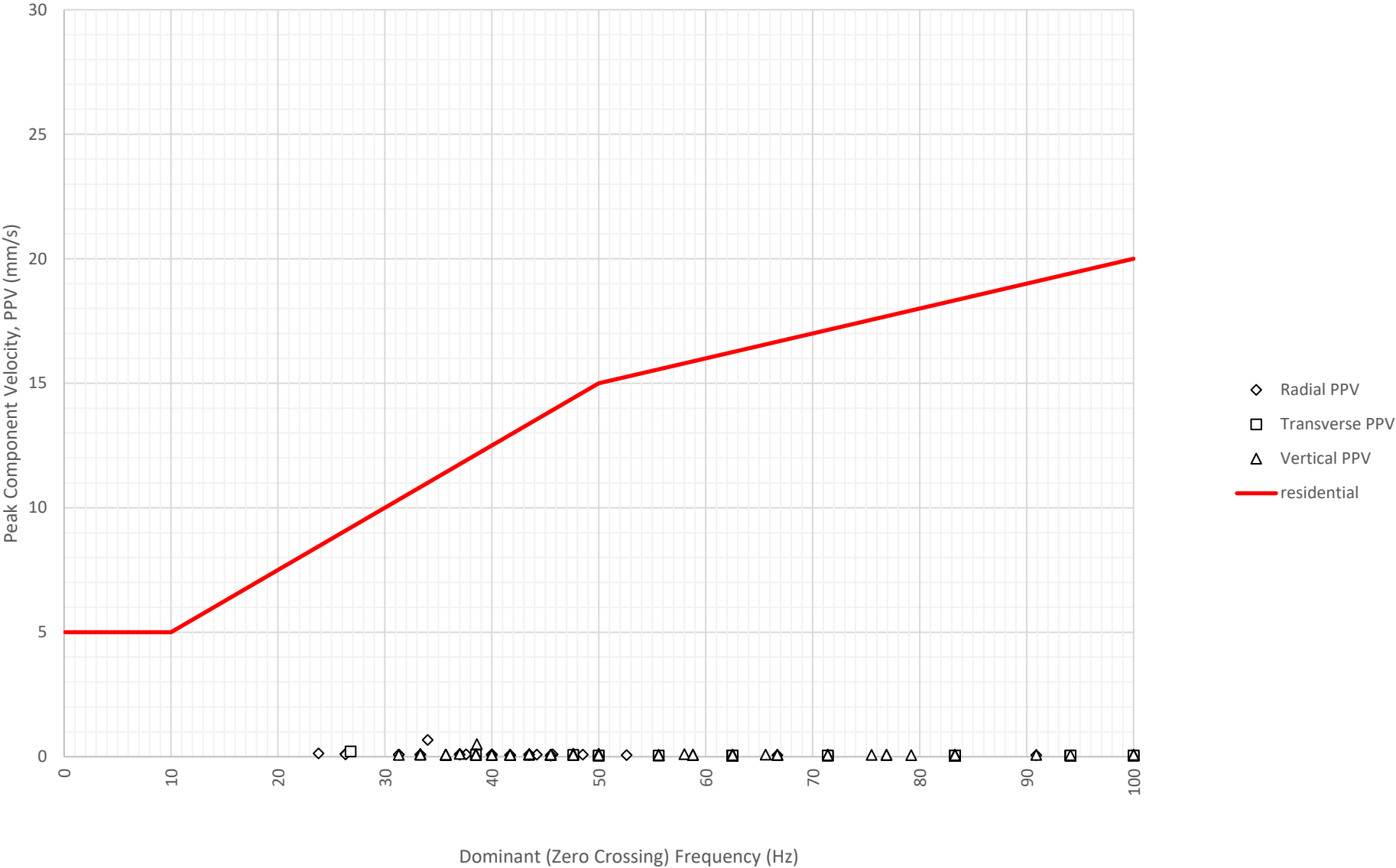
Frequency Content of Vibration Levels at East Boundary Opposite Shoalhaven Street (ETM7326) on 5-06-2024
