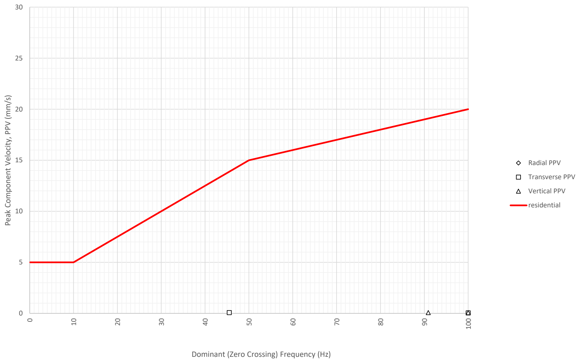
Frequency Content of Vibration Levels at East Boundary Opposite Shoalhaven Street (ETM7326) on 16-06-2024
