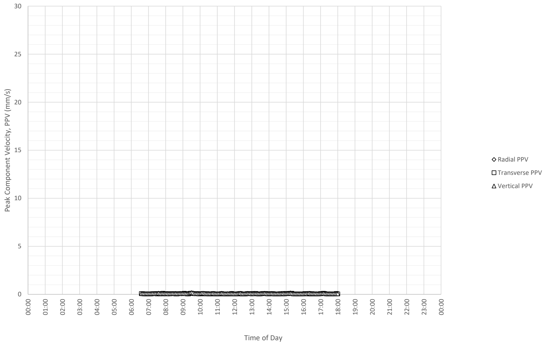
Daily Monitored Vibration Levels at East Boundary Opposite Shoalhaven Street (ETM7326) on 7-06-2024
