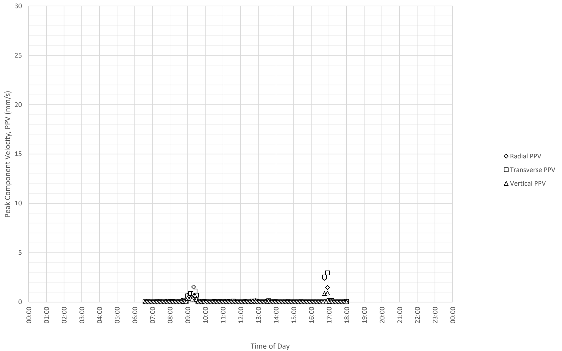
Daily Monitored Vibration Levels at North Boundary Near Block A and B (ETM7687) on 13-06-2024
