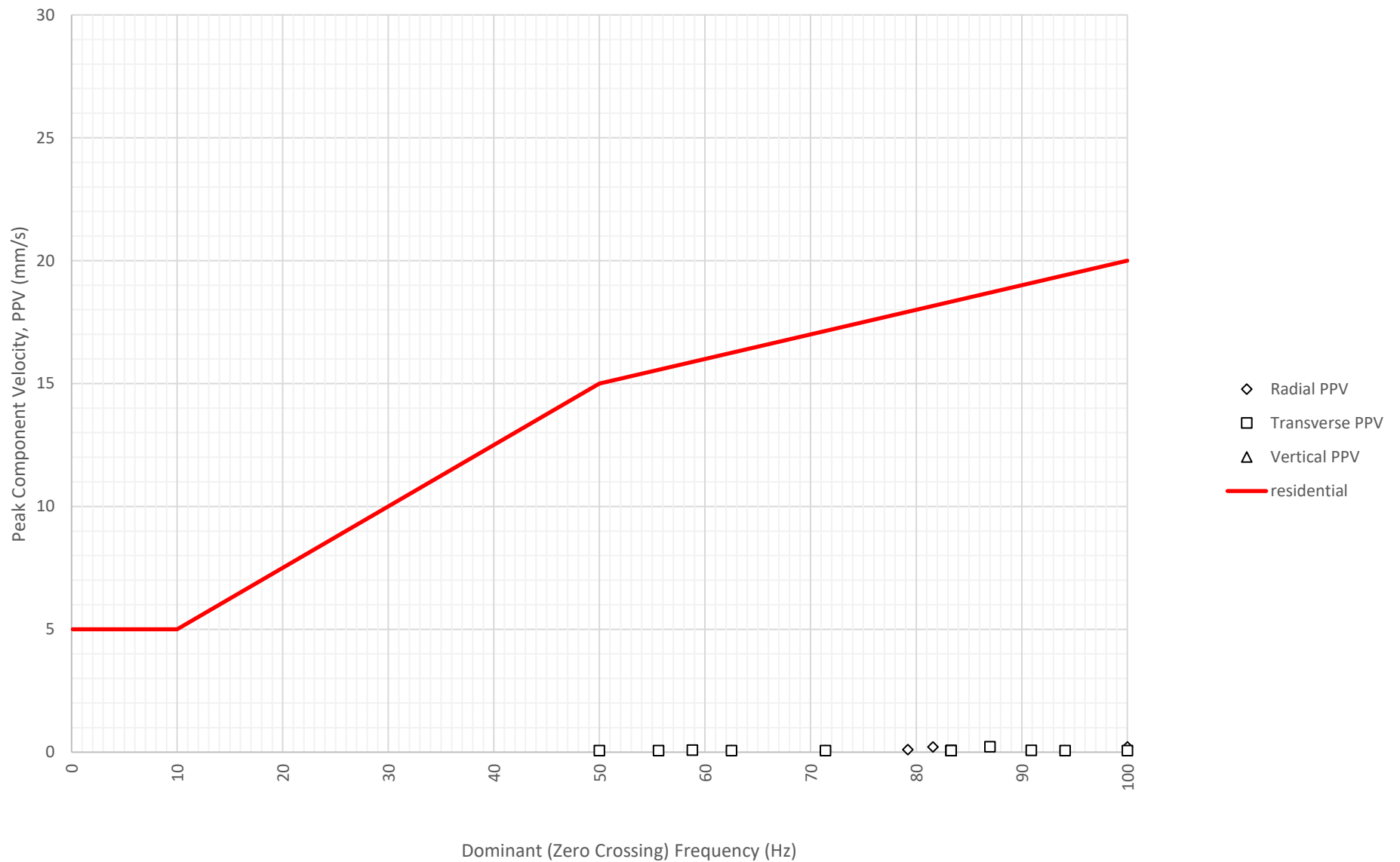
Frequency Content of Vibration Levels at North Boundary Near Block A and B (ETM7687) on 26-06-2024
