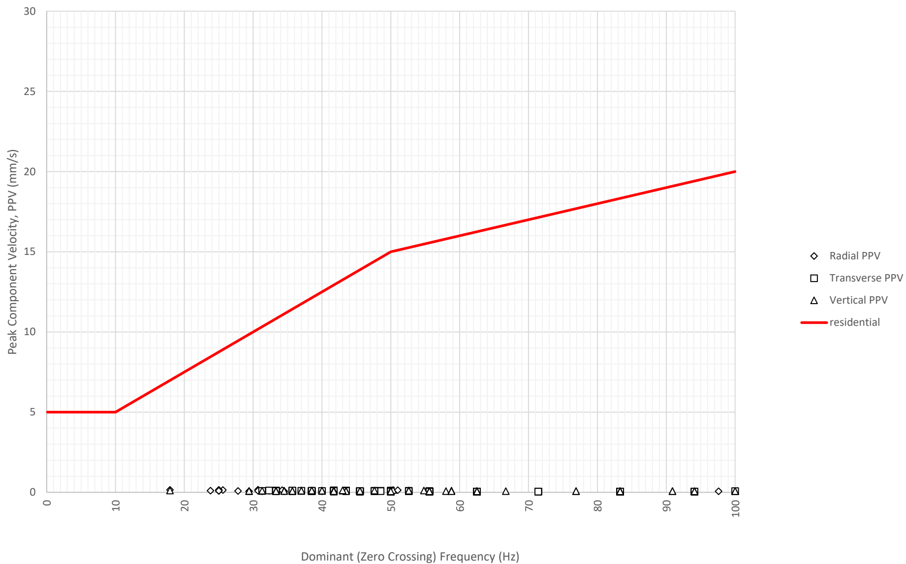
Frequency Content of Vibration Levels at East Boundary Opposite Shoalhaven Street (ETM7326) on 18-06-2024
