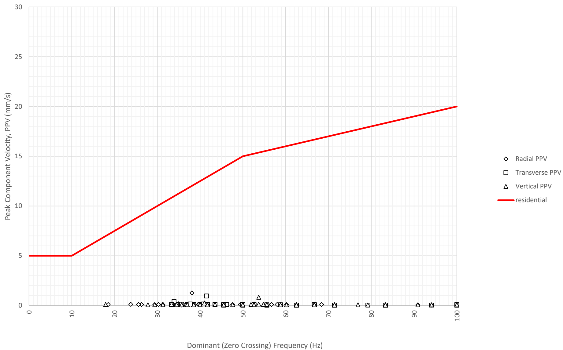
Frequency Content of Vibration Levels at East Boundary Opposite Shoalhaven Street (ETM7326) on 20-06-2024
