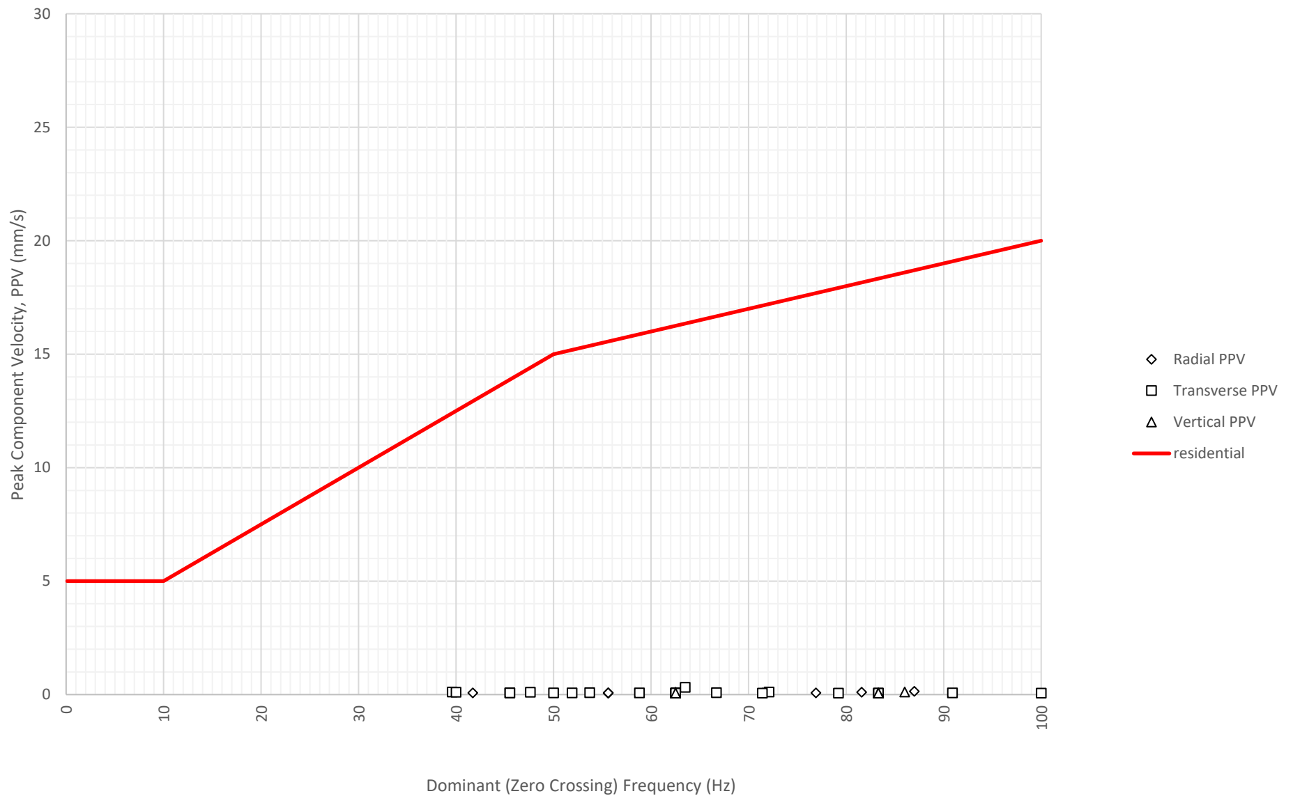
Frequency Content of Vibration Levels at North Boundary Near Block A and B (ETM7687) on 18-06-2024
