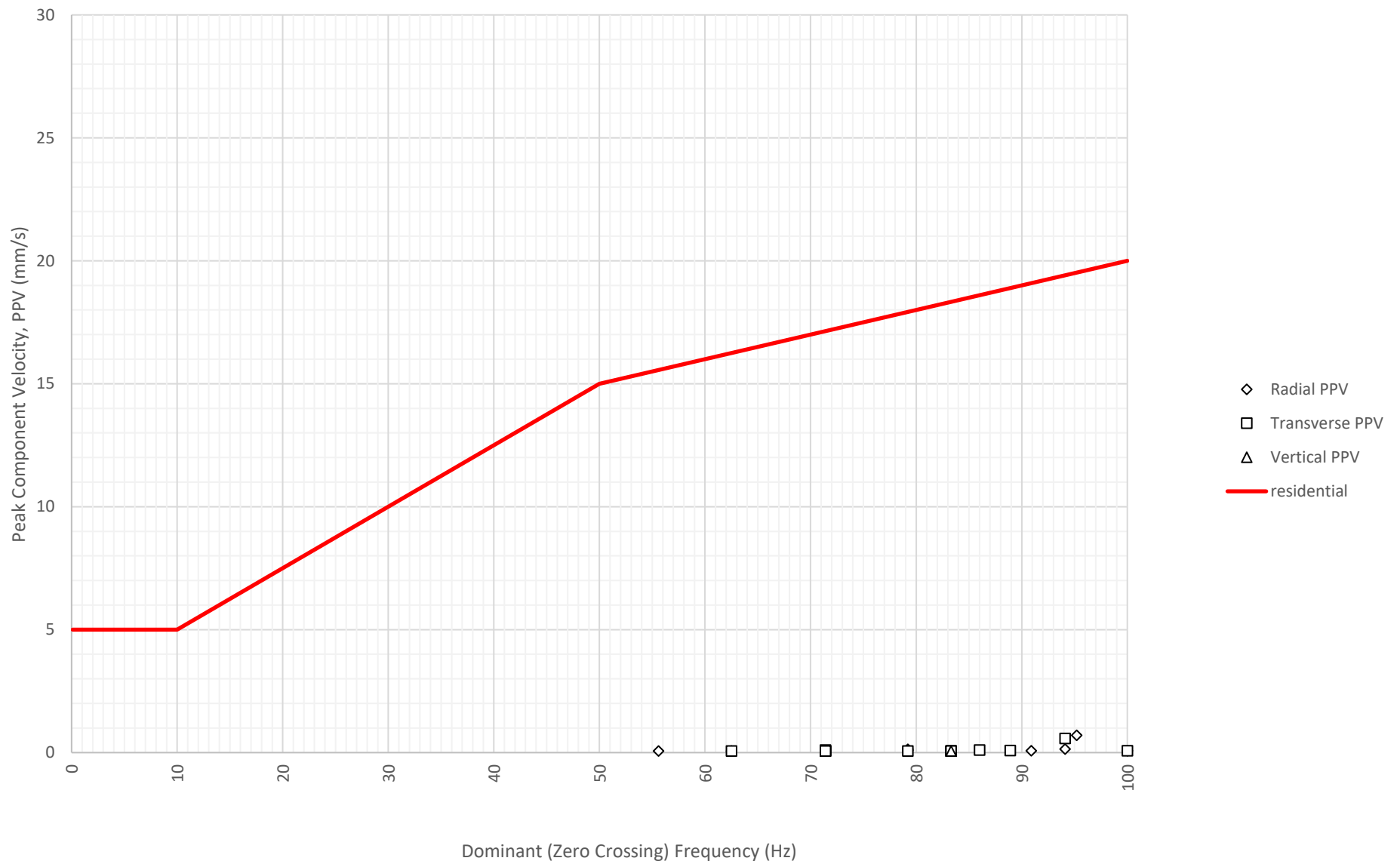
Frequency Content of Vibration Levels at North Boundary Near Block A and B (ETM7687) on 24-06-2024
