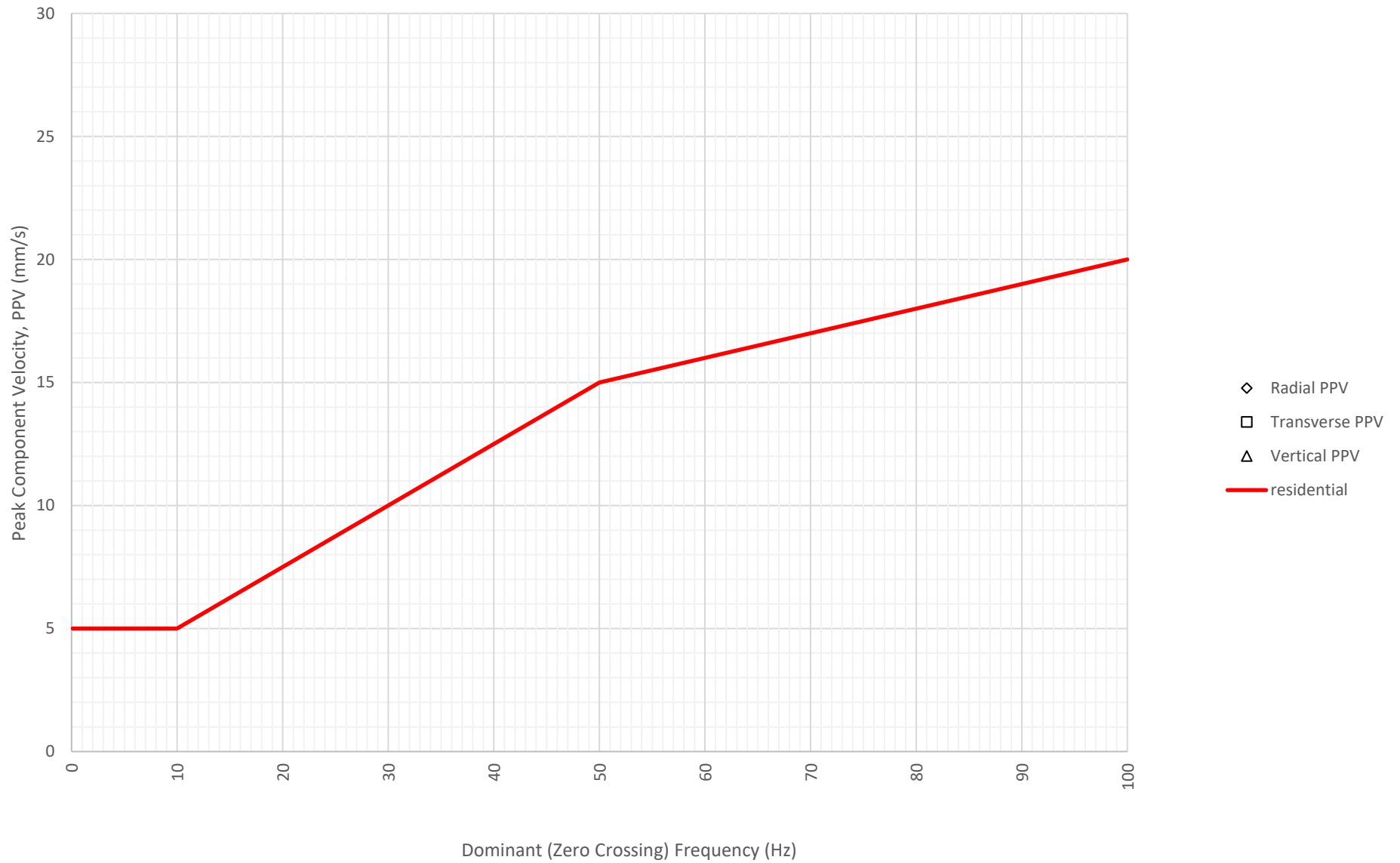
Frequency Content of Vibration Levels at North Boundary Near Block A and B (ETM7687) on 30-06-2024
