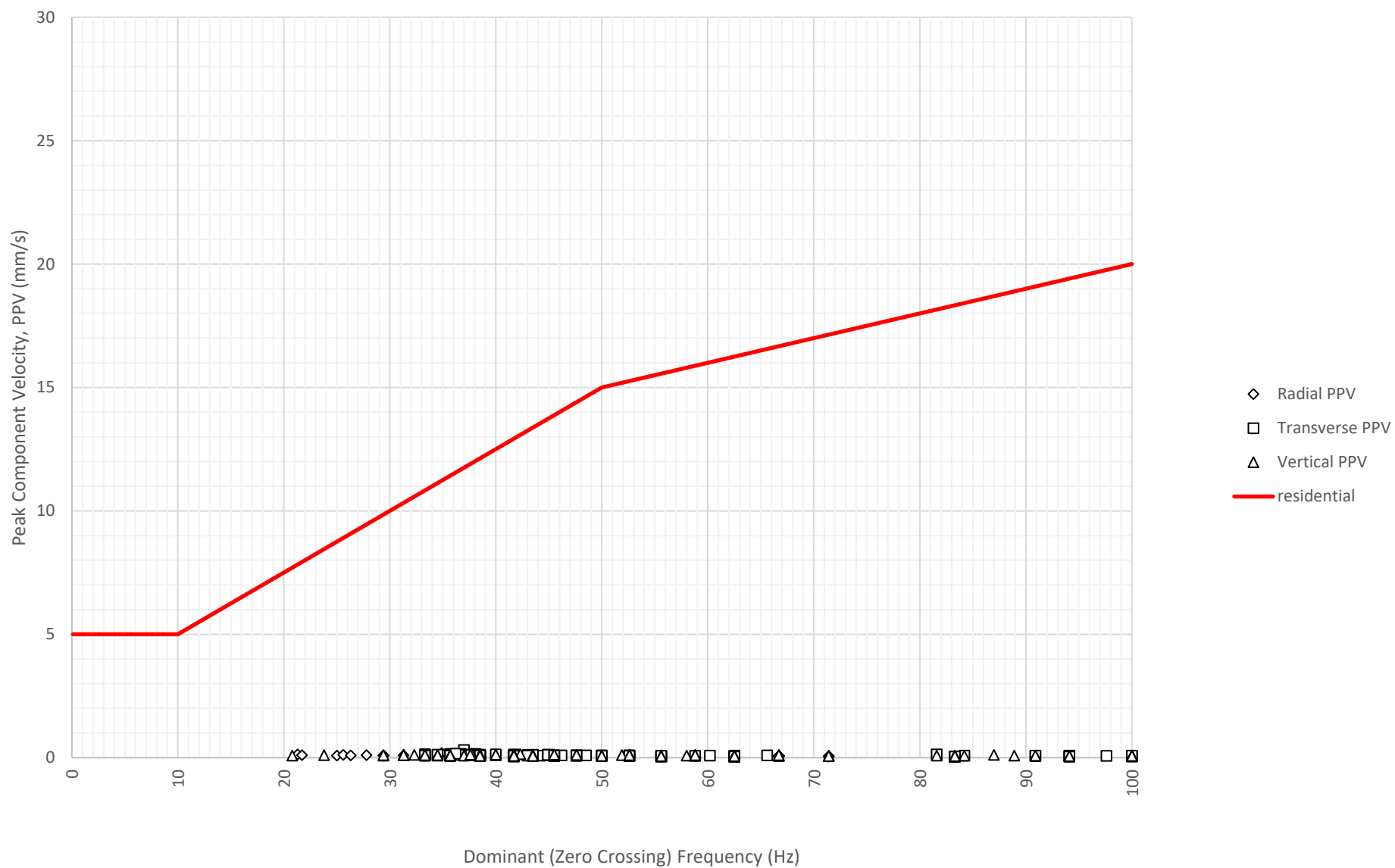
Frequency Content of Vibration Levels at East Boundary Opposite Shoalhaven Street (ETM7326) on 25-06-2024
