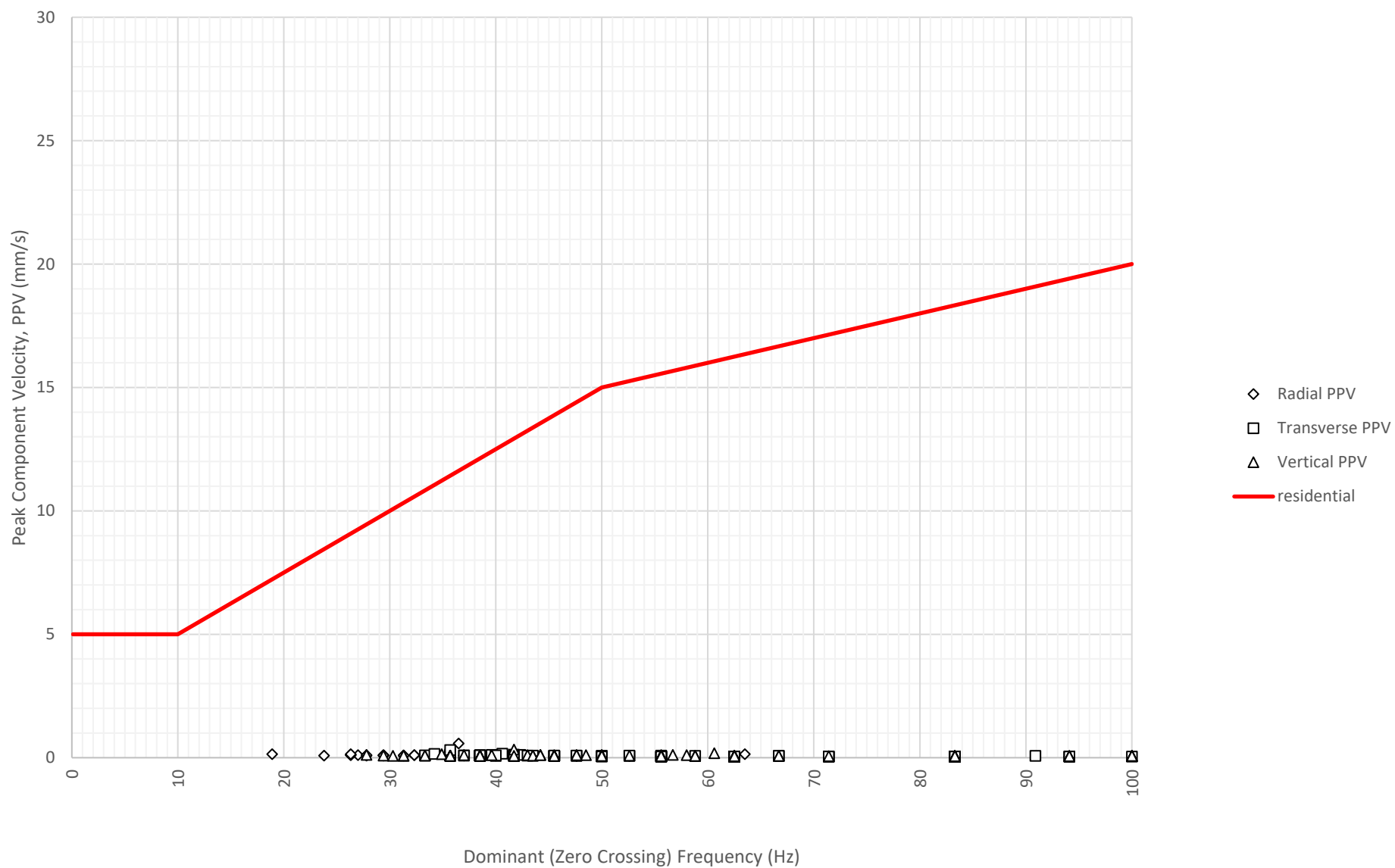
Frequency Content of Vibration Levels at East Boundary Opposite Shoalhaven Street (ETM7326) on 13-06-2024
