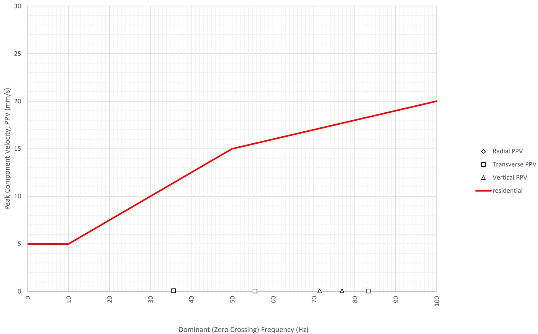
Frequency Content of Vibration Levels at East Boundary Opposite Shoalhaven Street (ETM7326) on 9-06-2024
