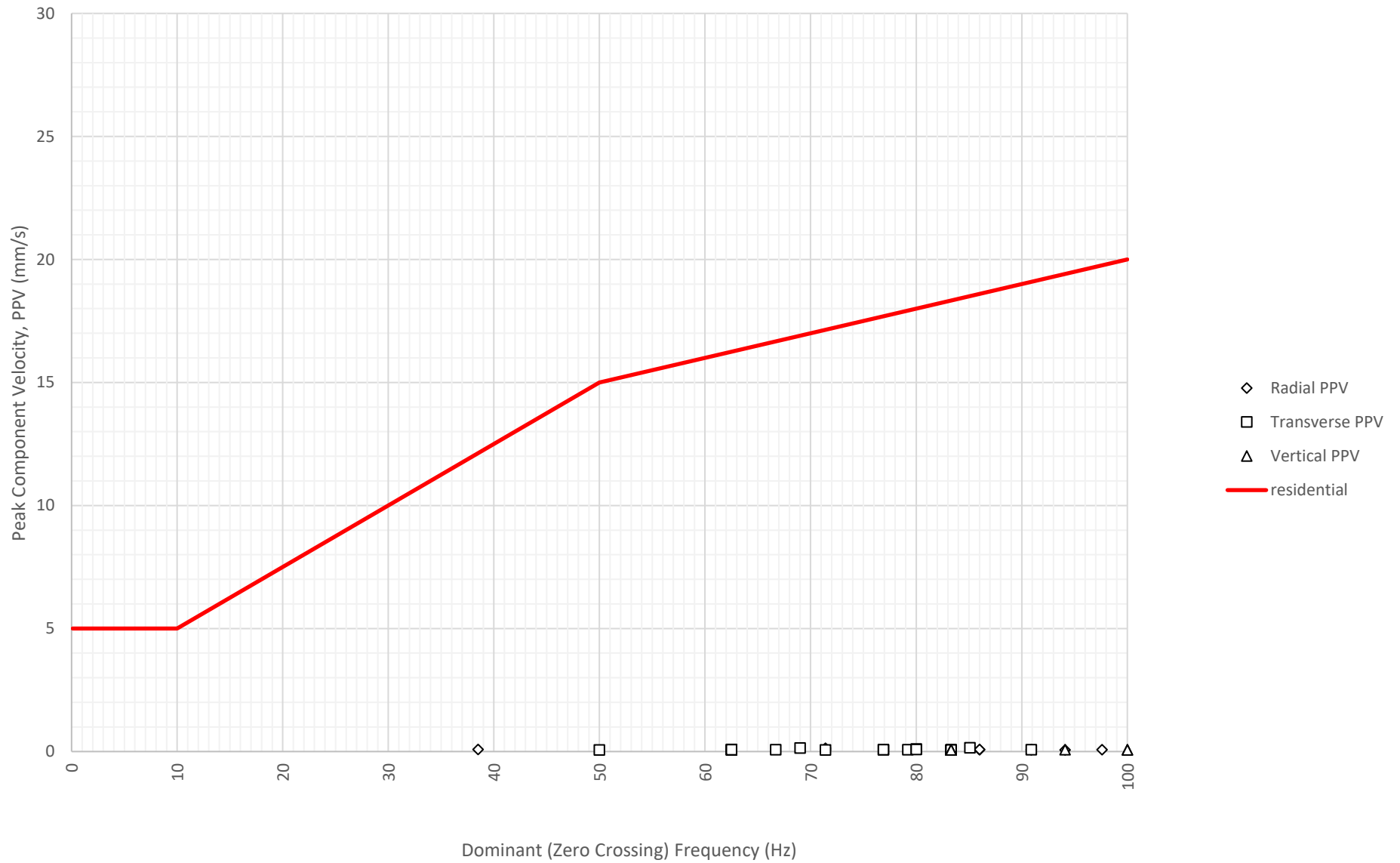
Frequency Content of Vibration Levels at North Boundary Near Block A and B (ETM7687) on 3-06-2024
