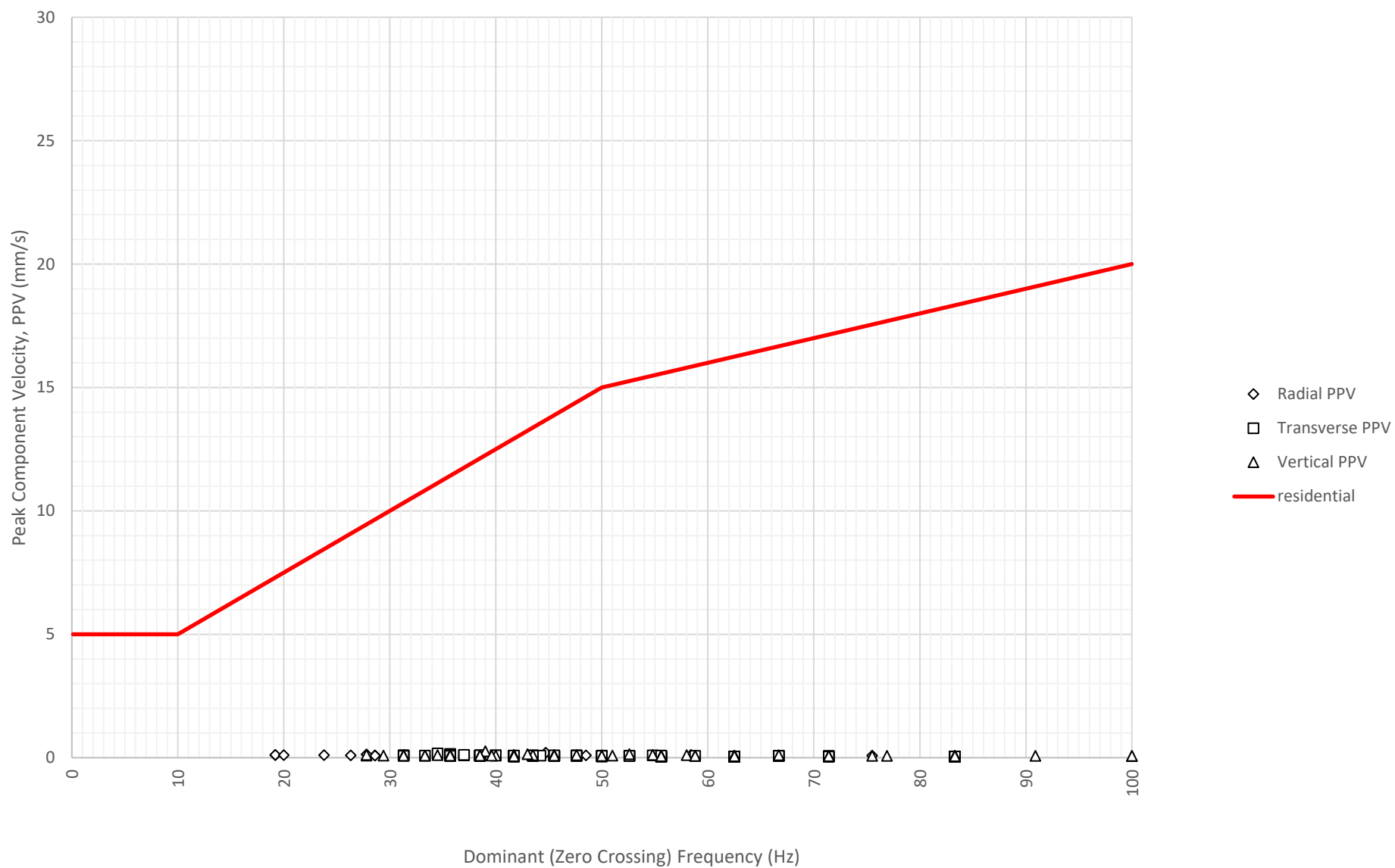
Frequency Content of Vibration Levels at East Boundary Opposite Shoalhaven Street (ETM7326) on 12-06-2024
