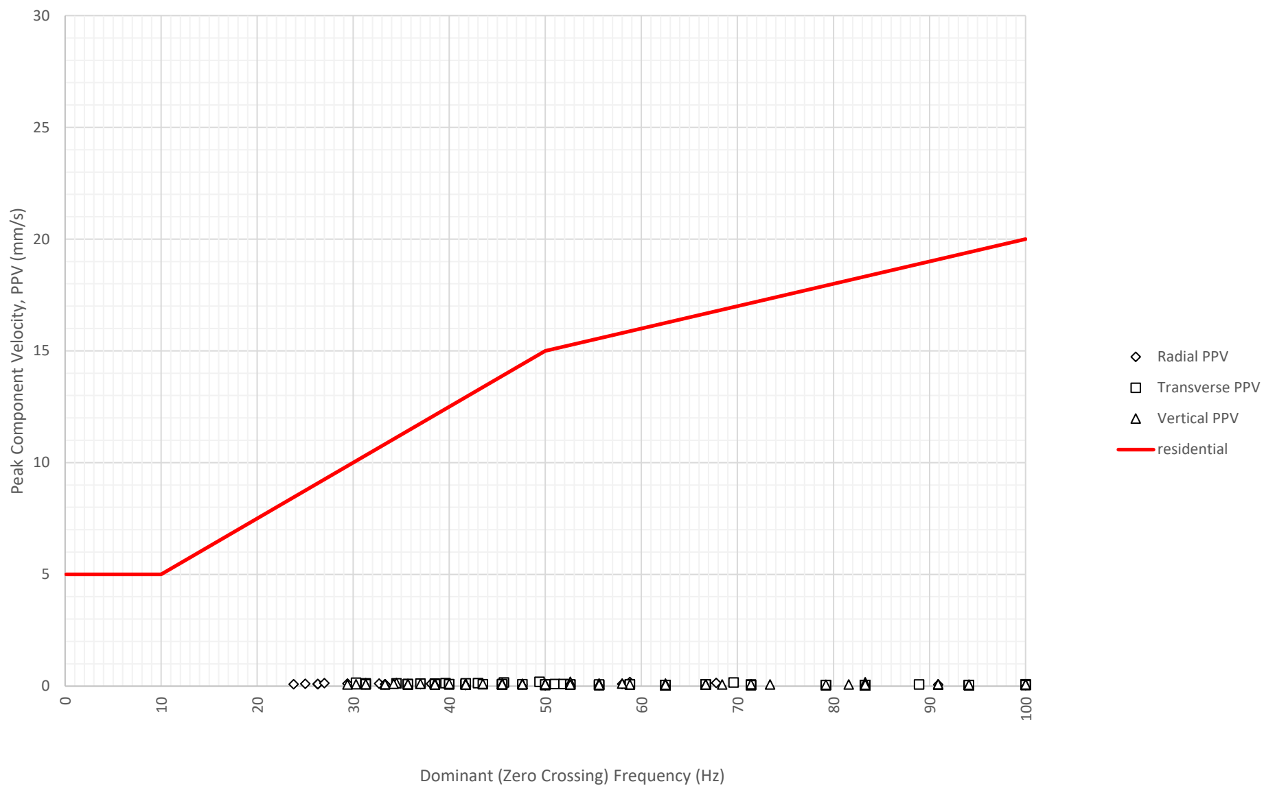
Frequency Content of Vibration Levels at East Boundary Opposite Shoalhaven Street (ETM7326) on 14-06-2024
