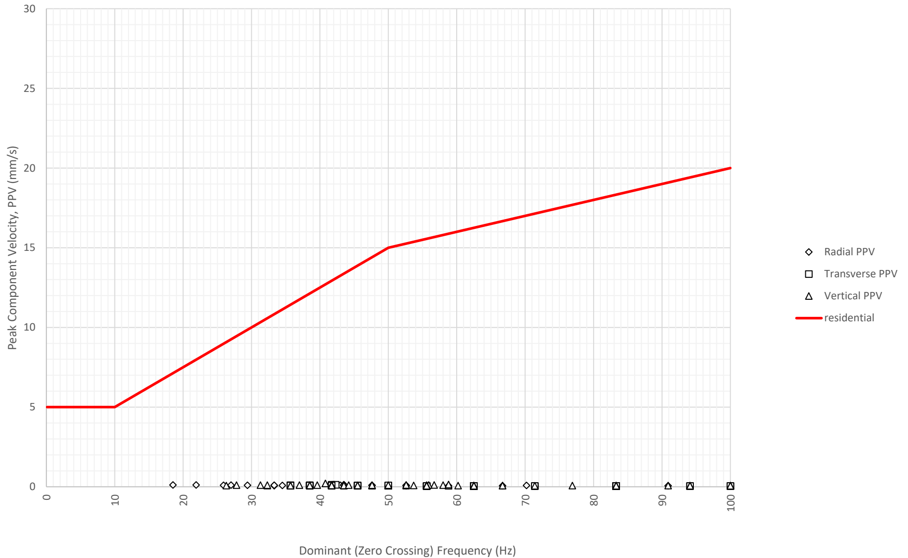
Frequency Content of Vibration Levels at East Boundary Opposite Shoalhaven Street (ETM7326) on 4-06-2024
