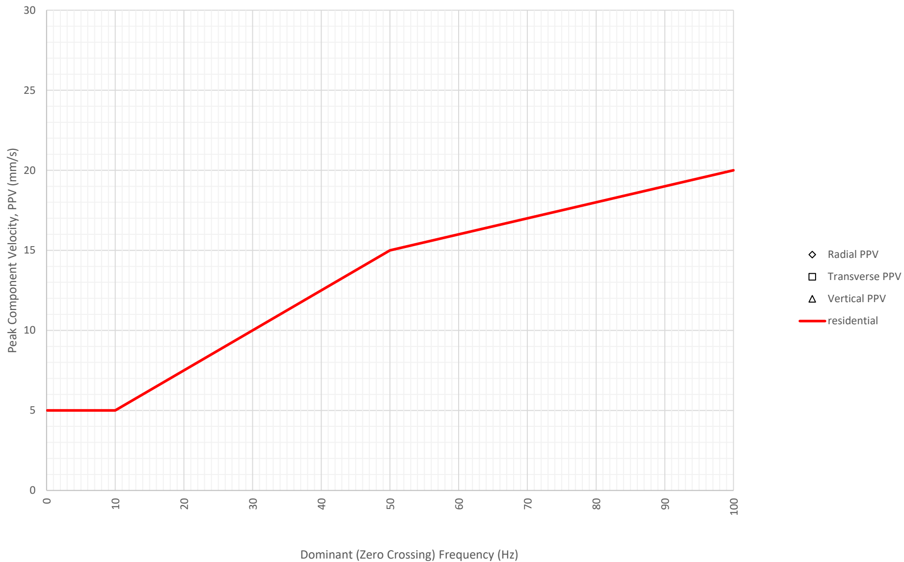
Frequency Content of Vibration Levels at North Boundary Near Block A and B (ETM7687) on 15-09-2024
