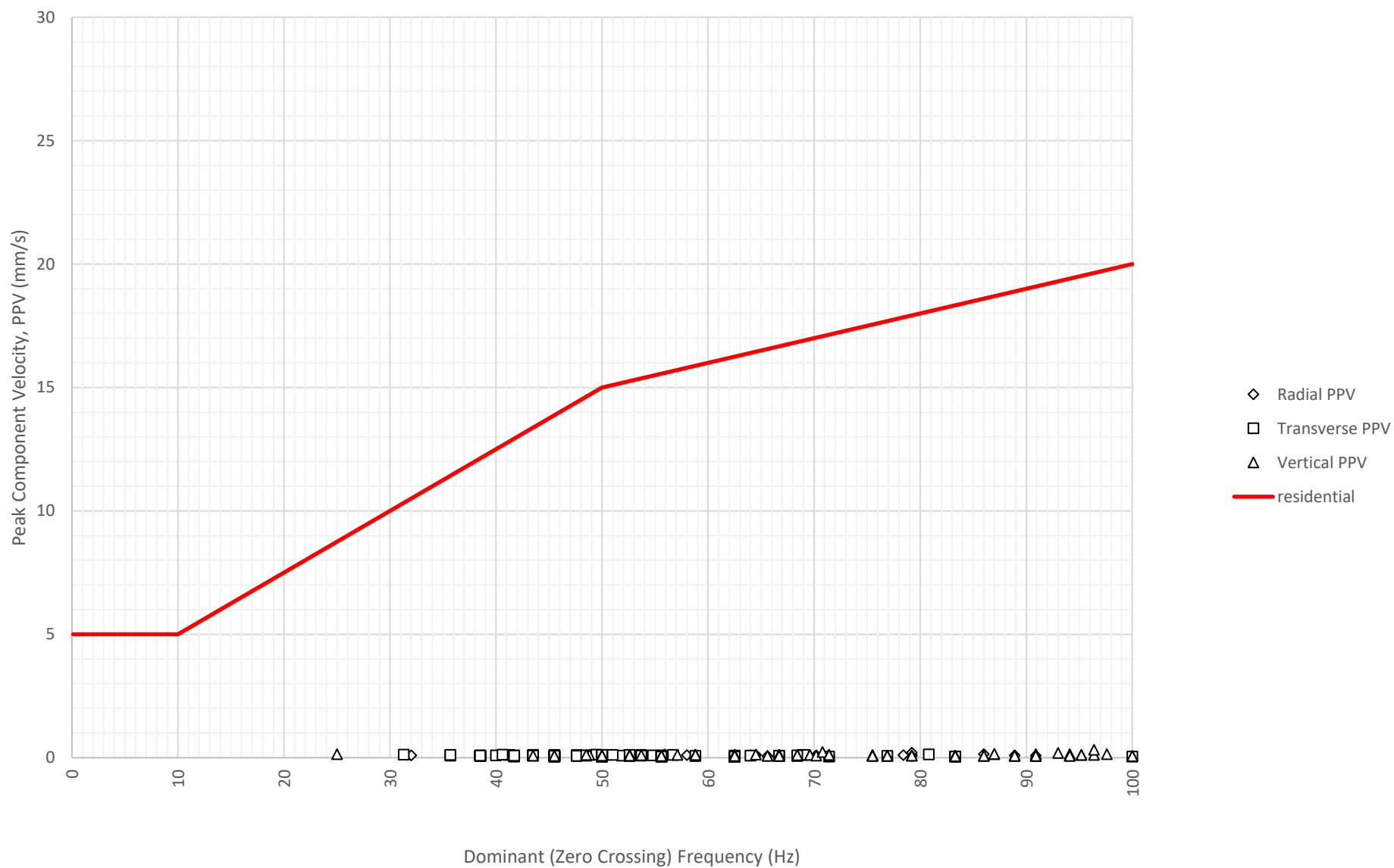
Frequency Content of Vibration Levels at East Boundary Opposite Shoalhaven Street (ETM7326) on 23-09-2024
