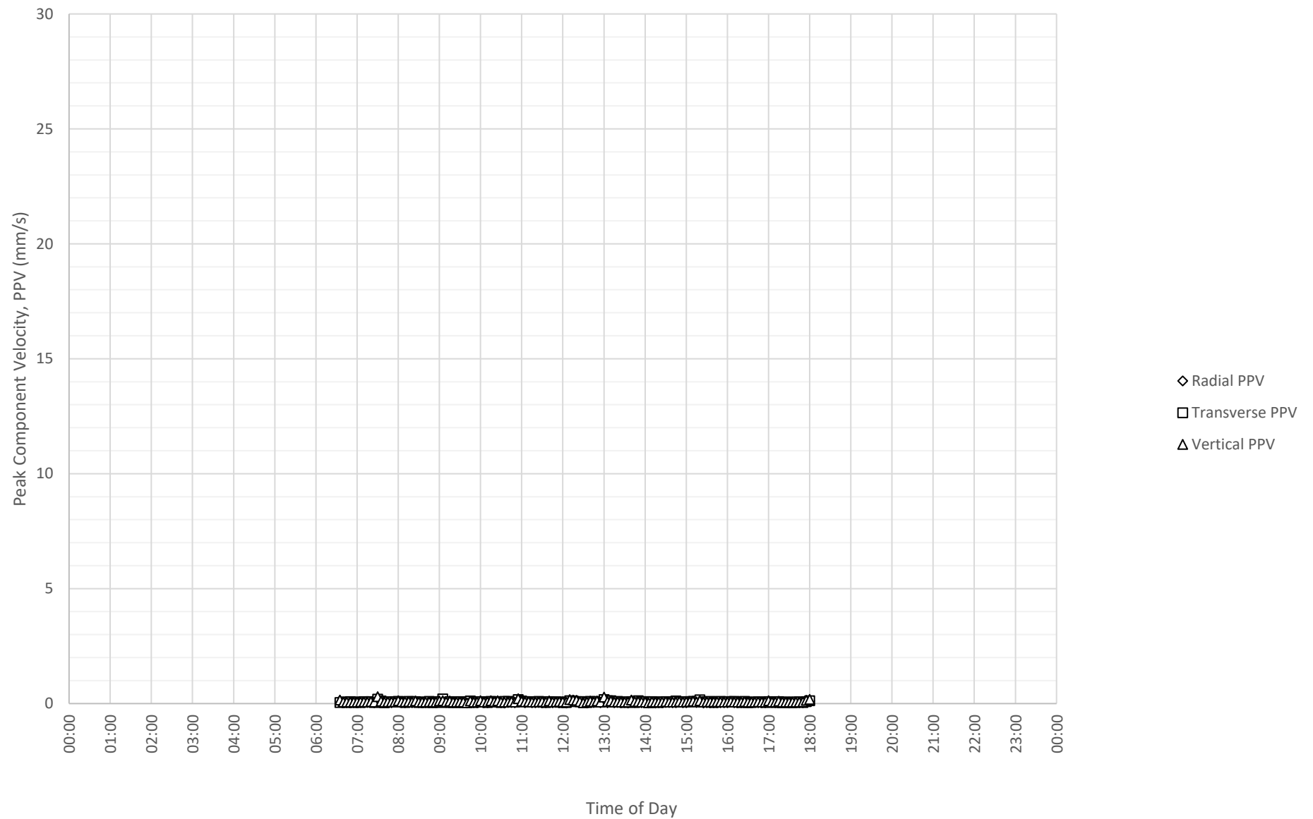
Daily Monitored Vibration Levels at East Boundary Opposite Shoalhaven Street (ETM7326) on 12-09-2024
