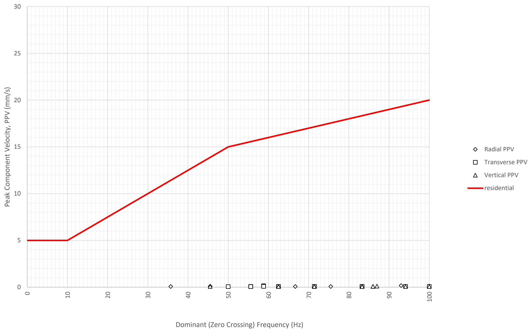
Frequency Content of Vibration Levels at North Boundary Near Block A and B (ETM7687) on 13-09-2024
