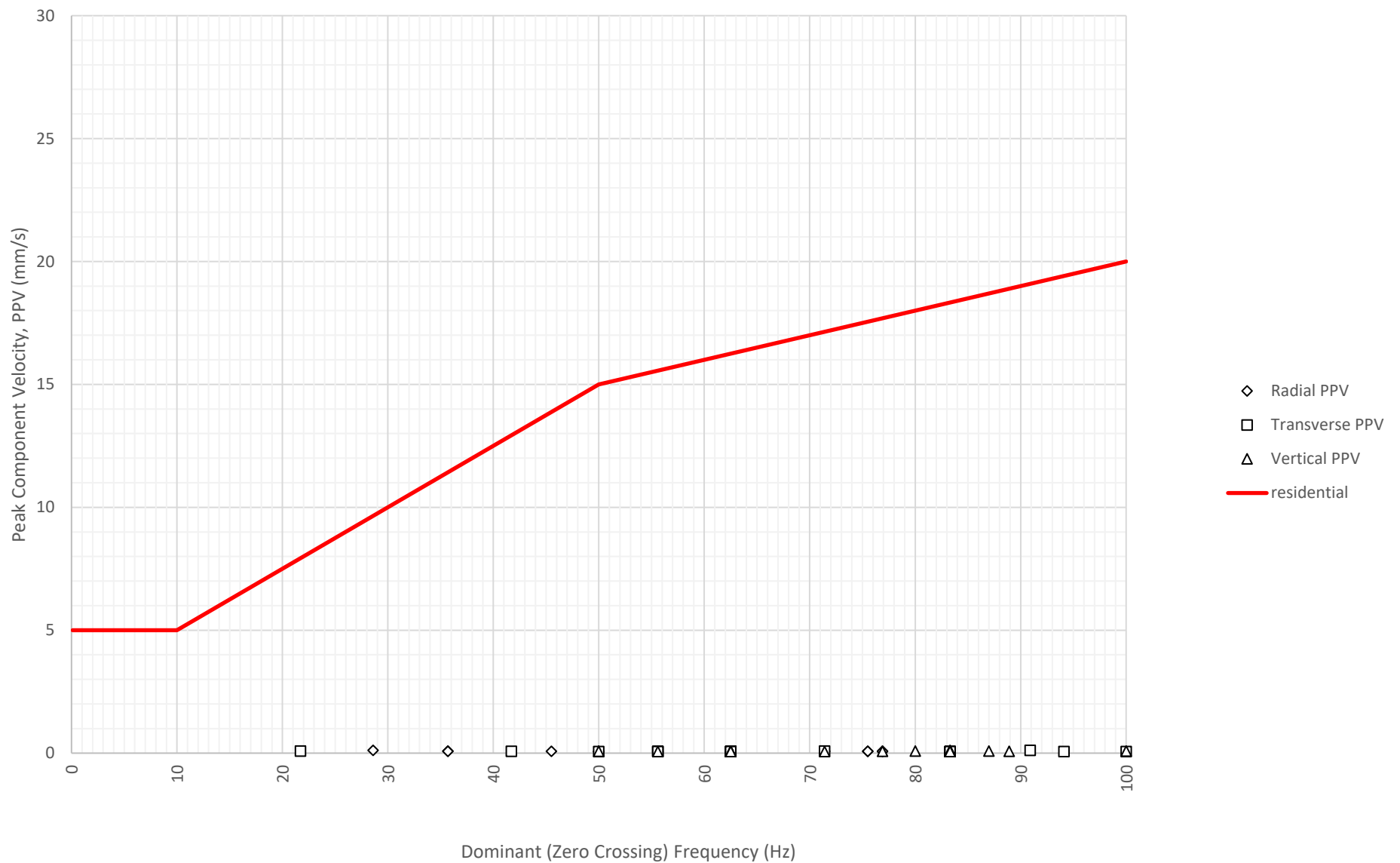
Frequency Content of Vibration Levels at North Boundary Near Block A and B (ETM7687) on 2-09-2024
