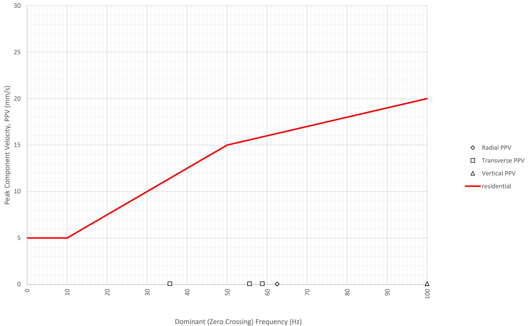
Frequency Content of Vibration Levels at East Boundary Opposite Shoalhaven Street (ETM7326) on 15-09-2024
