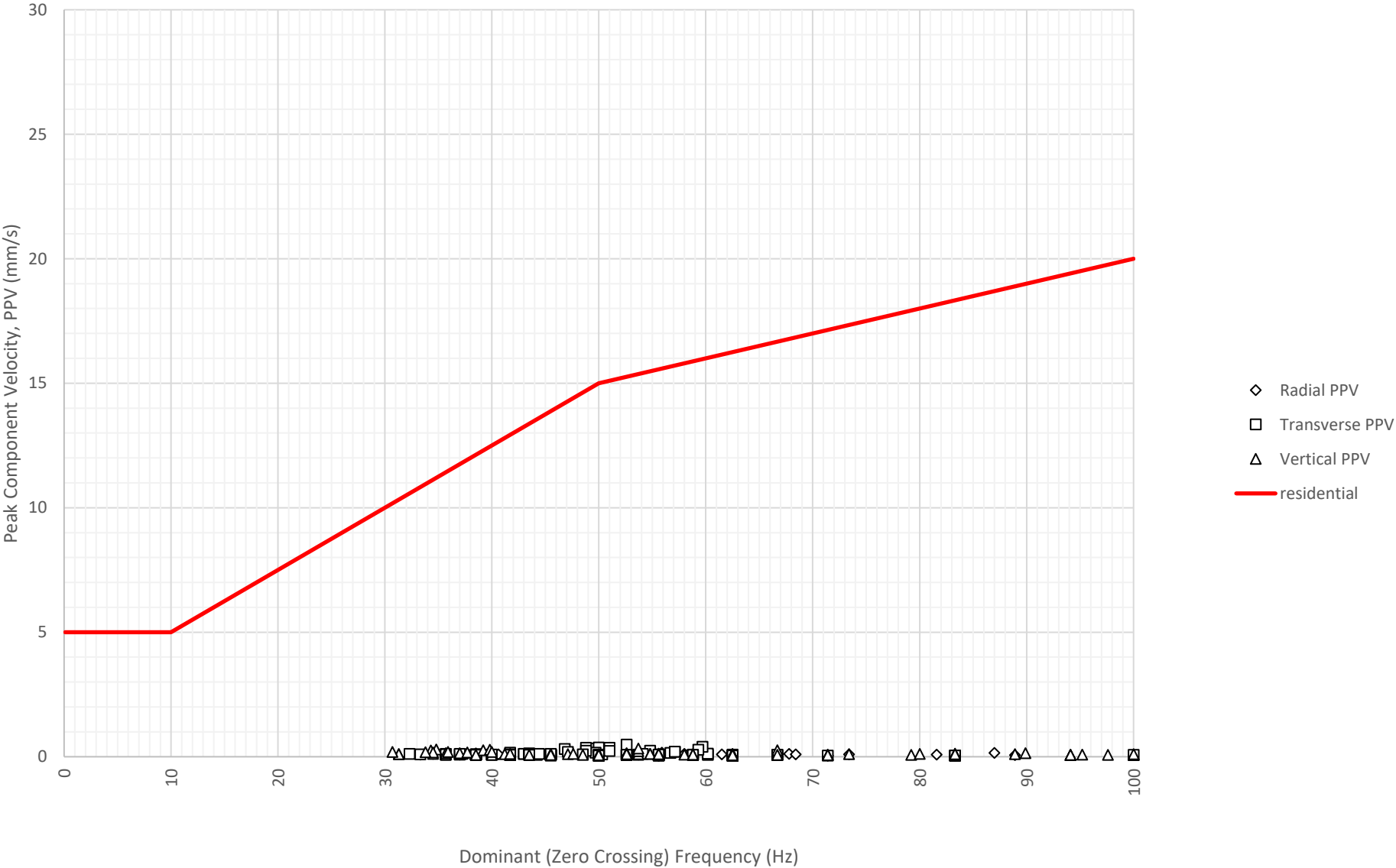
Frequency Content of Vibration Levels at East Boundary Opposite Shoalhaven Street (ETM7326) on 5-09-2024
