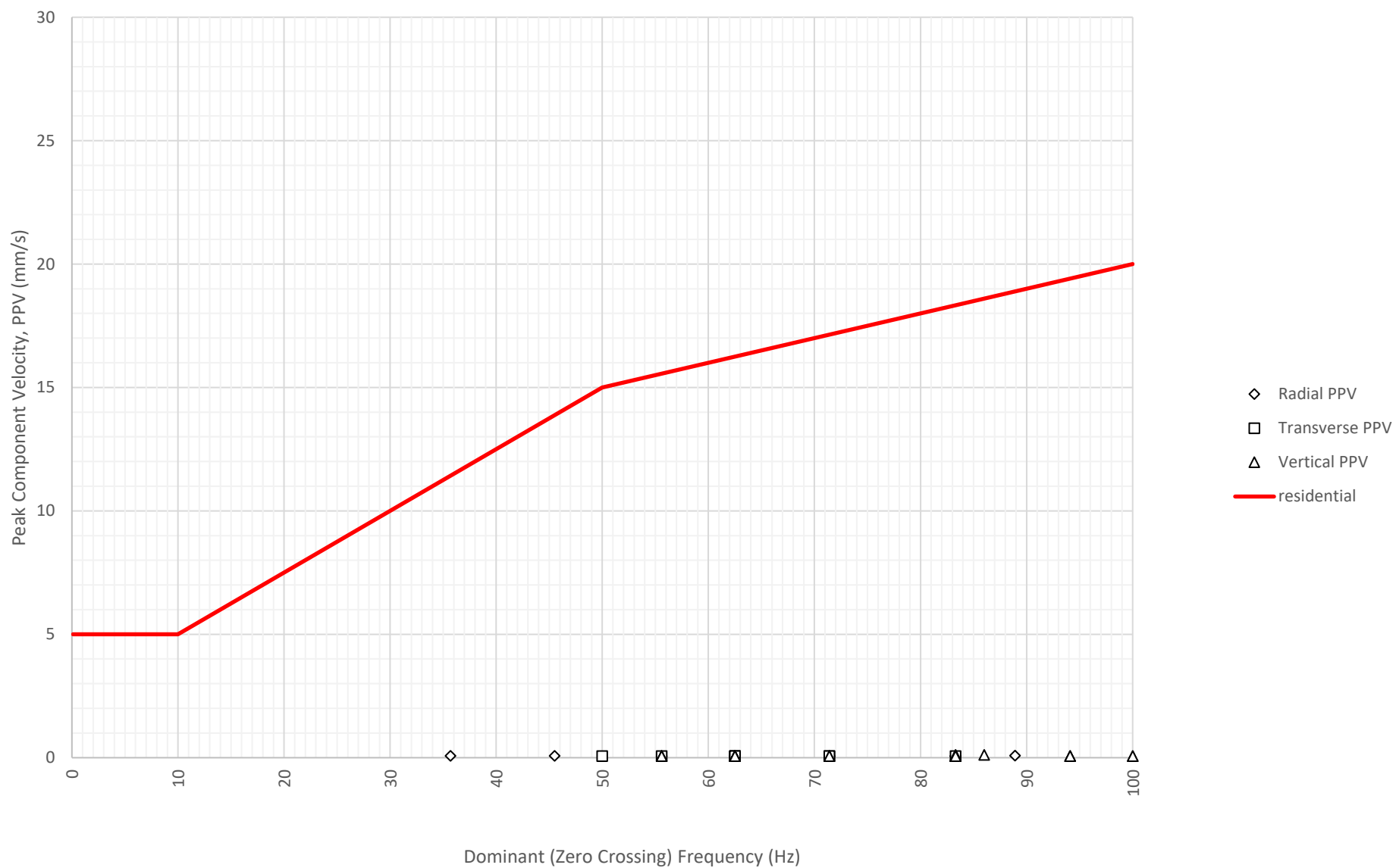
Frequency Content of Vibration Levels at North Boundary Near Block A and B (ETM7687) on 23-09-2024
