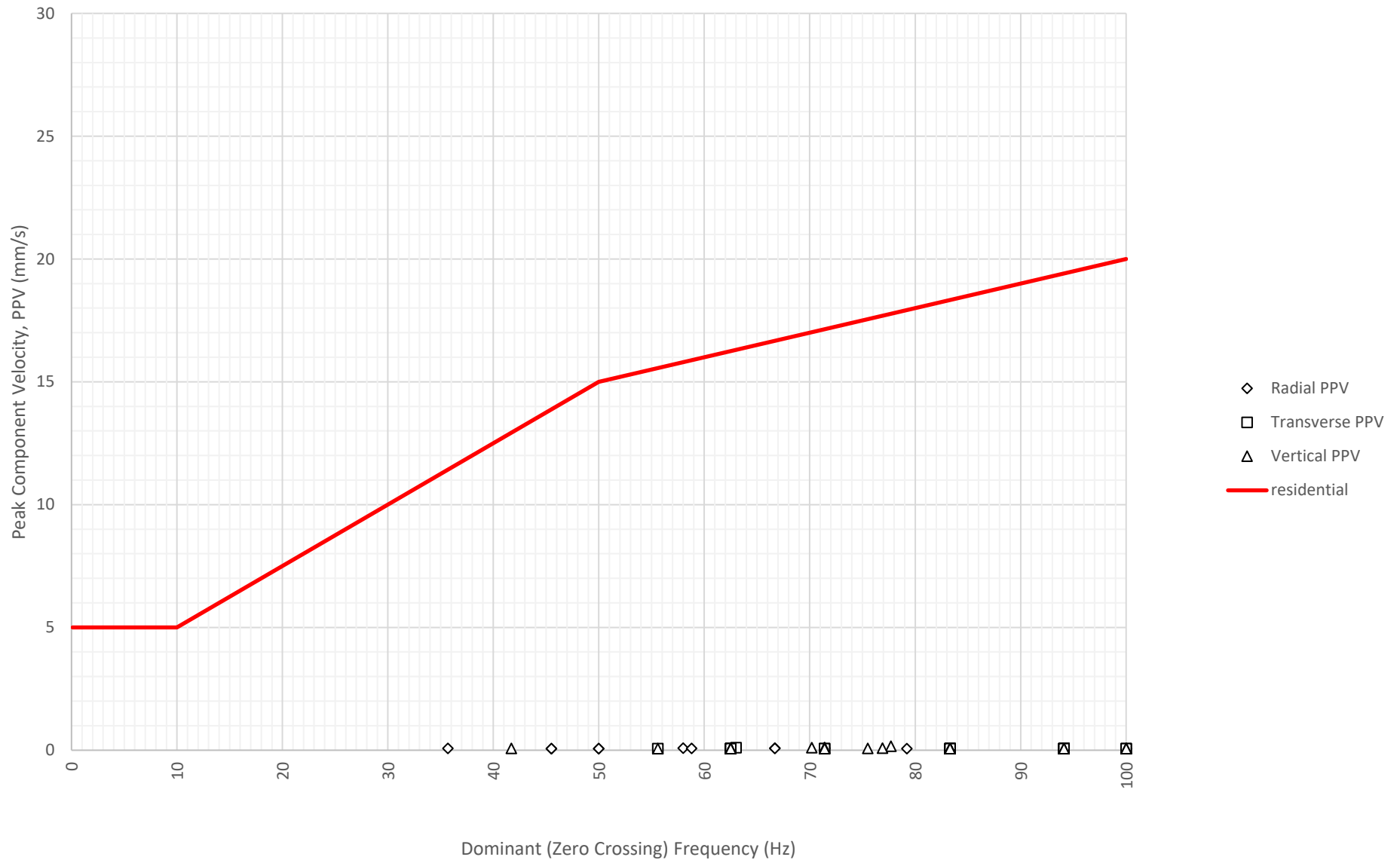
Frequency Content of Vibration Levels at North Boundary Near Block A and B (ETM7687) on 6-09-2024
