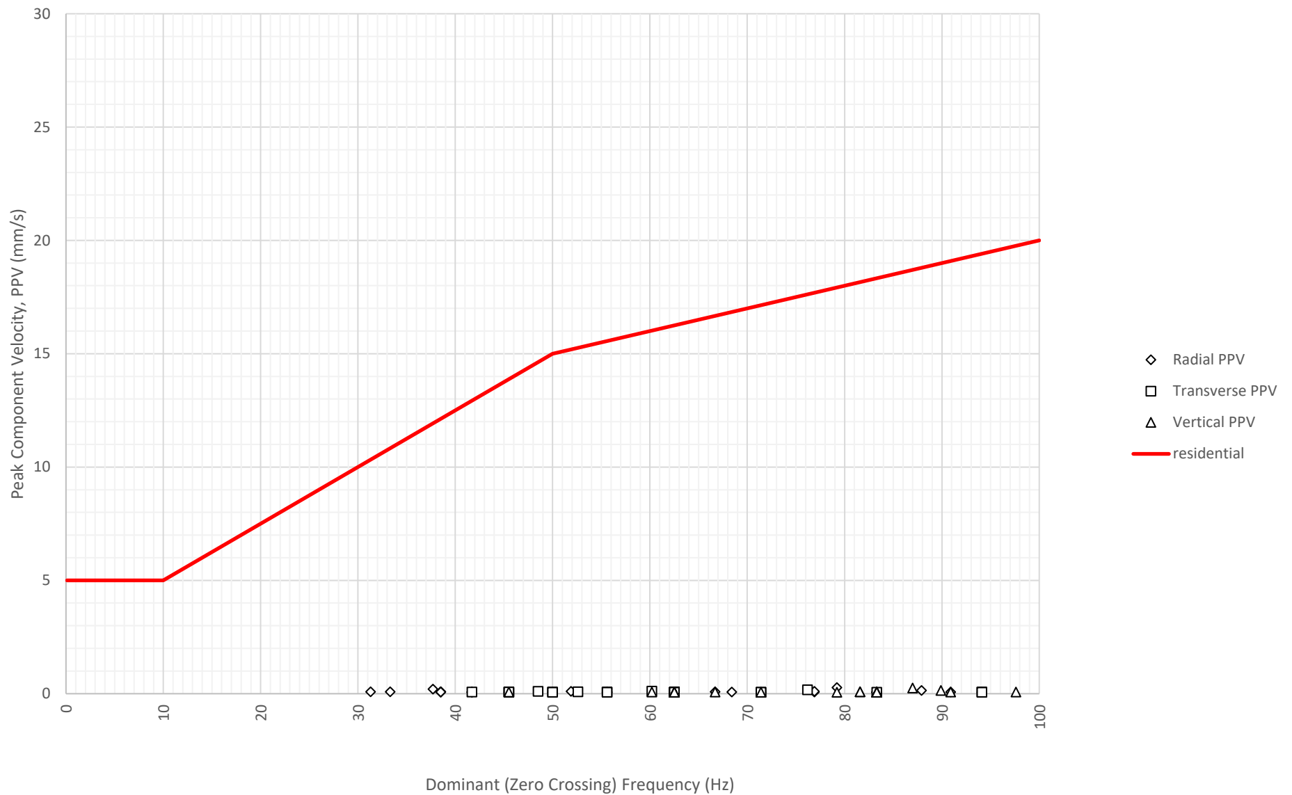
Frequency Content of Vibration Levels at North Boundary Near Block A and B (ETM7687) on 3-09-2024
