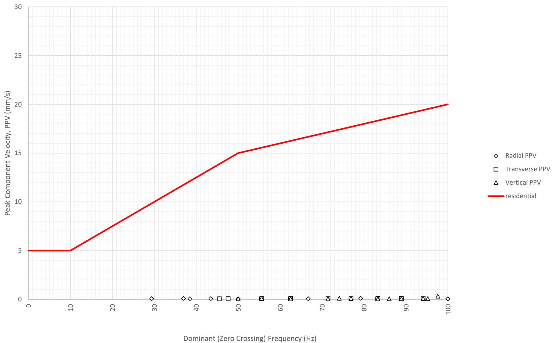
Frequency Content of Vibration Levels at North Boundary Near Block A and B (ETM7687) on 19-09-2024
