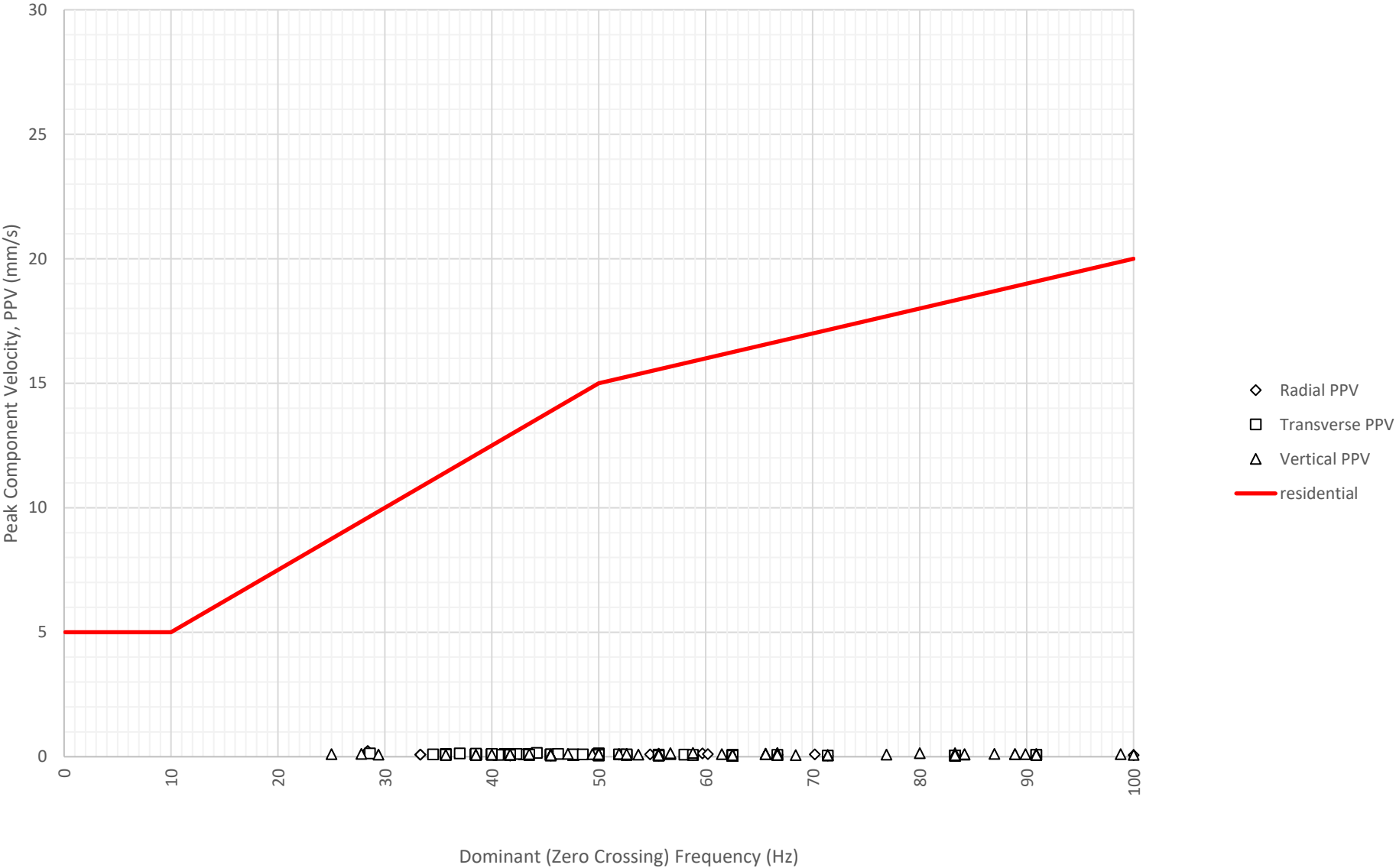
Frequency Content of Vibration Levels at East Boundary Opposite Shoalhaven Street (ETM7326) on 2-09-2024
