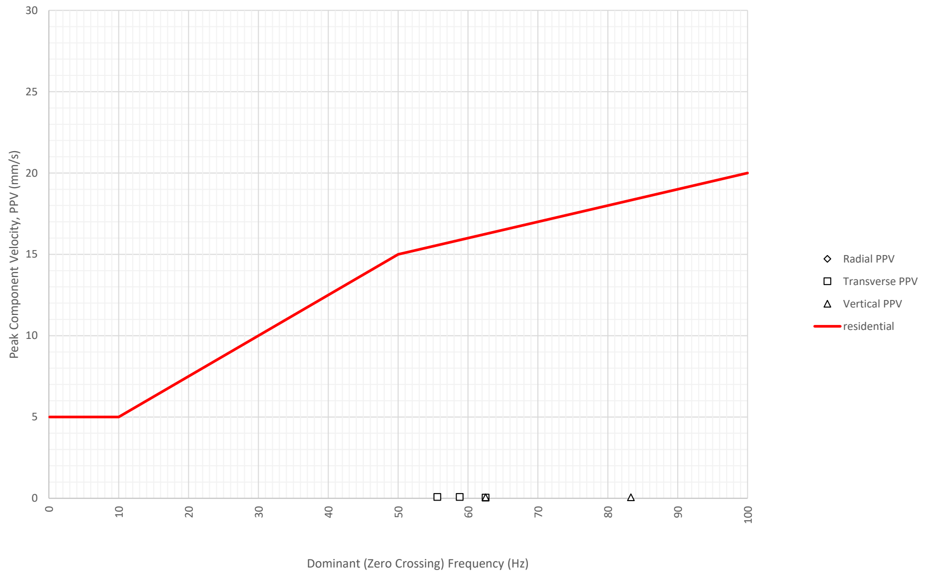
Frequency Content of Vibration Levels at East Boundary Opposite Shoalhaven Street (ETM7326) on 22-09-2024
