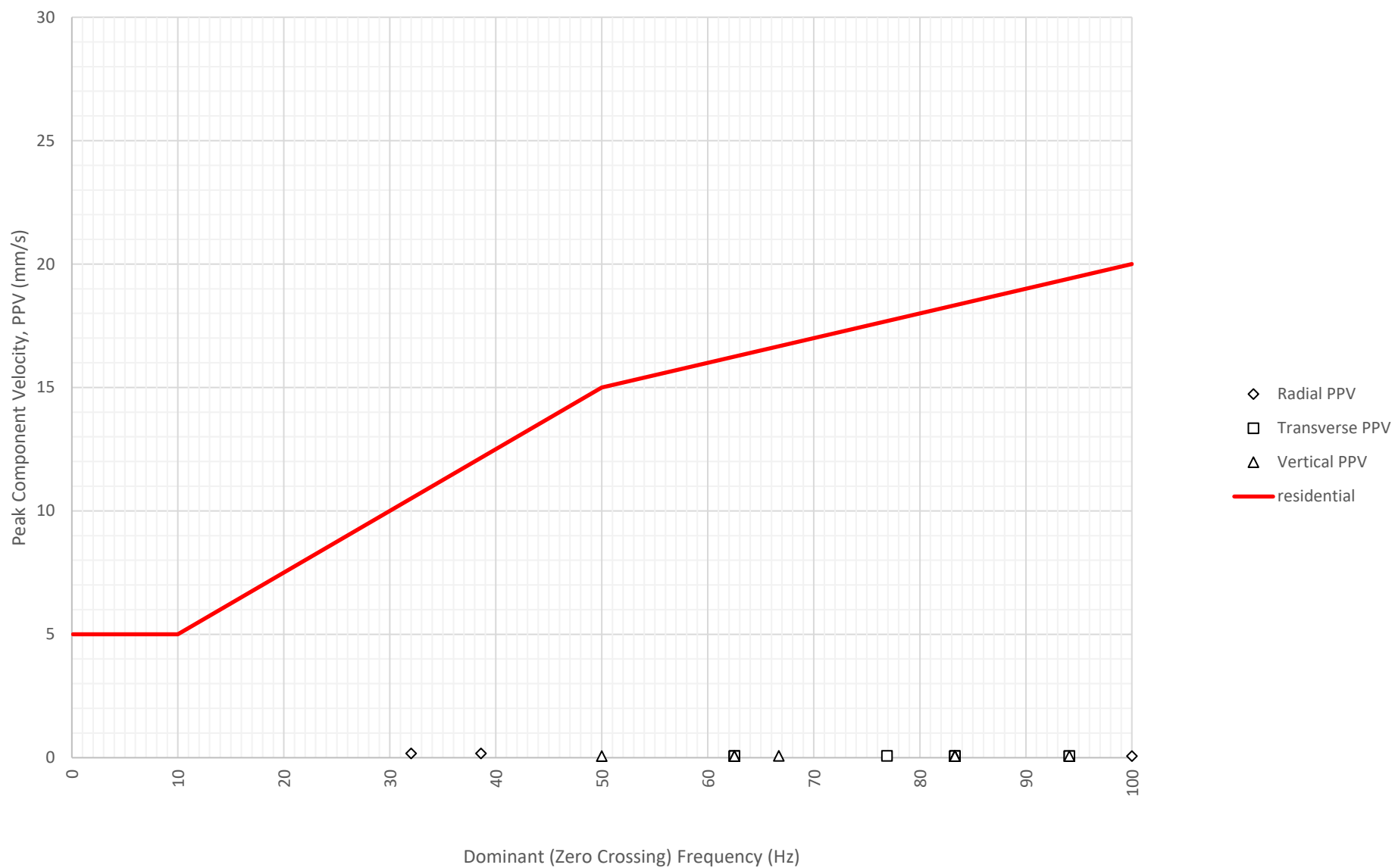
Frequency Content of Vibration Levels at North Boundary Near Block A and B (ETM7687) on 14-09-2024
