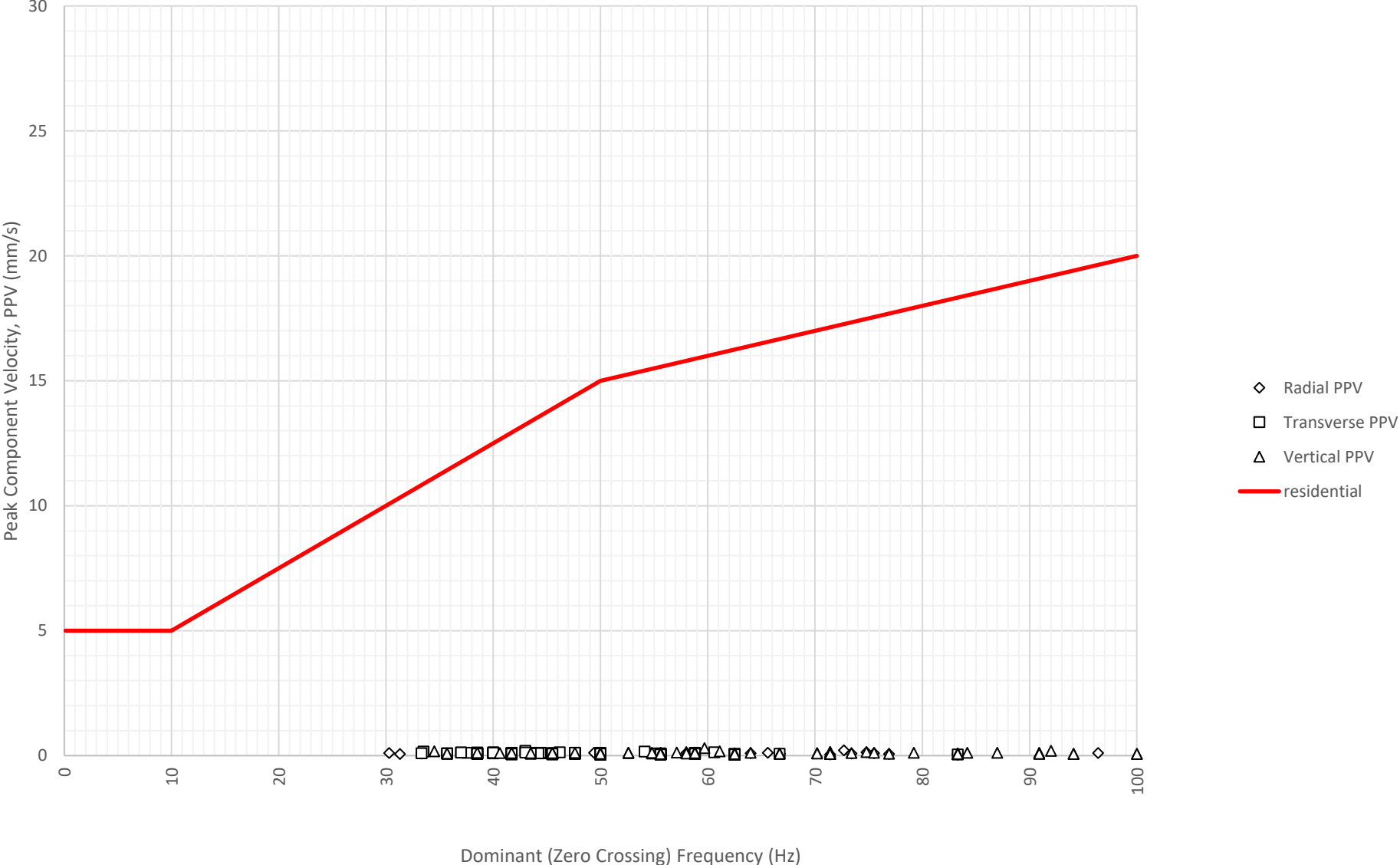
Frequency Content of Vibration Levels at East Boundary Opposite Shoalhaven Street (ETM7326) on 9-09-2024
