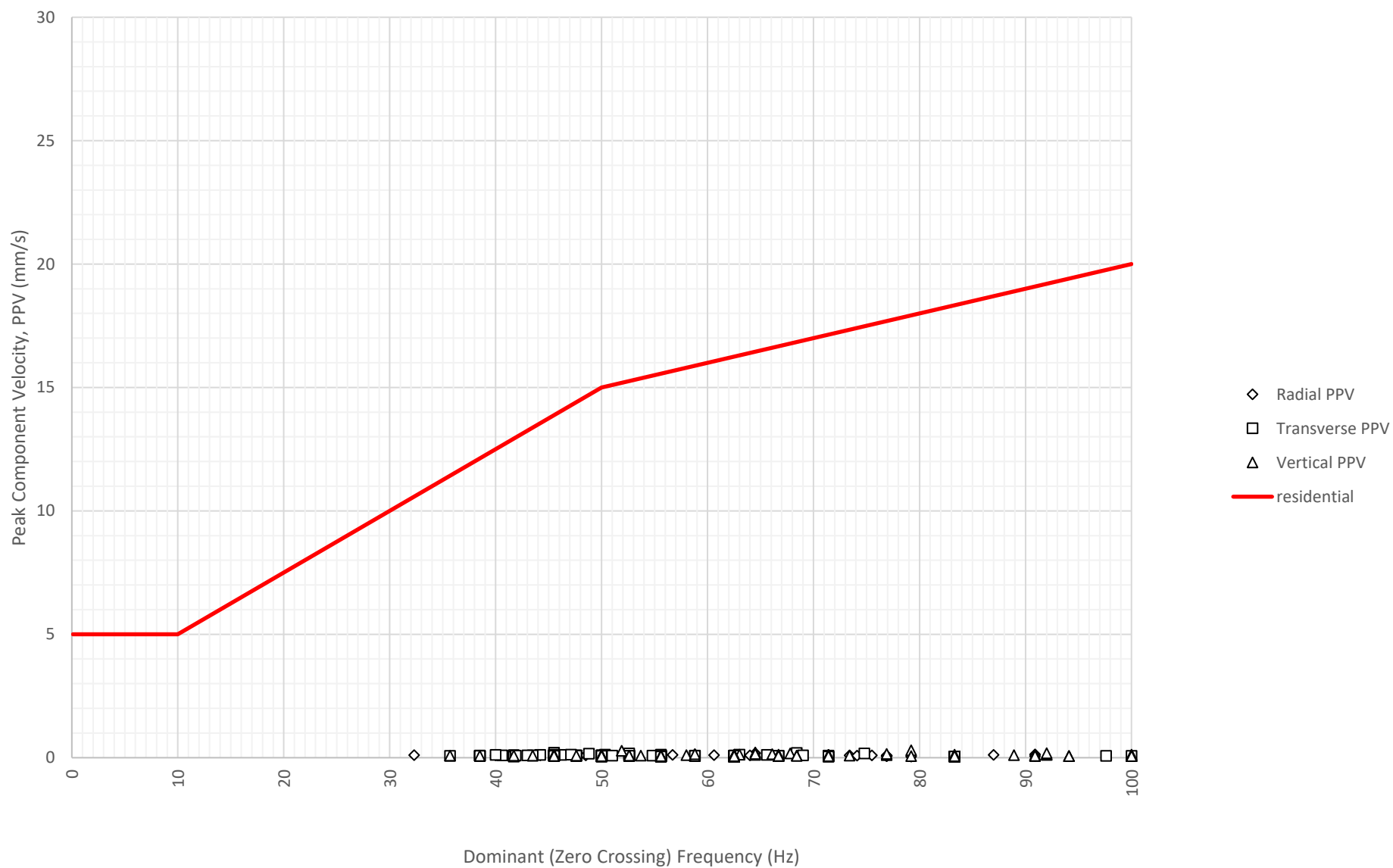
Frequency Content of Vibration Levels at East Boundary Opposite Shoalhaven Street (ETM7326) on 12-09-2024
