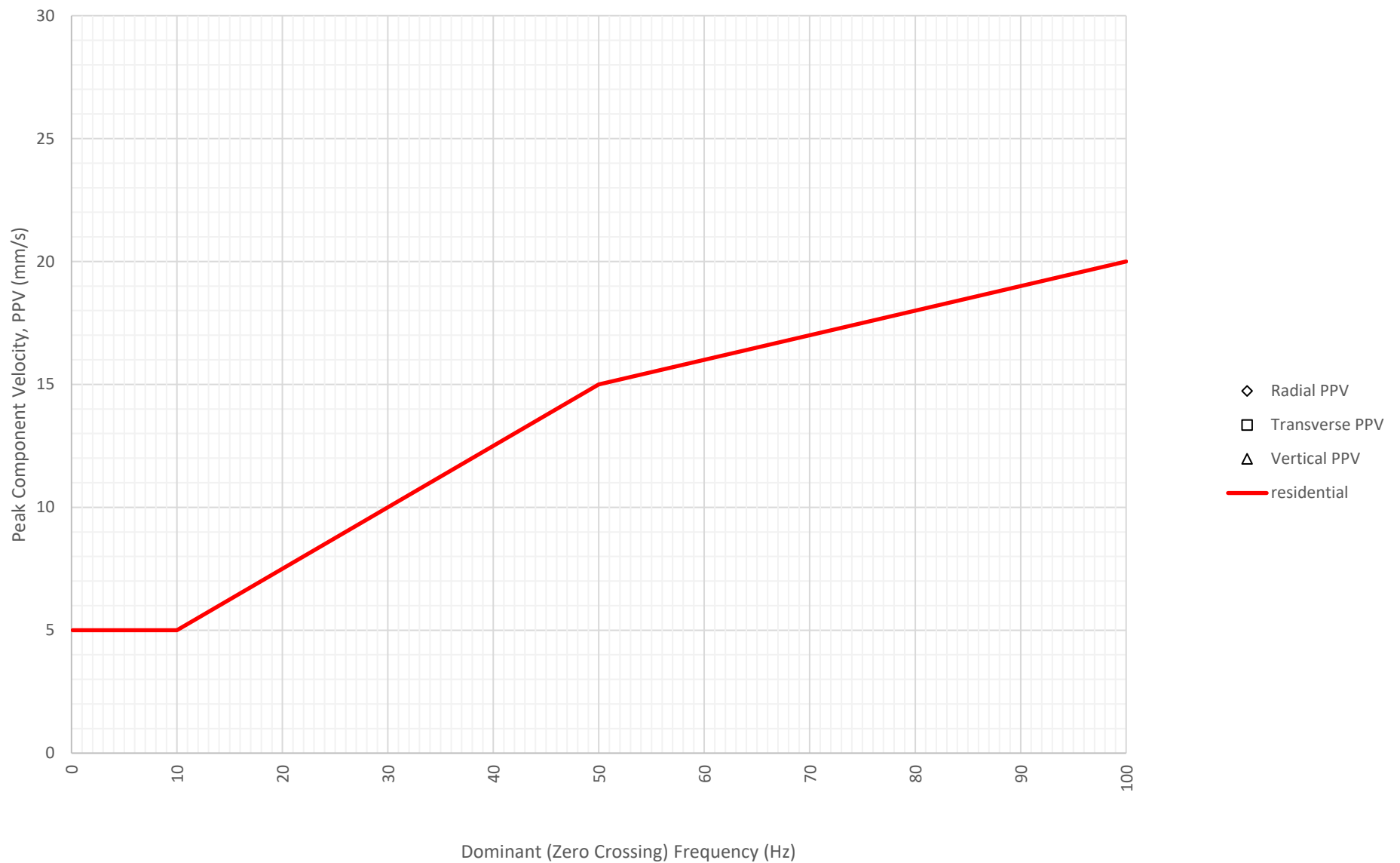
Frequency Content of Vibration Levels at North Boundary Near Block A and B (ETM7687) on 29-09-2024
