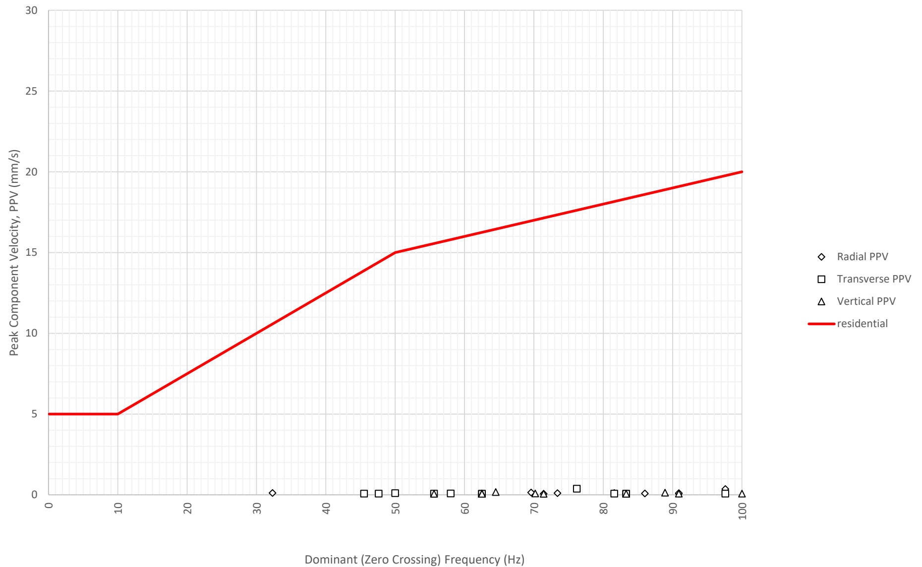
Frequency Content of Vibration Levels at North Boundary Near Block A and B (ETM7687) on 25-09-2024
