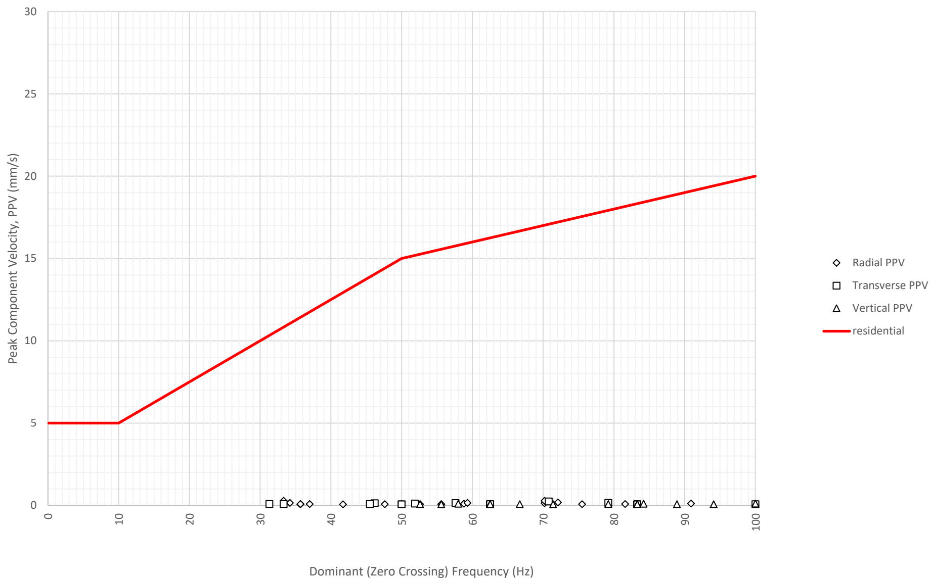
Frequency Content of Vibration Levels at North Boundary Near Block A and B (ETM7687) on 12-09-2024
