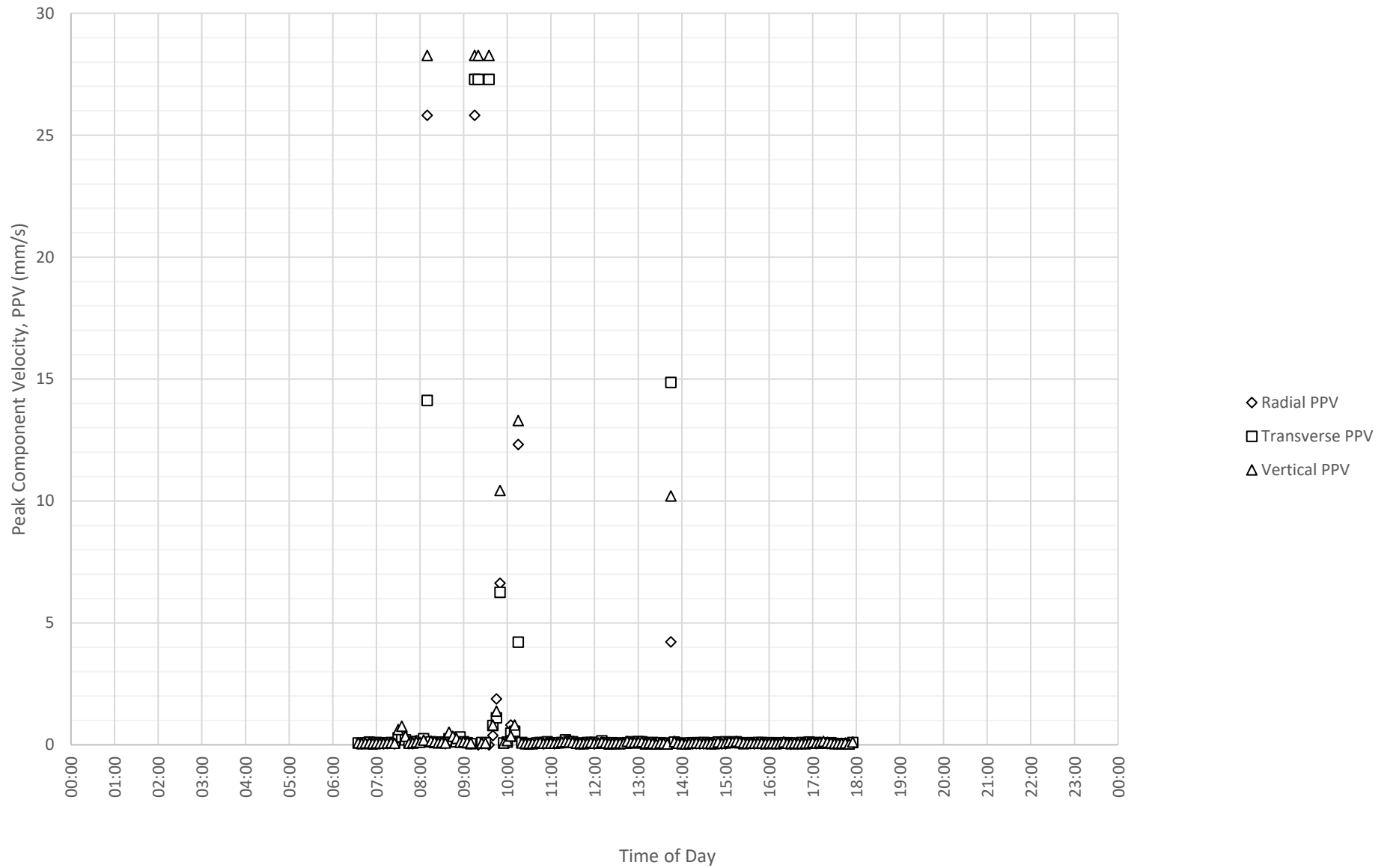
Daily Monitored Vibration Levels at East Boundary Opposite Shoalhaven Street (ETM7326) on 13-09-2024
