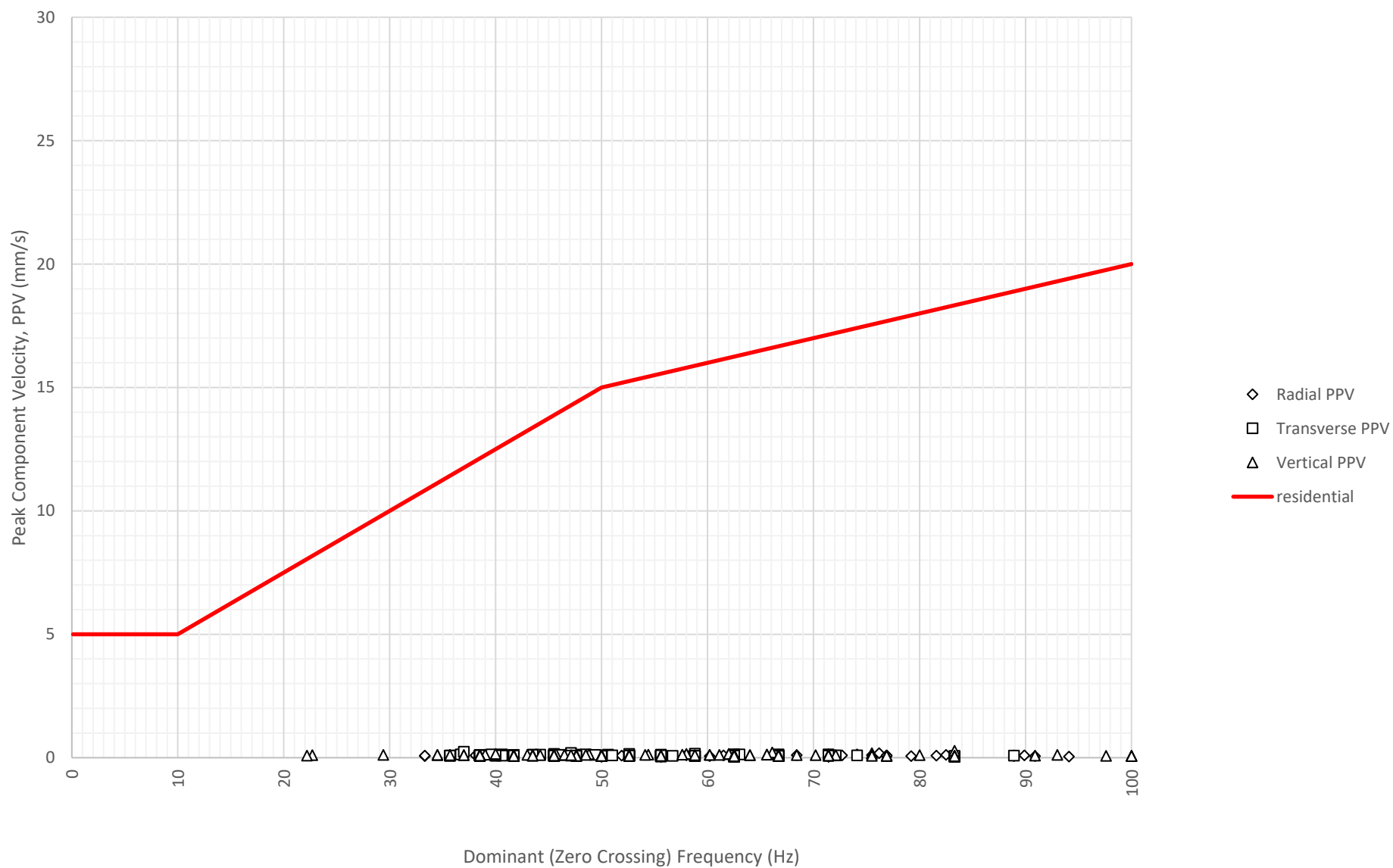
Frequency Content of Vibration Levels at East Boundary Opposite Shoalhaven Street (ETM7326) on 16-09-2024
