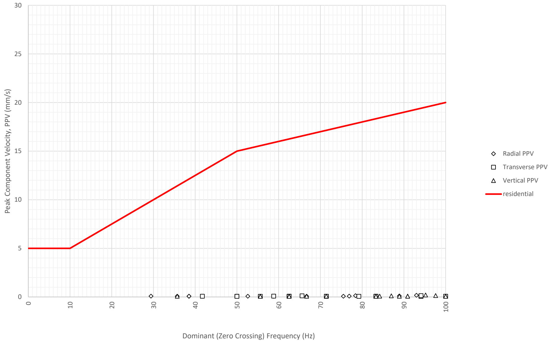
Frequency Content of Vibration Levels at North Boundary Near Block A and B (ETM7687) on 4-09-2024
