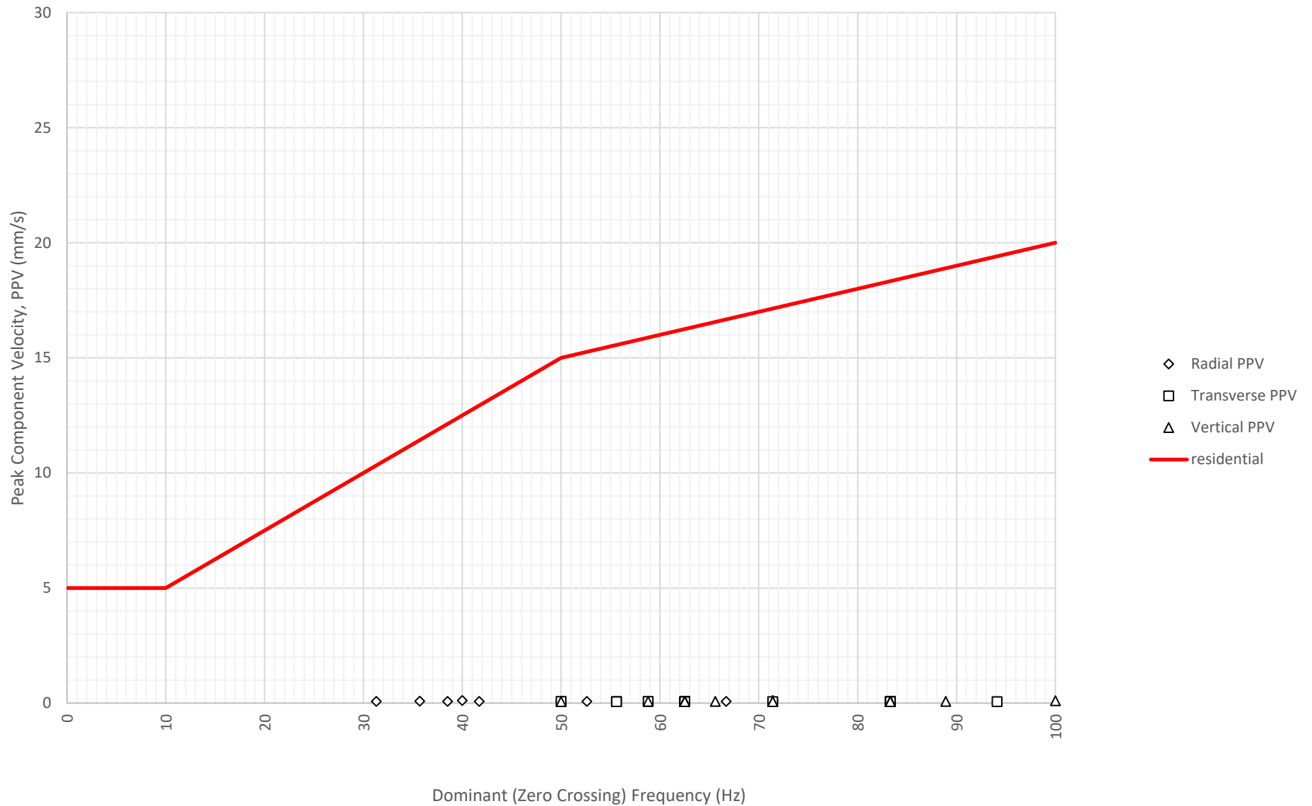
Frequency Content of Vibration Levels at North Boundary Near Block A and B (ETM7687) on 9-09-2024
