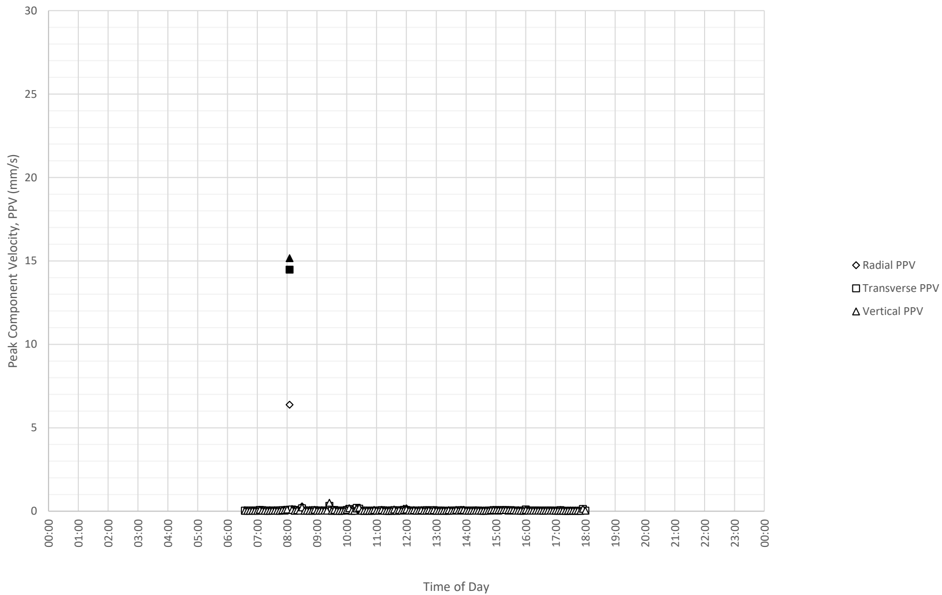
Daily Monitored Vibration Levels at North Boundary Near Block A and B (ETM7687) on 5-09-2024
