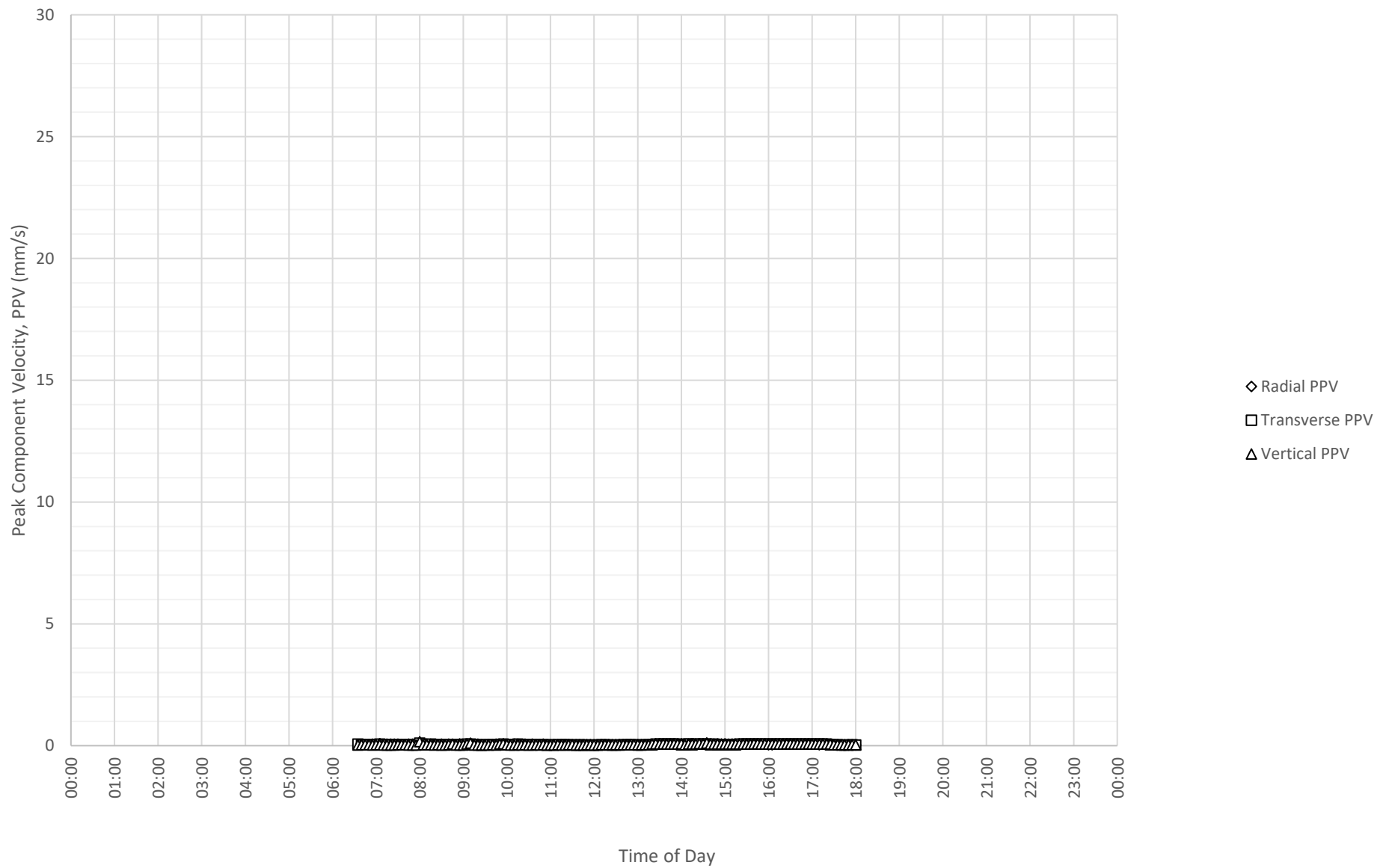
Daily Monitored Vibration Levels at North Boundary Near Block A and B (ETM7687) on 6-09-2024
