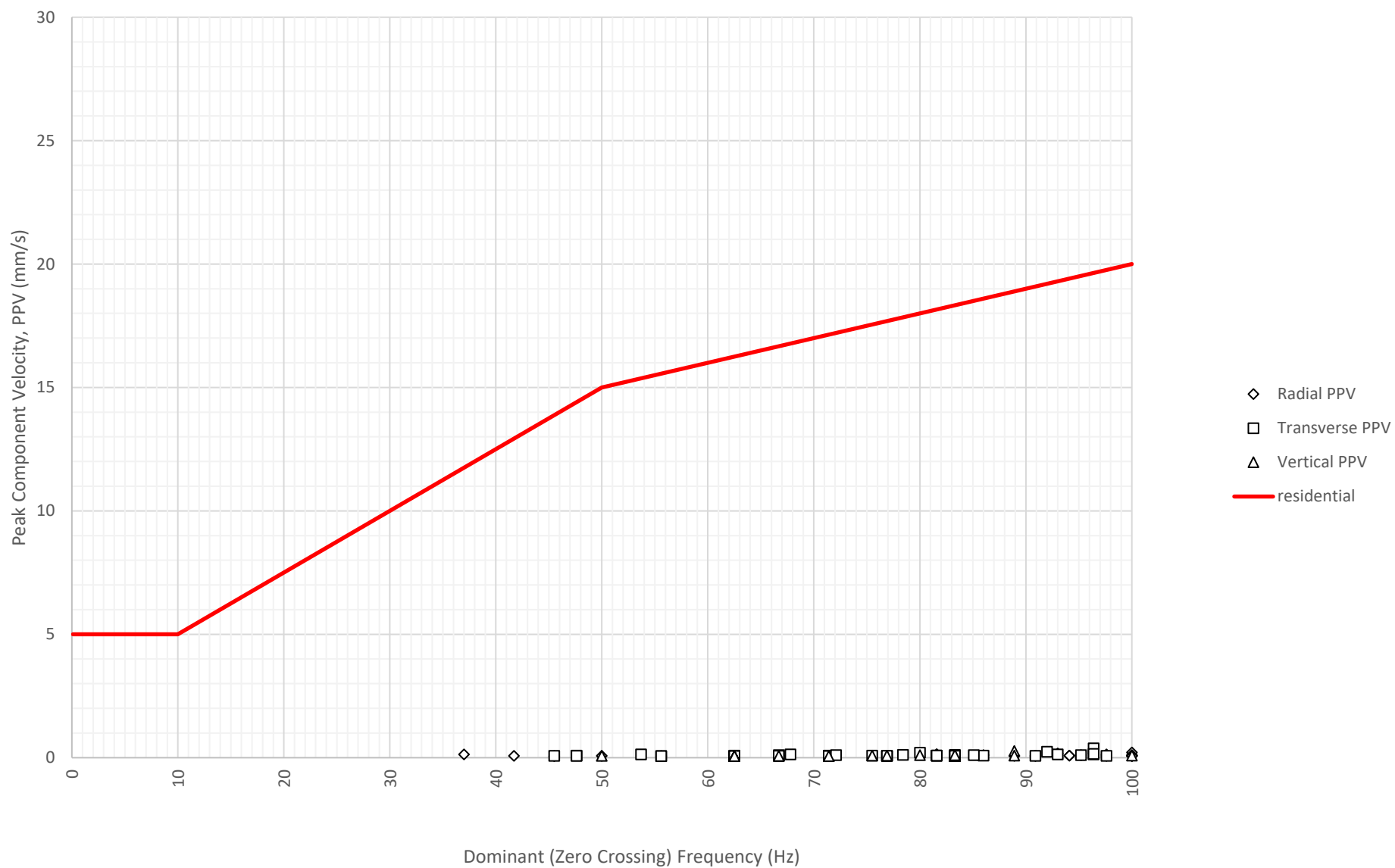
Frequency Content of Vibration Levels at North Boundary Near Block A and B (ETM7687) on 27-09-2024
