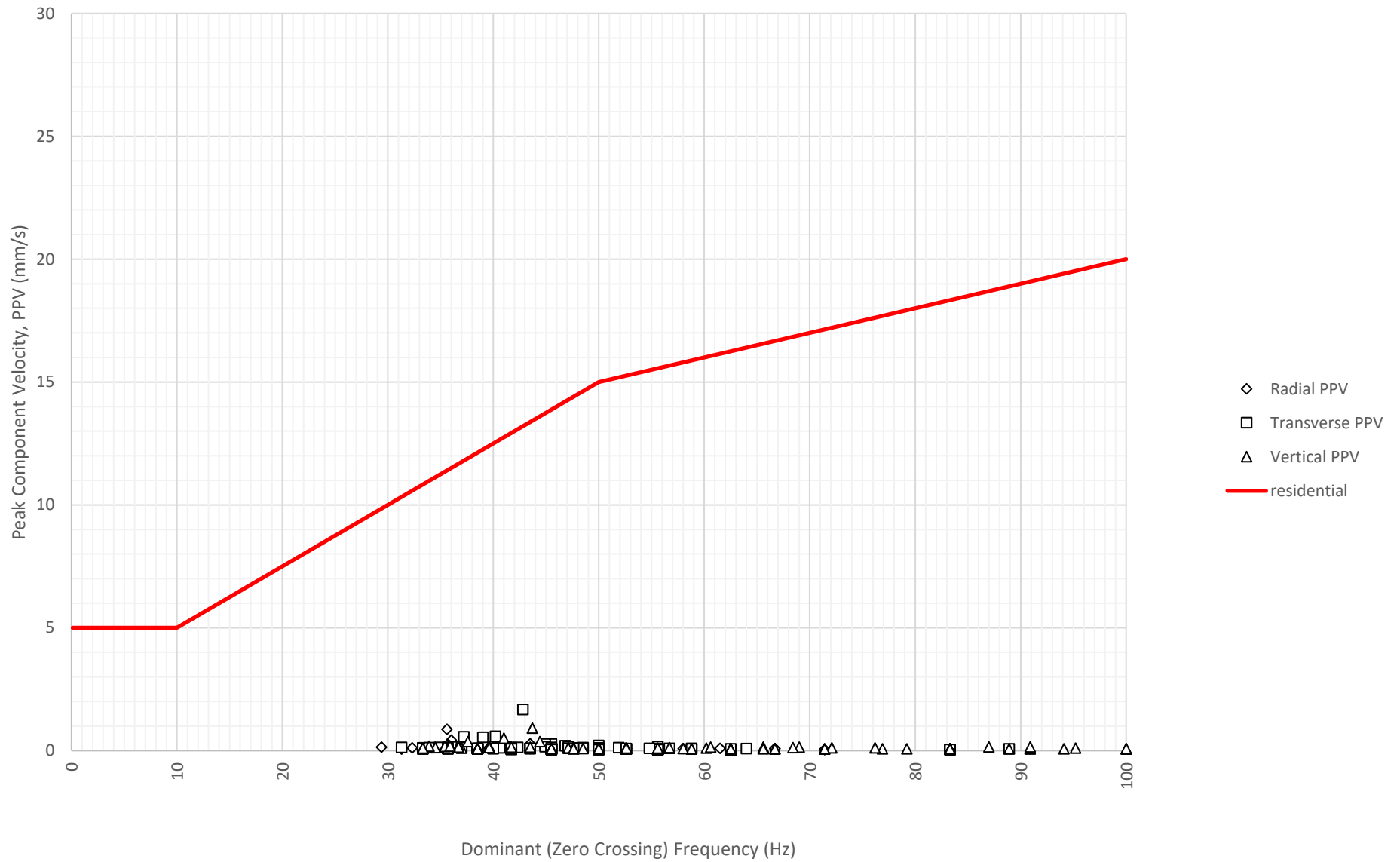
Frequency Content of Vibration Levels at East Boundary Opposite Shoalhaven Street (ETM7326) on 6-09-2024
