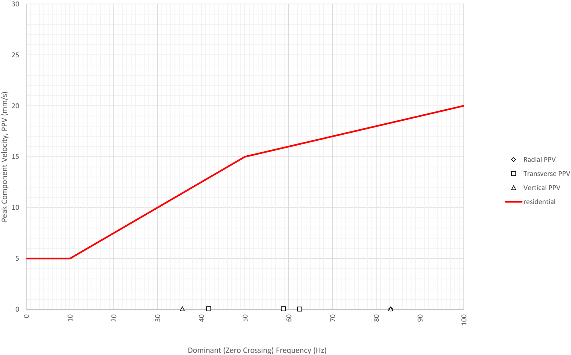
Frequency Content of Vibration Levels at East Boundary Opposite Shoalhaven Street (ETM7326) on 8-09-2024
