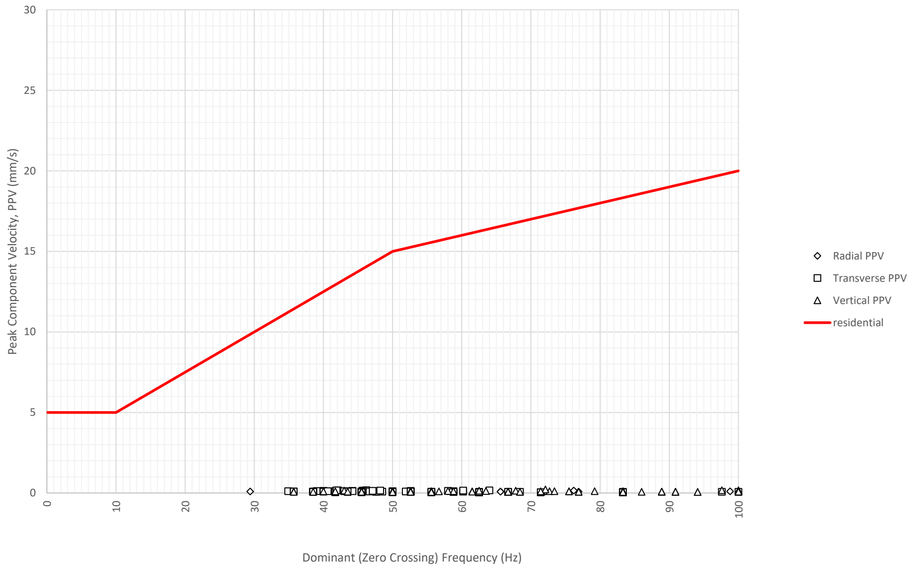
Frequency Content of Vibration Levels at East Boundary Opposite Shoalhaven Street (ETM7326) on 10-09-2024
