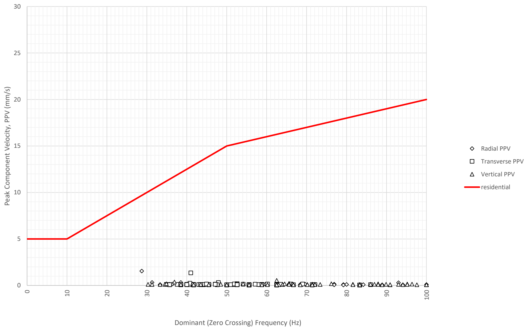
Frequency Content of Vibration Levels at East Boundary Opposite Shoalhaven Street (ETM7326) on 25-09-2024
