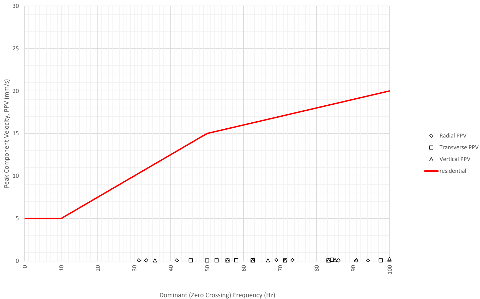
Frequency Content of Vibration Levels at North Boundary Near Block A and B (ETM7687) on 11-09-2024
