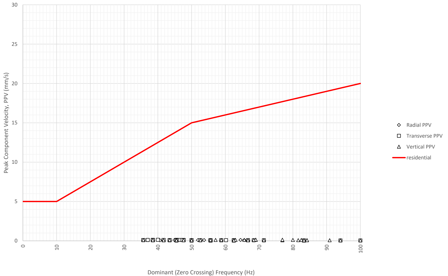
Frequency Content of Vibration Levels at East Boundary Opposite Shoalhaven Street (ETM7326) on 28-09-2024
