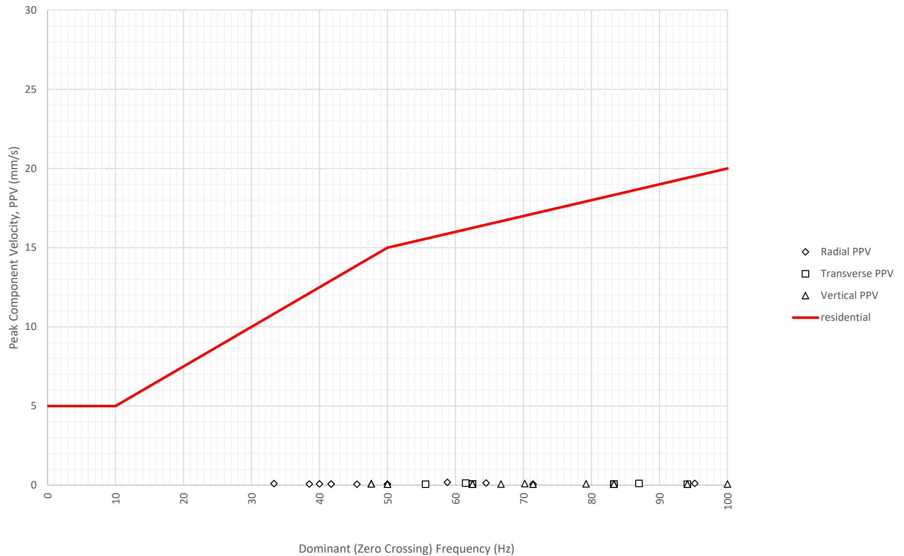
Frequency Content of Vibration Levels at North Boundary Near Block A and B (ETM7687) on 17-09-2024
