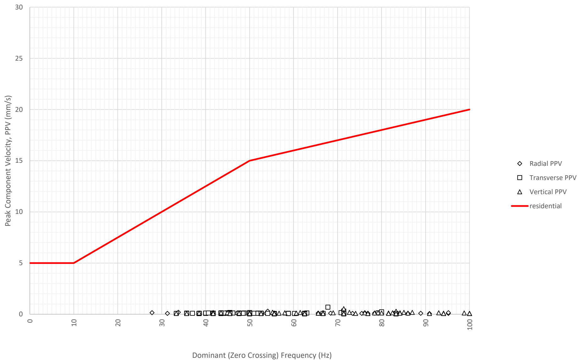
Frequency Content of Vibration Levels at East Boundary Opposite Shoalhaven Street (ETM7326) on 18-09-2024
