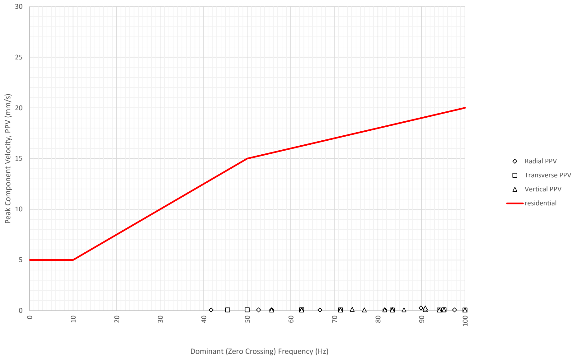
Frequency Content of Vibration Levels at North Boundary Near Block A and B (ETM7687) on 18-09-2024
