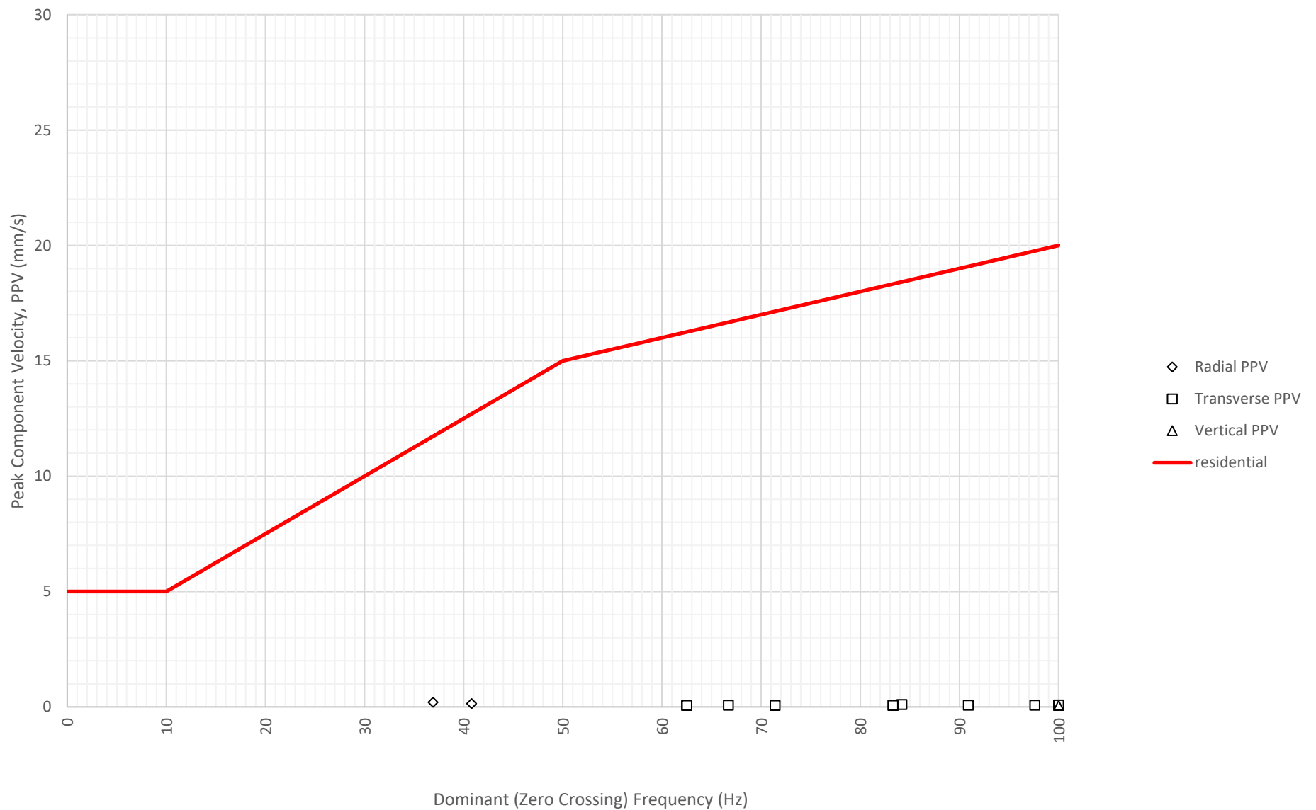
Frequency Content of Vibration Levels at North Boundary Near Block A and B (ETM7687) on 28-09-2024
