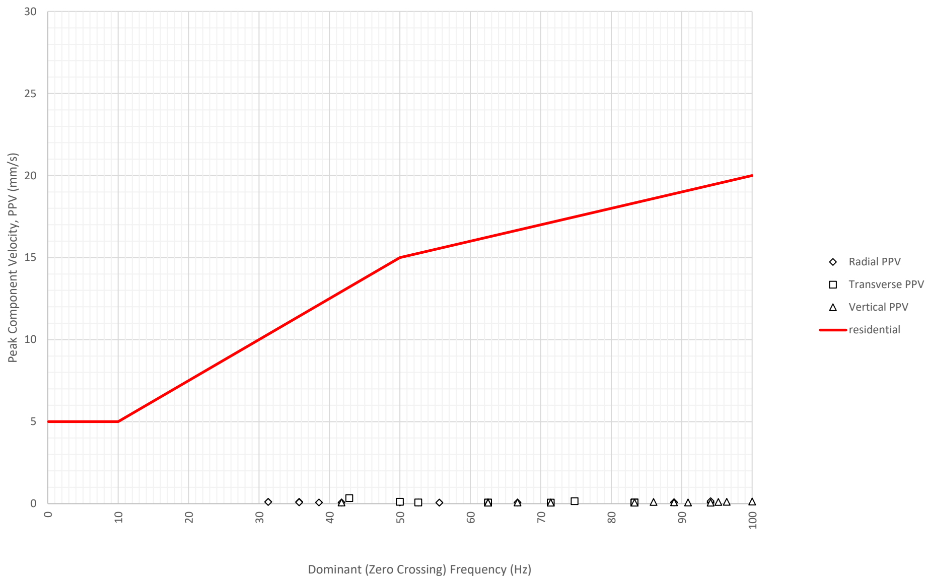
Frequency Content of Vibration Levels at North Boundary Near Block A and B (ETM7687) on 24-09-2024
