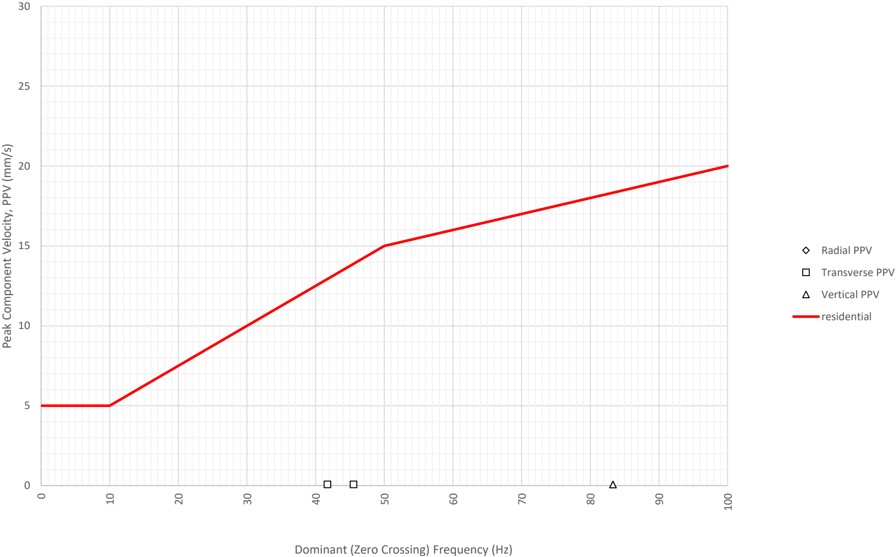
Frequency Content of Vibration Levels at East Boundary Opposite Shoalhaven Street (ETM7326) on 1-09-2024
