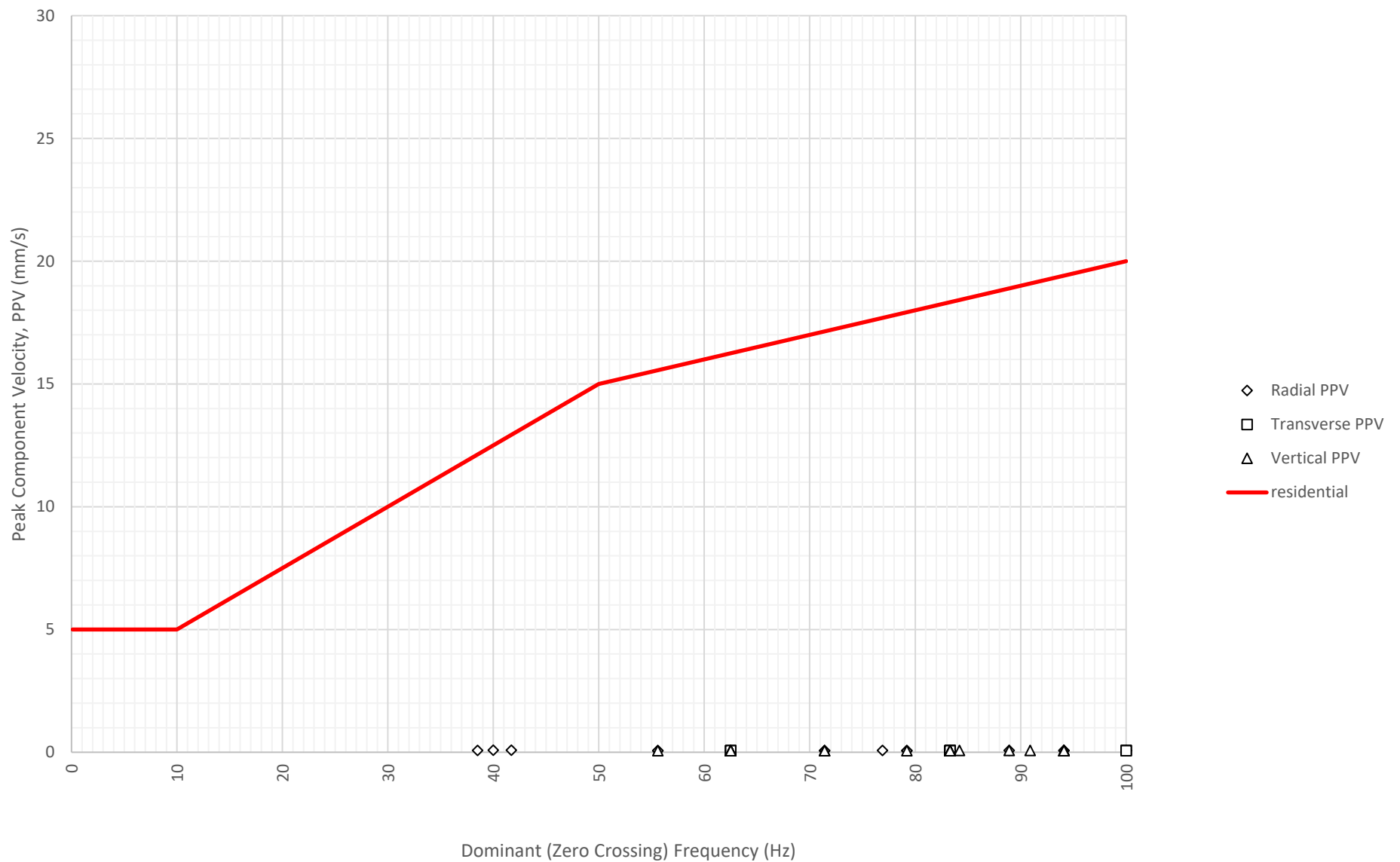
Frequency Content of Vibration Levels at North Boundary Near Block A and B (ETM7687) on 20-09-2024
