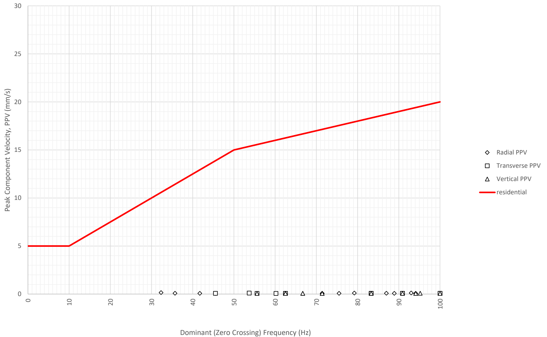
Frequency Content of Vibration Levels at North Boundary Near Block A and B (ETM7687) on 10-09-2024
