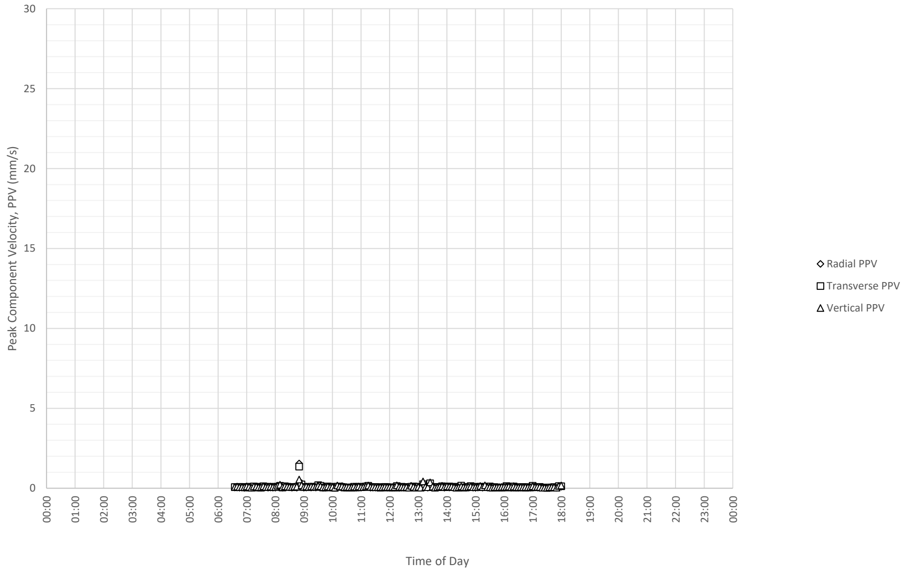
Daily Monitored Vibration Levels at East Boundary Opposite Shoalhaven Street (ETM7326) on 25-09-2024
