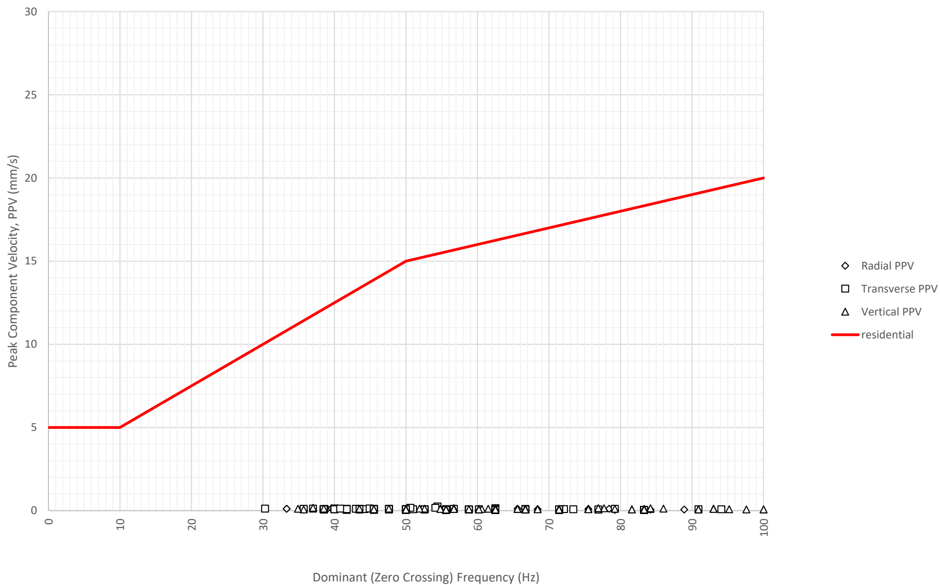
Frequency Content of Vibration Levels at East Boundary Opposite Shoalhaven Street (ETM7326) on 20-09-2024
