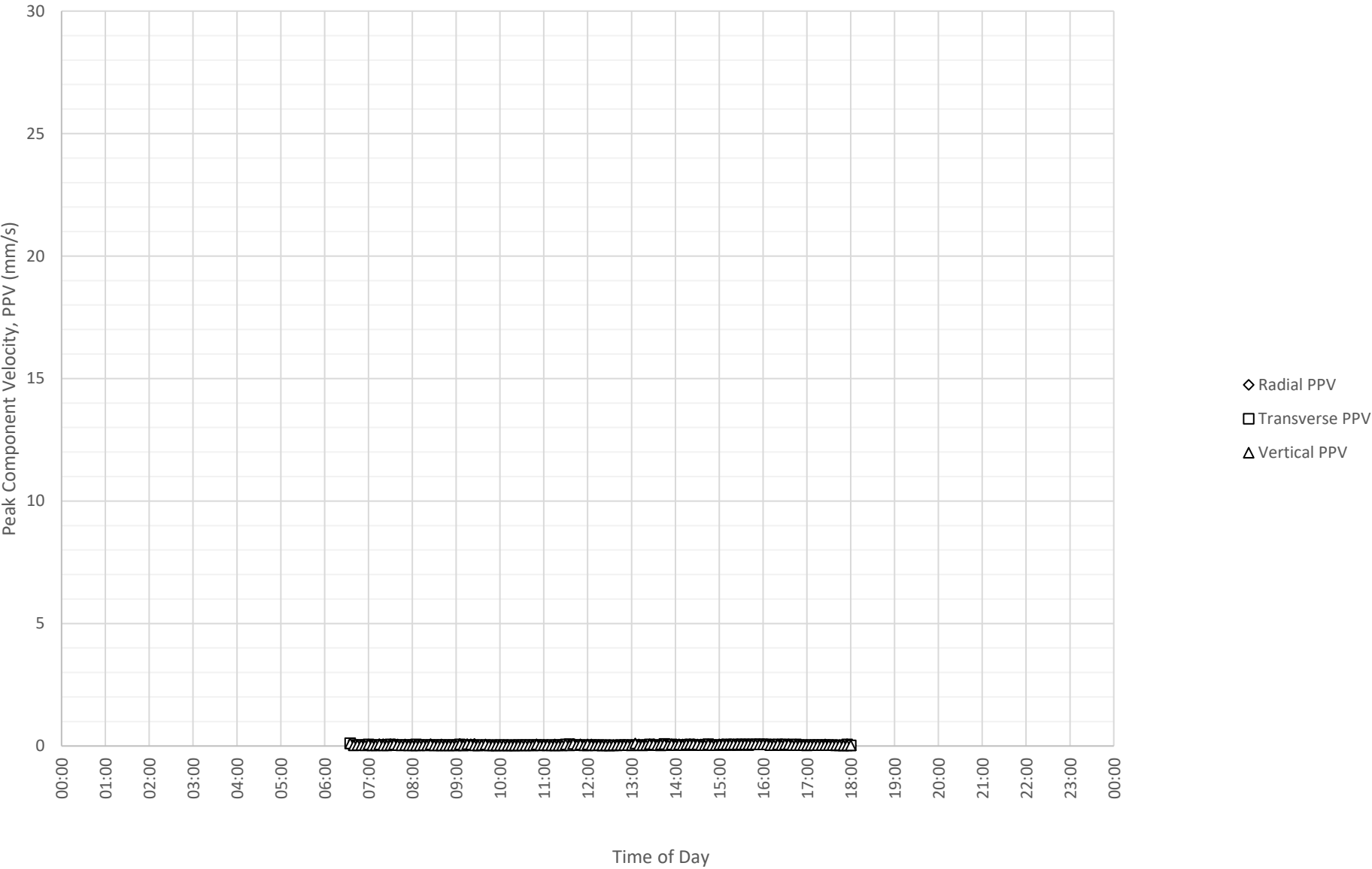
Daily Monitored Vibration Levels at North Boundary Near Block A and B (ETM7687) on 20-09-2024
