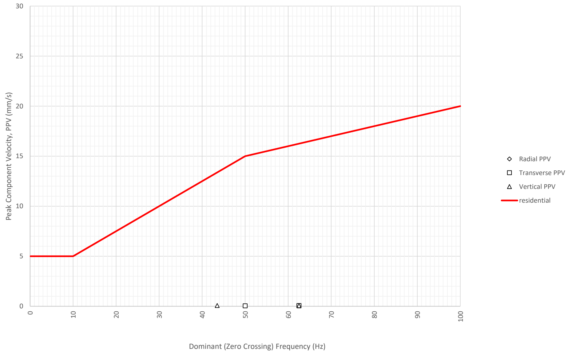
Frequency Content of Vibration Levels at East Boundary Opposite Shoalhaven Street (ETM7326) on 29-09-2024
