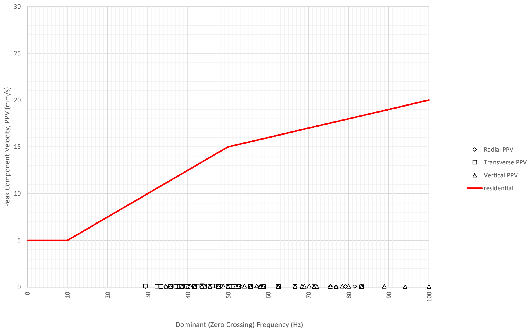
Frequency Content of Vibration Levels at East Boundary Opposite Shoalhaven Street (ETM7326) on 27-09-2024
