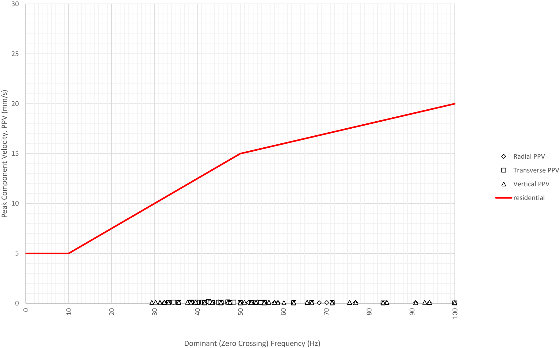
Frequency Content of Vibration Levels at East Boundary Opposite Shoalhaven Street (ETM7326) on 4-09-2024
