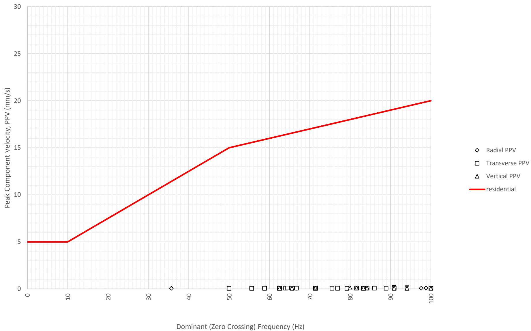
Frequency Content of Vibration Levels at North Boundary Near Block A and B (ETM7687) on 30-09-2024
