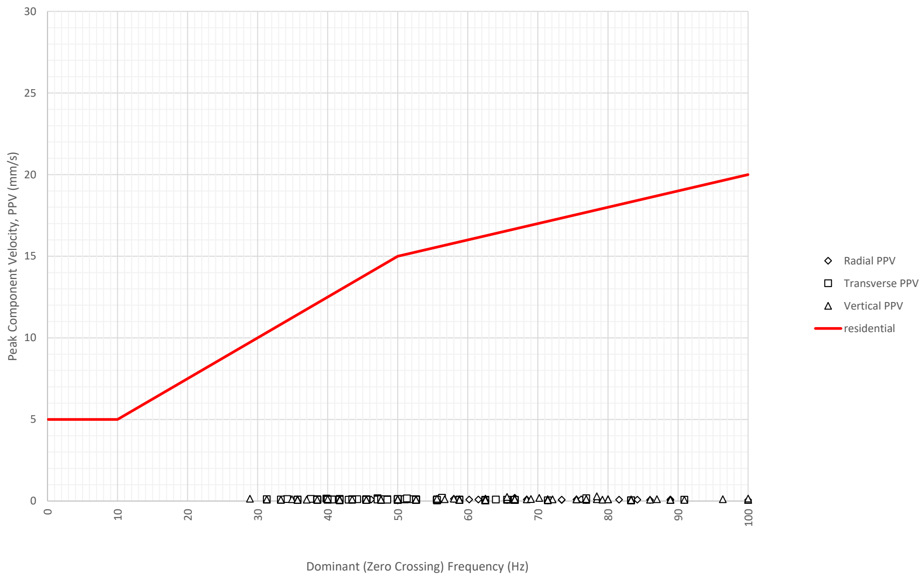
Frequency Content of Vibration Levels at East Boundary Opposite Shoalhaven Street (ETM7326) on 17-09-2024
