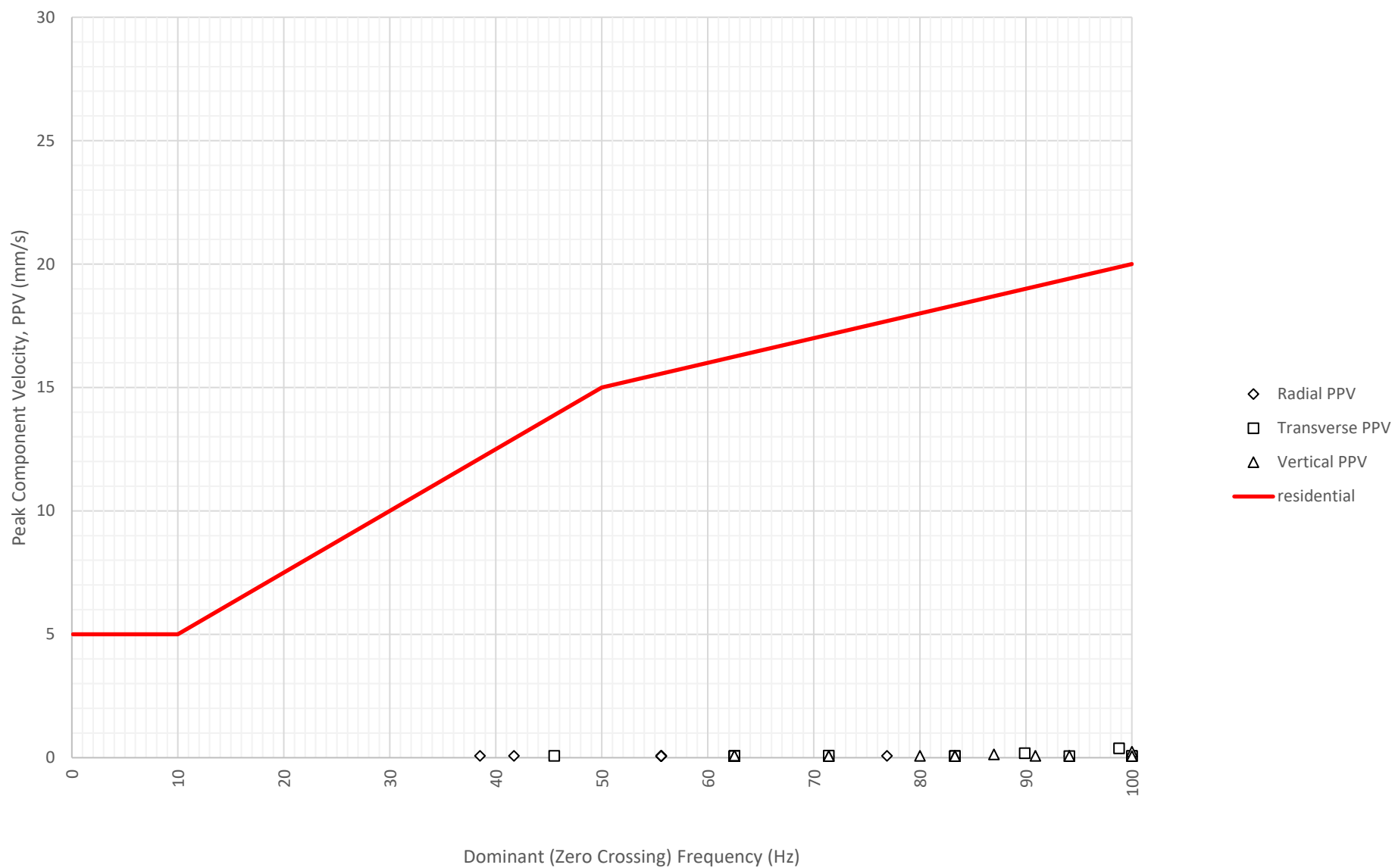
Frequency Content of Vibration Levels at North Boundary Near Block A and B (ETM7687) on 16-09-2024
