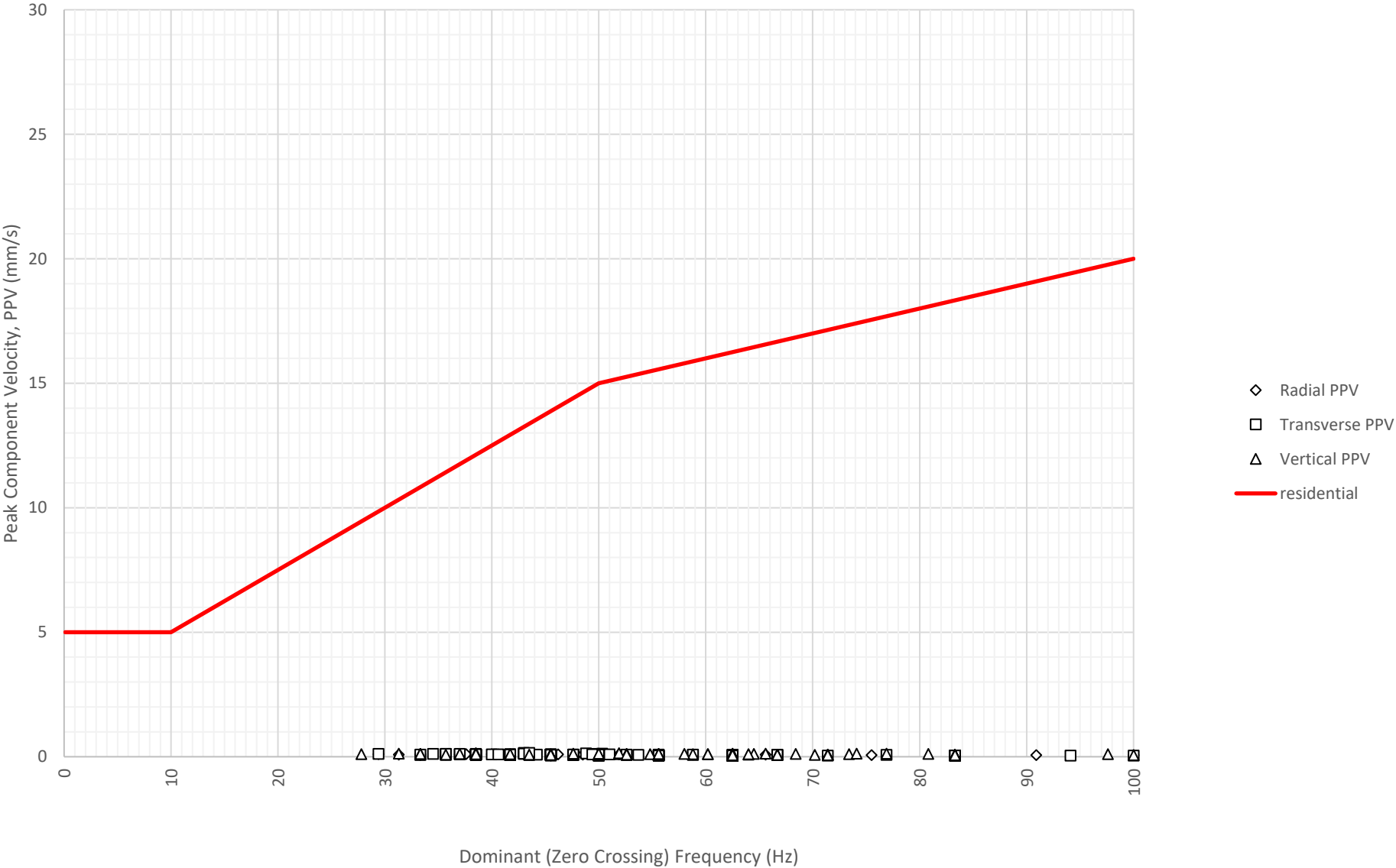
Frequency Content of Vibration Levels at East Boundary Opposite Shoalhaven Street (ETM7326) on 3-09-2024
