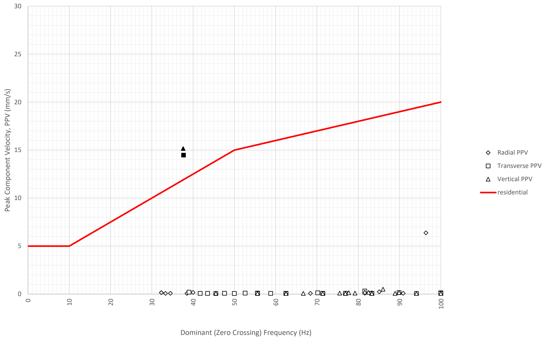
Frequency Content of Vibration Levels at North Boundary Near Block A and B (ETM7687) on 5-09-2024
