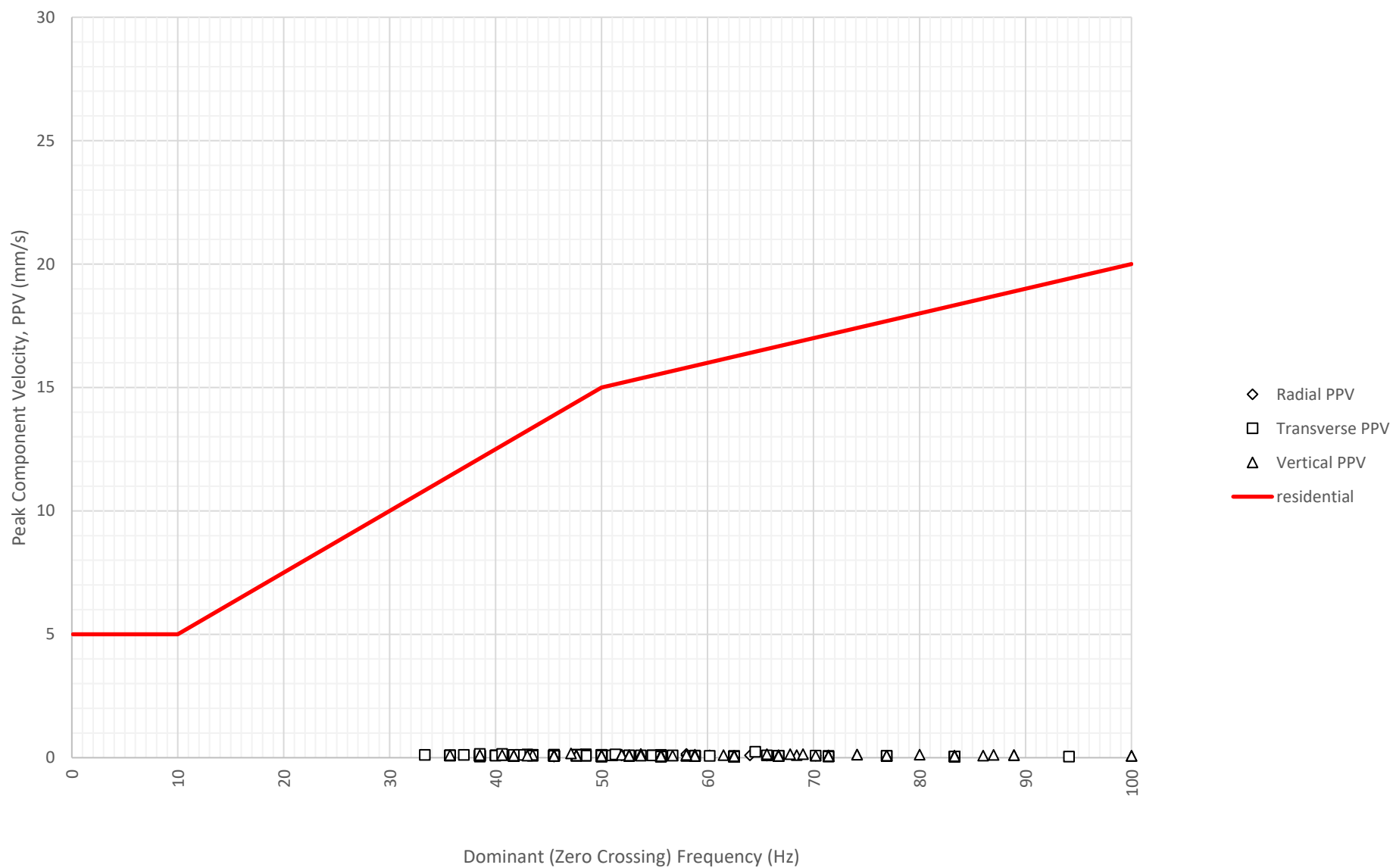
Frequency Content of Vibration Levels at East Boundary Opposite Shoalhaven Street (ETM7326) on 26-09-2024
