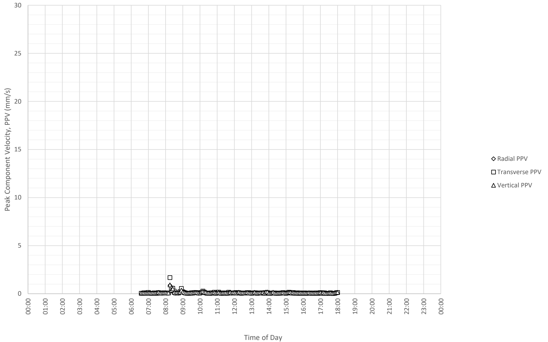
Daily Monitored Vibration Levels at East Boundary Opposite Shoalhaven Street (ETM7326) on 6-09-2024
