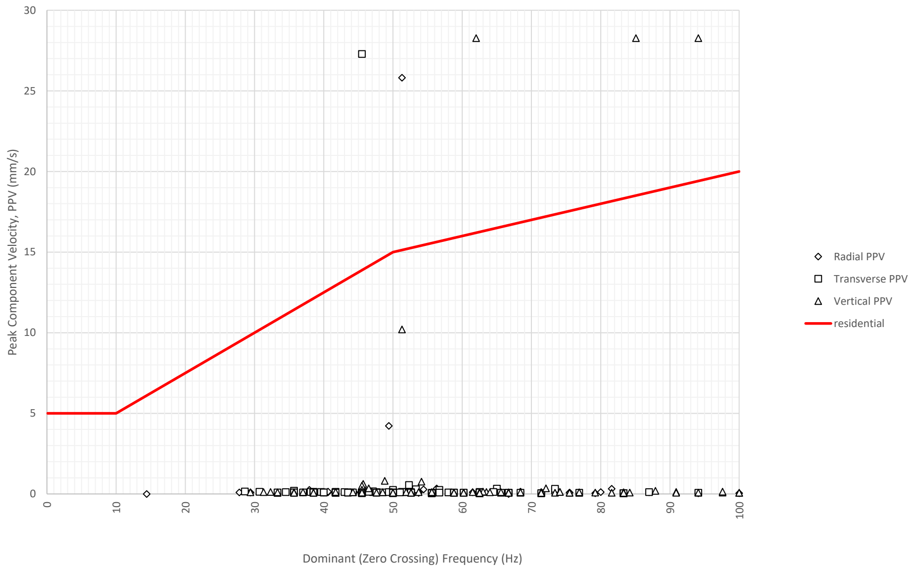
Frequency Content of Vibration Levels at East Boundary Opposite Shoalhaven Street (ETM7326) on 13-09-2024
