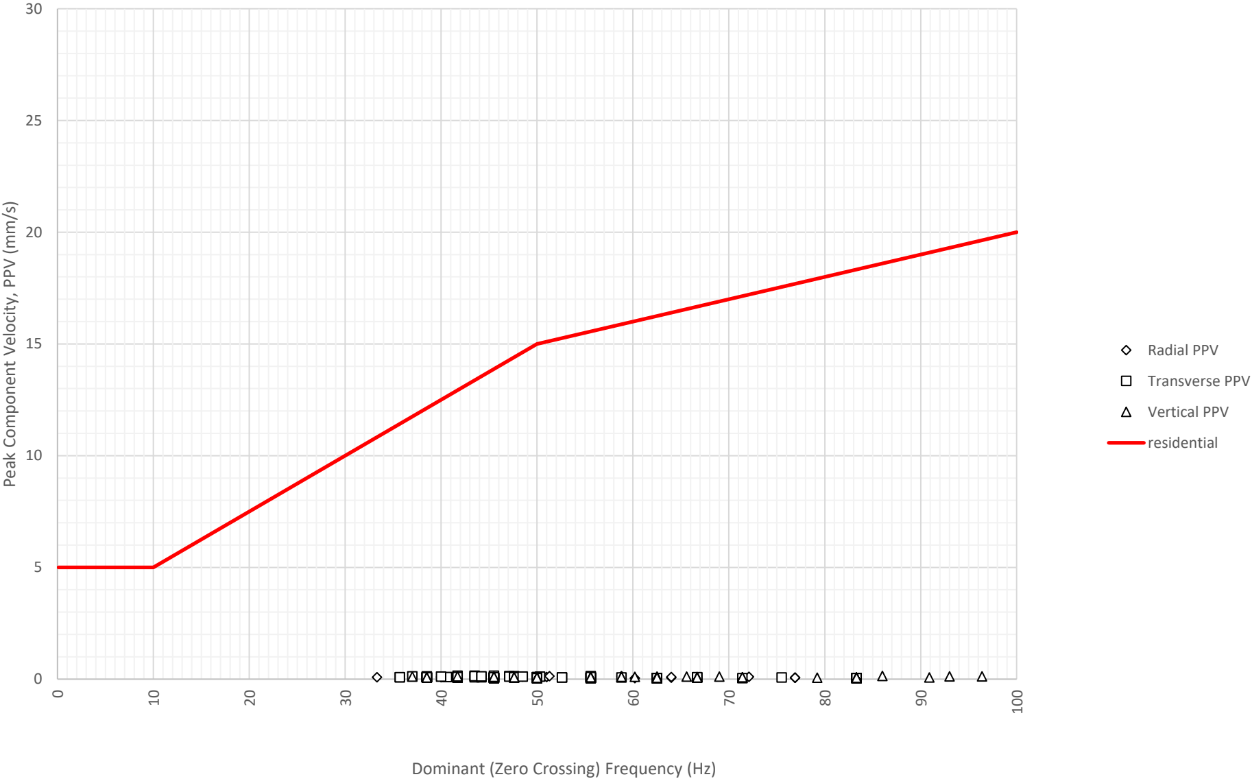
Frequency Content of Vibration Levels at East Boundary Opposite Shoalhaven Street (ETM7326) on 7-09-2024
