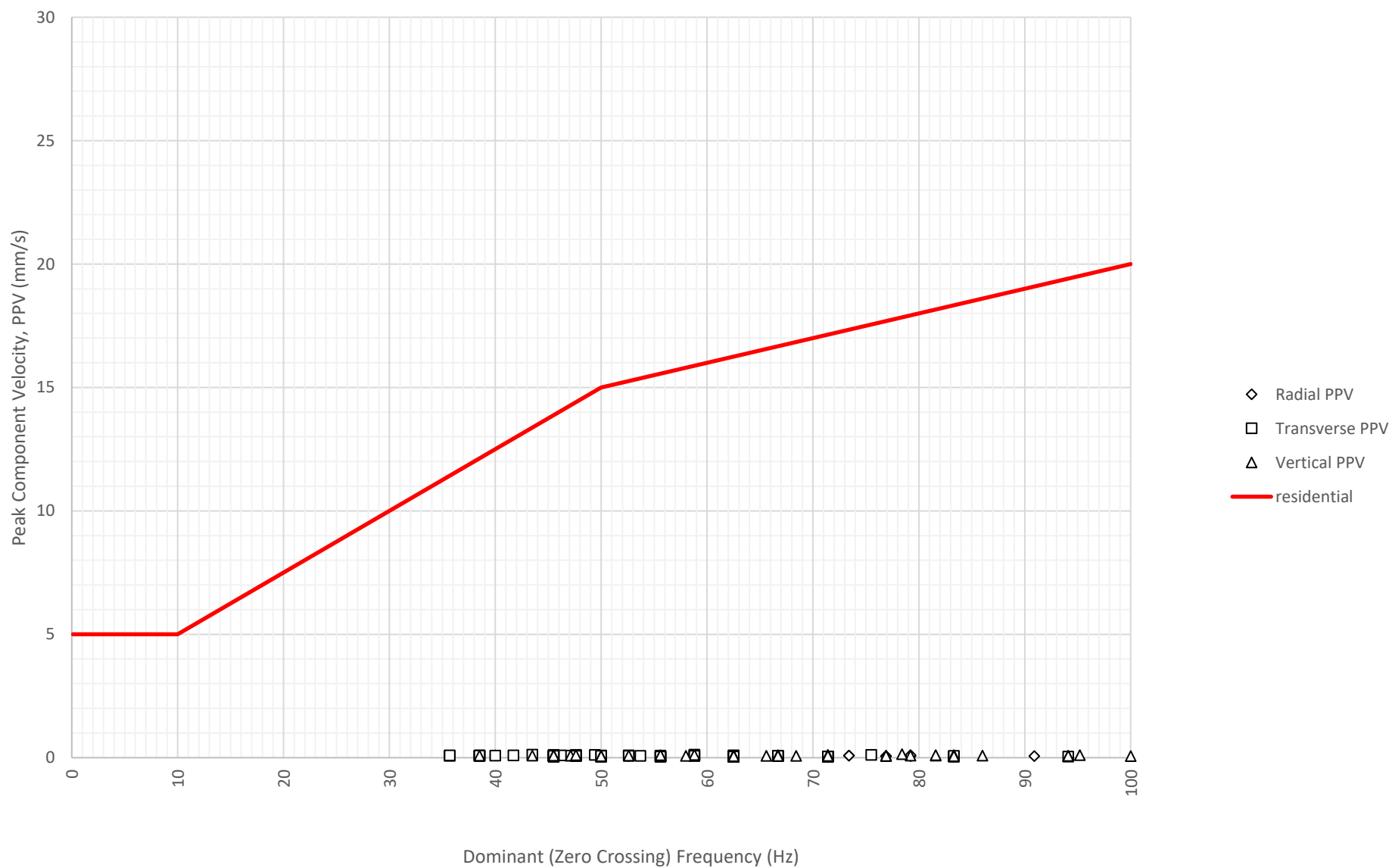
Frequency Content of Vibration Levels at East Boundary Opposite Shoalhaven Street (ETM7326) on 21-09-2024
