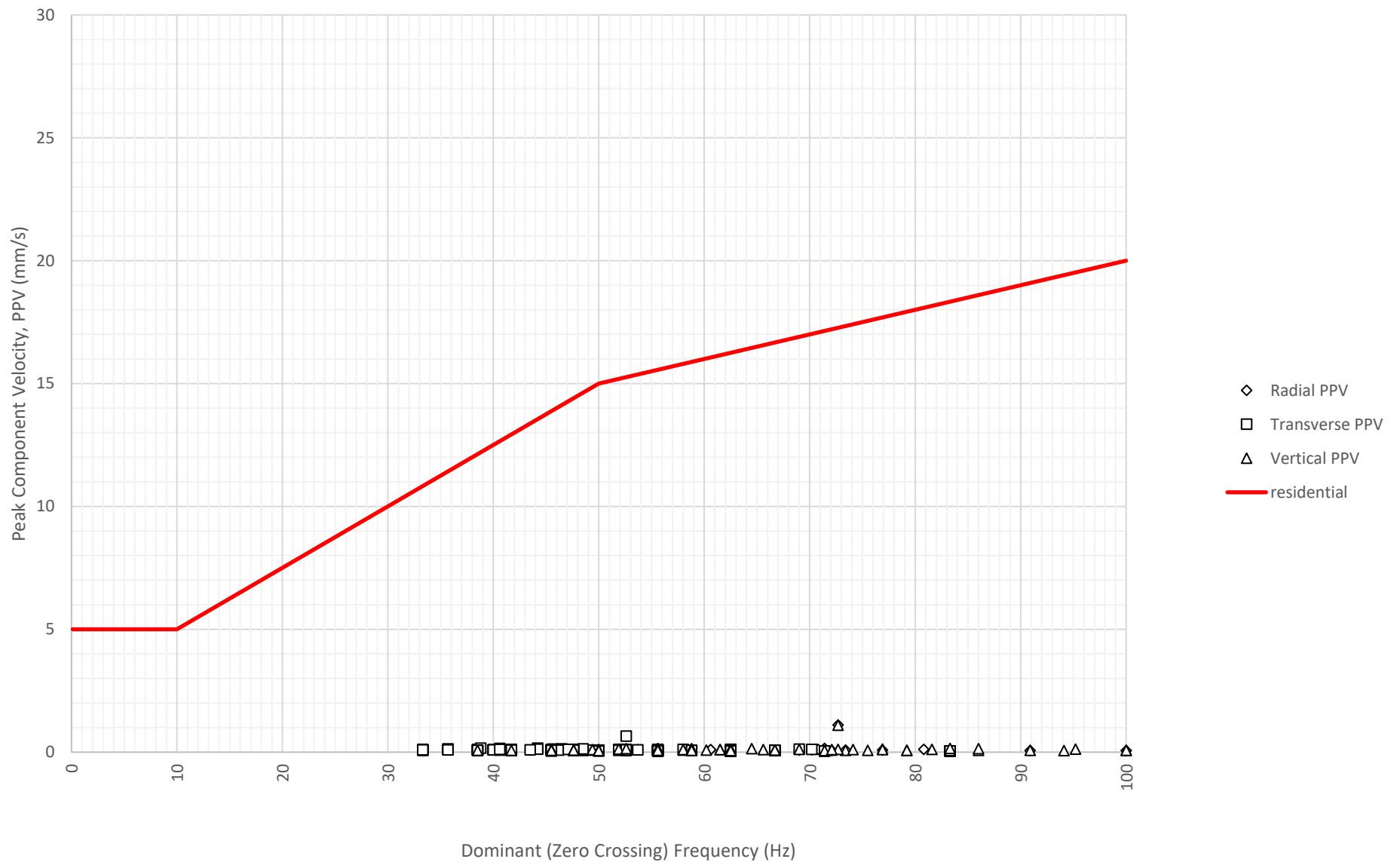
Frequency Content of Vibration Levels at East Boundary Opposite Shoalhaven Street (ETM7326) on 30-09-2024
