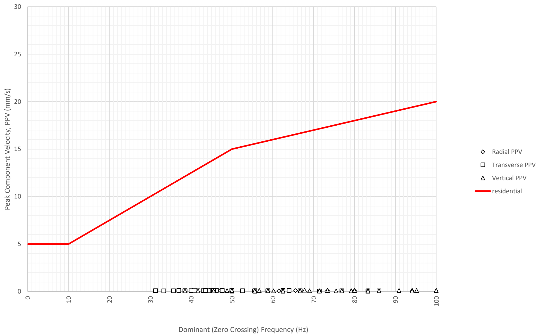
Frequency Content of Vibration Levels at East Boundary Opposite Shoalhaven Street (ETM7326) on 14-09-2024
