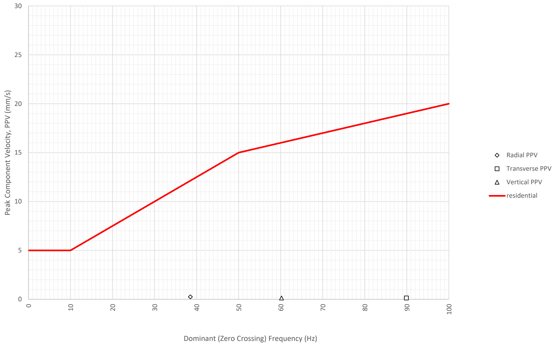
Frequency Content of Vibration Levels at North Boundary Near Block A and B (ETM7687) on 7-09-2024
