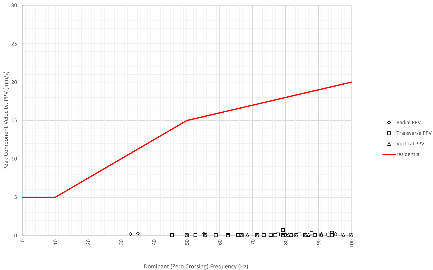
Frequency Content of Vibration Levels at North Boundary Near Block A and B (ETM7687) on 26-09-2024
