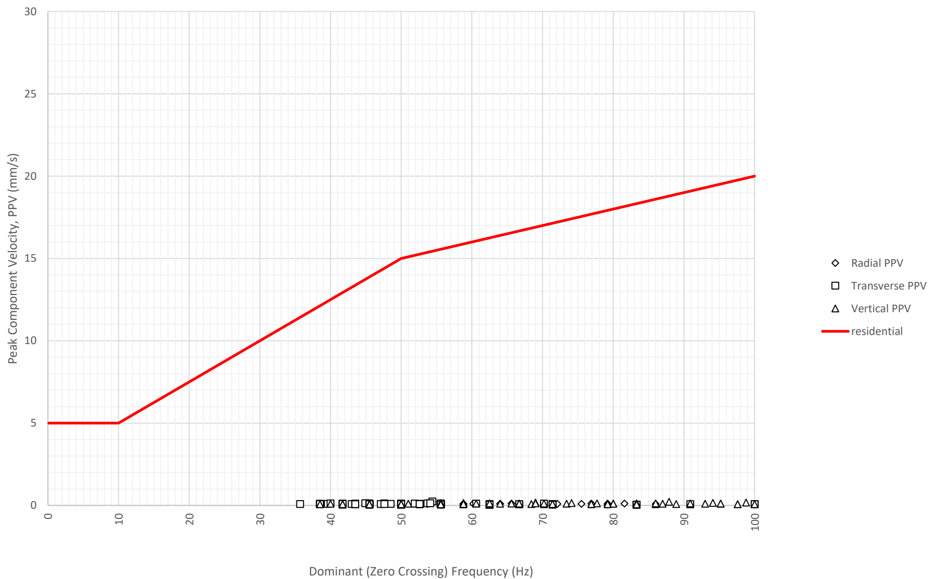
Frequency Content of Vibration Levels at East Boundary Opposite Shoalhaven Street (ETM7326) on 24-09-2024
