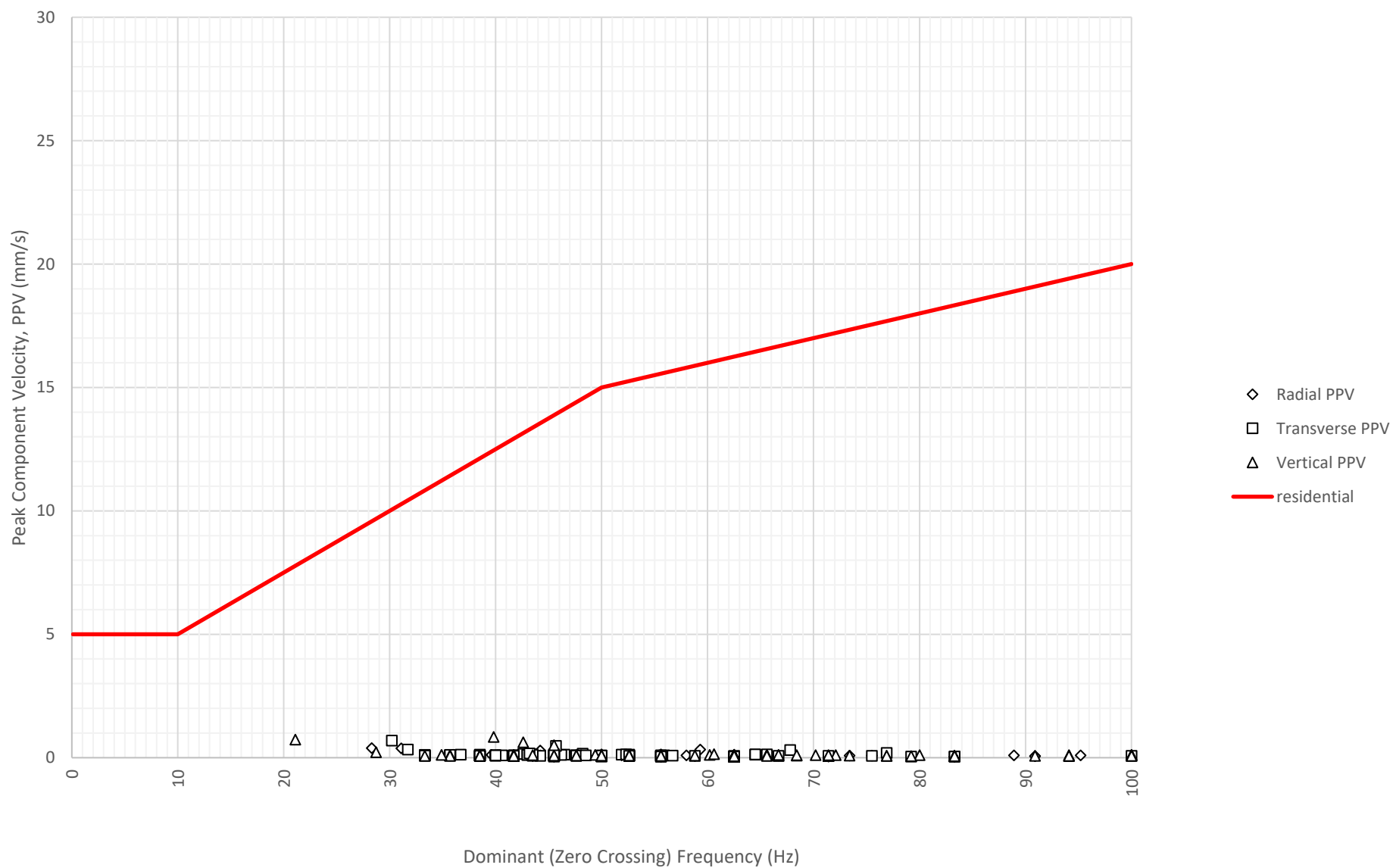
Frequency Content of Vibration Levels at East Boundary Opposite Shoalhaven Street (ETM7326) on 11-09-2024
