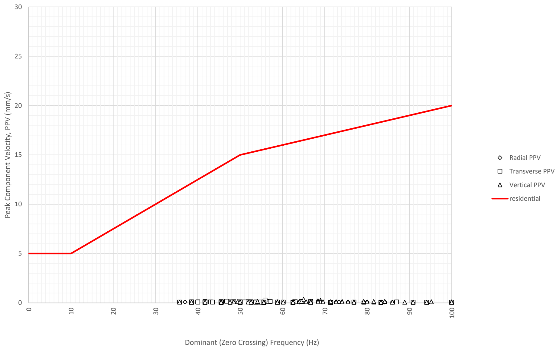
Frequency Content of Vibration Levels at East Boundary Opposite Shoalhaven Street (ETM7326) on 19-09-2024
