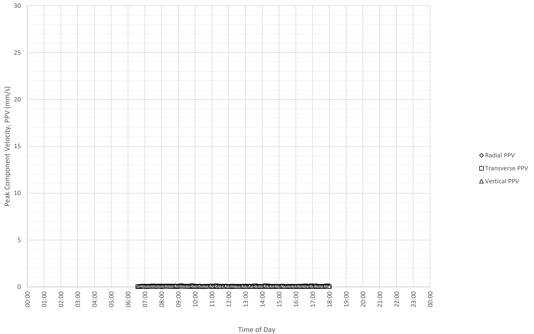
Daily Monitored Vibration Levels at East Boundary Opposite Shoalhaven Street (ETM7326) on 14-09-2024
