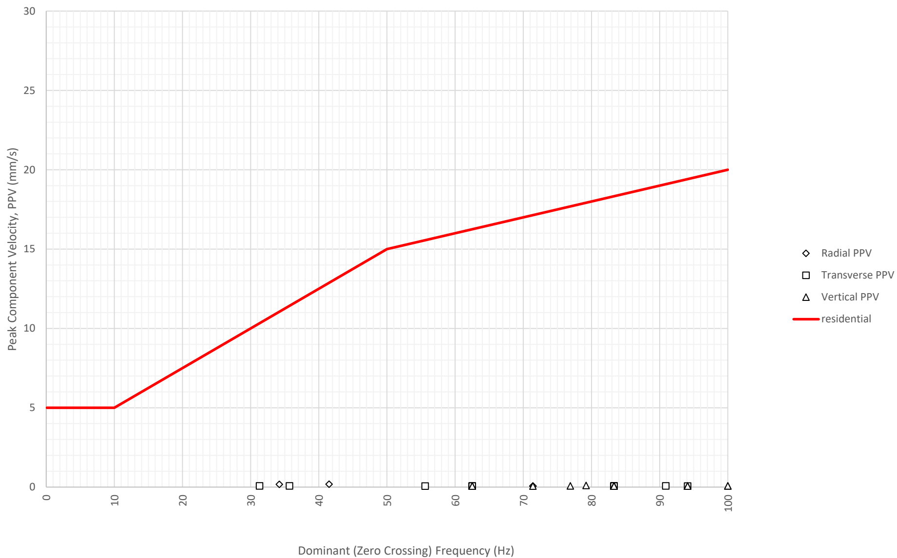
Frequency Content of Vibration Levels at North Boundary Near Block A and B (ETM7687) on 21-09-2024
