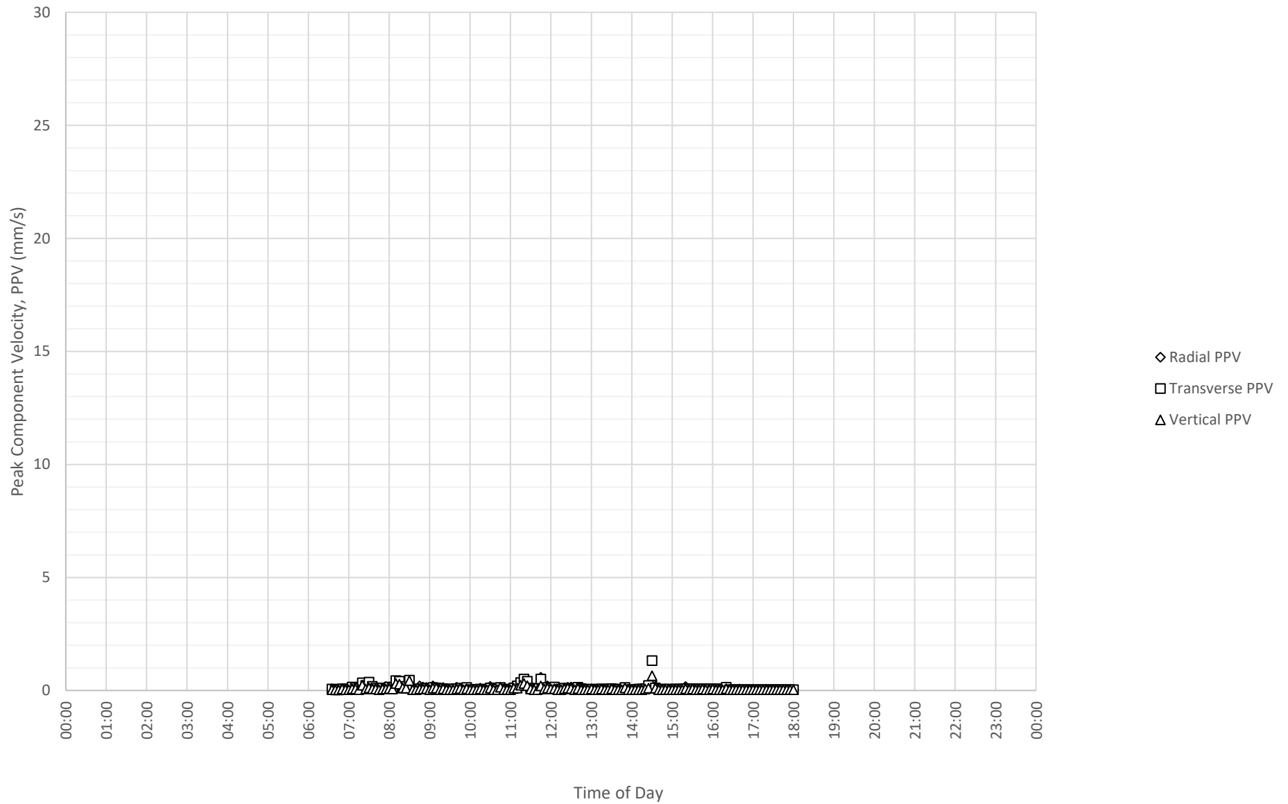
Daily Monitored Vibration Levels at North Boundary Near Block A and B (ETM7687) on 7-11-2024
