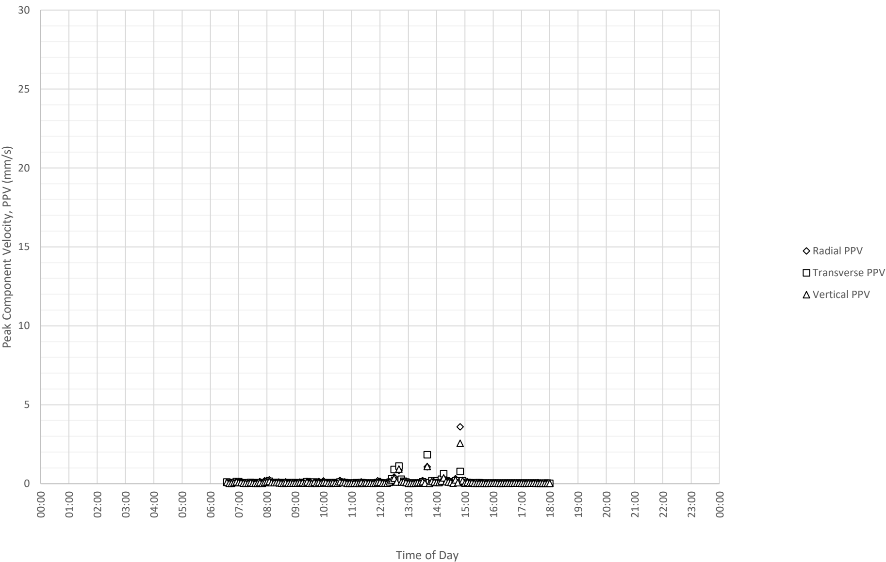
Daily Monitored Vibration Levels at North Boundary Near Block A and B (ETM7687) on 15-11-2024
