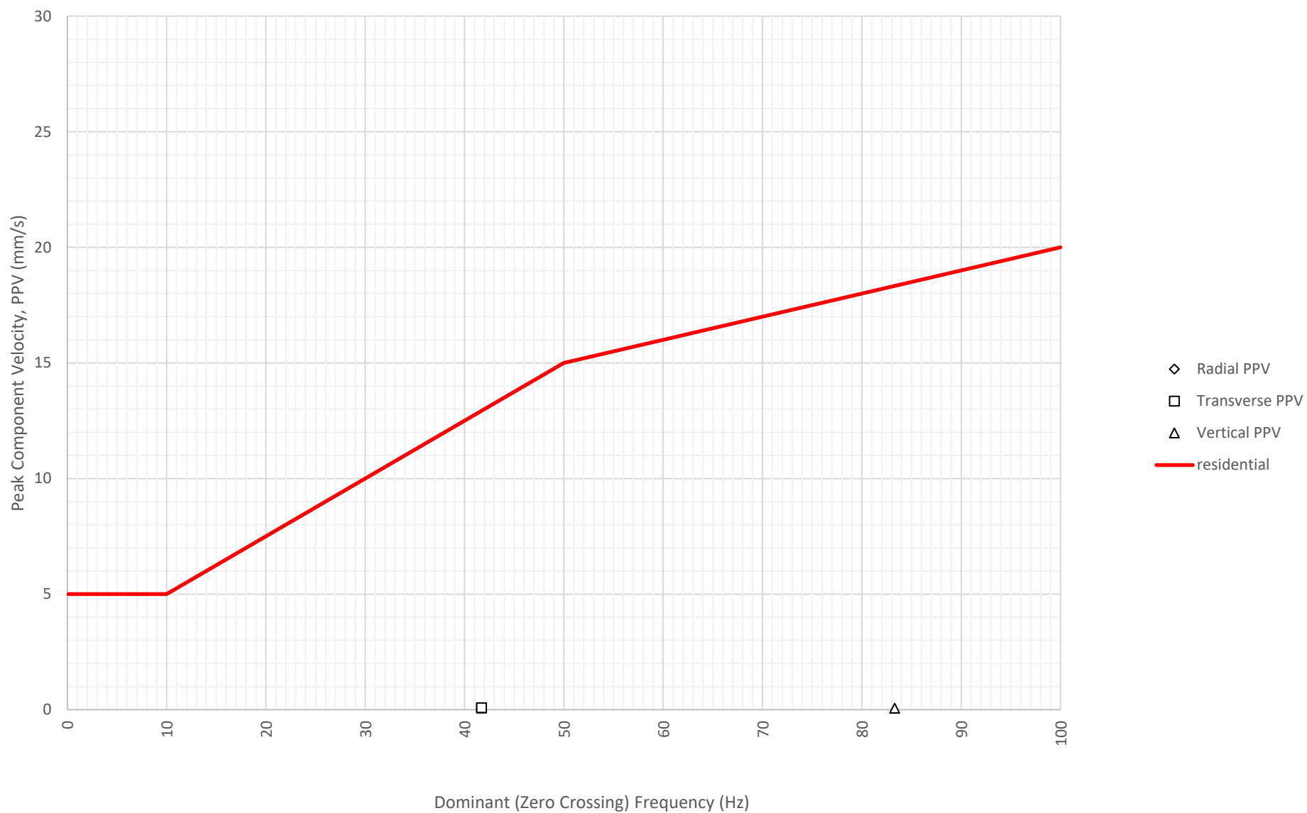
Frequency Content of Vibration Levels at East Boundary Opposite Shoalhaven Street (ETM7326) on 17-11-2024
