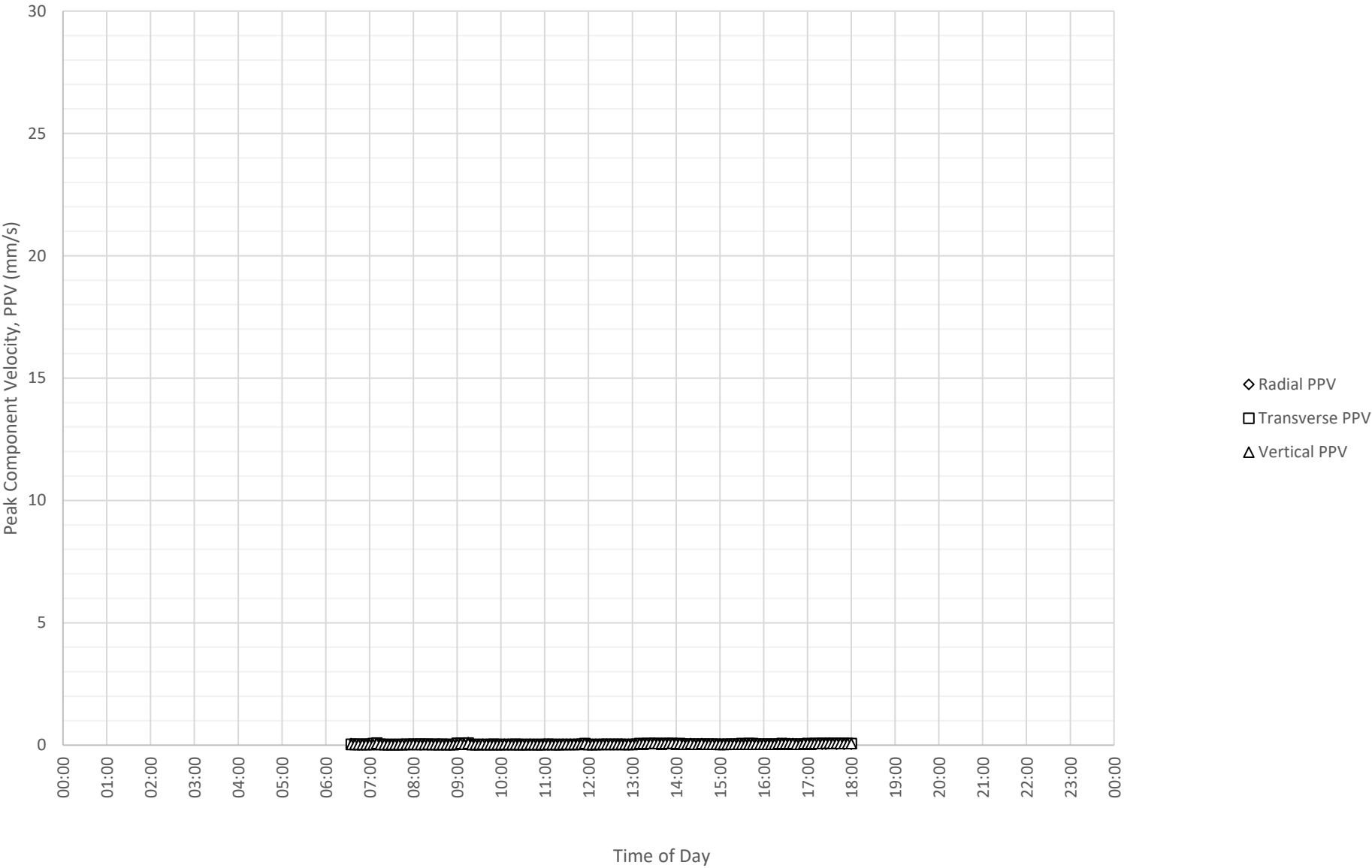
Daily Monitored Vibration Levels at North Boundary Near Block A and B (ETM7687) on 23-11-2024
