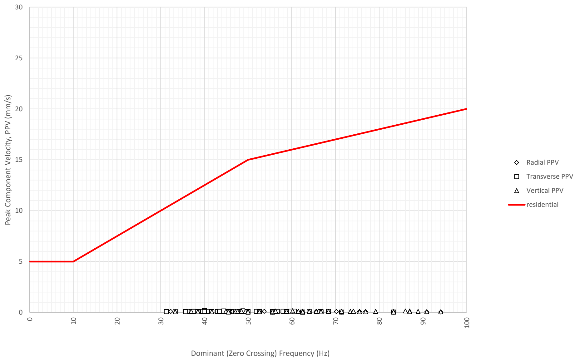
Frequency Content of Vibration Levels at East Boundary Opposite Shoalhaven Street (ETM7326) on 27-11-2024
