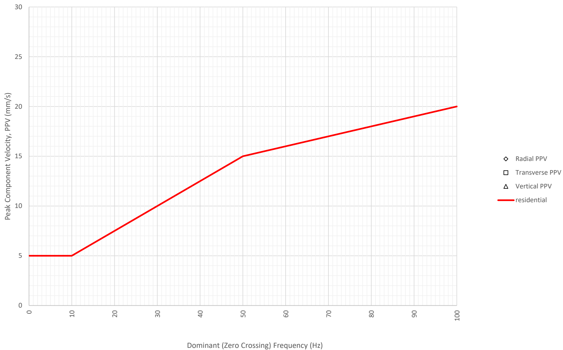
Frequency Content of Vibration Levels at North Boundary Near Block A and B (ETM7687) on 17-11-2024
