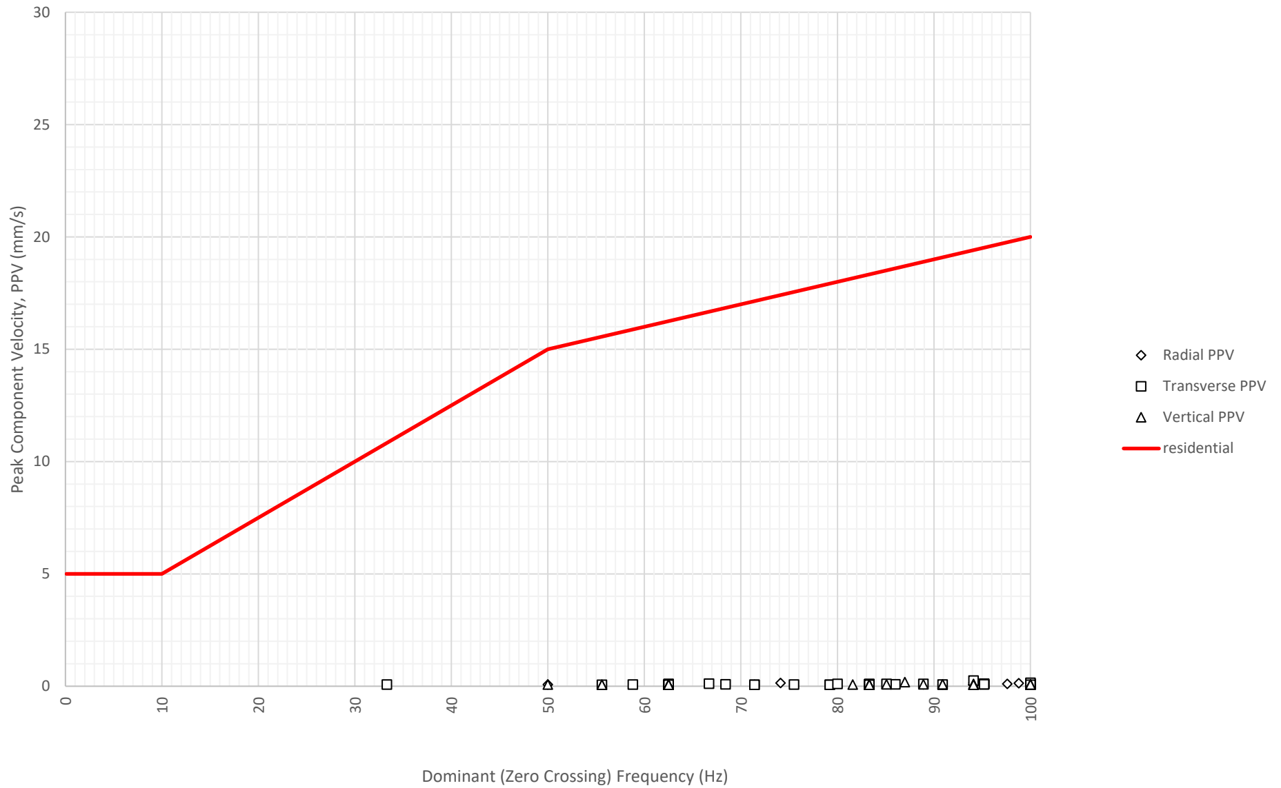
Frequency Content of Vibration Levels at North Boundary Near Block A and B (ETM7687) on 1-11-2024
