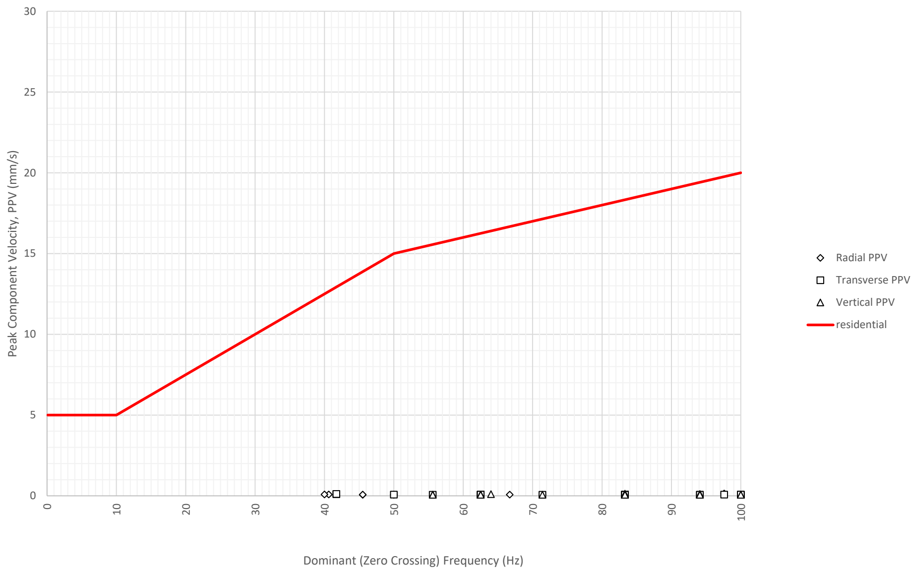
Frequency Content of Vibration Levels at North Boundary Near Block A and B (ETM7687) on 25-11-2024
