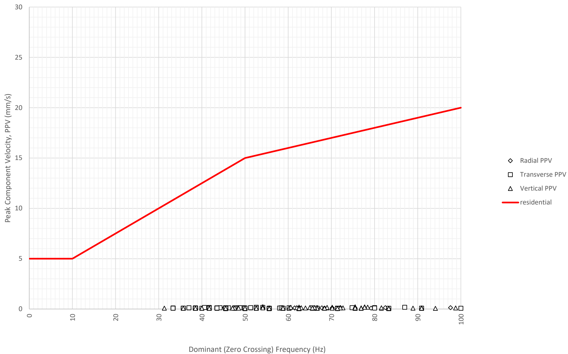
Frequency Content of Vibration Levels at East Boundary Opposite Shoalhaven Street (ETM7326) on 13-11-2024
