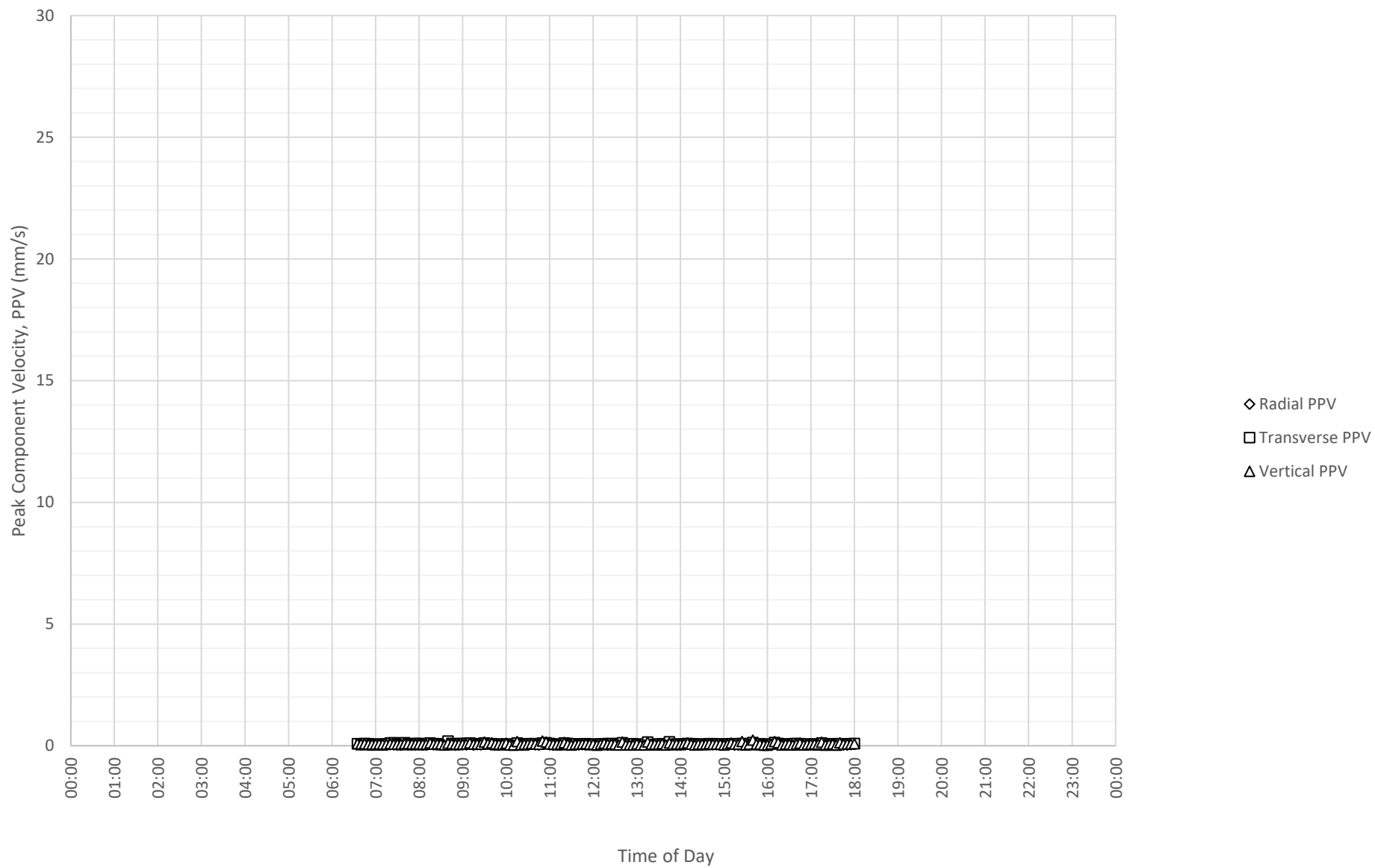
Daily Monitored Vibration Levels at East Boundary Opposite Shoalhaven Street (ETM7326) on 2-11-2024
