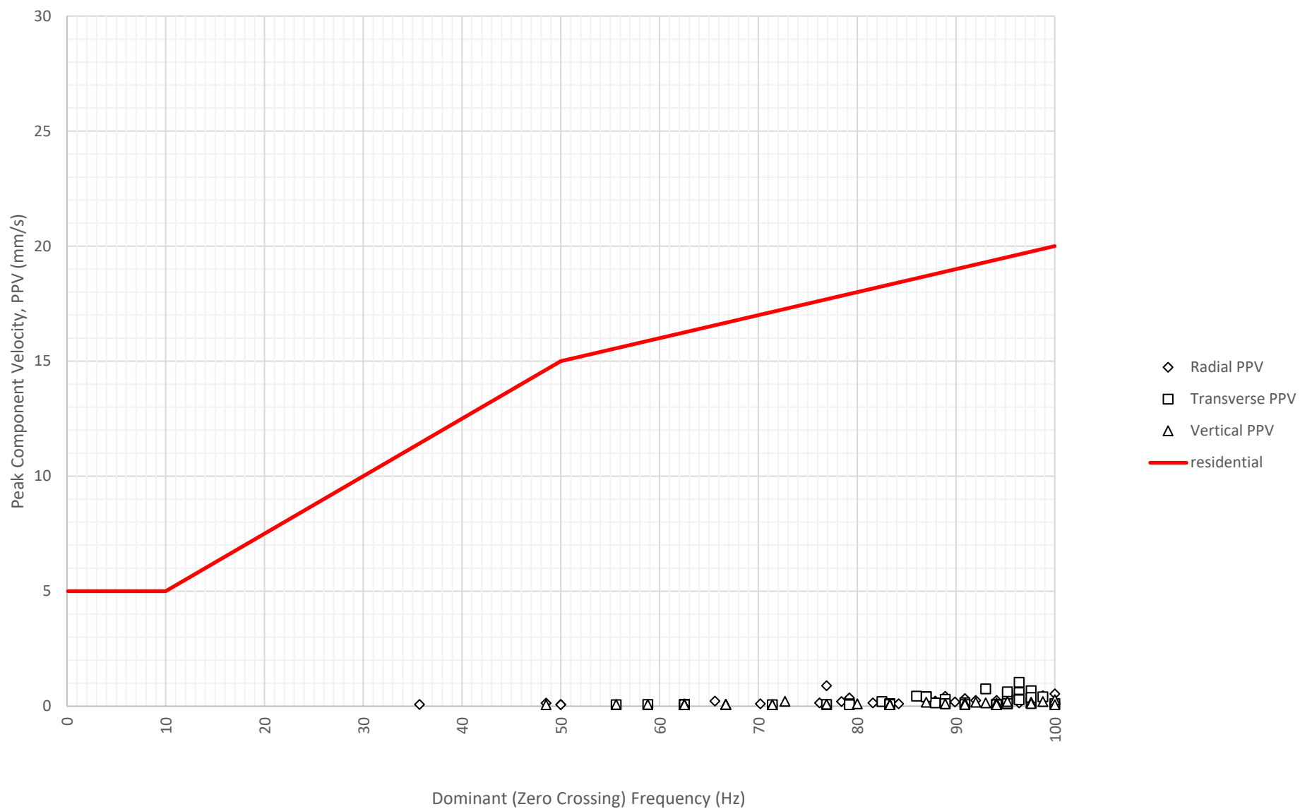
Frequency Content of Vibration Levels at North Boundary Near Block A and B (ETM7687) on 22-11-2024
