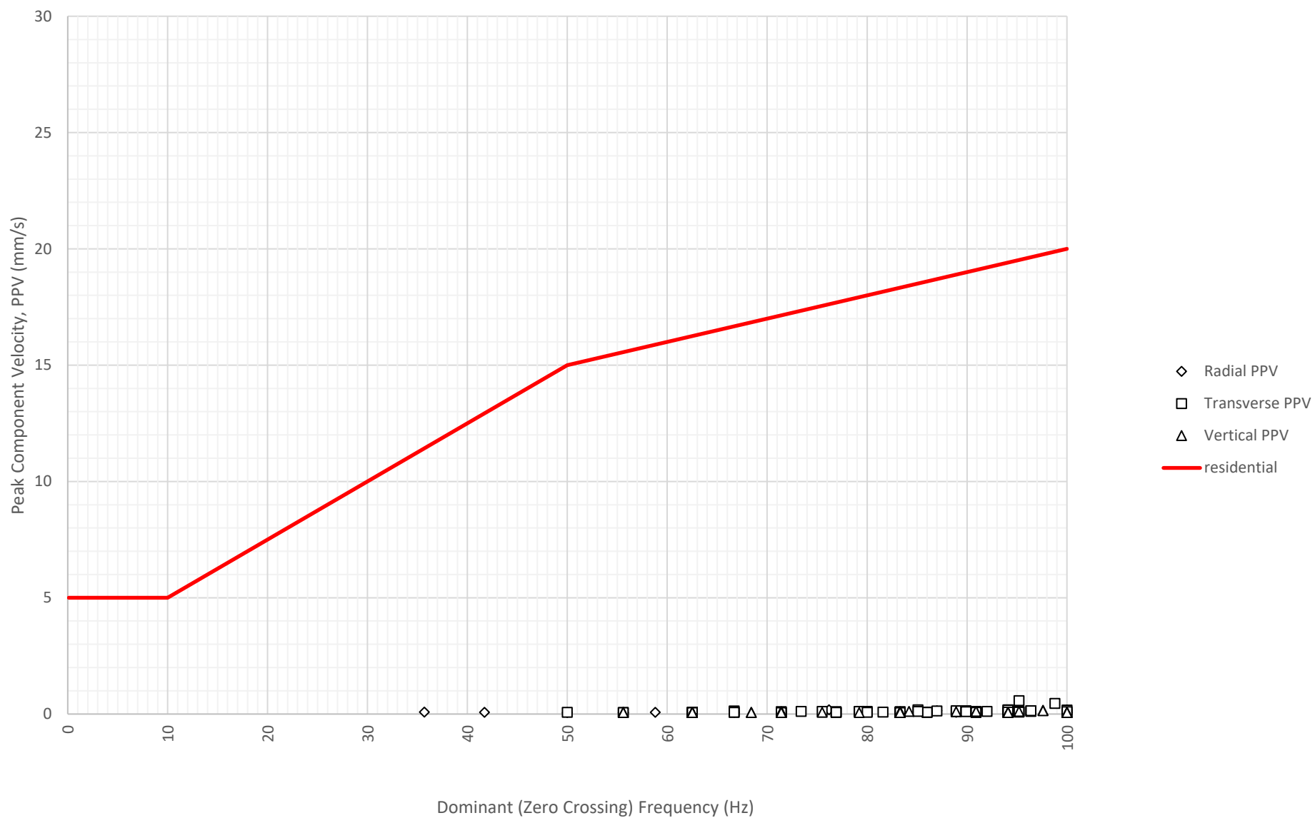
Frequency Content of Vibration Levels at North Boundary Near Block A and B (ETM7687) on 18-11-2024
