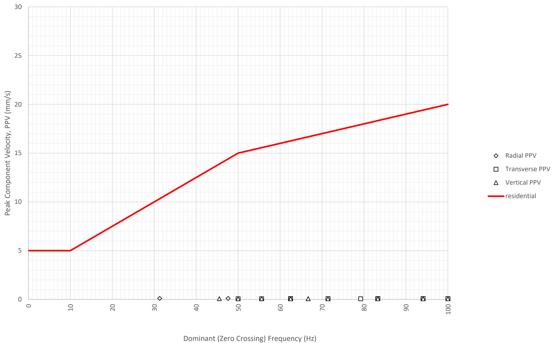
Frequency Content of Vibration Levels at North Boundary Near Block A and B (ETM7687) on 16-11-2024
