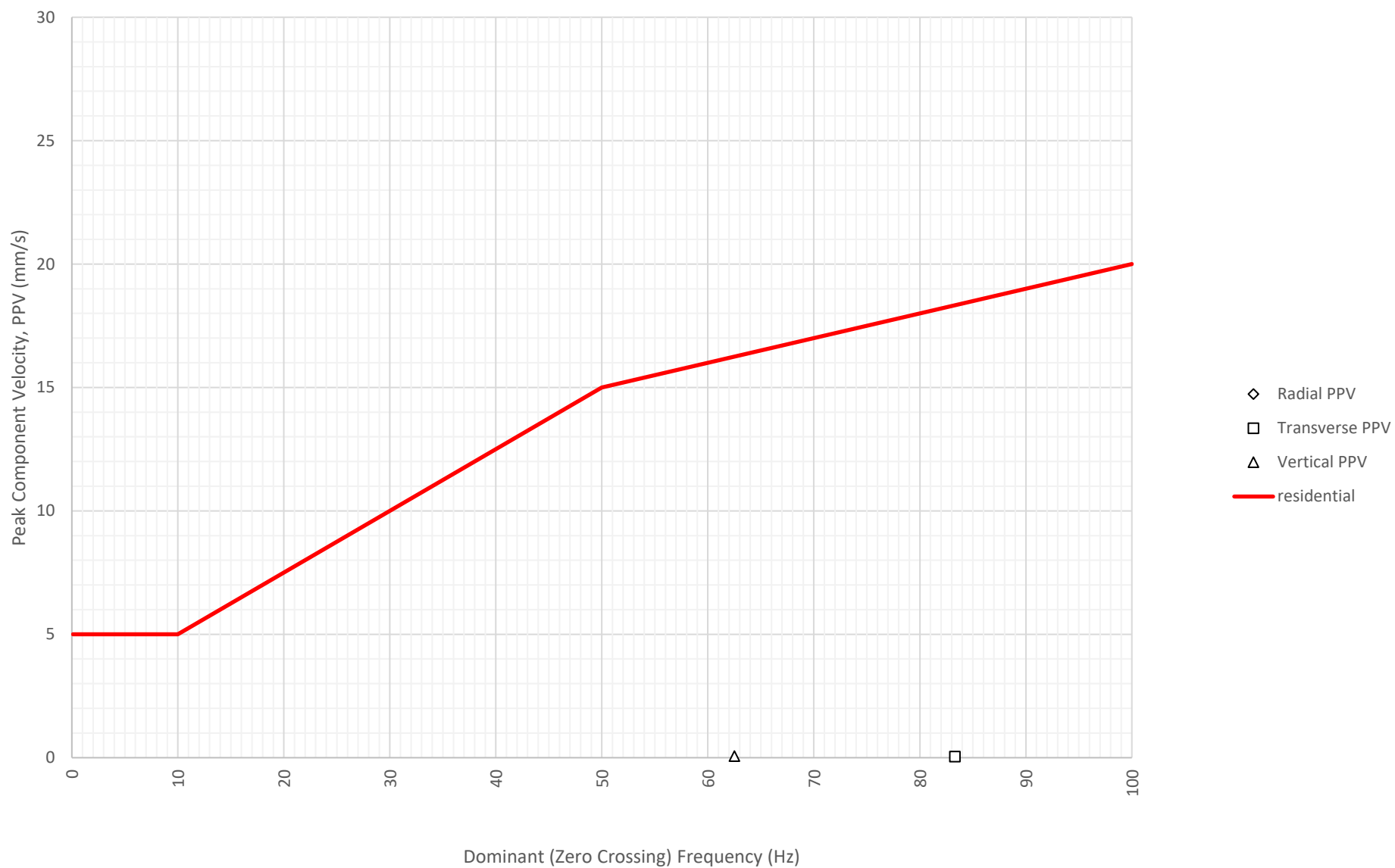
Frequency Content of Vibration Levels at East Boundary Opposite Shoalhaven Street (ETM7326) on 10-11-2024
