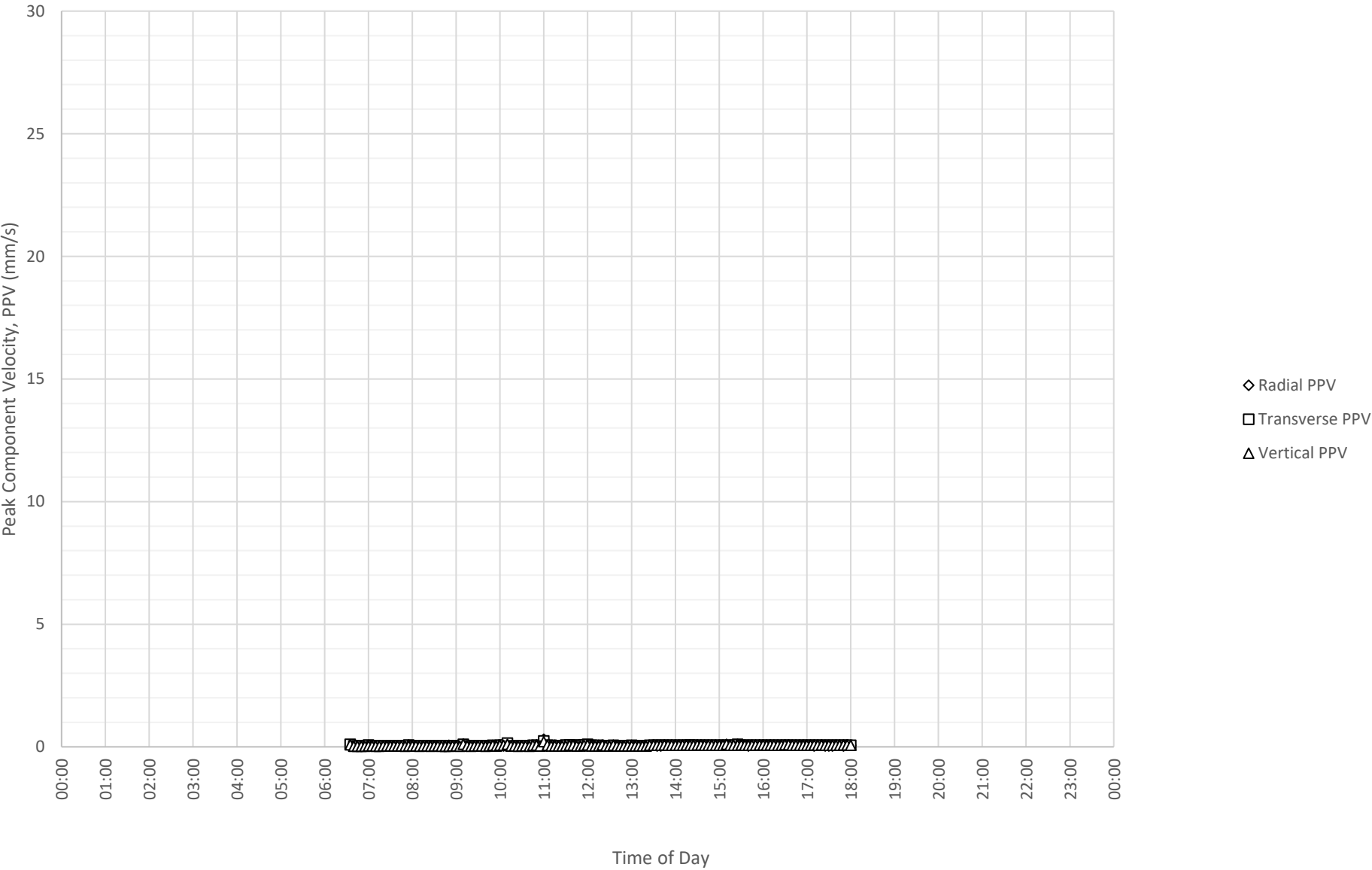
Daily Monitored Vibration Levels at North Boundary Near Block A and B (ETM7687) on 26-11-2024
