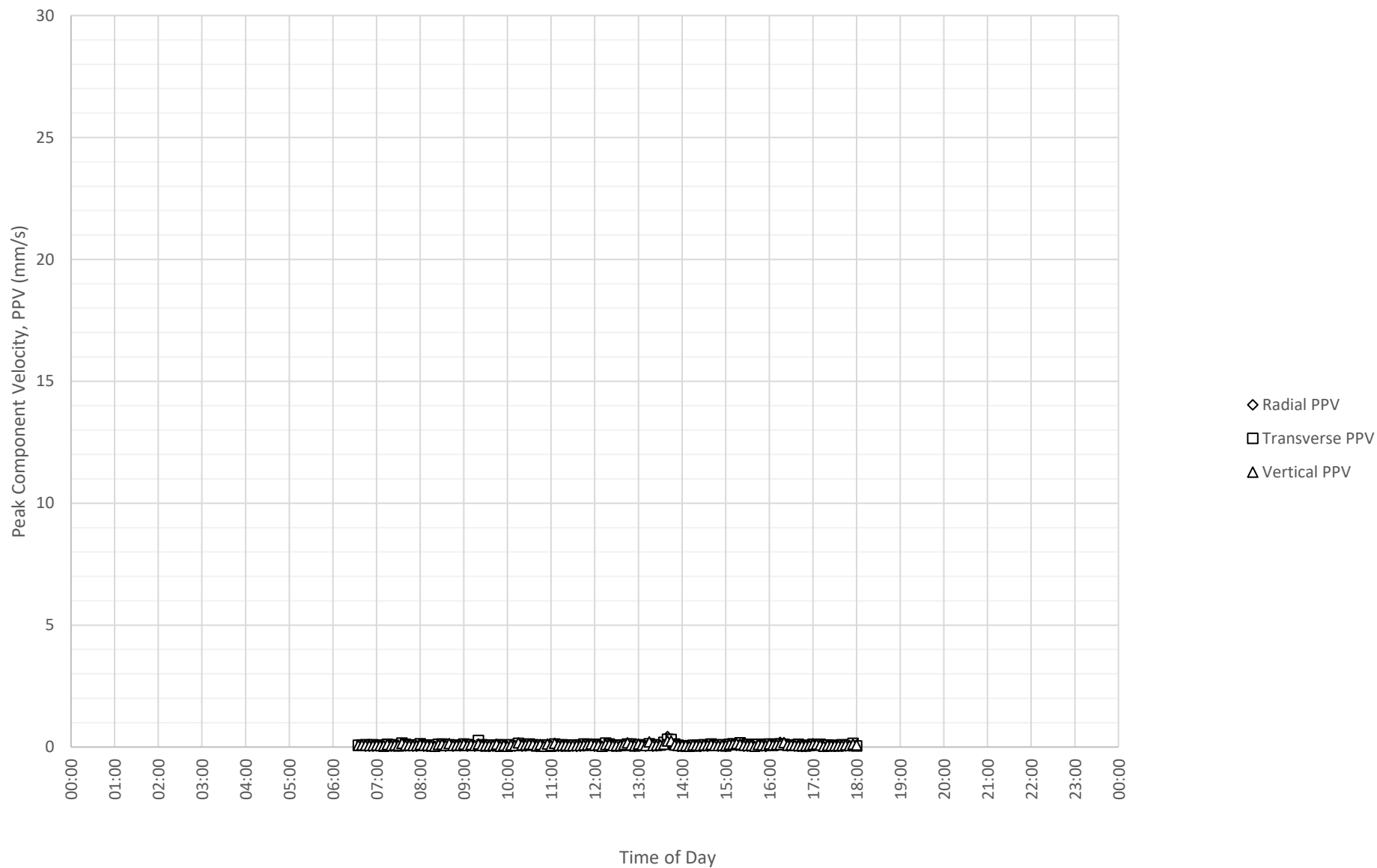
Daily Monitored Vibration Levels at East Boundary Opposite Shoalhaven Street (ETM7326) on 5-11-2024
