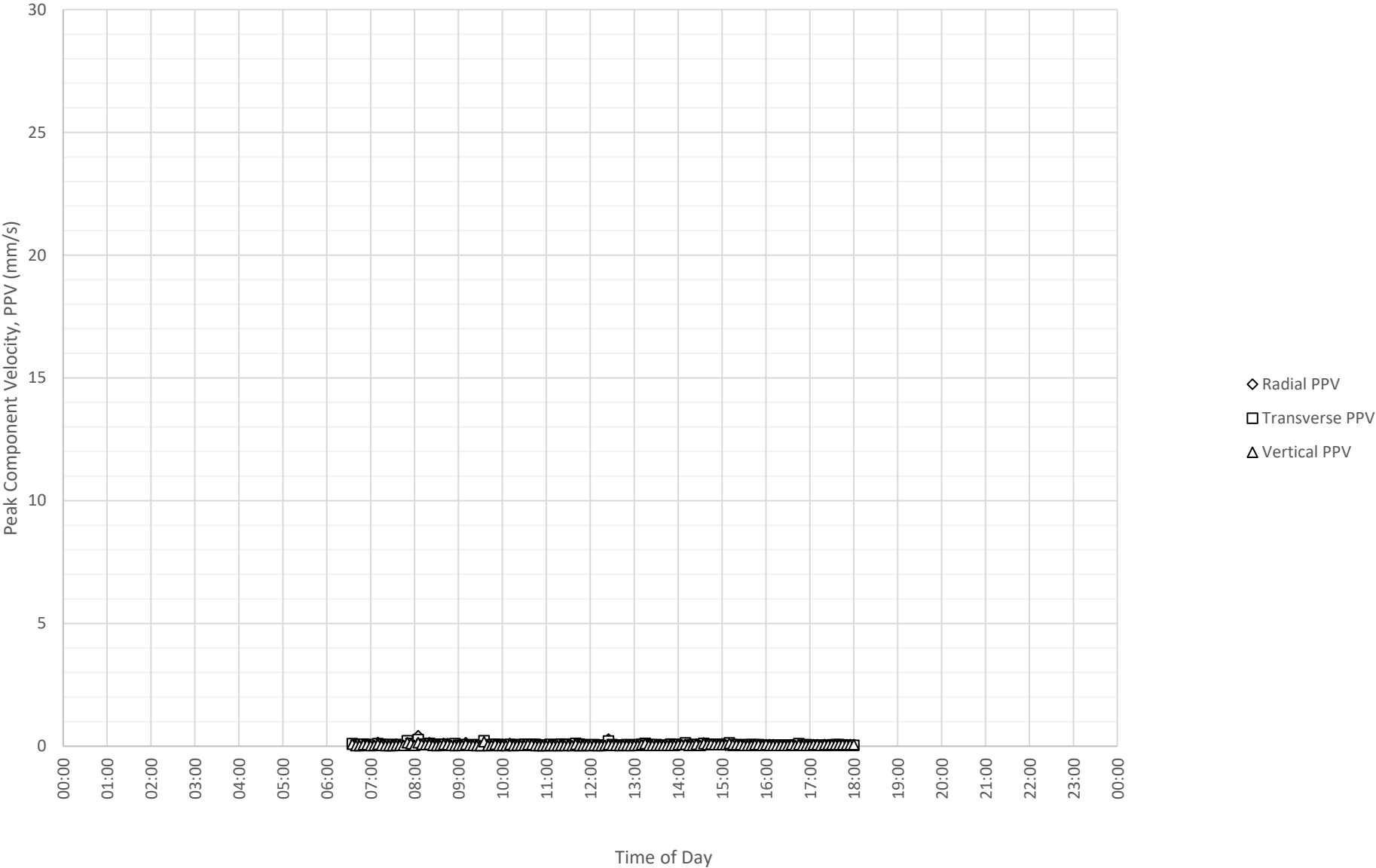
Daily Monitored Vibration Levels at North Boundary Near Block A and B (ETM7687) on 8-11-2024
