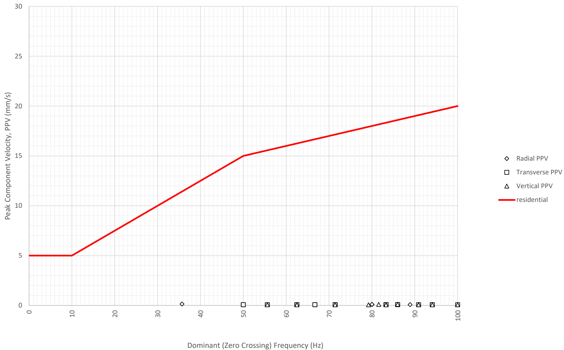
Frequency Content of Vibration Levels at North Boundary Near Block A and B (ETM7687) on 11-11-2024
