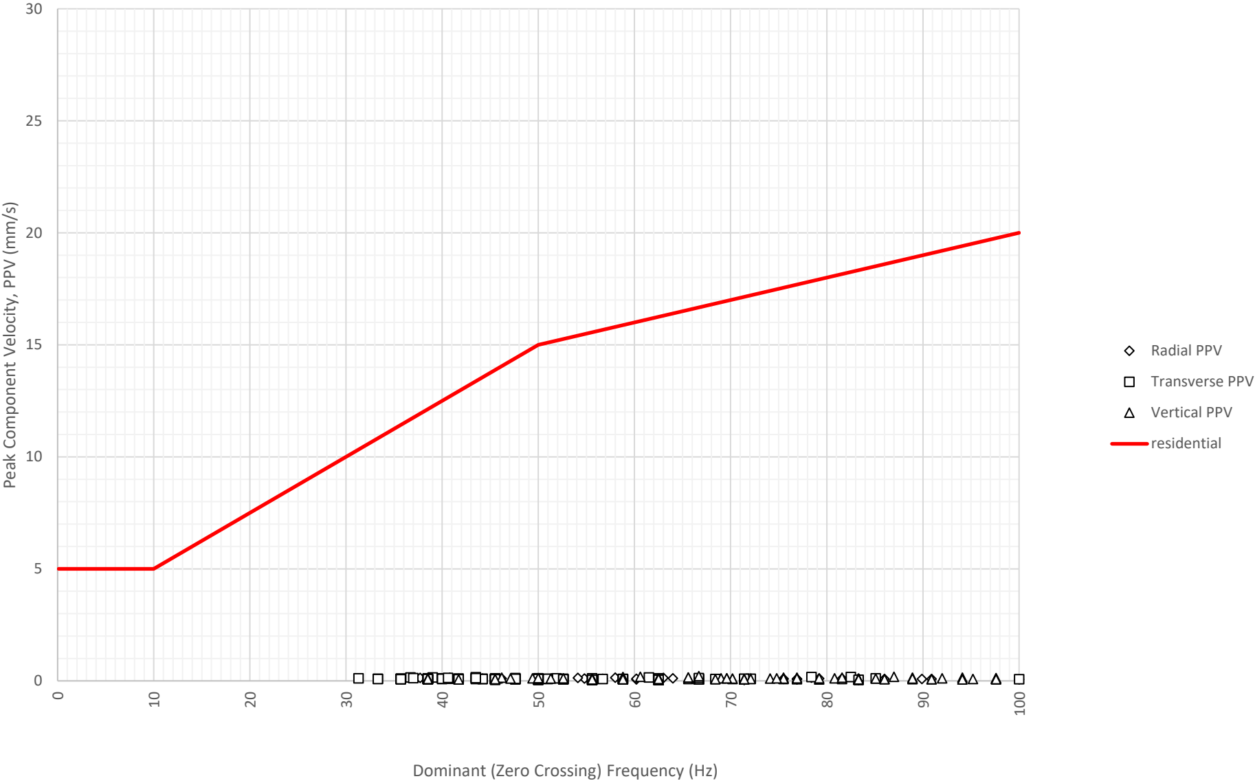
Frequency Content of Vibration Levels at East Boundary Opposite Shoalhaven Street (ETM7326) on 8-11-2024
