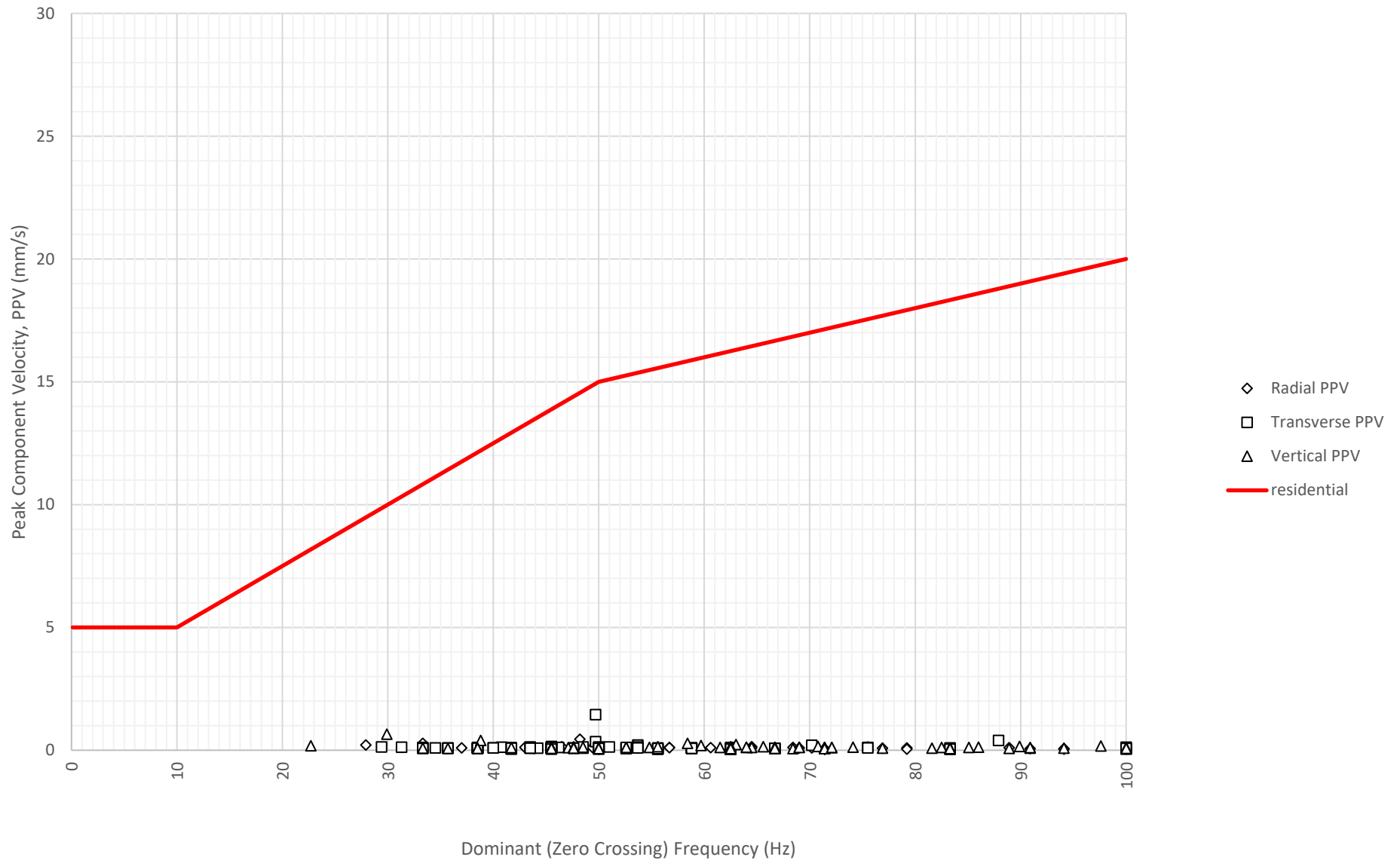
Frequency Content of Vibration Levels at East Boundary Opposite Shoalhaven Street (ETM7326) on 6-11-2024
