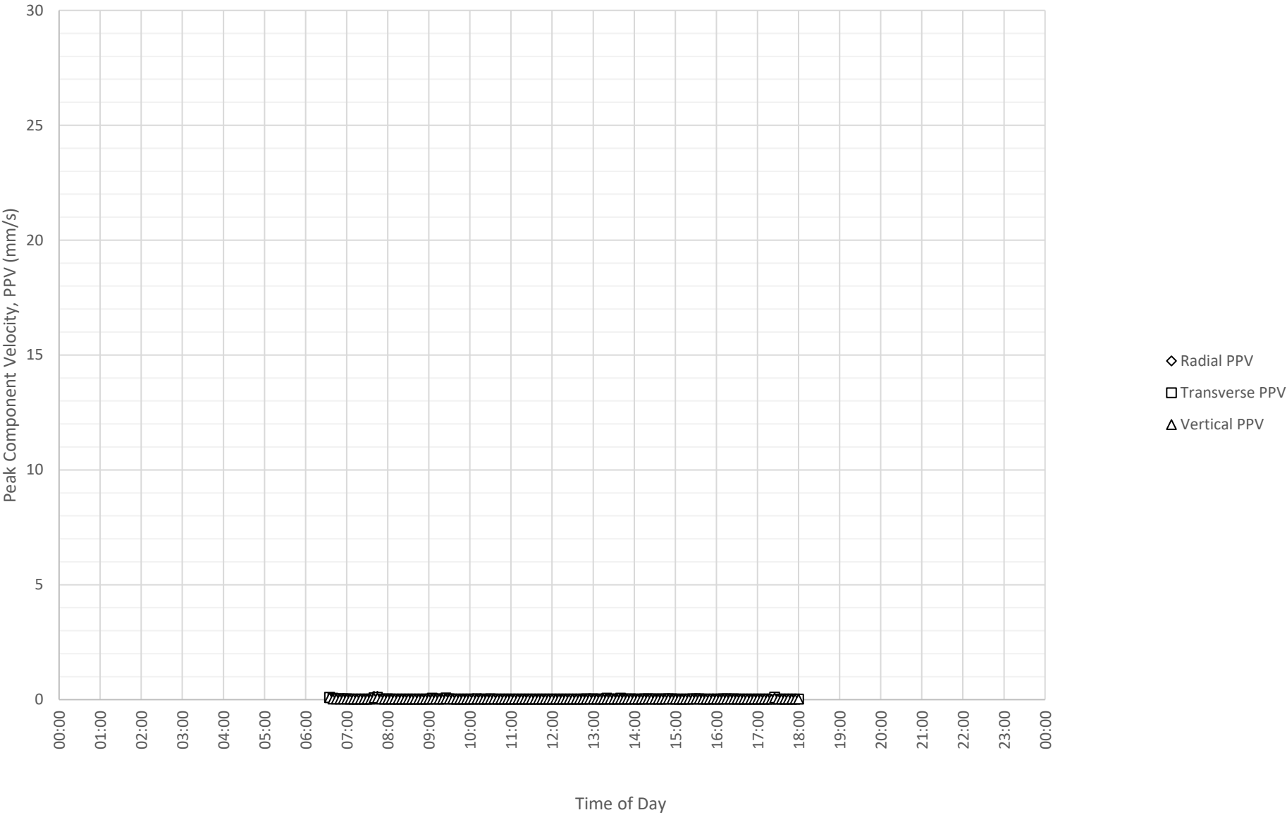
Daily Monitored Vibration Levels at North Boundary Near Block A and B (ETM7687) on 2-11-2024
