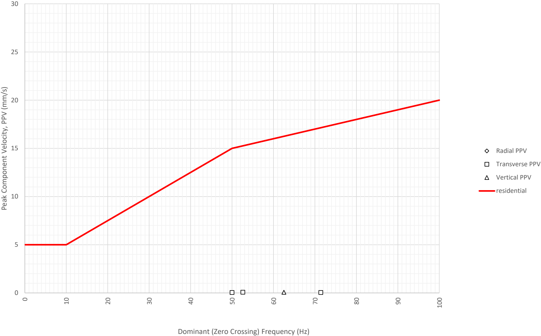
Frequency Content of Vibration Levels at East Boundary Opposite Shoalhaven Street (ETM7326) on 3-11-2024
