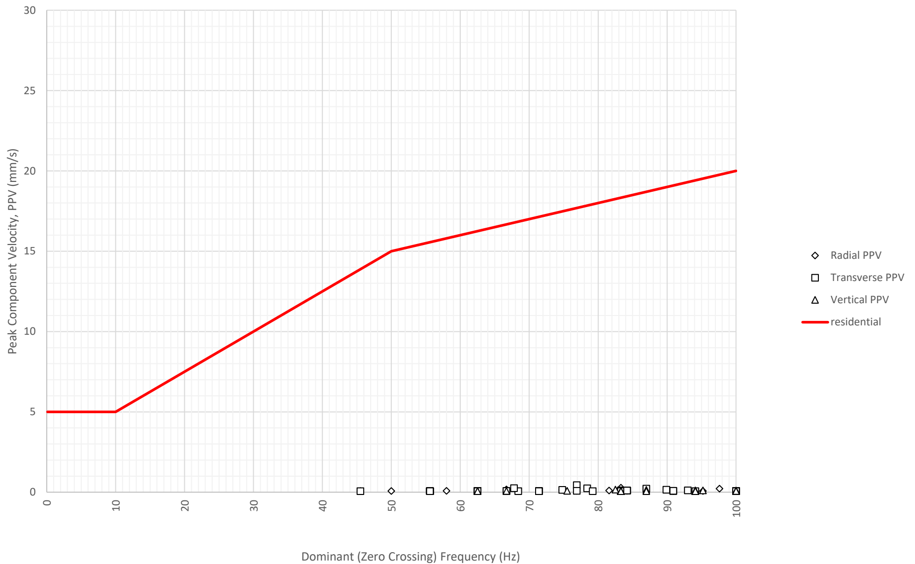
Frequency Content of Vibration Levels at North Boundary Near Block A and B (ETM7687) on 29-11-2024
