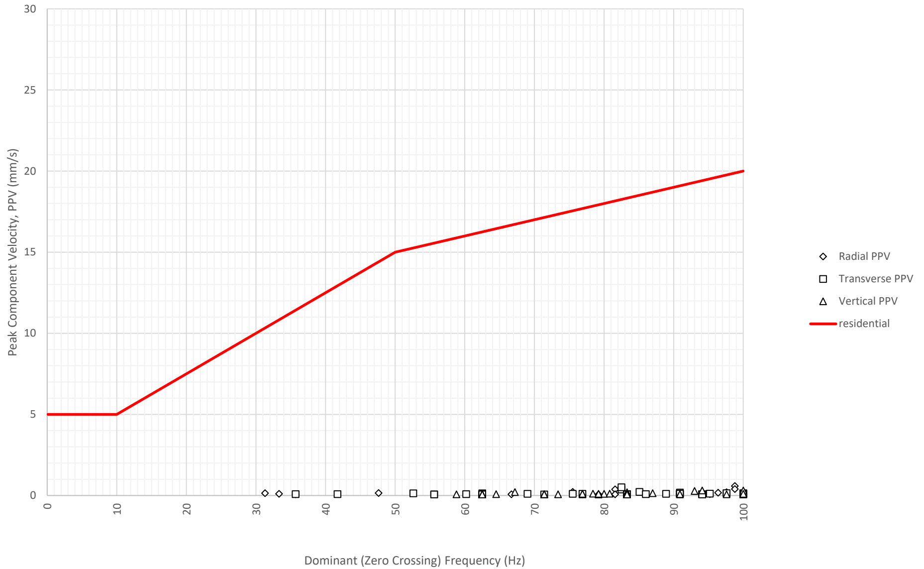
Frequency Content of Vibration Levels at North Boundary Near Block A and B (ETM7687) on 7-11-2024
