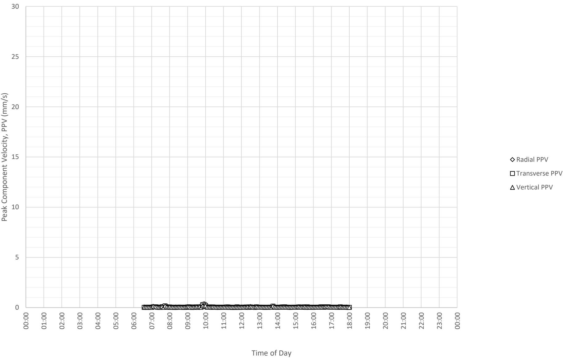
Daily Monitored Vibration Levels at North Boundary Near Block A and B (ETM7687) on 12-11-2024
