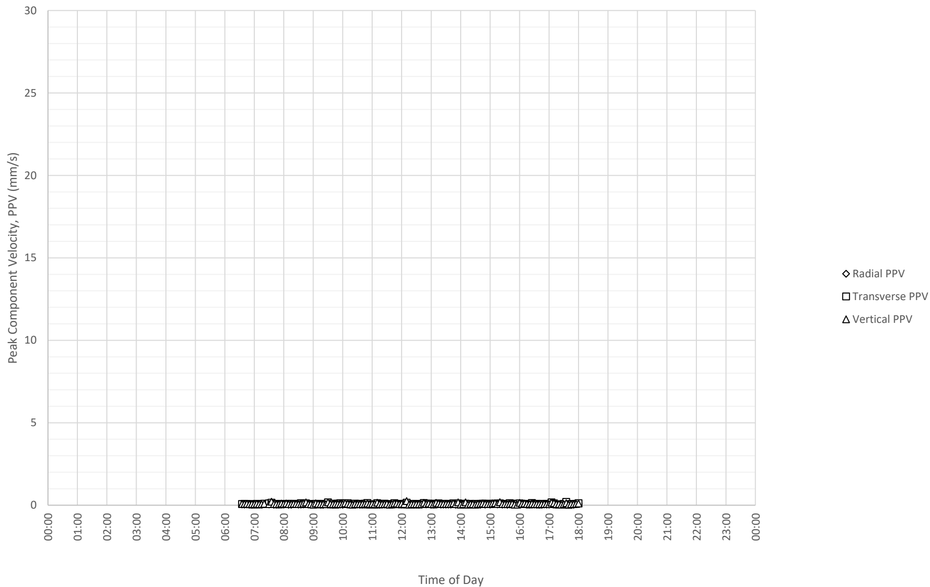
Daily Monitored Vibration Levels at East Boundary Opposite Shoalhaven Street (ETM7326) on 11-11-2024
