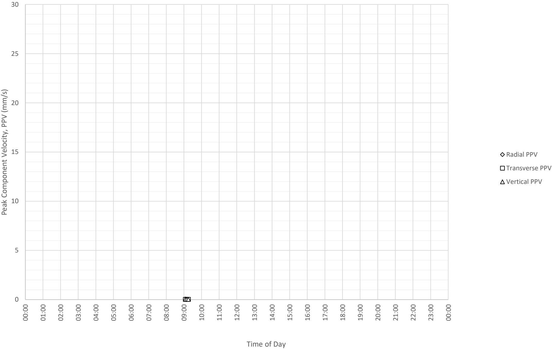
Daily Monitored Vibration Levels at North Boundary Near Block A and B (ETM7687) on 17-11-2024
