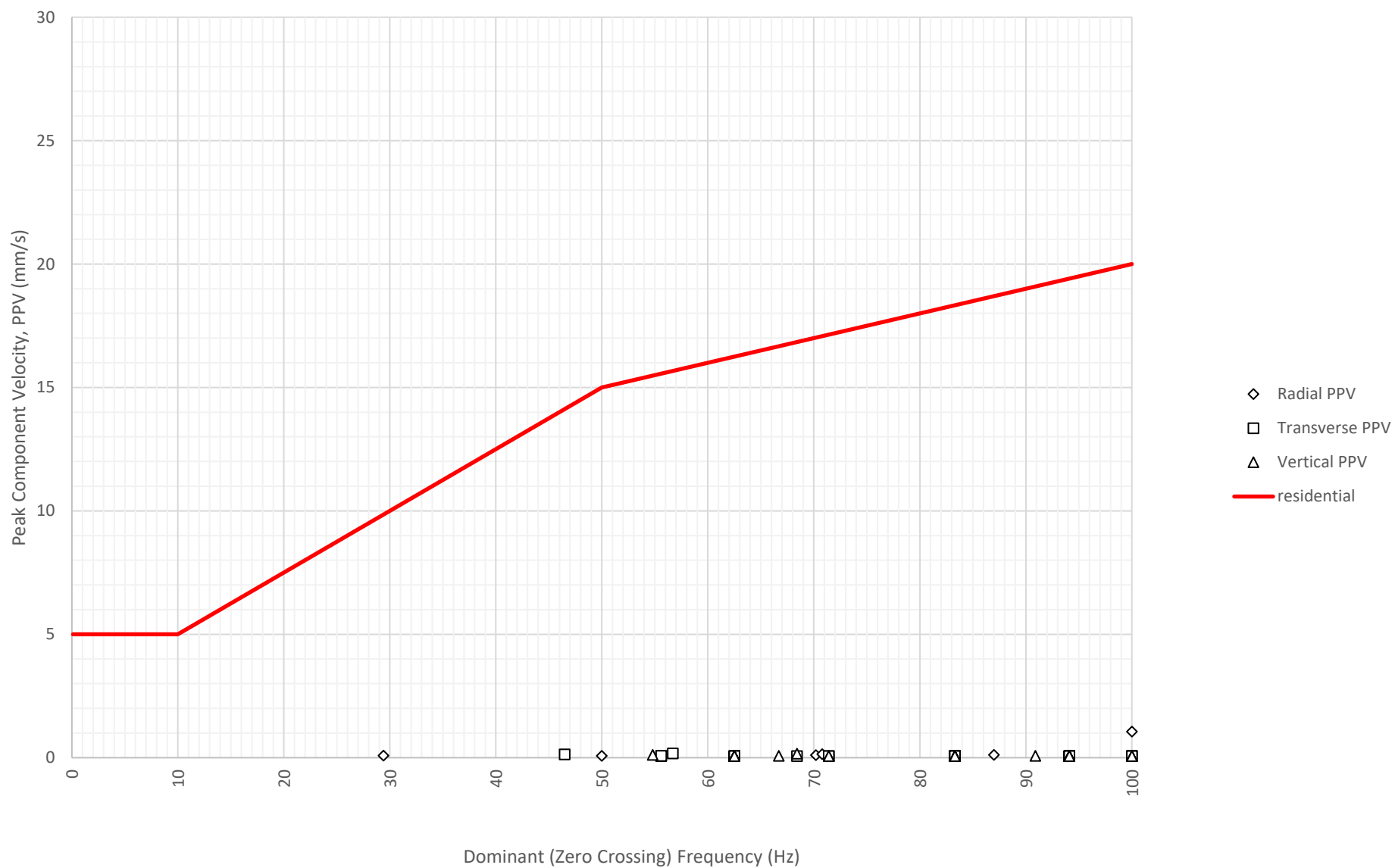
Frequency Content of Vibration Levels at North Boundary Near Block A and B (ETM7687) on 27-11-2024
