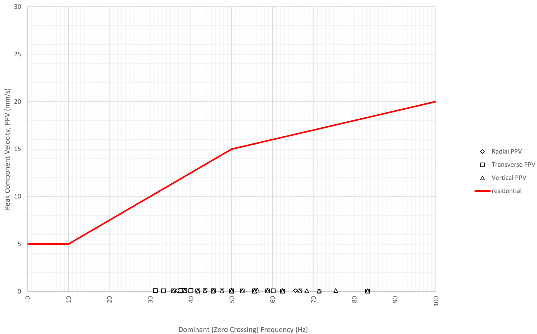
Frequency Content of Vibration Levels at East Boundary Opposite Shoalhaven Street (ETM7326) on 30-11-2024
