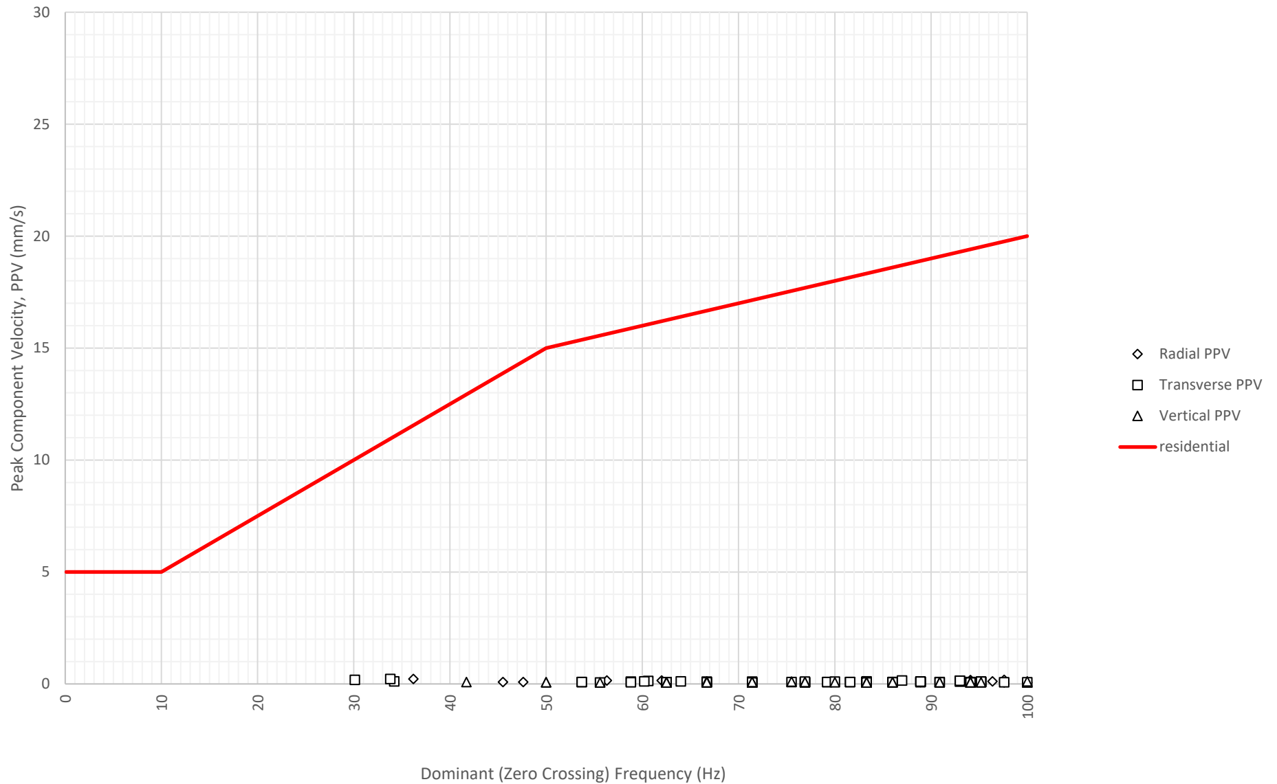
Frequency Content of Vibration Levels at North Boundary Near Block A and B (ETM7687) on 5-11-2024
