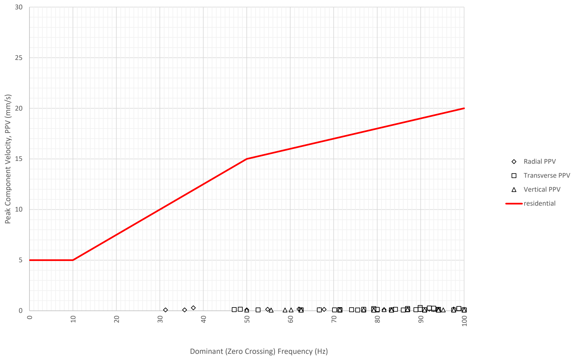
Frequency Content of Vibration Levels at North Boundary Near Block A and B (ETM7687) on 21-11-2024
