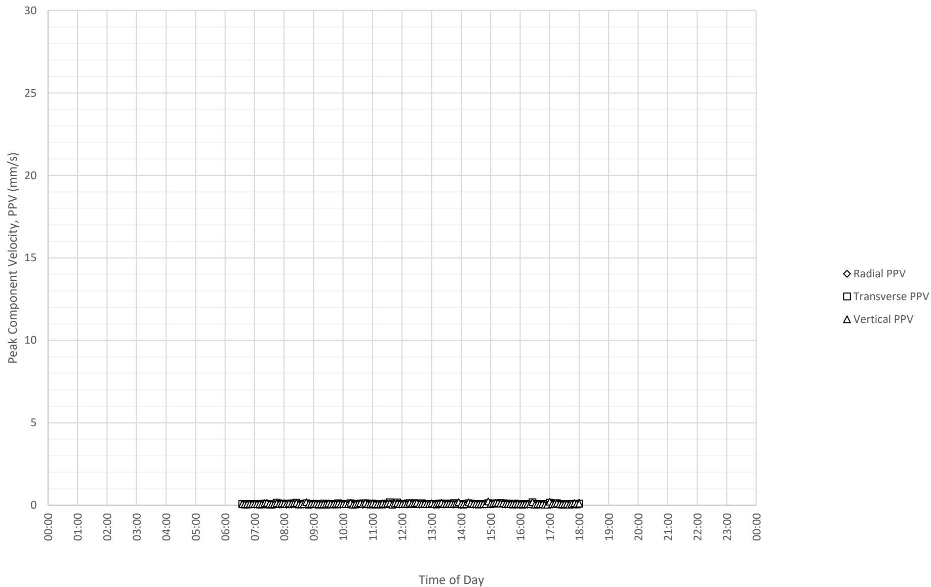
Daily Monitored Vibration Levels at East Boundary Opposite Shoalhaven Street (ETM7326) on 8-11-2024
