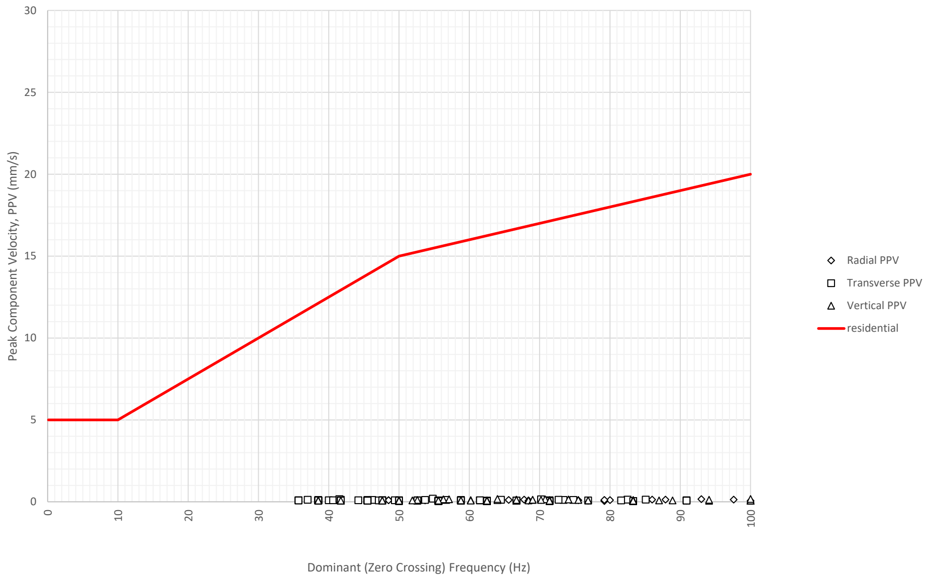
Frequency Content of Vibration Levels at East Boundary Opposite Shoalhaven Street (ETM7326) on 2-11-2024
