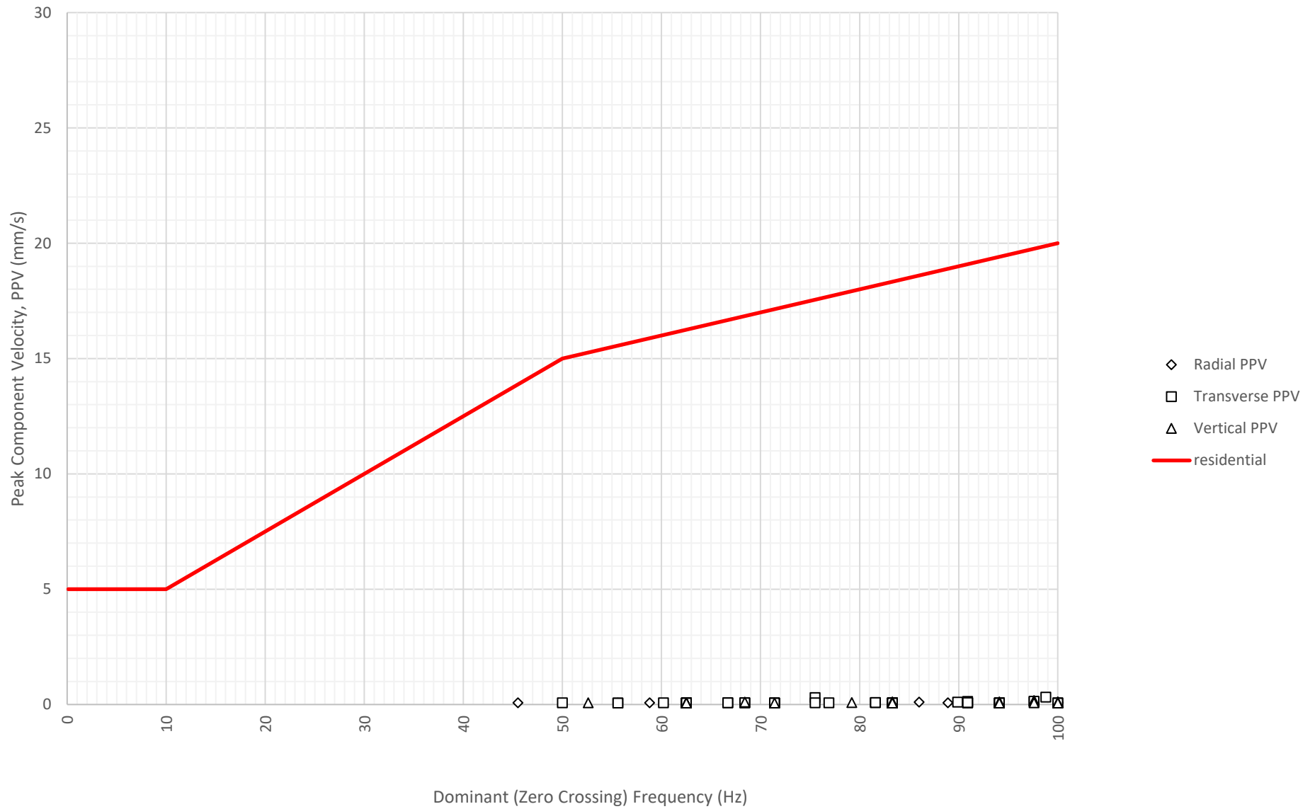
Frequency Content of Vibration Levels at North Boundary Near Block A and B (ETM7687) on 6-11-2024
