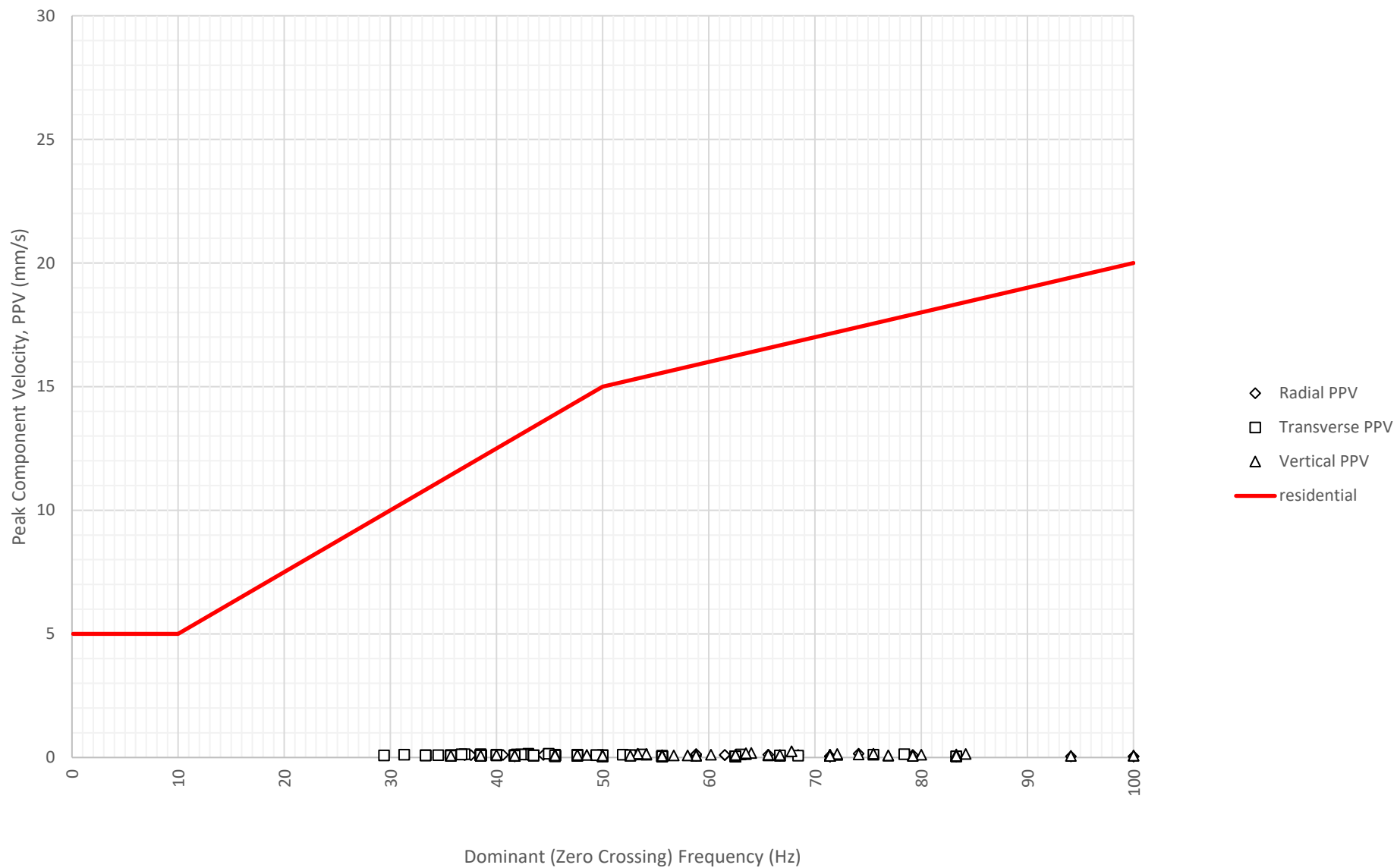
Frequency Content of Vibration Levels at East Boundary Opposite Shoalhaven Street (ETM7326) on 26-11-2024
