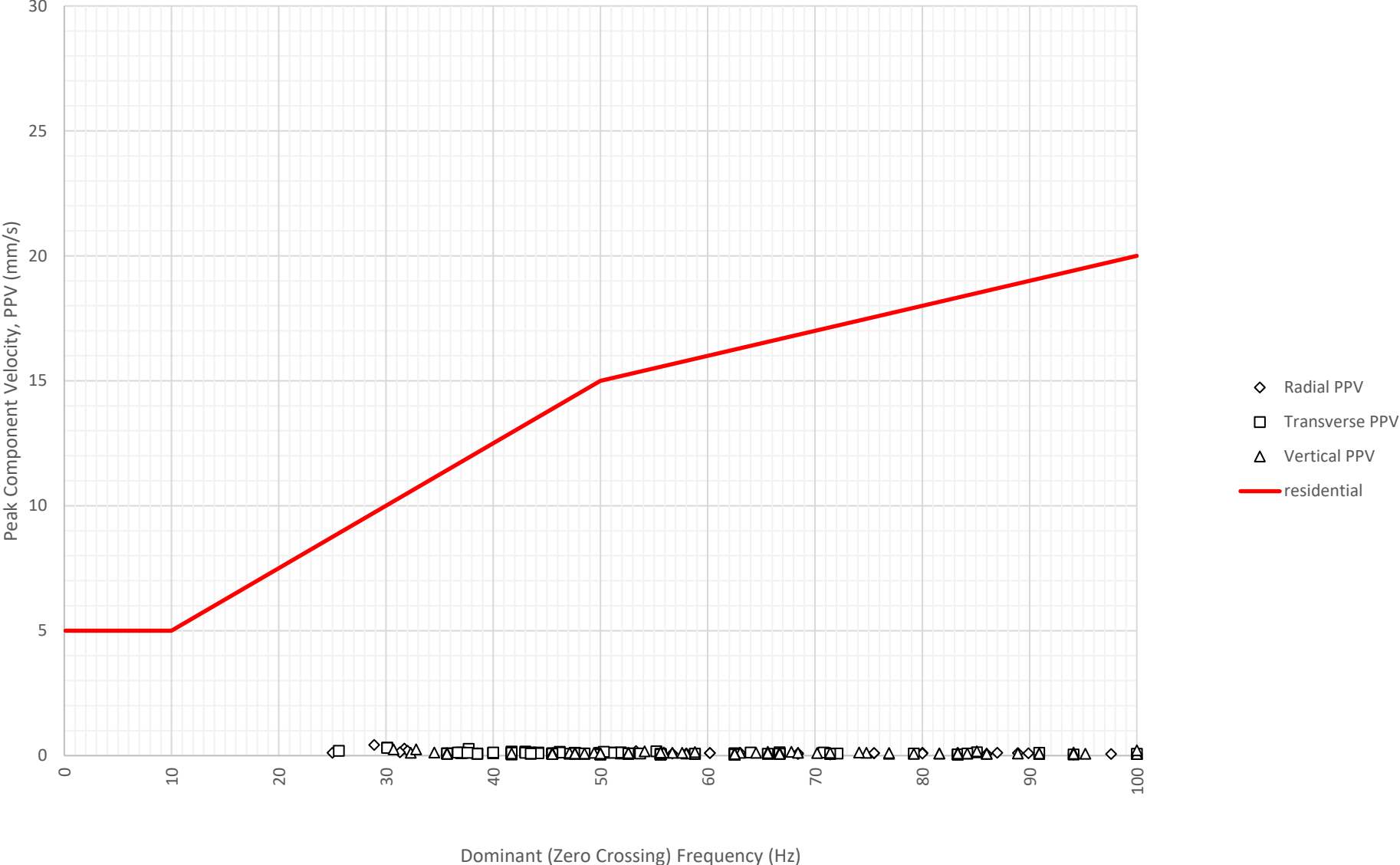
Frequency Content of Vibration Levels at East Boundary Opposite Shoalhaven Street (ETM7326) on 5-11-2024
