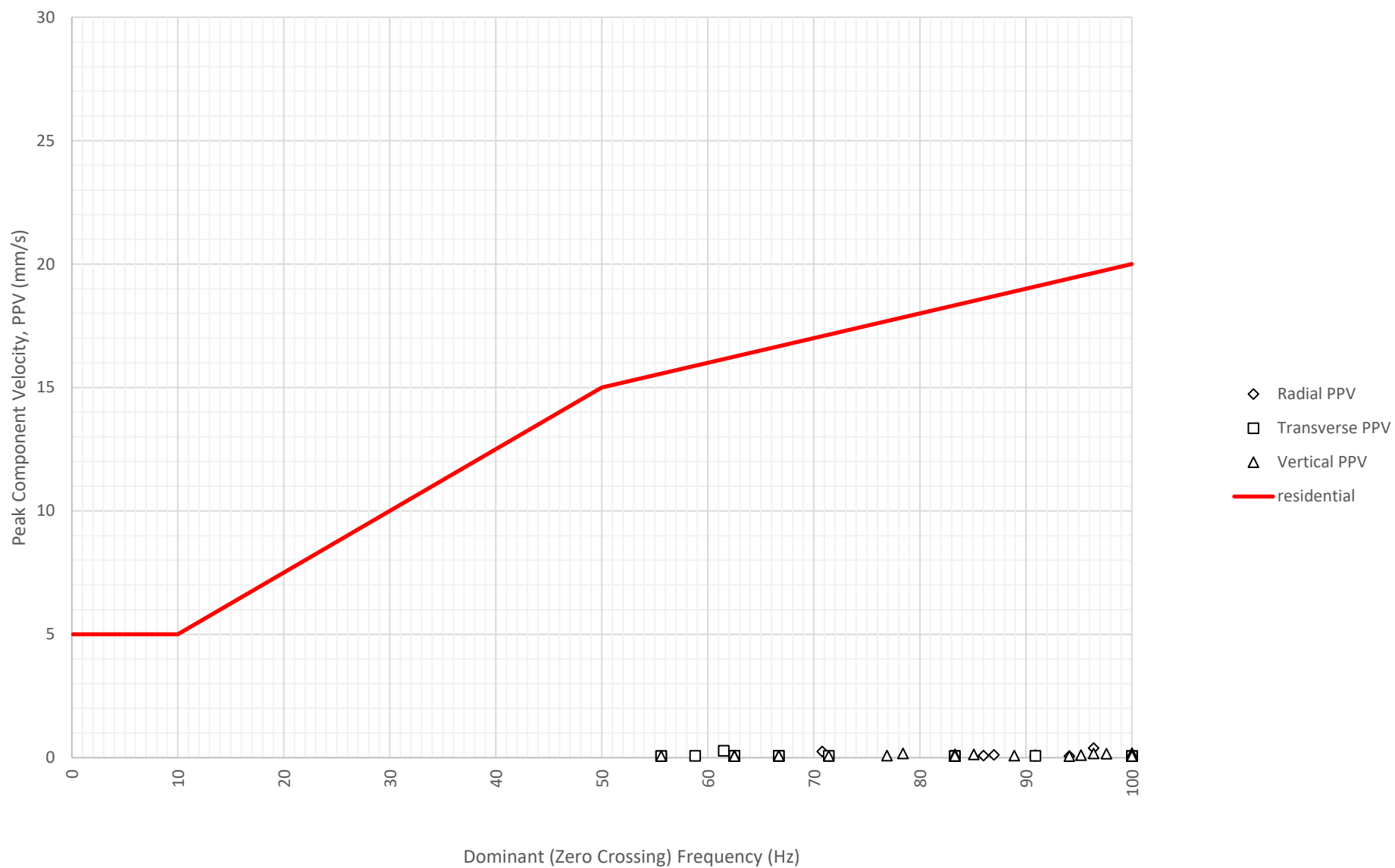
Frequency Content of Vibration Levels at North Boundary Near Block A and B (ETM7687) on 12-11-2024
