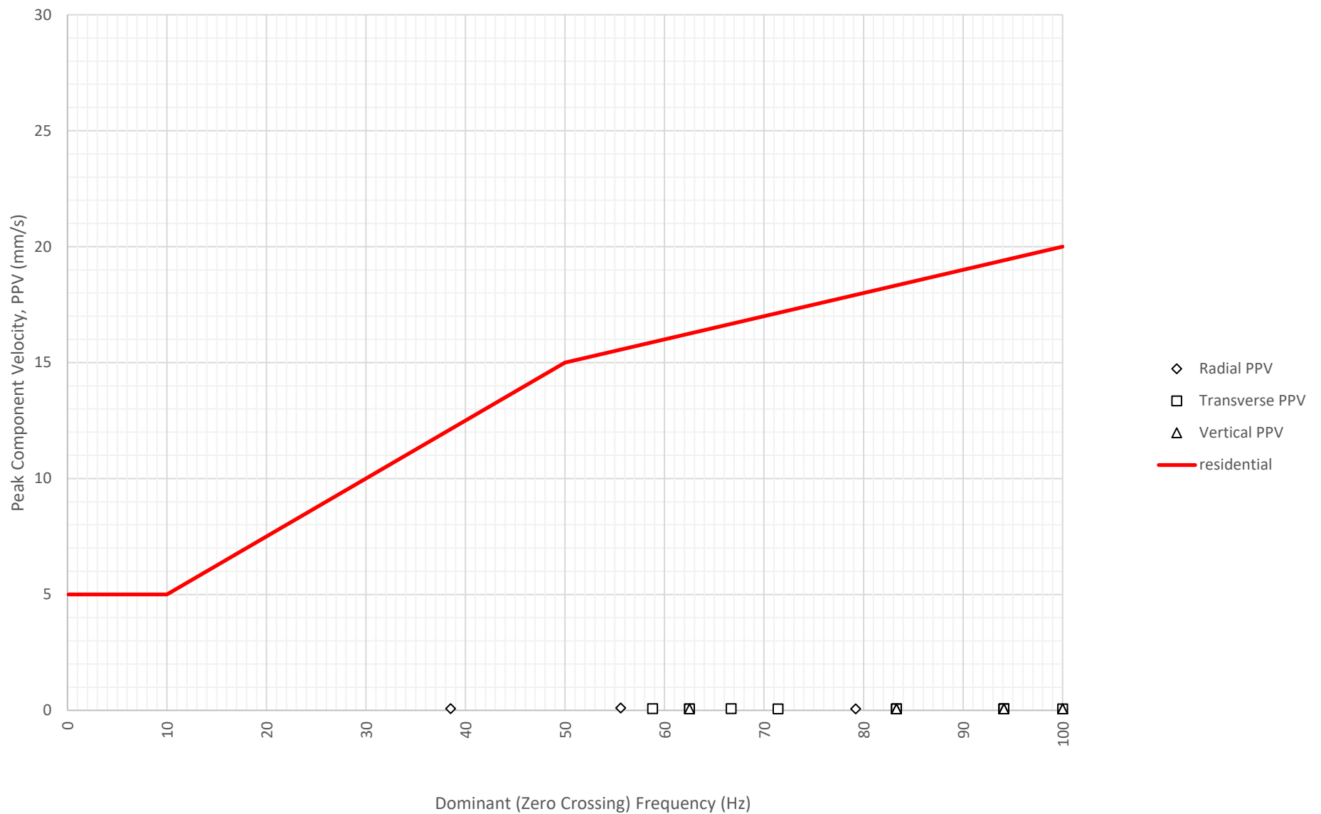
Frequency Content of Vibration Levels at North Boundary Near Block A and B (ETM7687) on 9-11-2024
