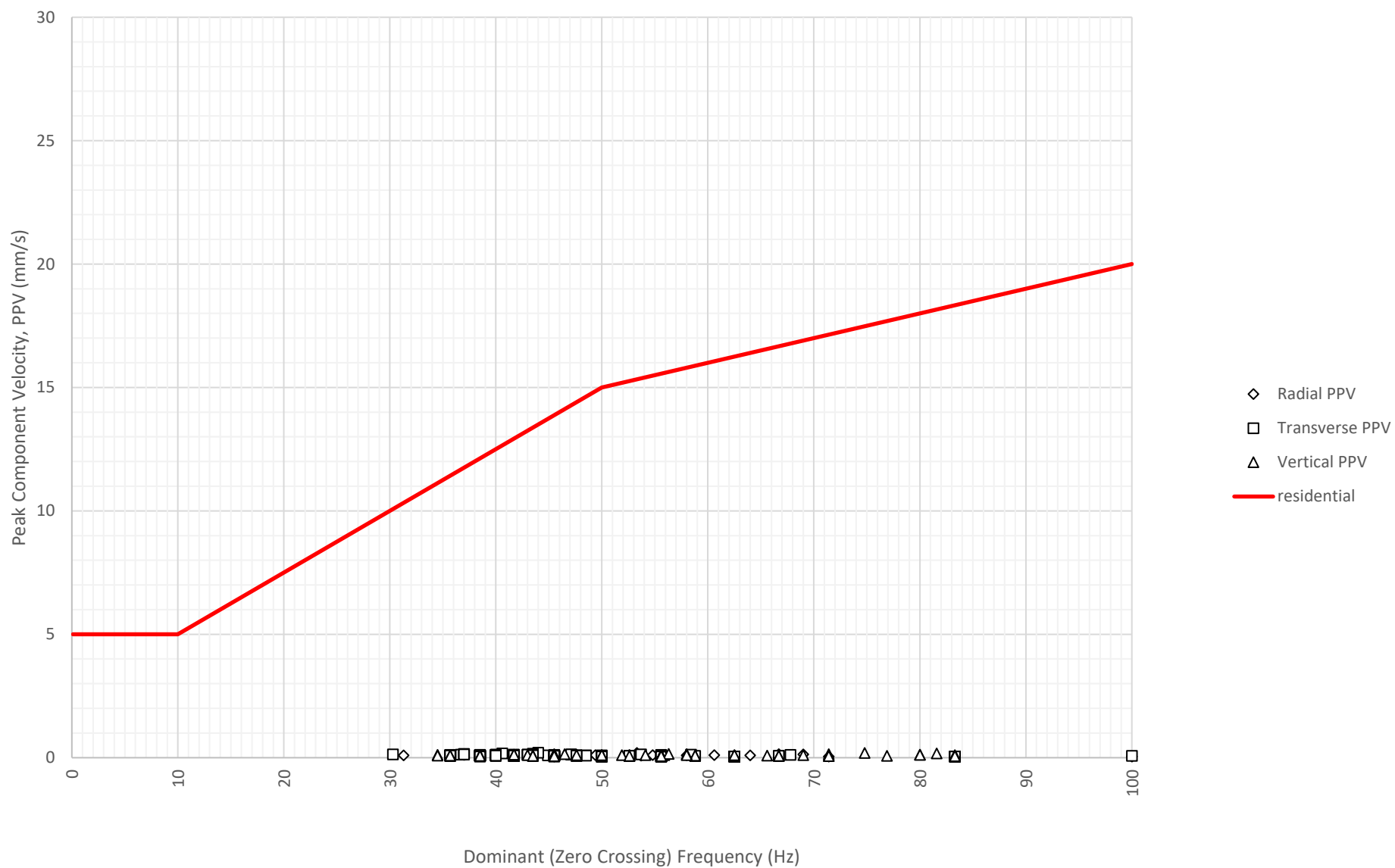
Frequency Content of Vibration Levels at East Boundary Opposite Shoalhaven Street (ETM7326) on 29-11-2024
