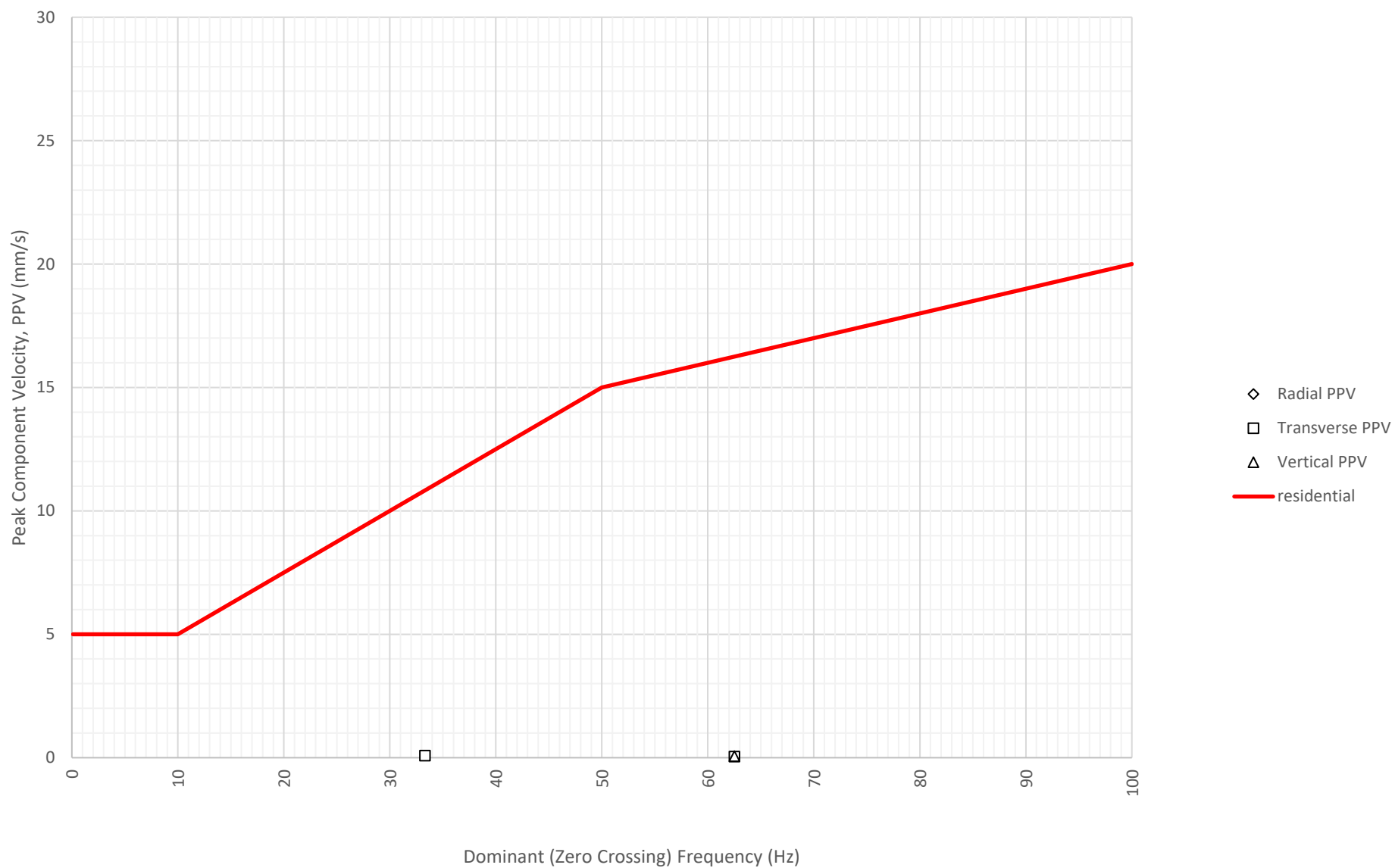
Frequency Content of Vibration Levels at East Boundary Opposite Shoalhaven Street (ETM7326) on 24-11-2024
