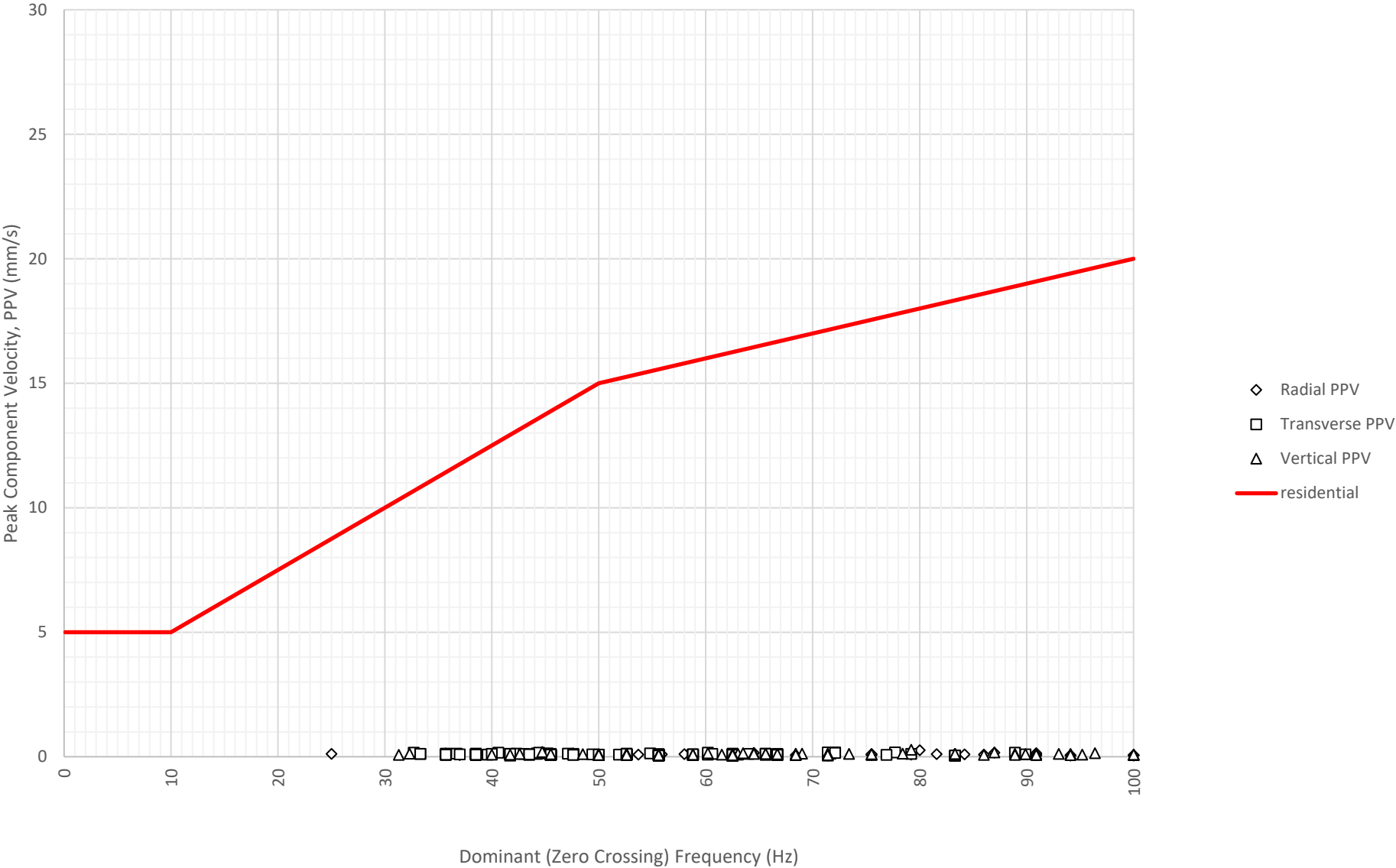
Frequency Content of Vibration Levels at East Boundary Opposite Shoalhaven Street (ETM7326) on 1-11-2024
