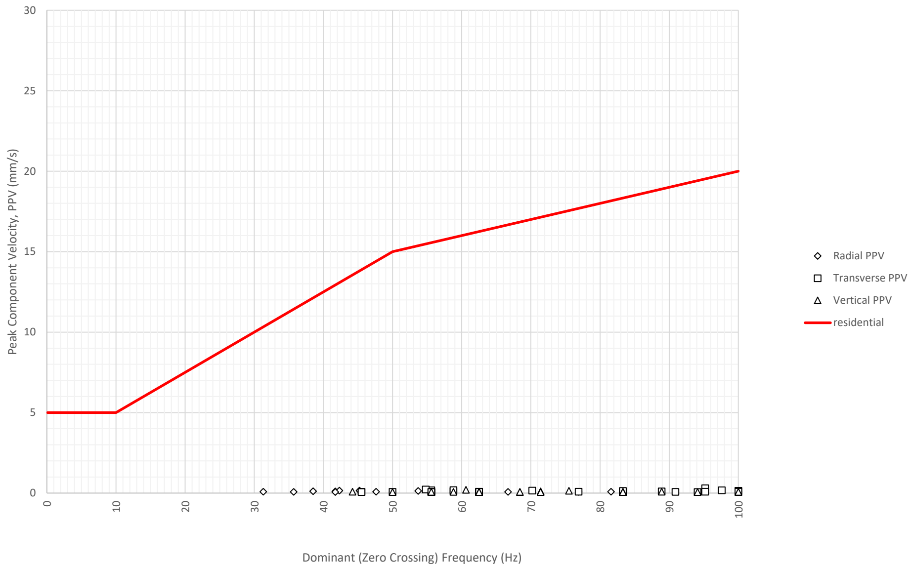
Frequency Content of Vibration Levels at North Boundary Near Block A and B (ETM7687) on 28-11-2024
