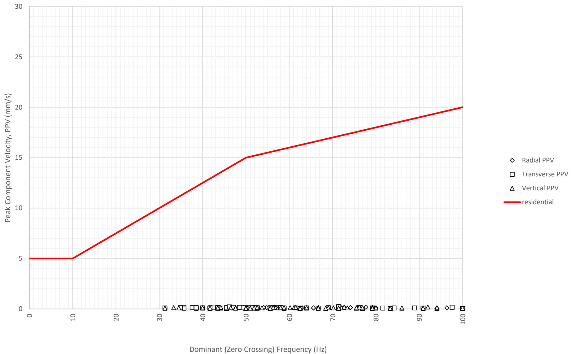
Frequency Content of Vibration Levels at East Boundary Opposite Shoalhaven Street (ETM7326) on 15-11-2024
