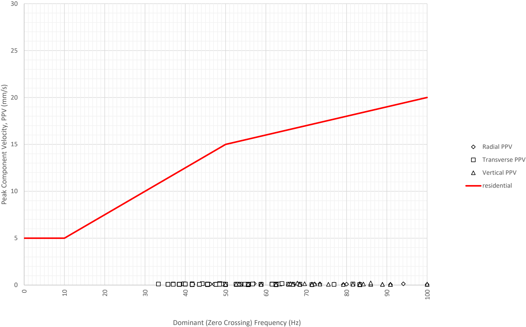
Frequency Content of Vibration Levels at East Boundary Opposite Shoalhaven Street (ETM7326) on 9-11-2024
