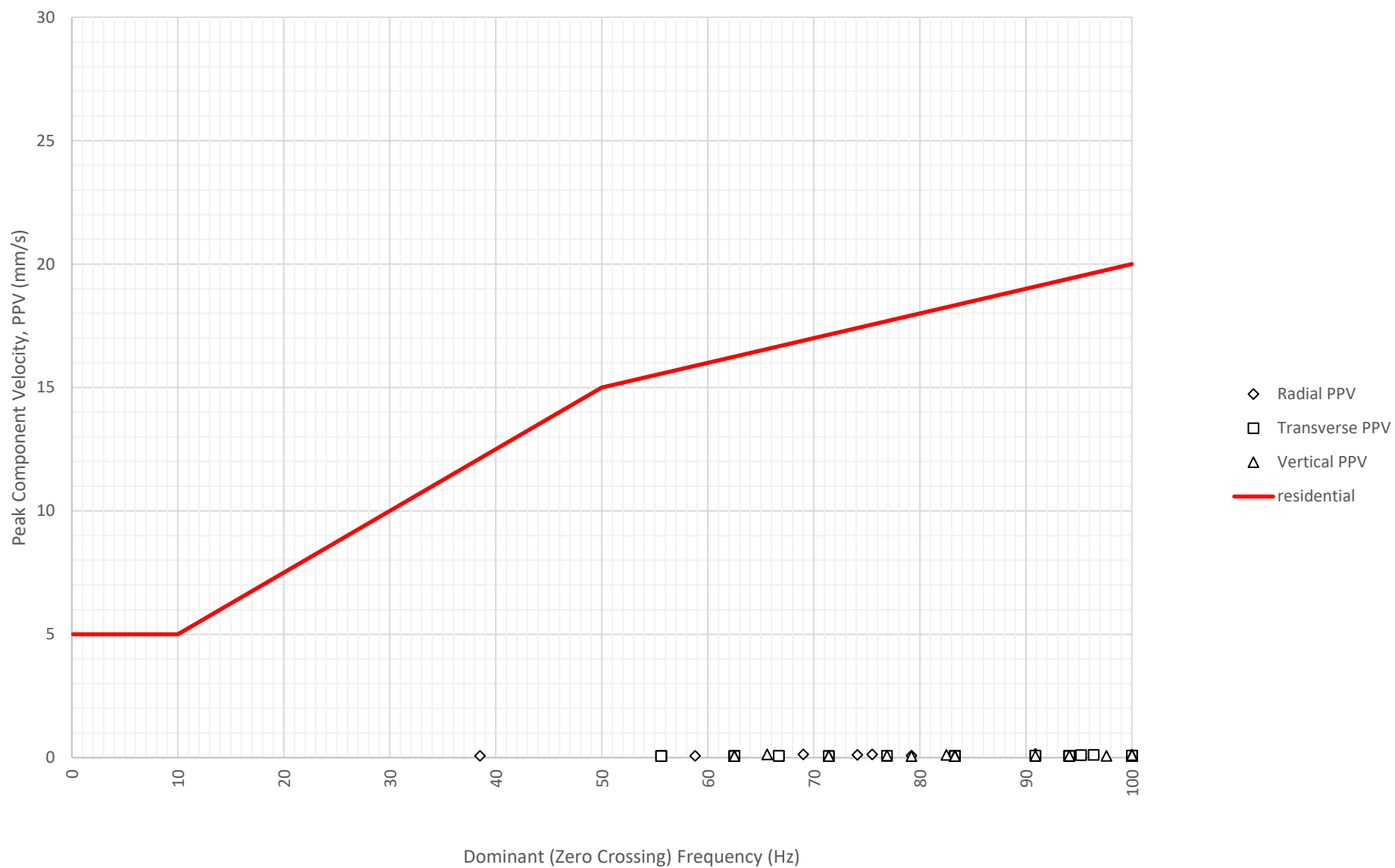
Frequency Content of Vibration Levels at North Boundary Near Block A and B (ETM7687) on 15-11-2024
