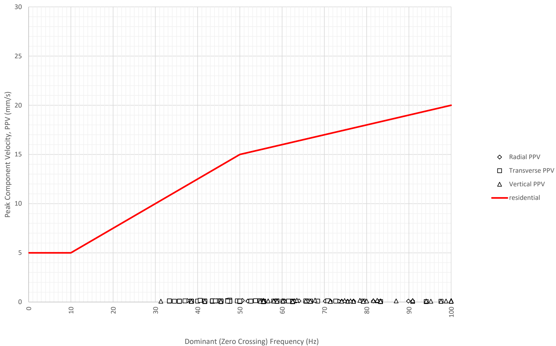
Frequency Content of Vibration Levels at East Boundary Opposite Shoalhaven Street (ETM7326) on 12-11-2024
