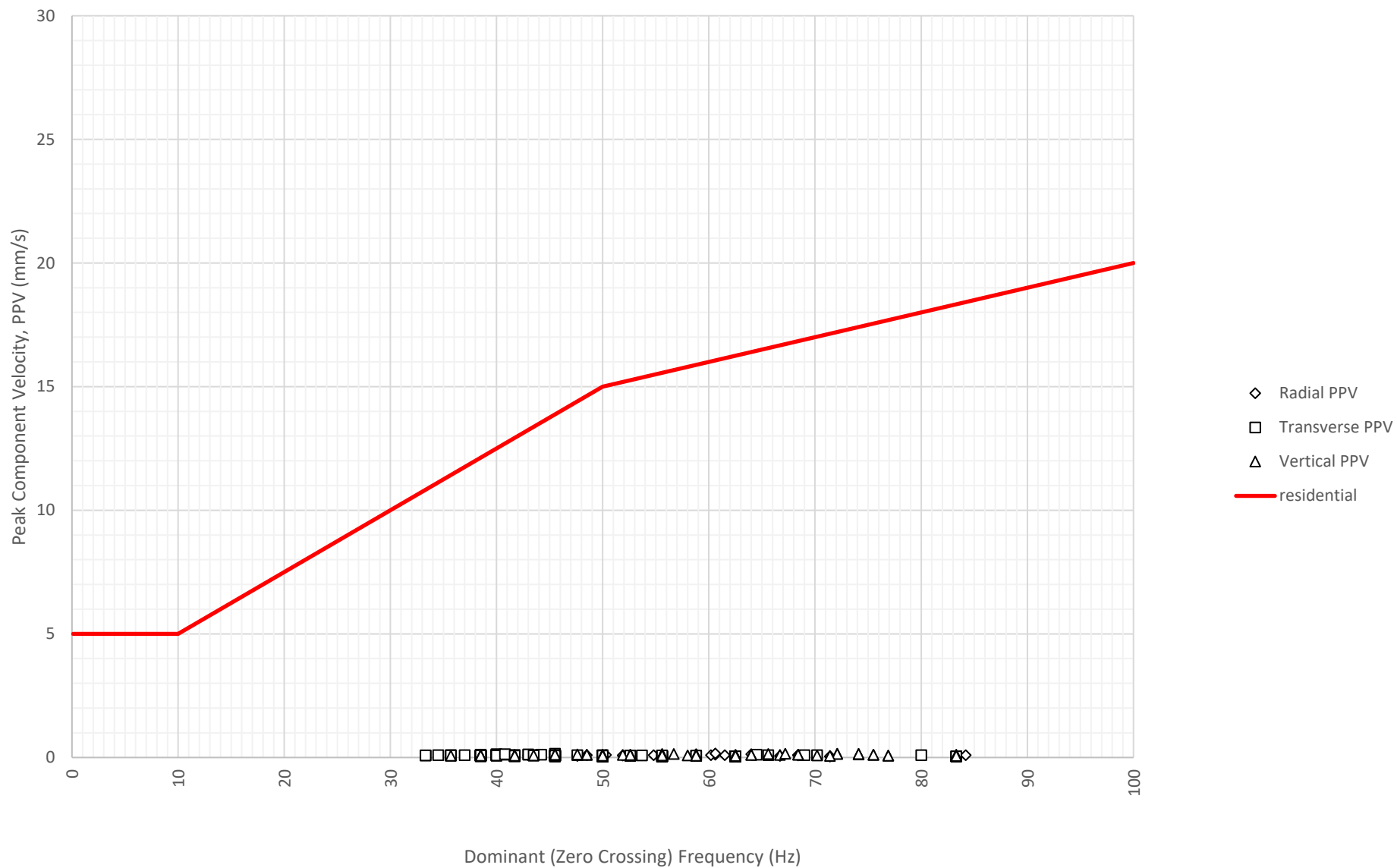
Frequency Content of Vibration Levels at East Boundary Opposite Shoalhaven Street (ETM7326) on 22-11-2024
