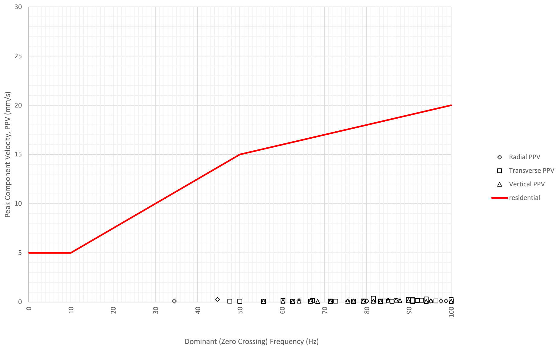
Frequency Content of Vibration Levels at North Boundary Near Block A and B (ETM7687) on 20-11-2024
