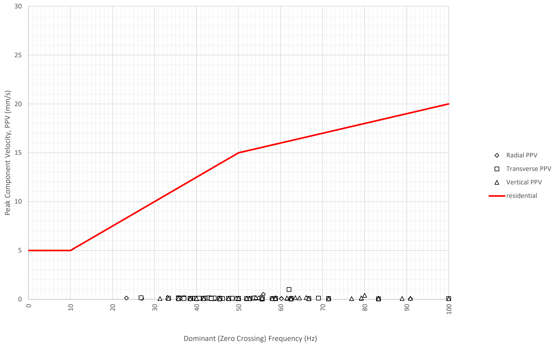
Frequency Content of Vibration Levels at East Boundary Opposite Shoalhaven Street (ETM7326) on 18-11-2024
