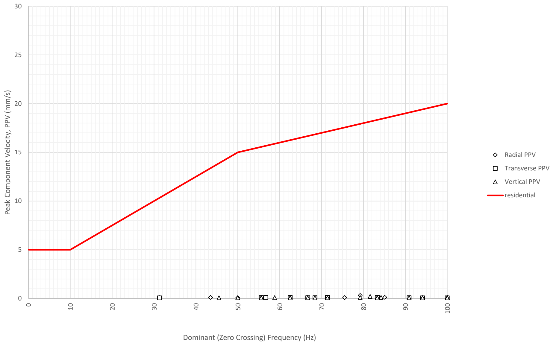
Frequency Content of Vibration Levels at North Boundary Near Block A and B (ETM7687) on 26-11-2024
