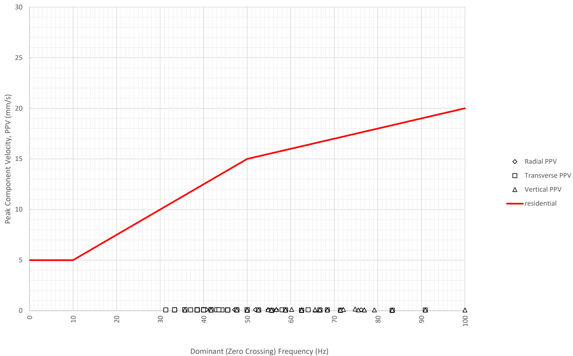
Frequency Content of Vibration Levels at East Boundary Opposite Shoalhaven Street (ETM7326) on 23-11-2024
