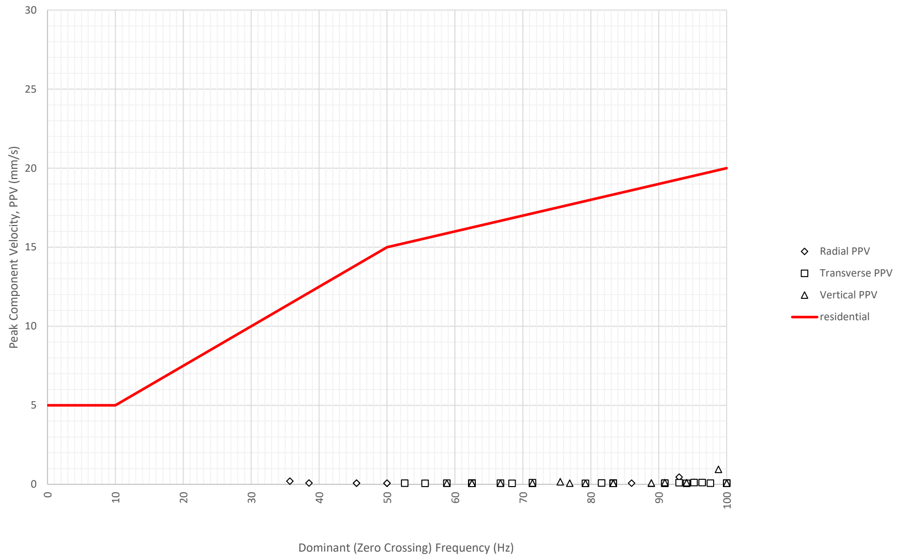
Frequency Content of Vibration Levels at North Boundary Near Block A and B (ETM7687) on 14-11-2024
