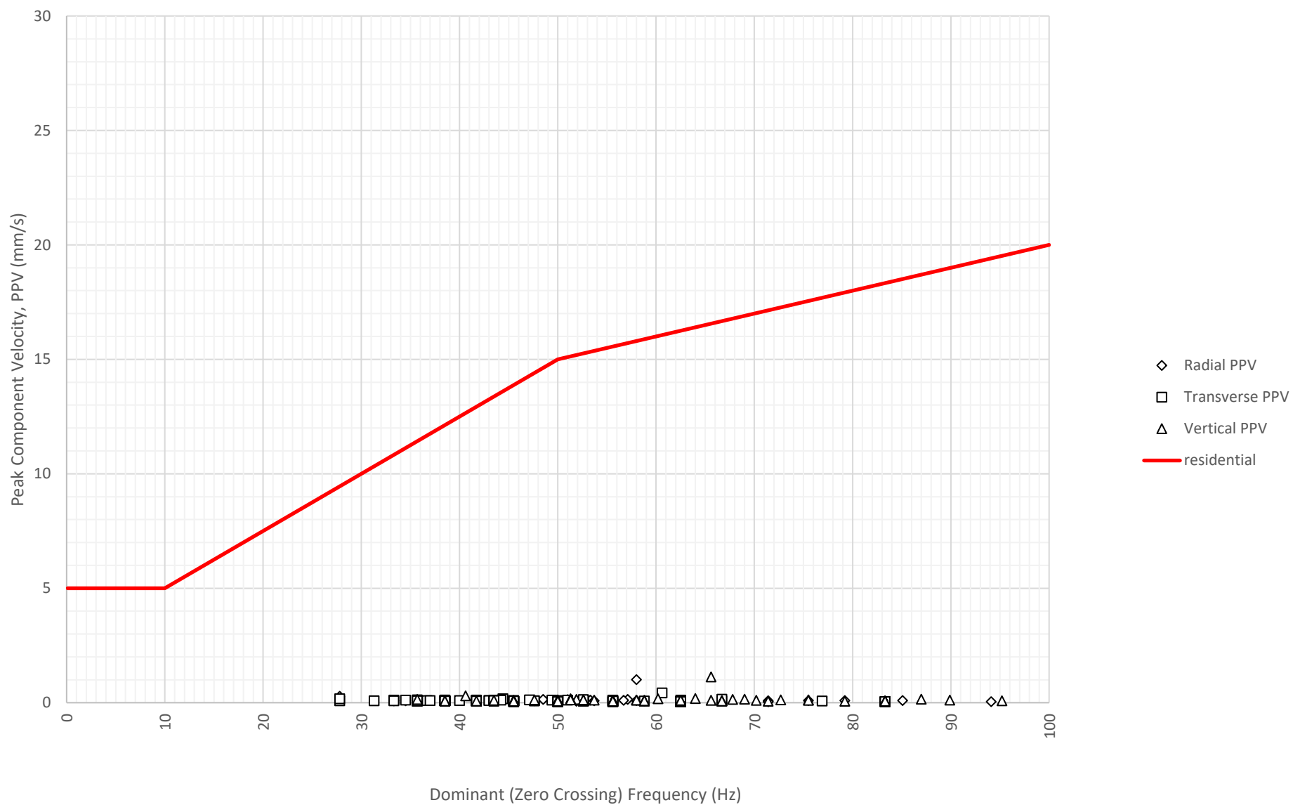
Frequency Content of Vibration Levels at East Boundary Opposite Shoalhaven Street (ETM7326) on 21-11-2024
