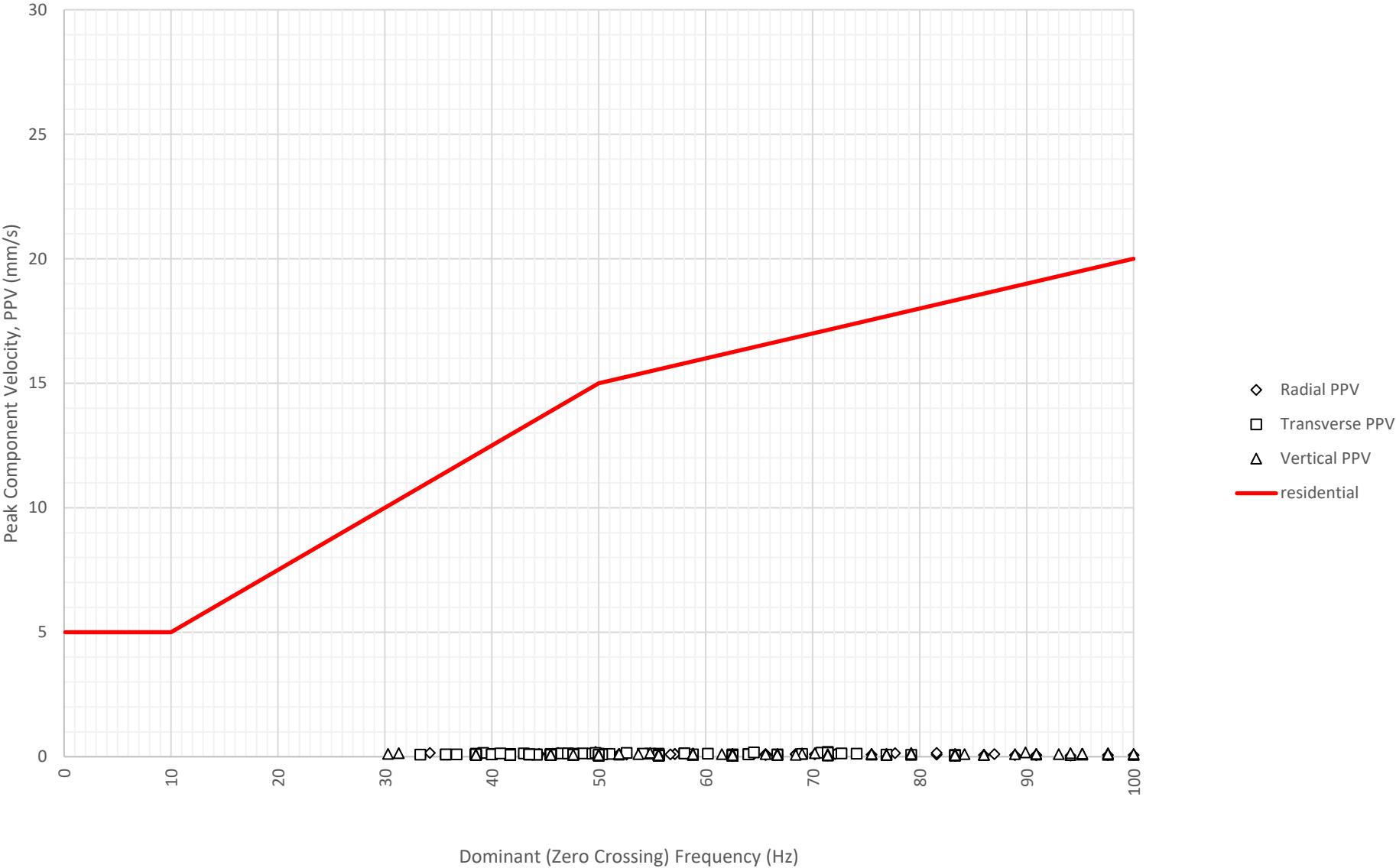
Frequency Content of Vibration Levels at East Boundary Opposite Shoalhaven Street (ETM7326) on 7-11-2024
