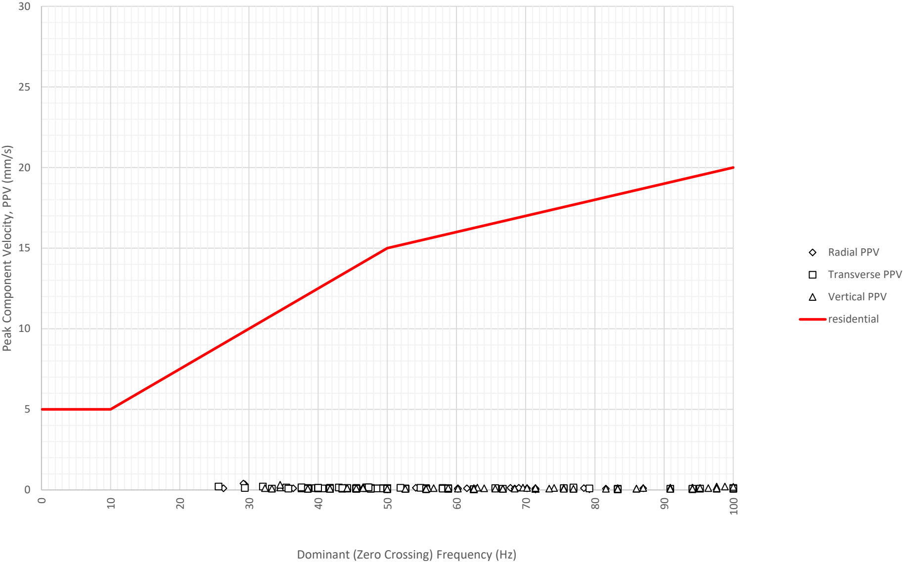
Frequency Content of Vibration Levels at East Boundary Opposite Shoalhaven Street (ETM7326) on 4-11-2024
