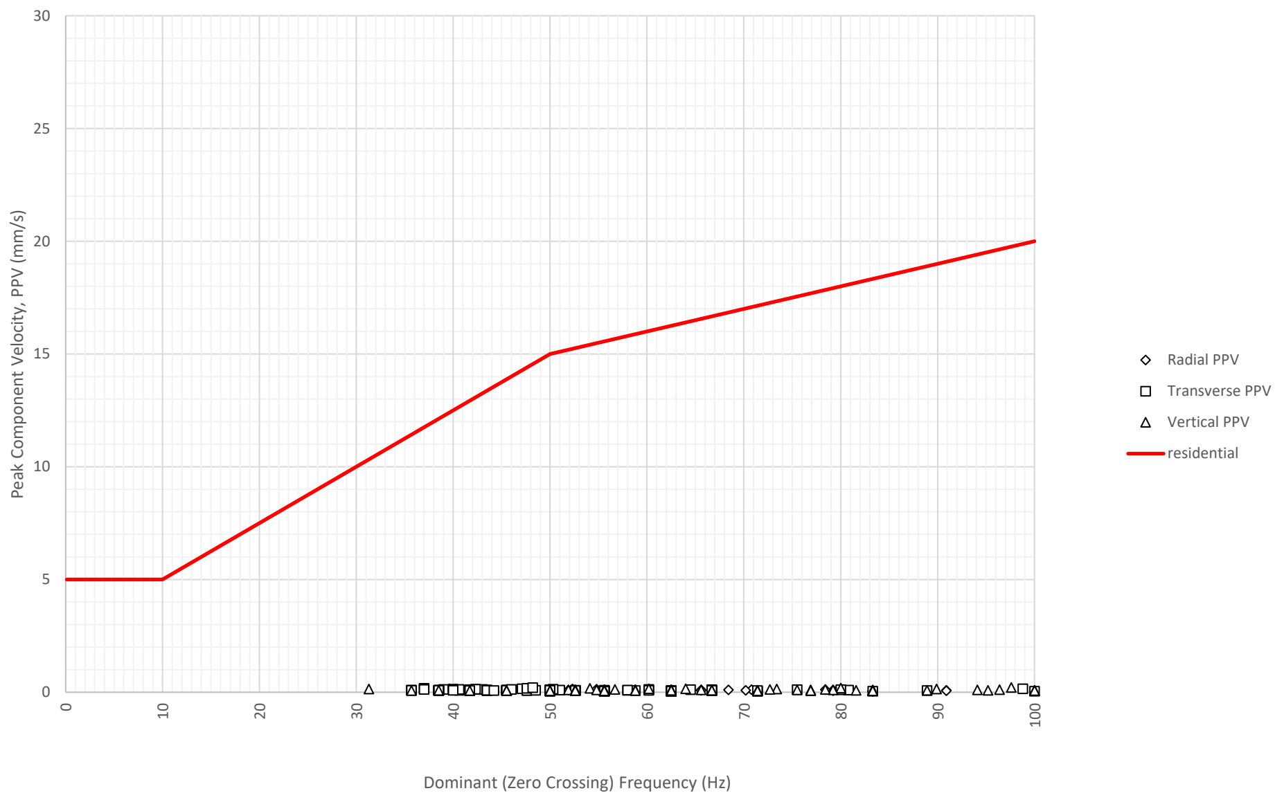
Frequency Content of Vibration Levels at East Boundary Opposite Shoalhaven Street (ETM7326) on 11-11-2024
