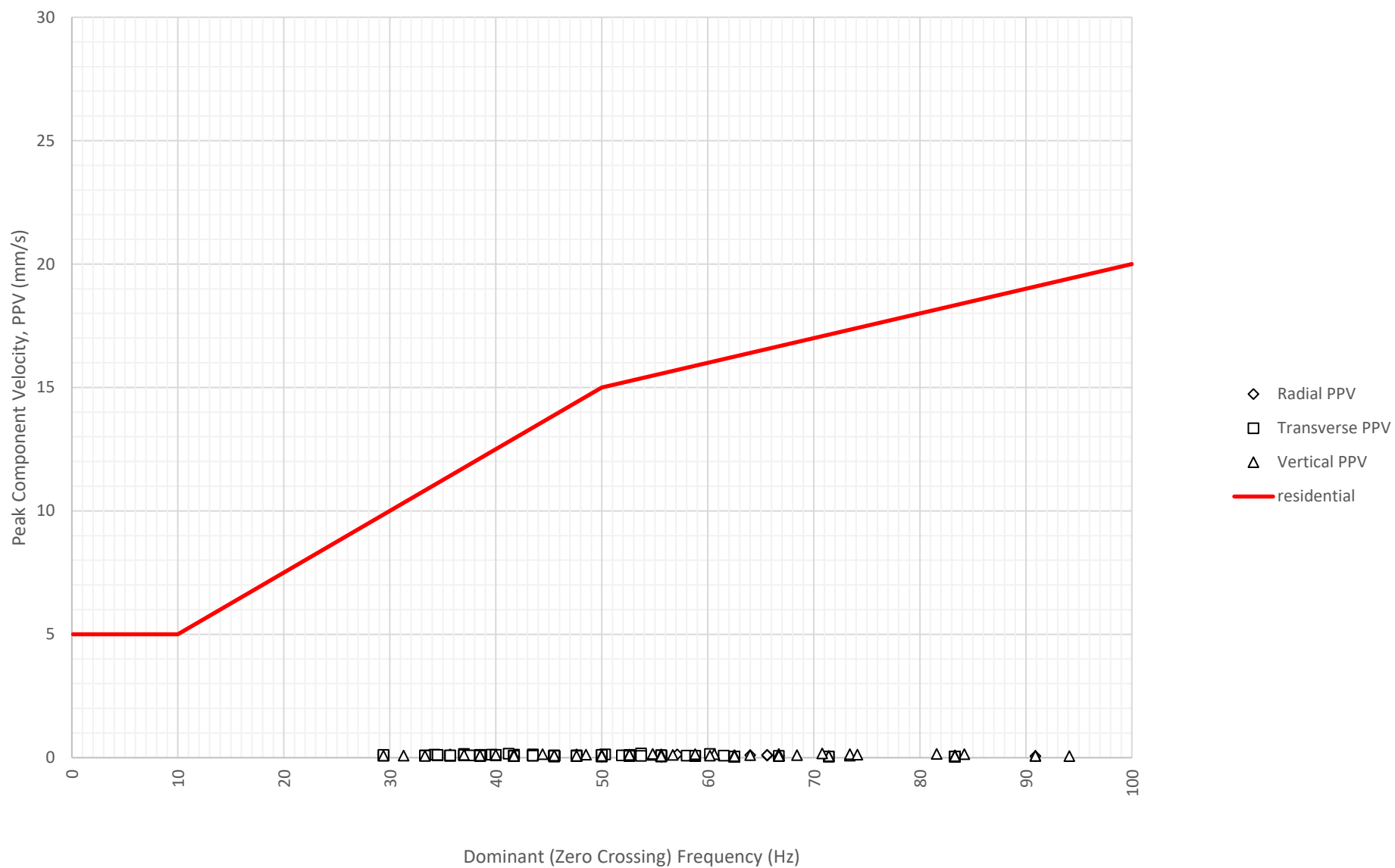
Frequency Content of Vibration Levels at East Boundary Opposite Shoalhaven Street (ETM7326) on 20-11-2024
