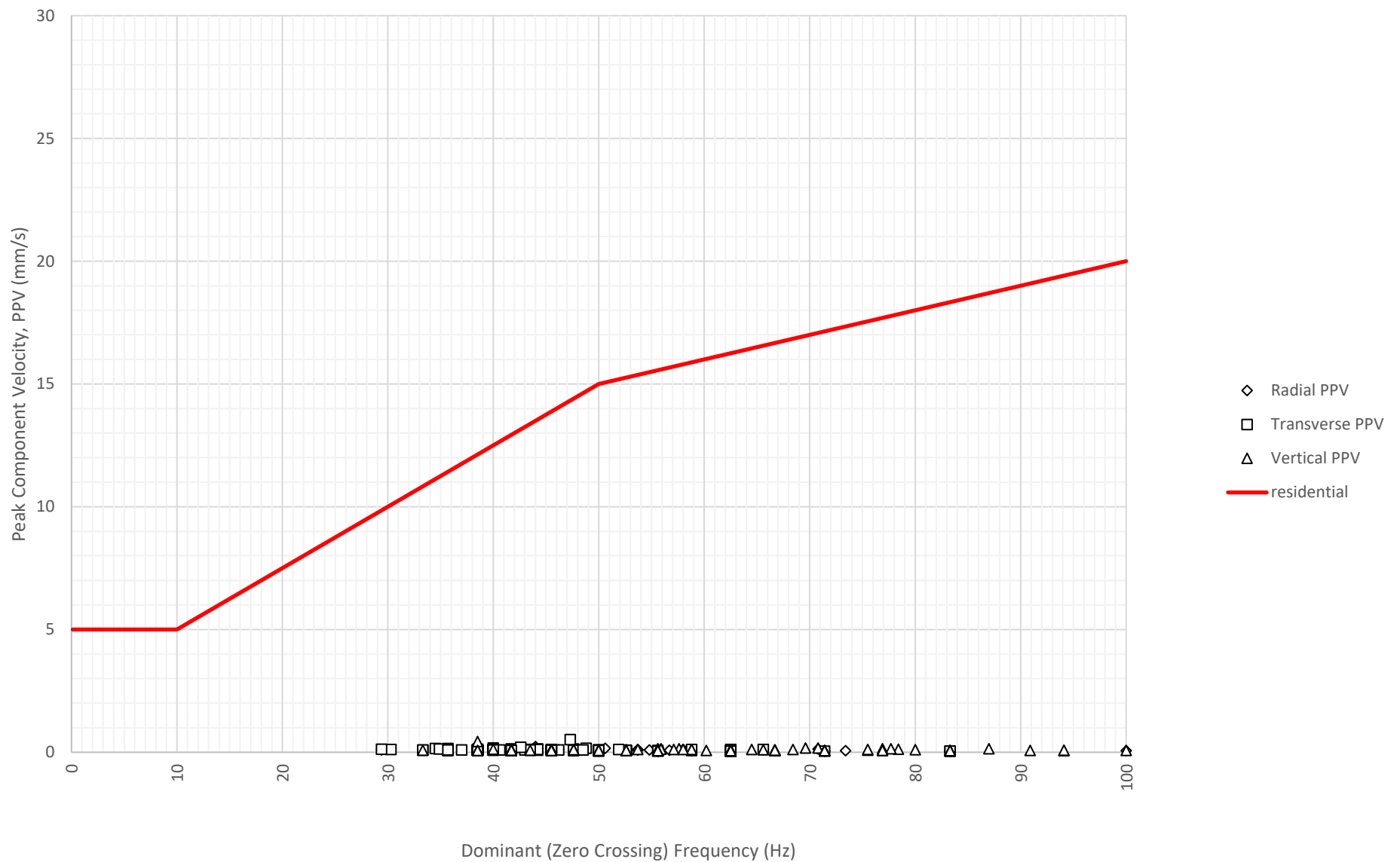
Frequency Content of Vibration Levels at East Boundary Opposite Shoalhaven Street (ETM7326) on 25-11-2024
