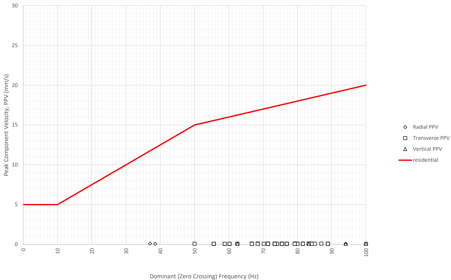
Frequency Content of Vibration Levels at North Boundary Near Block A and B (ETM7687) on 30-11-2024
