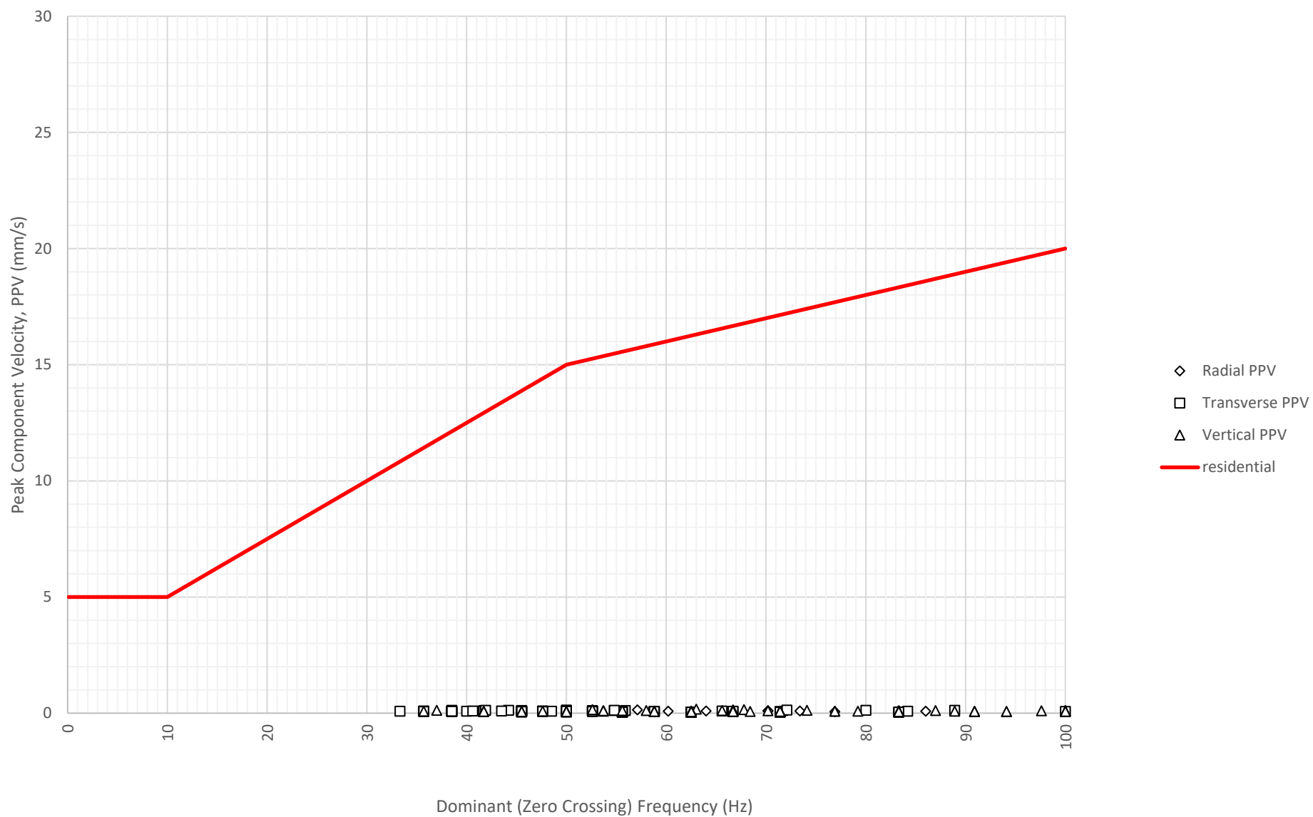
Frequency Content of Vibration Levels at East Boundary Opposite Shoalhaven Street (ETM7326) on 16-11-2024
