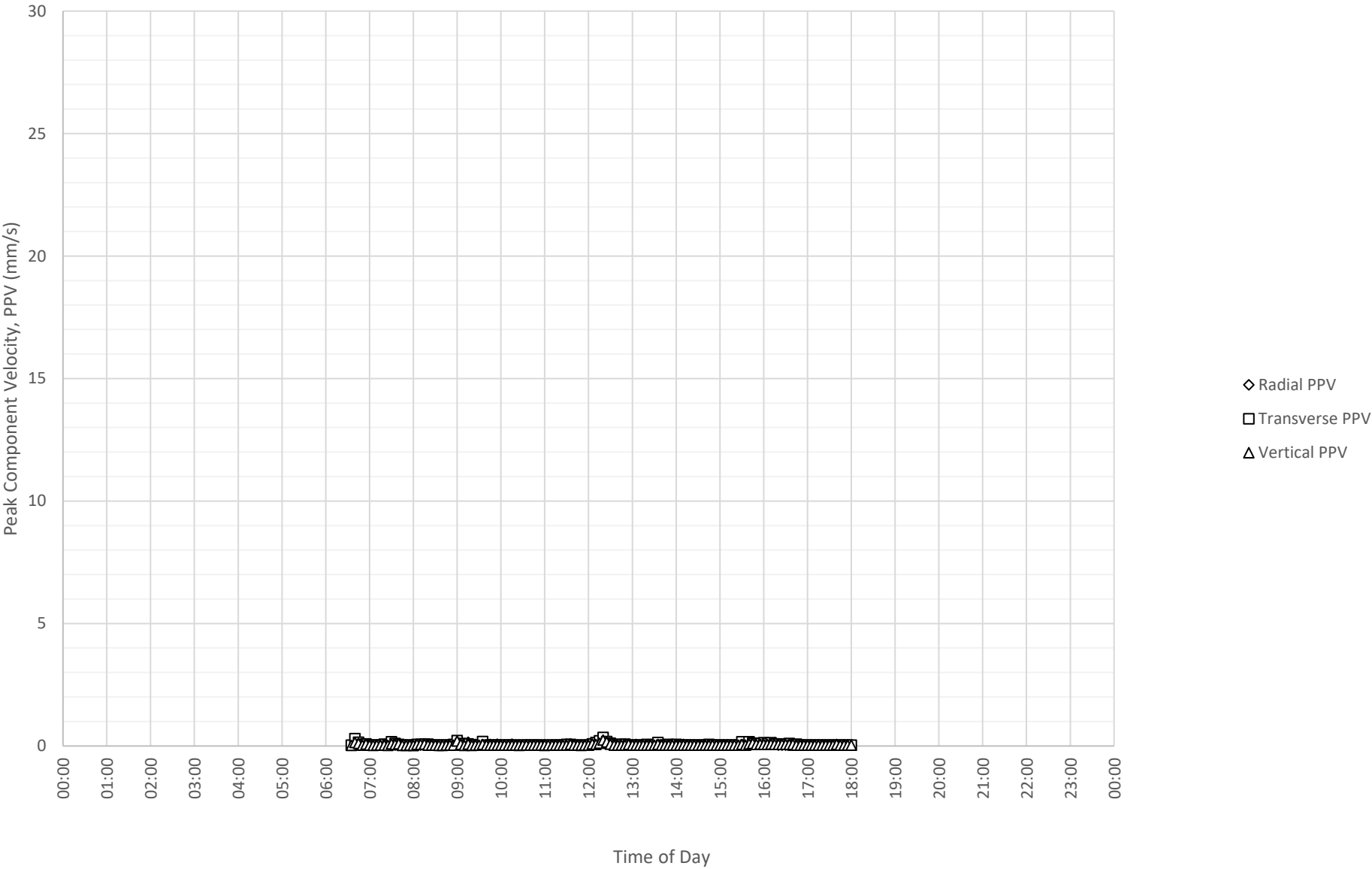
Daily Monitored Vibration Levels at North Boundary Near Block A and B (ETM7687) on 28-11-2024
