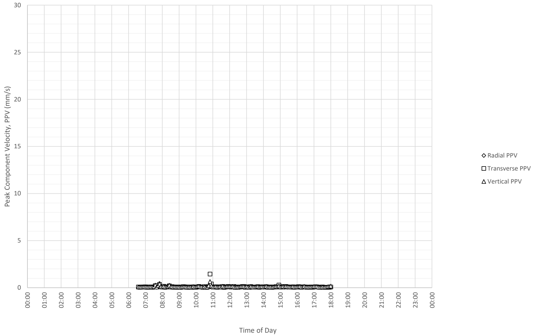
Daily Monitored Vibration Levels at East Boundary Opposite Shoalhaven Street (ETM7326) on 6-11-2024
