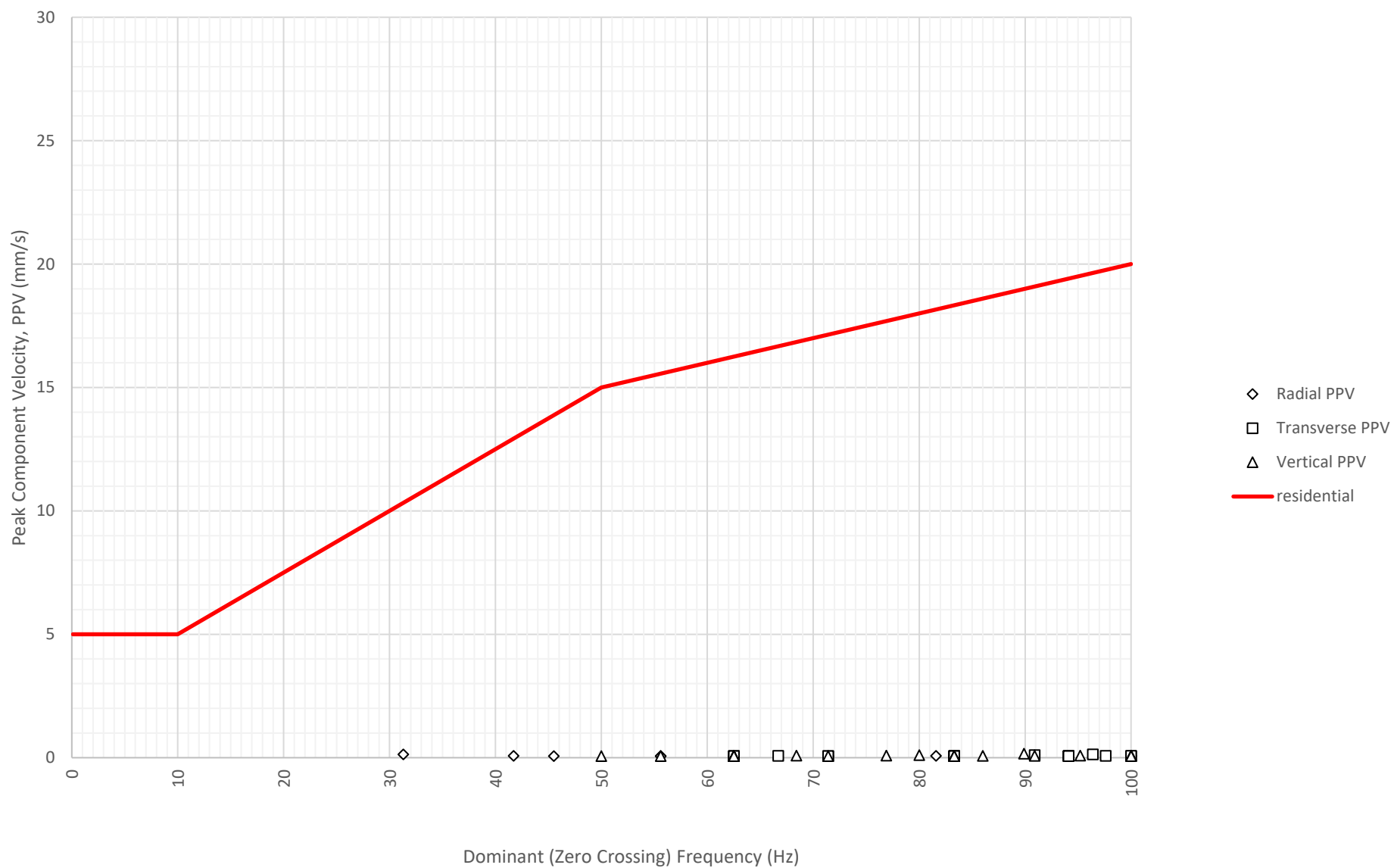
Frequency Content of Vibration Levels at North Boundary Near Block A and B (ETM7687) on 13-11-2024
