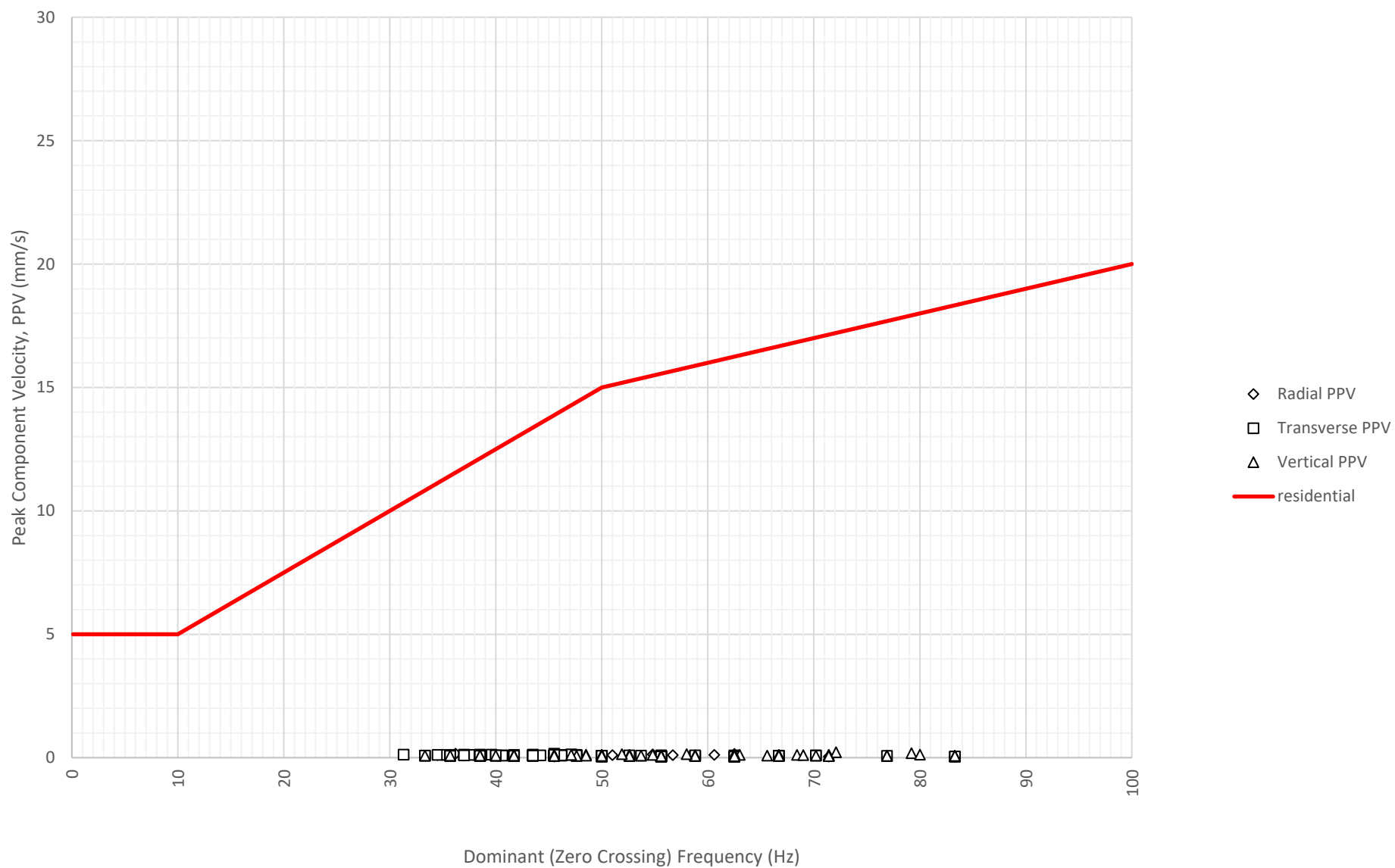
Frequency Content of Vibration Levels at East Boundary Opposite Shoalhaven Street (ETM7326) on 28-11-2024
