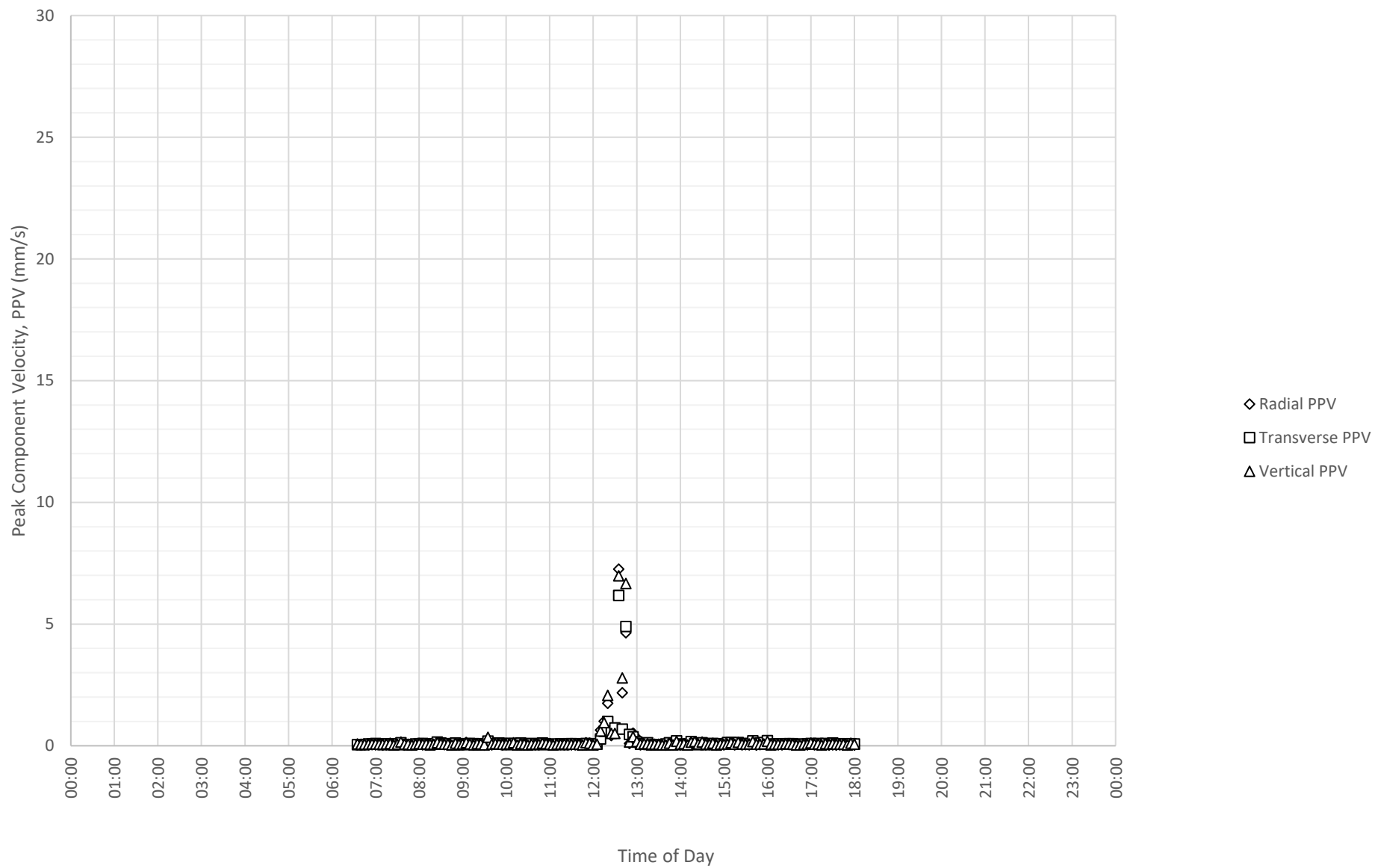
Daily Monitored Vibration Levels at East Boundary Opposite Shoalhaven Street (ETM7326) on 19-11-2024
