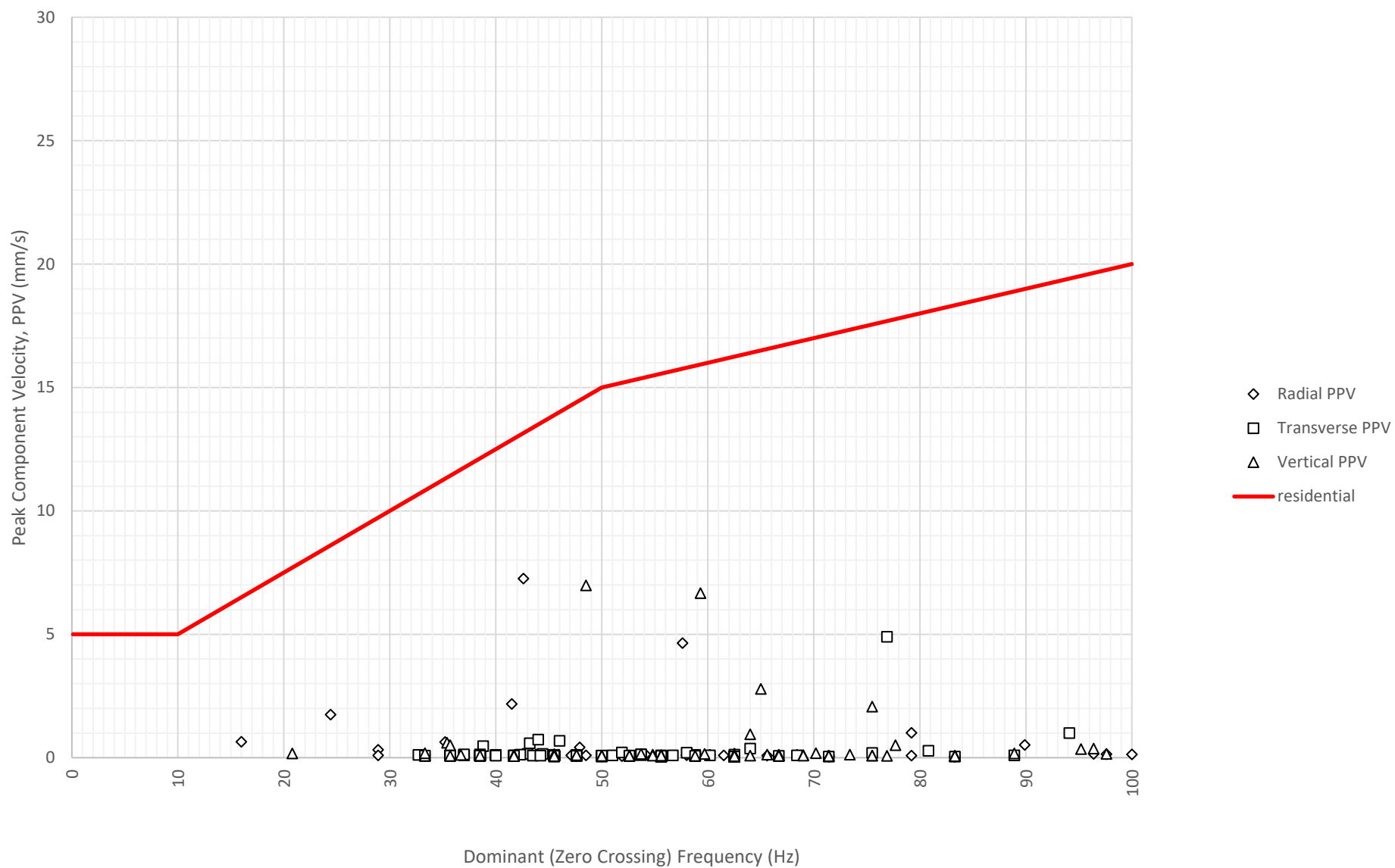
Frequency Content of Vibration Levels at East Boundary Opposite Shoalhaven Street (ETM7326) on 19-11-2024
