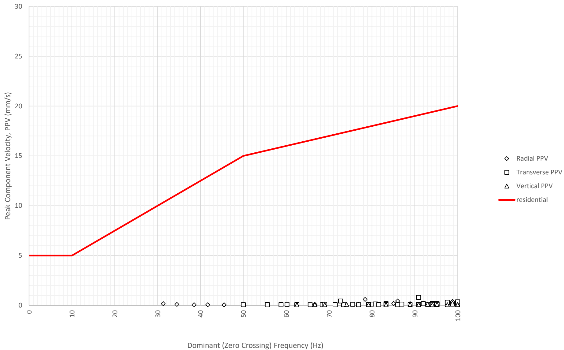
Frequency Content of Vibration Levels at North Boundary Near Block A and B (ETM7687) on 19-11-2024
