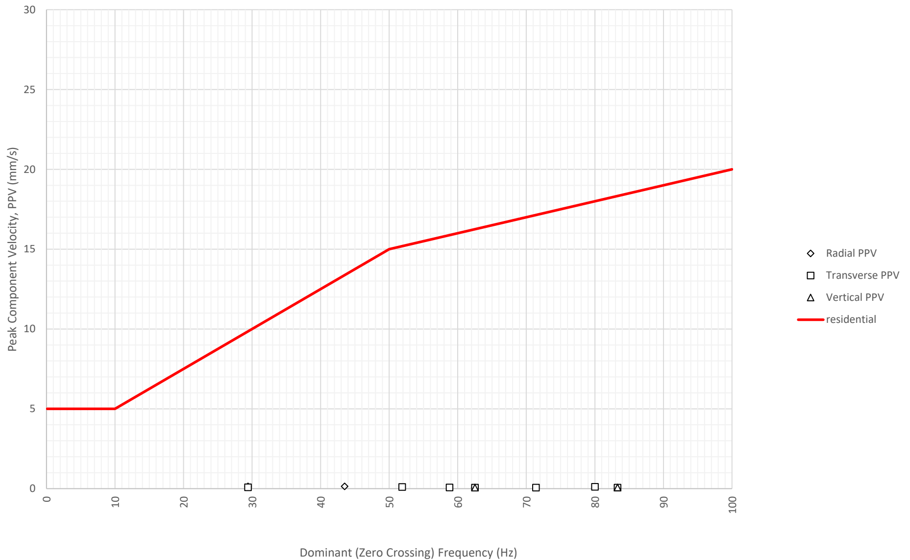
Frequency Content of Vibration Levels at North Boundary Near Block A and B (ETM7687) on 2-11-2024
