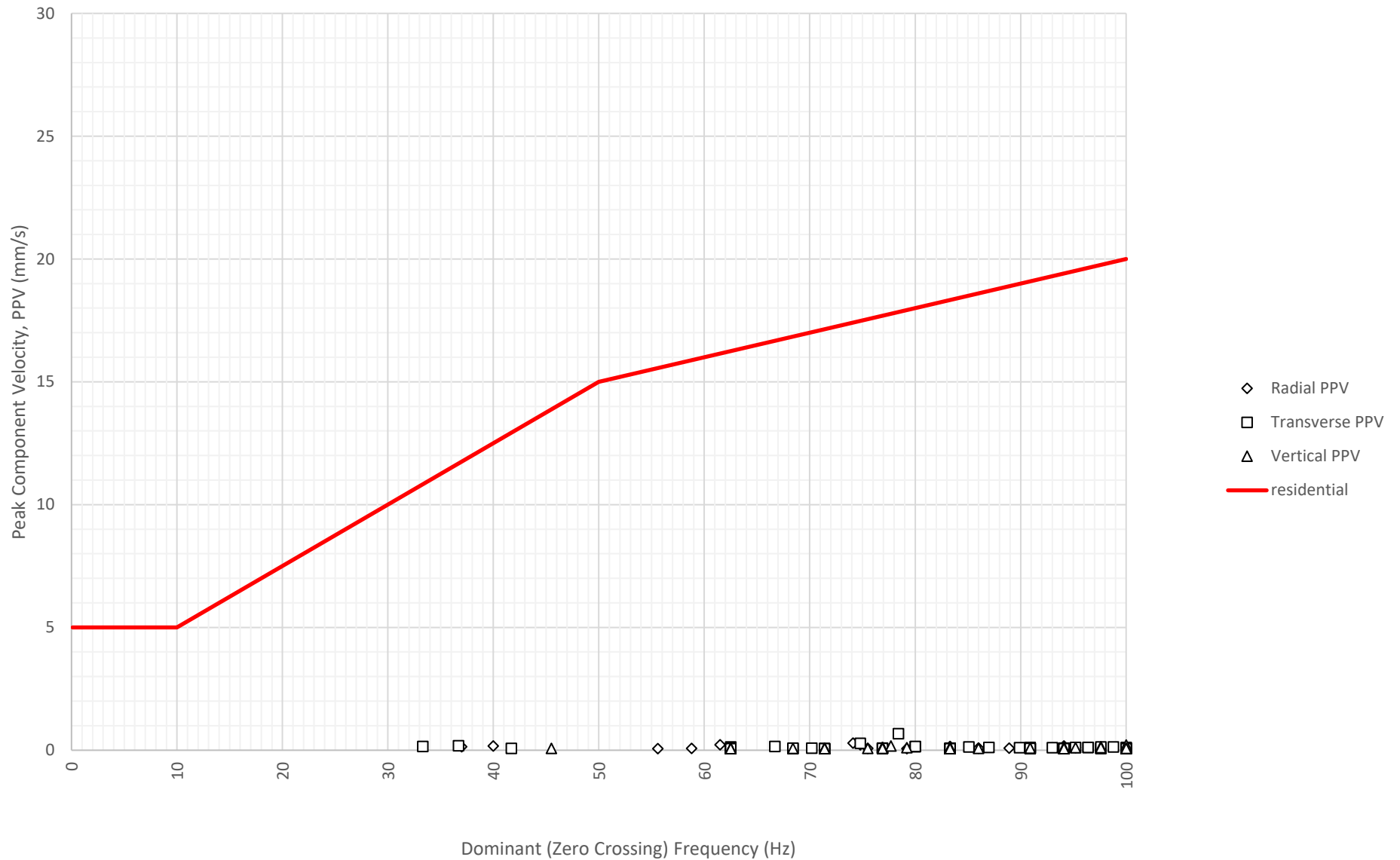
Frequency Content of Vibration Levels at North Boundary Near Block A and B (ETM7687) on 4-11-2024
