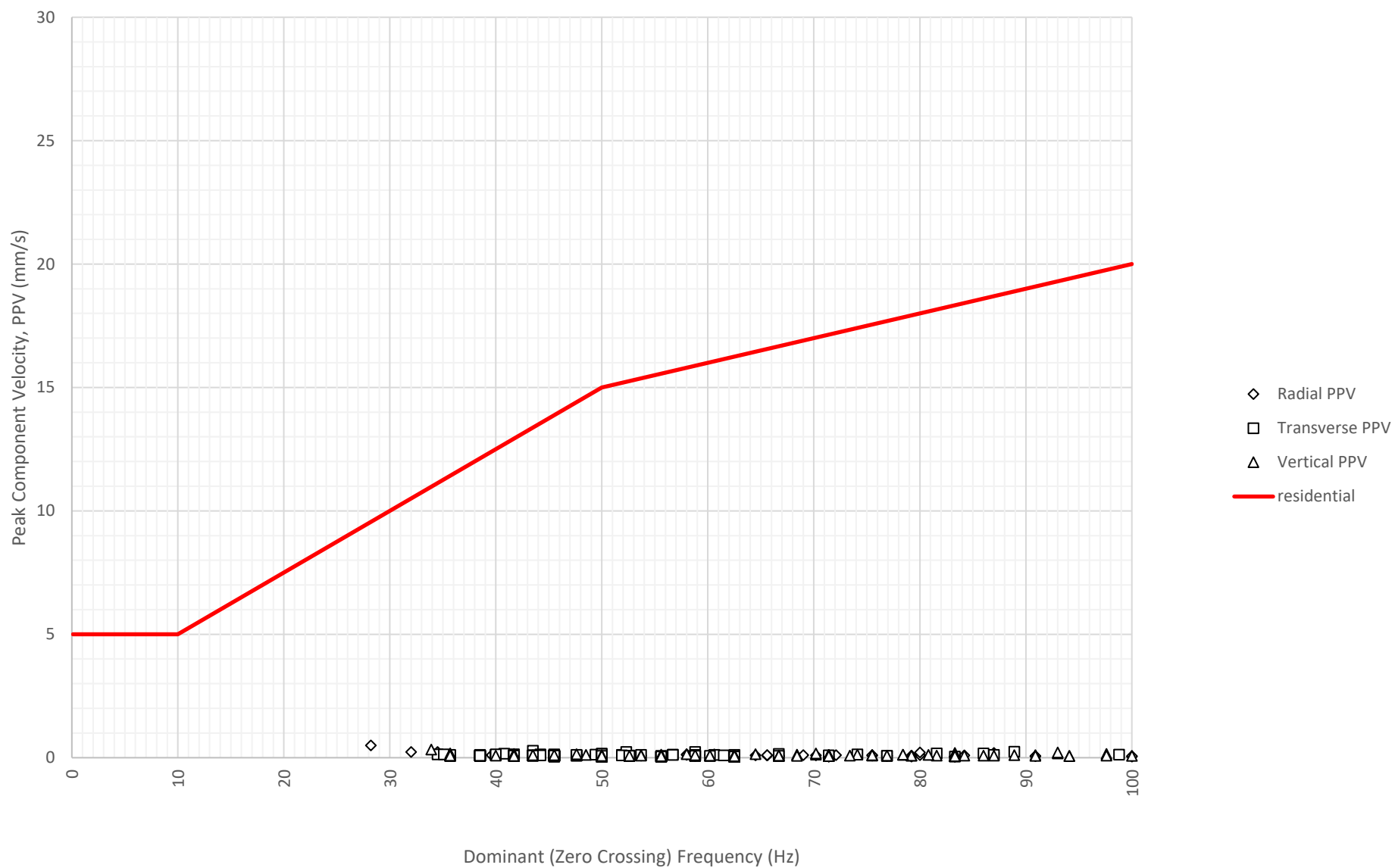
Frequency Content of Vibration Levels at East Boundary Opposite Shoalhaven Street (ETM7326) on 14-11-2024
