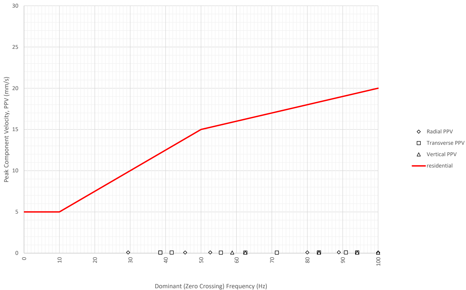
Frequency Content of Vibration Levels at North Boundary Near Block A and B (ETM7687) on 23-11-2024
