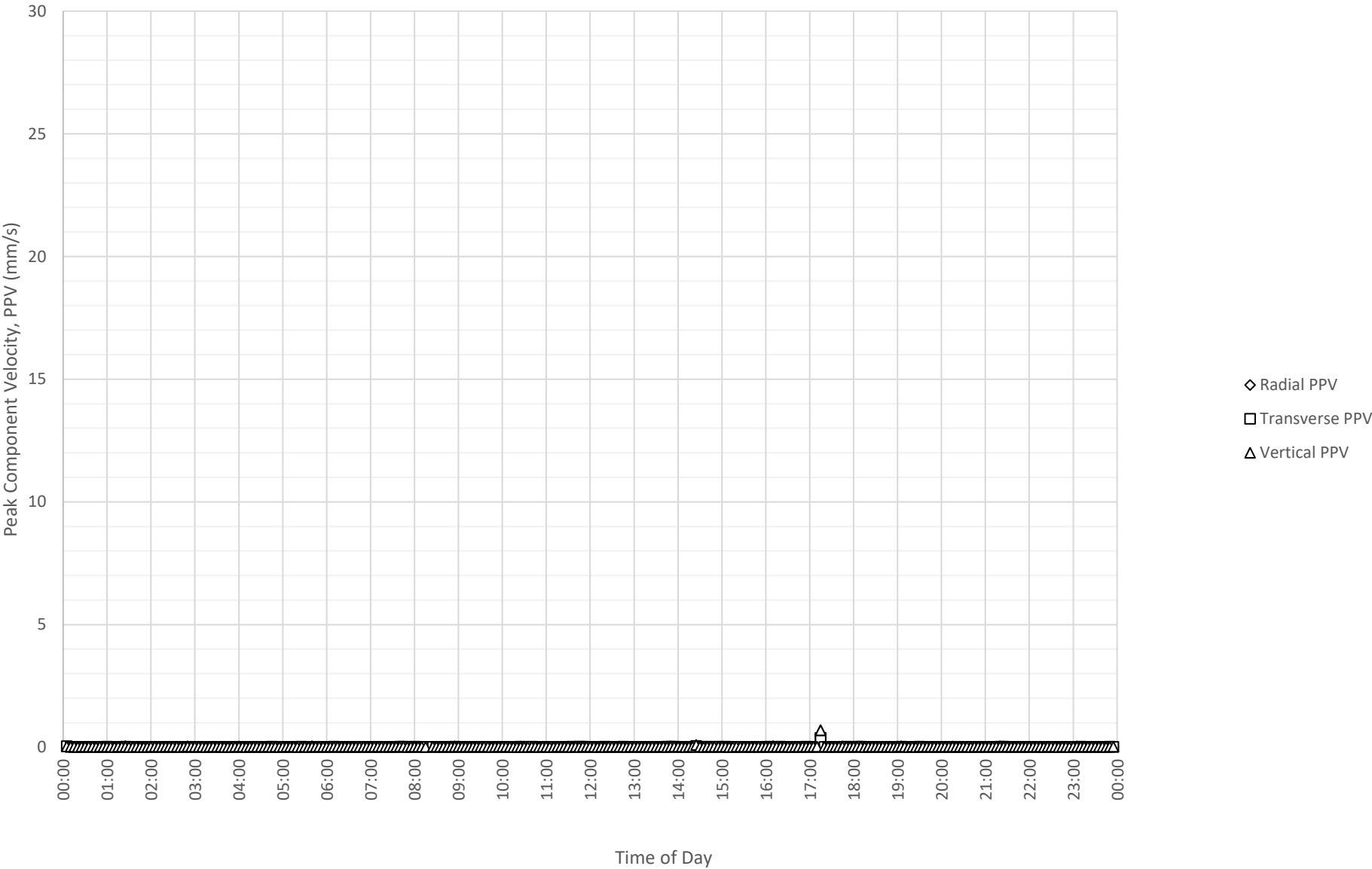
Daily Monitored Vibration Levels at Charles Perkins Centre - Observation Room Corridor on 8-10-2024
