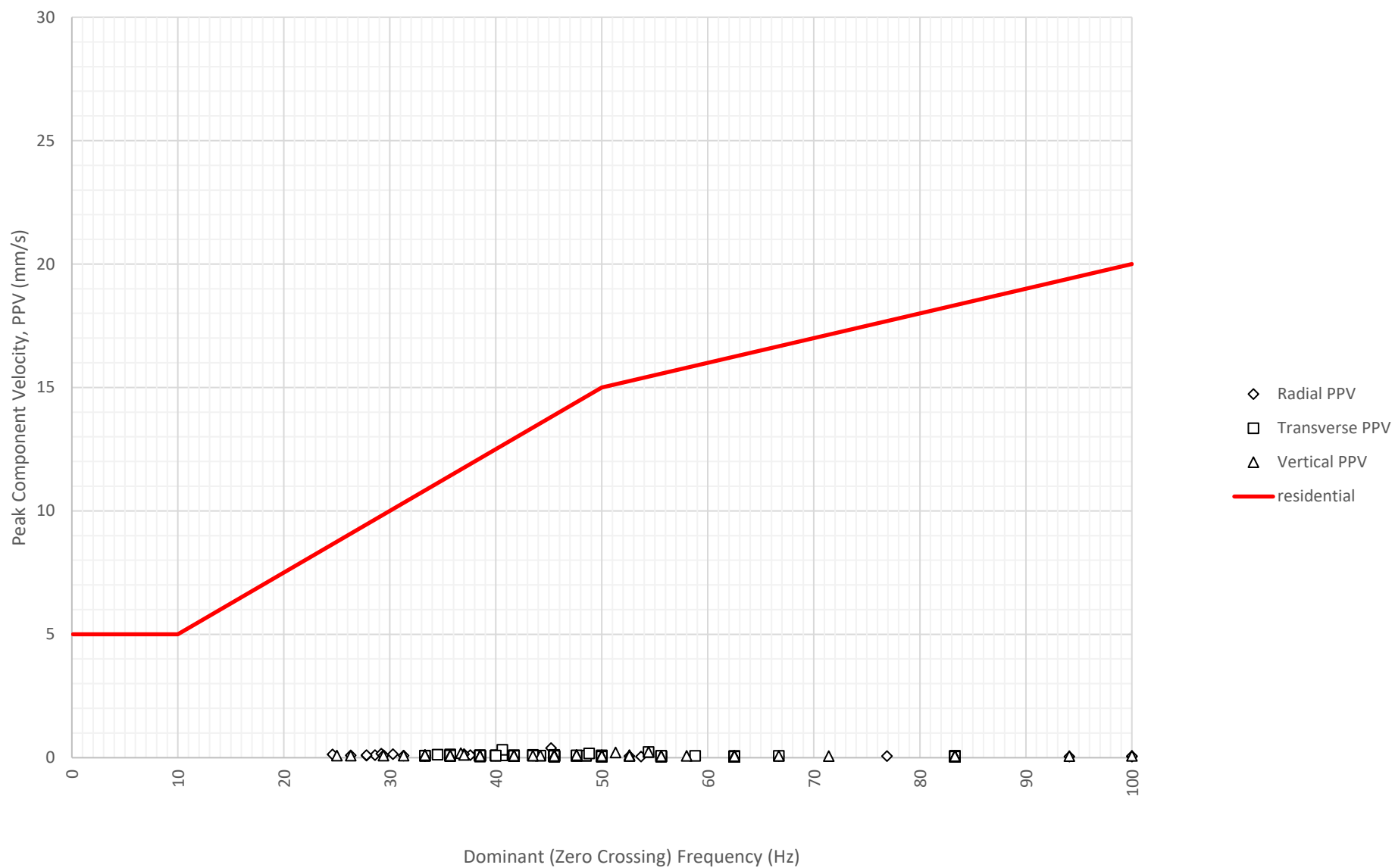
Frequency Content of Vibration Levels at East Boundary Opposite Shoalhaven Street (ETM7326) on 16-08-2024
