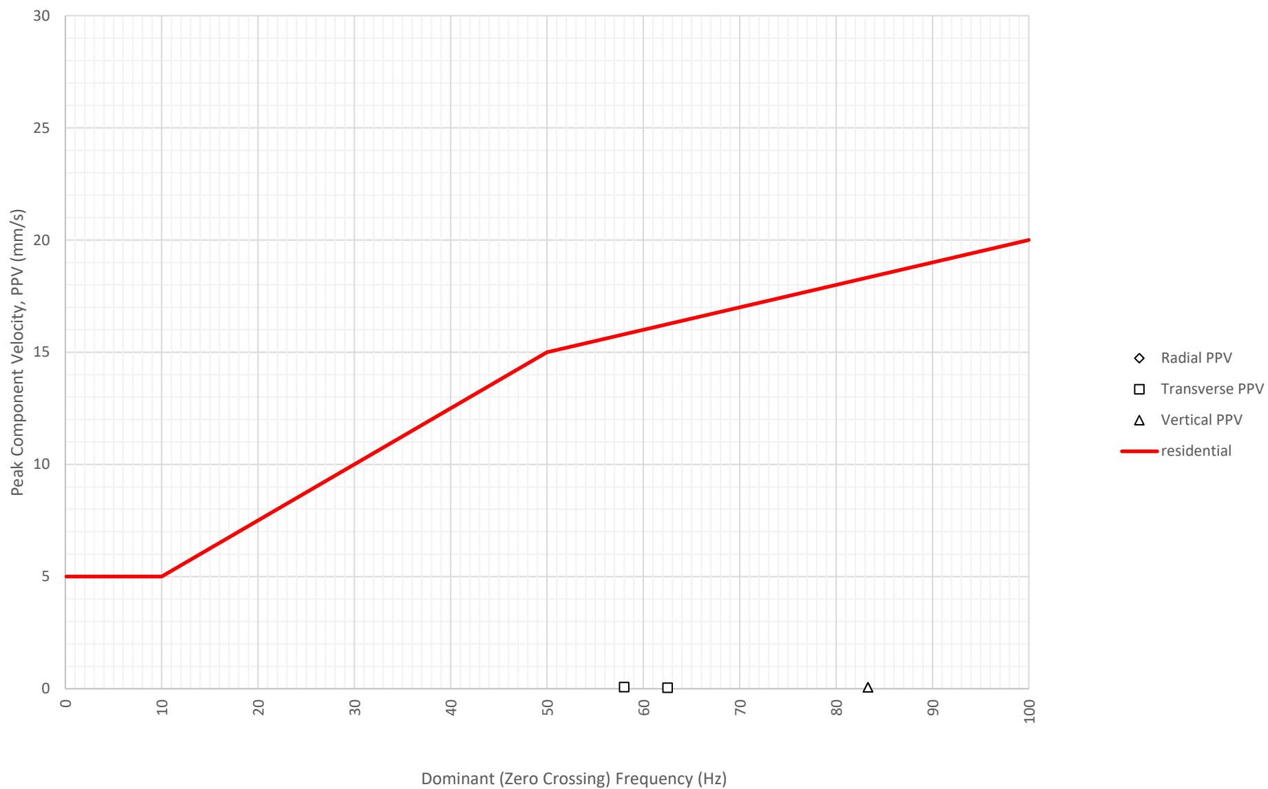
Frequency Content of Vibration Levels at East Boundary Opposite Shoalhaven Street (ETM7326) on 25-08-2024
