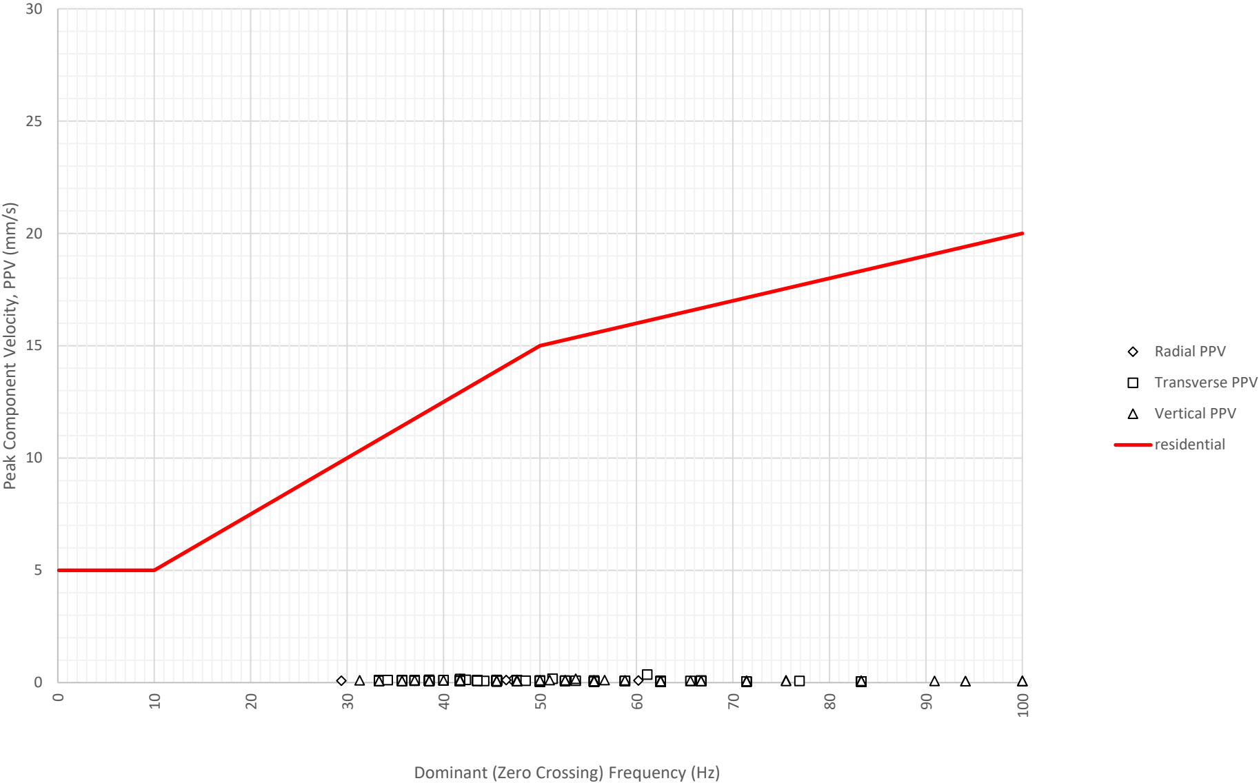
Frequency Content of Vibration Levels at East Boundary Opposite Shoalhaven Street (ETM7326) on 5-08-2024
