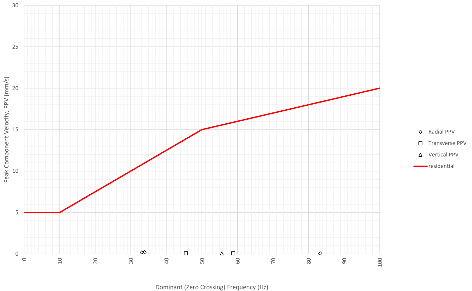
Frequency Content of Vibration Levels at North Boundary Near Block A and B (ETM7687) on 10-08-2024
