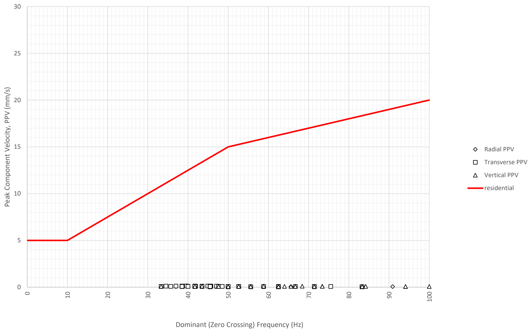
Frequency Content of Vibration Levels at East Boundary Opposite Shoalhaven Street (ETM7326) on 31-08-2024
