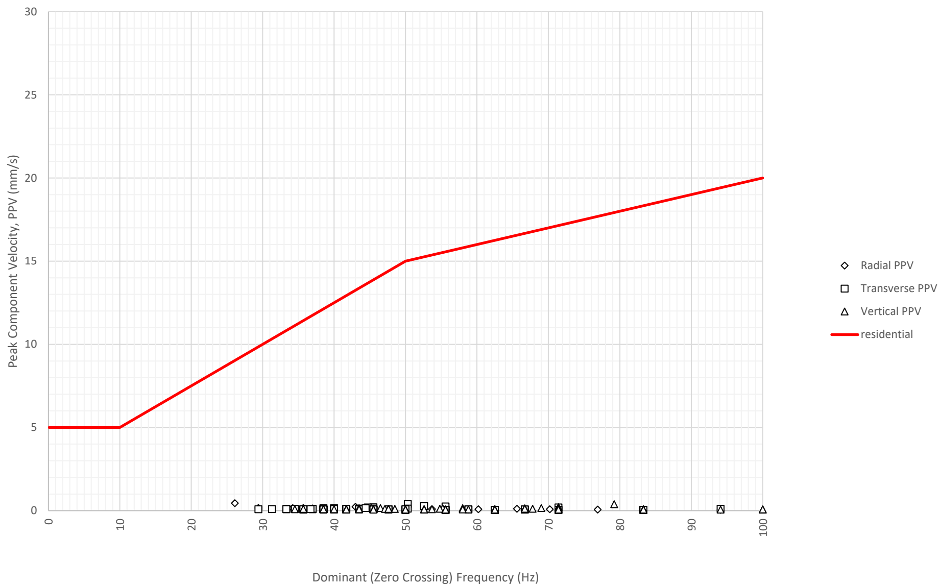
Frequency Content of Vibration Levels at East Boundary Opposite Shoalhaven Street (ETM7326) on 26-08-2024
