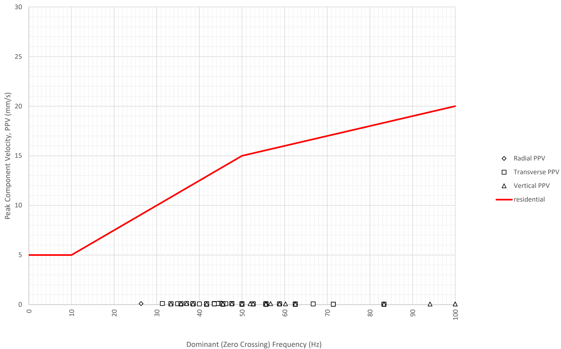
Frequency Content of Vibration Levels at East Boundary Opposite Shoalhaven Street (ETM7326) on 24-08-2024
