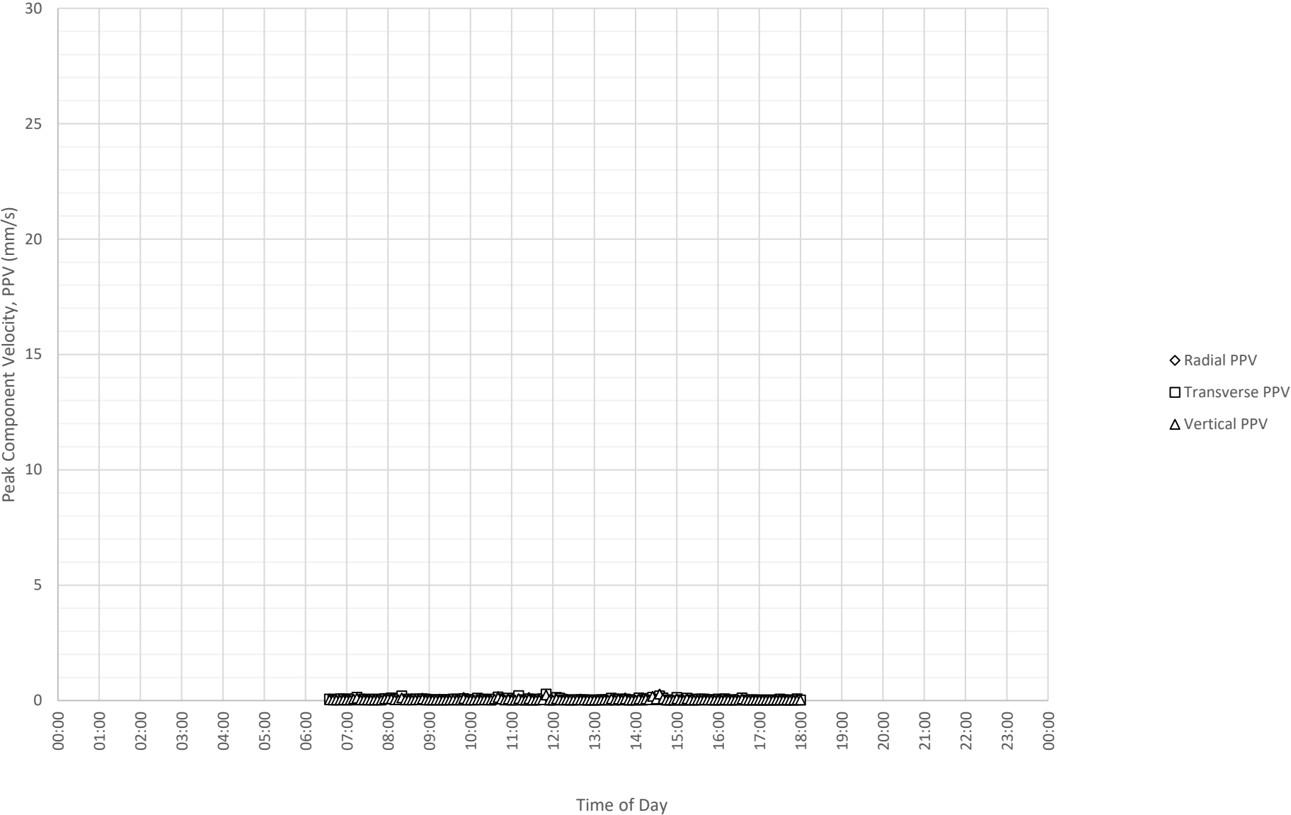
Daily Monitored Vibration Levels at North Boundary Near Block A and B (ETM7687) on 13-08-2024
