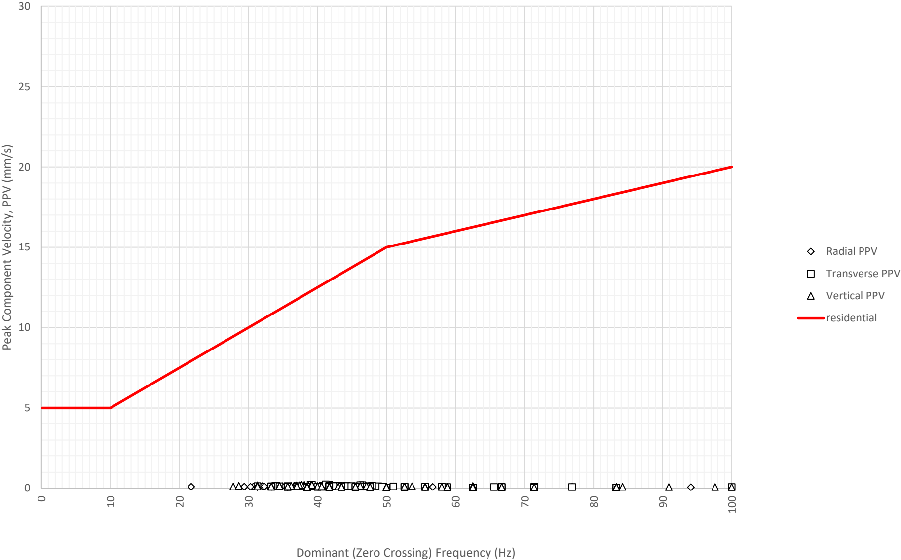
Frequency Content of Vibration Levels at East Boundary Opposite Shoalhaven Street (ETM7326) on 8-08-2024
