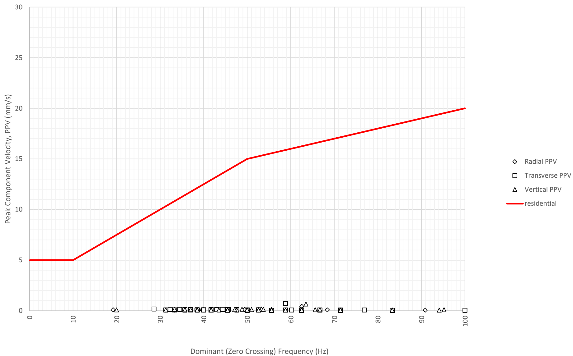
Frequency Content of Vibration Levels at East Boundary Opposite Shoalhaven Street (ETM7326) on 21-08-2024
