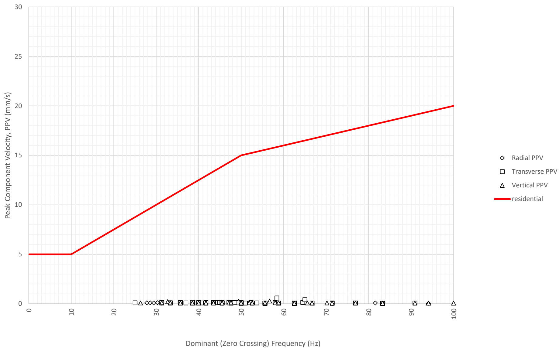
Frequency Content of Vibration Levels at East Boundary Opposite Shoalhaven Street (ETM7326) on 12-08-2024
