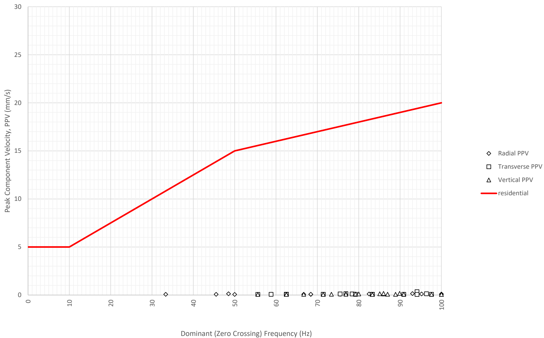
Frequency Content of Vibration Levels at North Boundary Near Block A and B (ETM7687) on 30-08-2024
