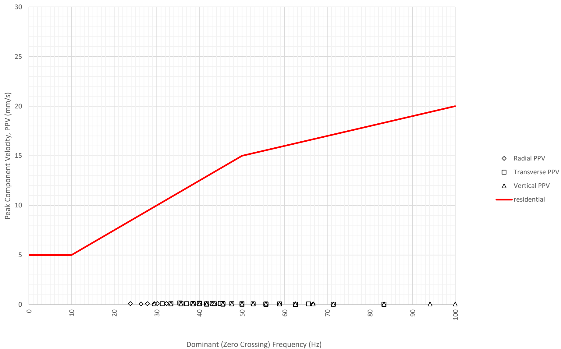
Frequency Content of Vibration Levels at East Boundary Opposite Shoalhaven Street (ETM7326) on 14-08-2024
