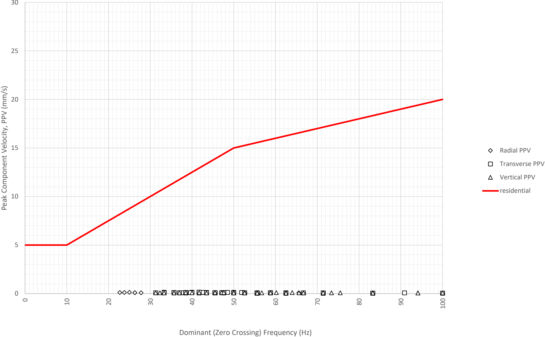
Frequency Content of Vibration Levels at East Boundary Opposite Shoalhaven Street (ETM7326) on 9-08-2024
