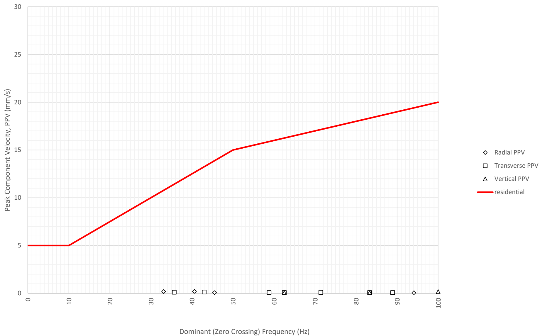
Frequency Content of Vibration Levels at North Boundary Near Block A and B (ETM7687) on 17-08-2024
