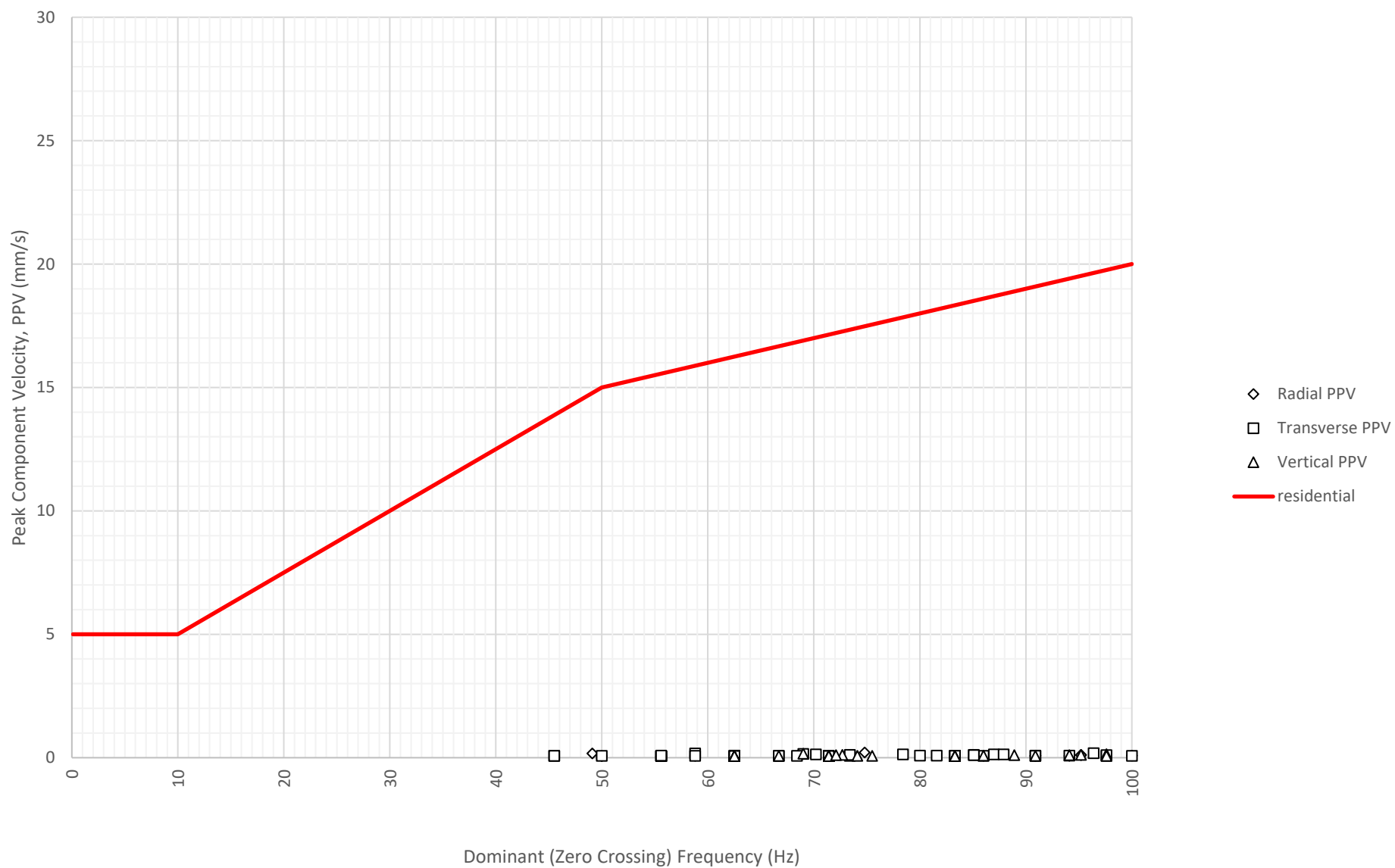
Frequency Content of Vibration Levels at North Boundary Near Block A and B (ETM7687) on 16-08-2024
