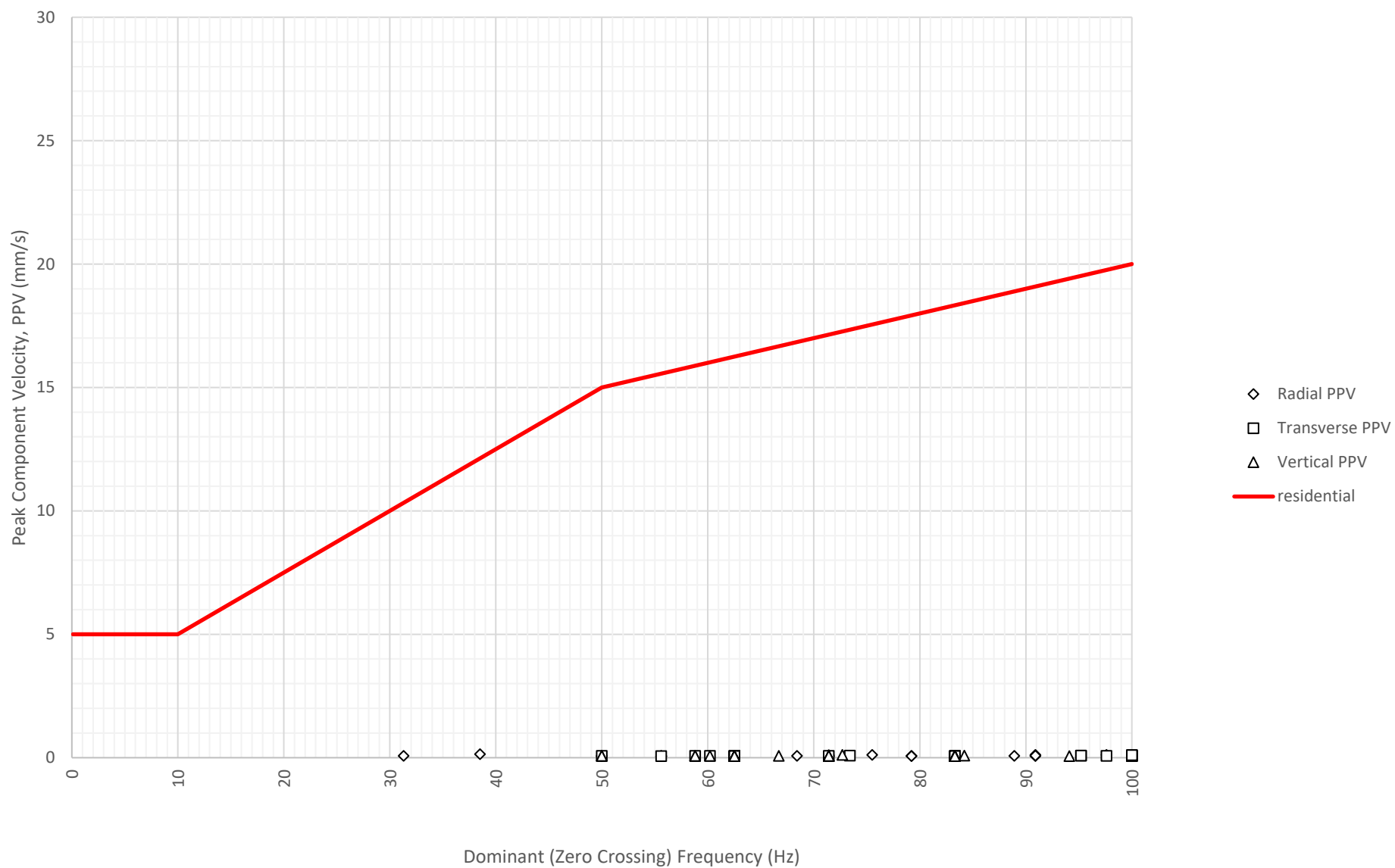
Frequency Content of Vibration Levels at North Boundary Near Block A and B (ETM7687) on 27-08-2024
