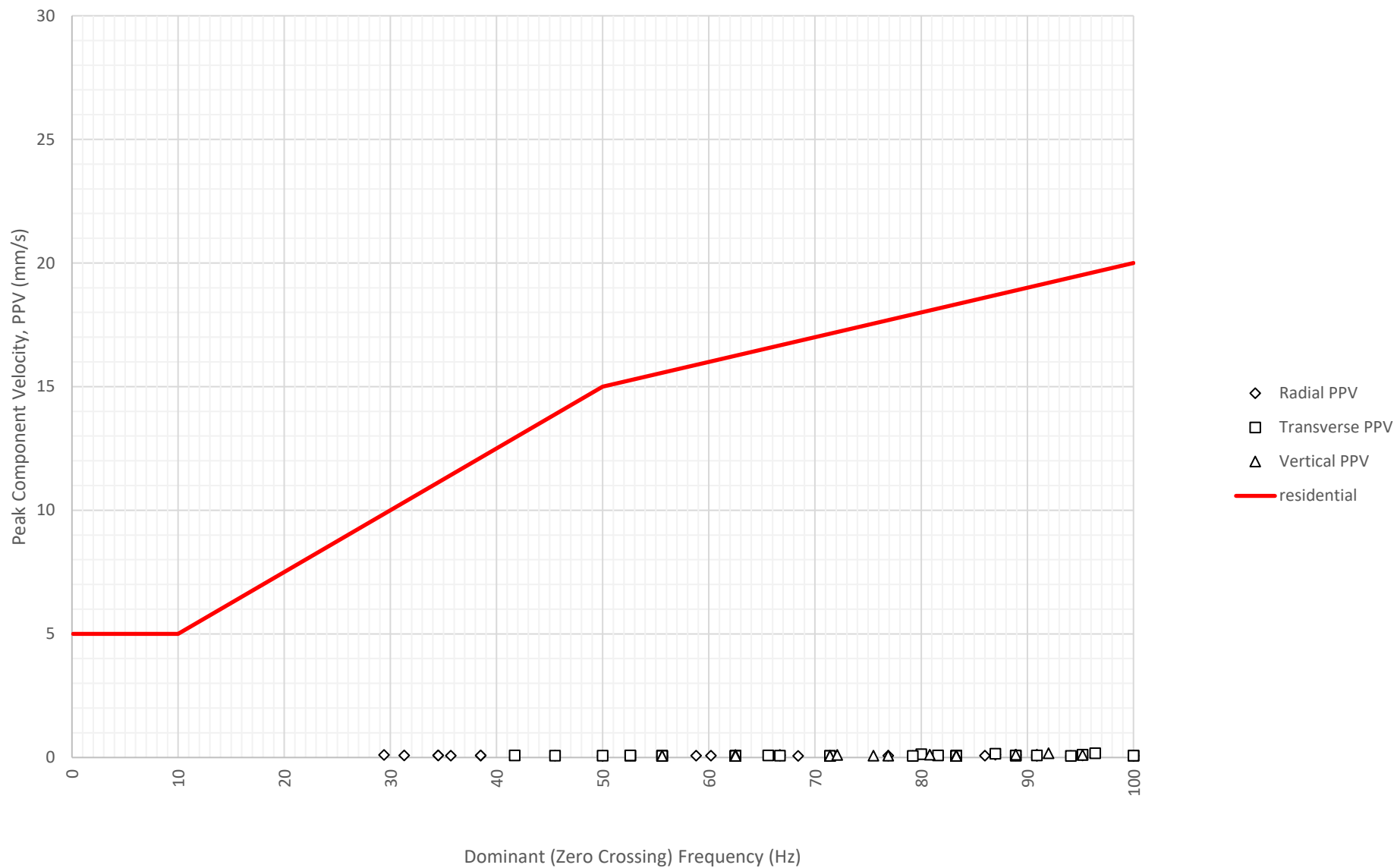
Frequency Content of Vibration Levels at North Boundary Near Block A and B (ETM7687) on 28-08-2024
