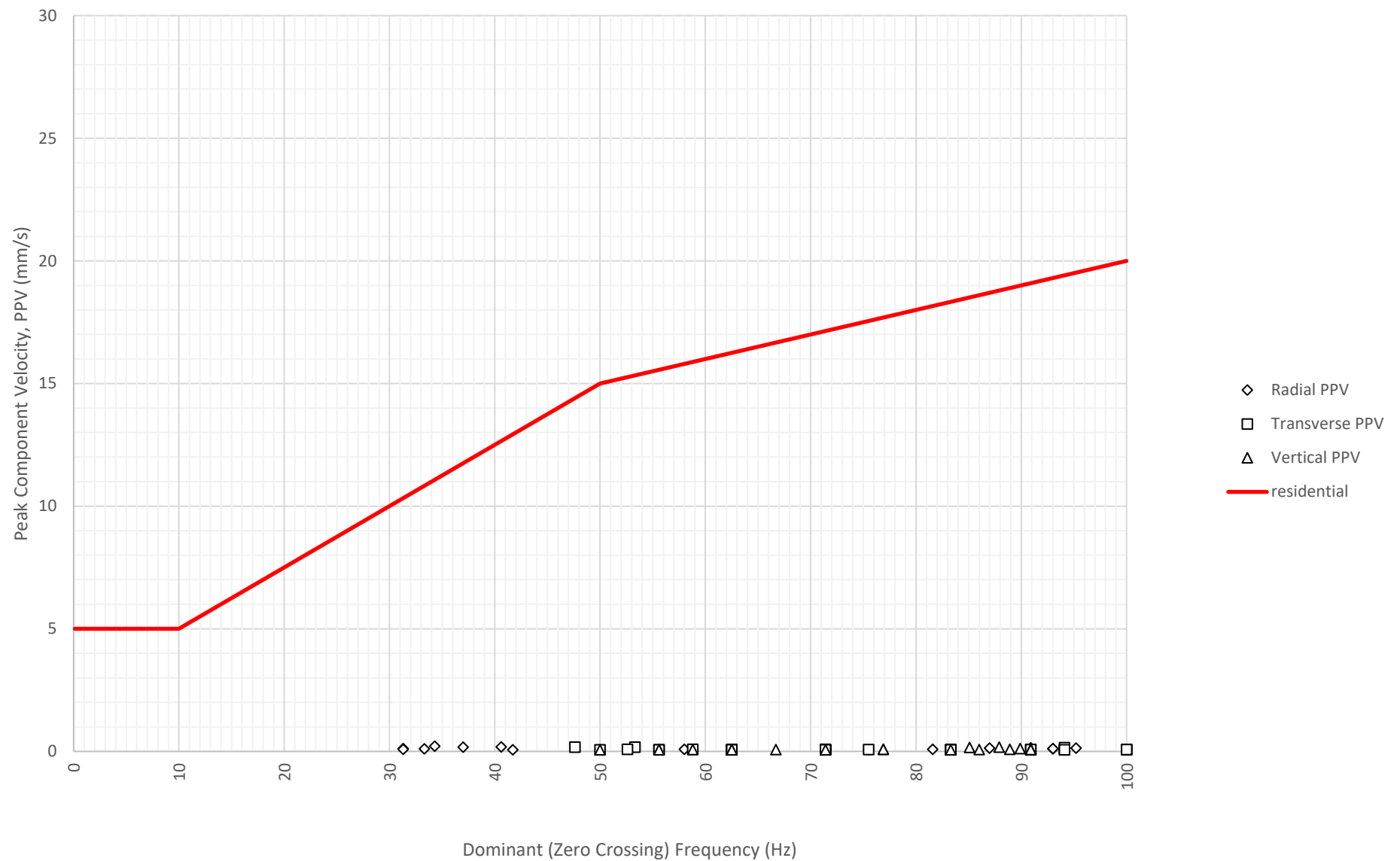
Frequency Content of Vibration Levels at North Boundary Near Block A and B (ETM7687) on 29-08-2024
