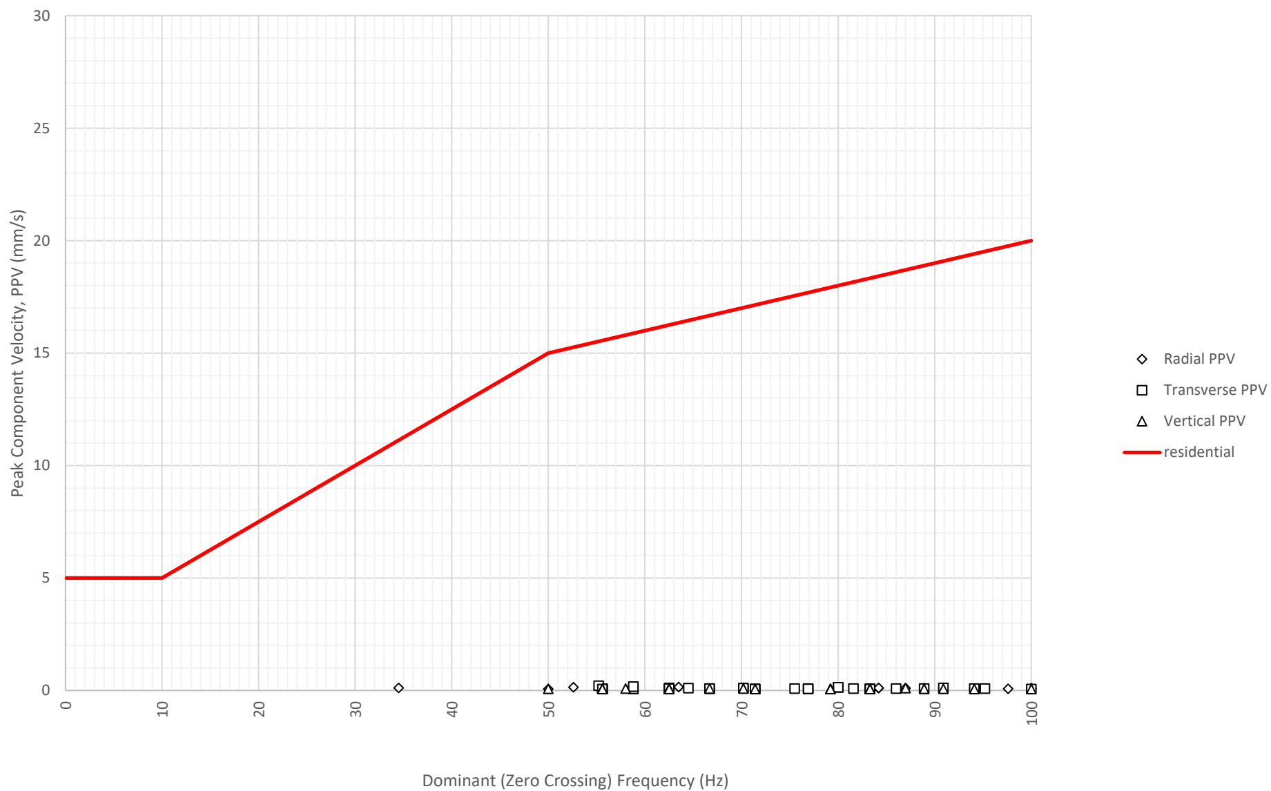
Frequency Content of Vibration Levels at North Boundary Near Block A and B (ETM7687) on 20-08-2024
