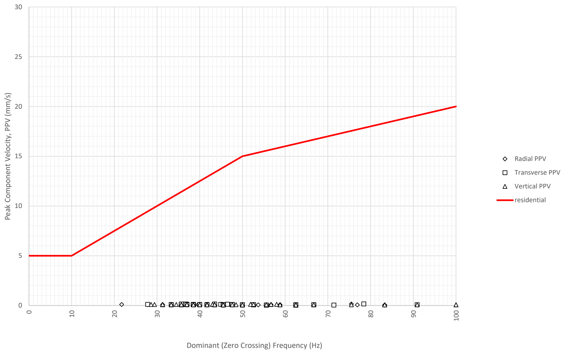
Frequency Content of Vibration Levels at East Boundary Opposite Shoalhaven Street (ETM7326) on 20-08-2024
