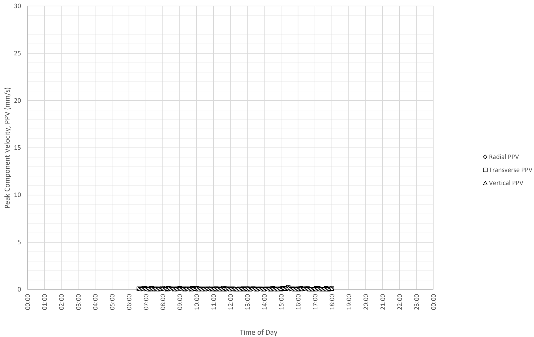
Daily Monitored Vibration Levels at East Boundary Opposite Shoalhaven Street (ETM7326) on 6-08-2024
