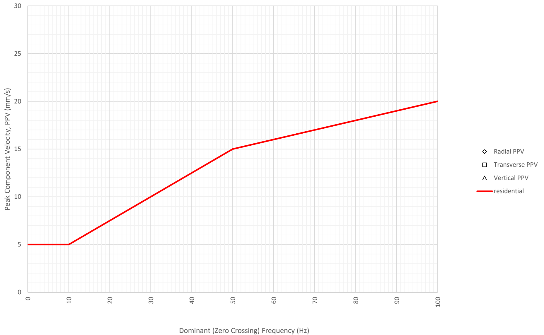
Frequency Content of Vibration Levels at North Boundary Near Block A and B (ETM7687) on 11-08-2024
