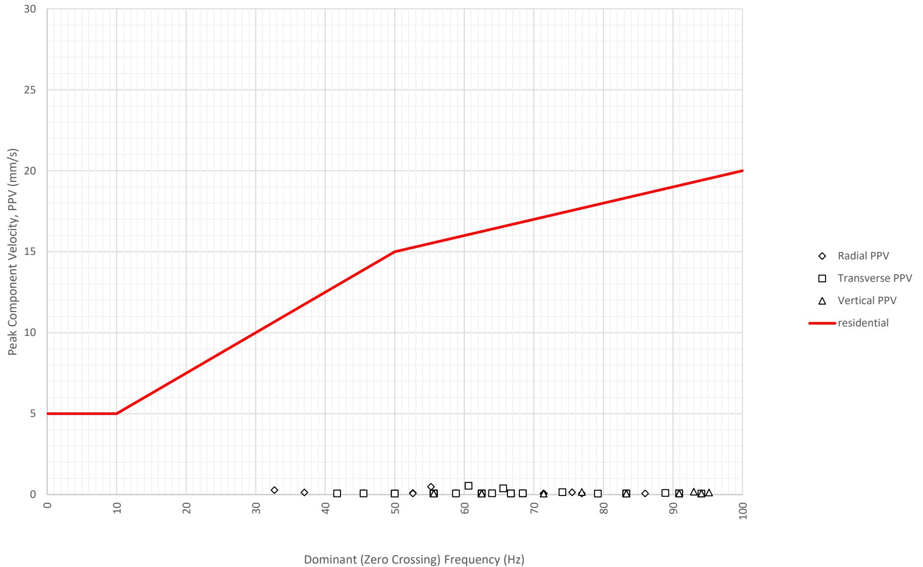
Frequency Content of Vibration Levels at North Boundary Near Block A and B (ETM7687) on 8-08-2024
