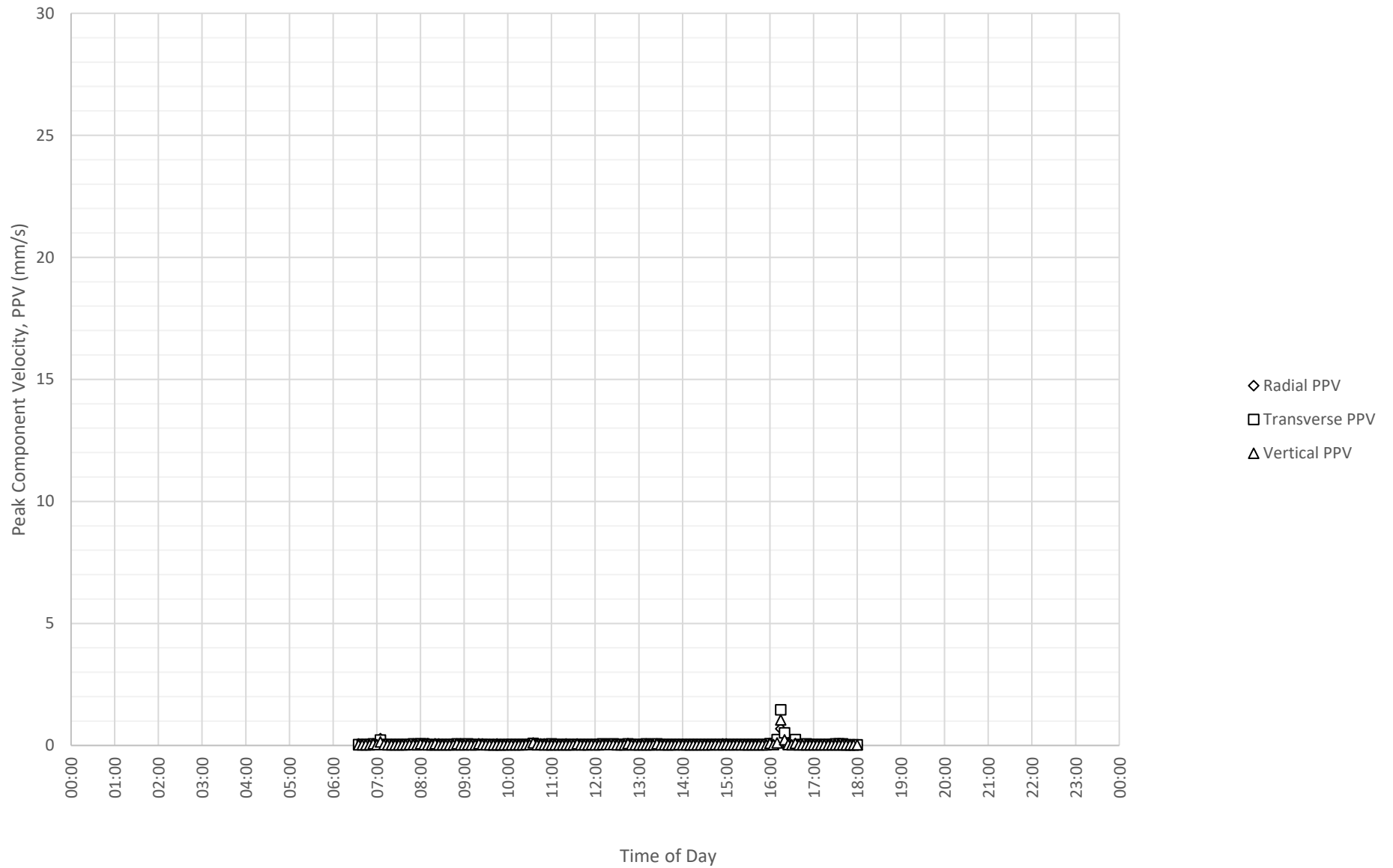
Daily Monitored Vibration Levels at North Boundary Near Block A and B (ETM7687) on 7-08-2024
