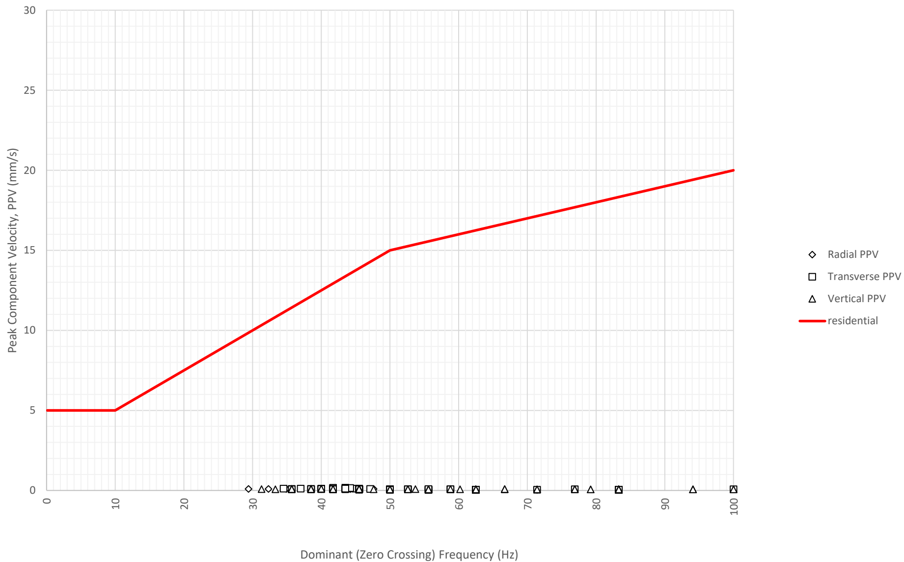
Frequency Content of Vibration Levels at East Boundary Opposite Shoalhaven Street (ETM7326) on 3-08-2024
