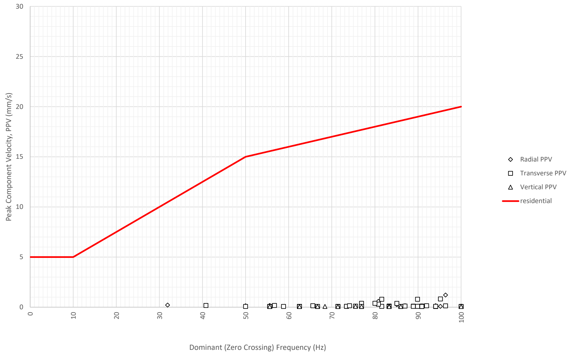
Frequency Content of Vibration Levels at North Boundary Near Block A and B (ETM7687) on 15-08-2024
