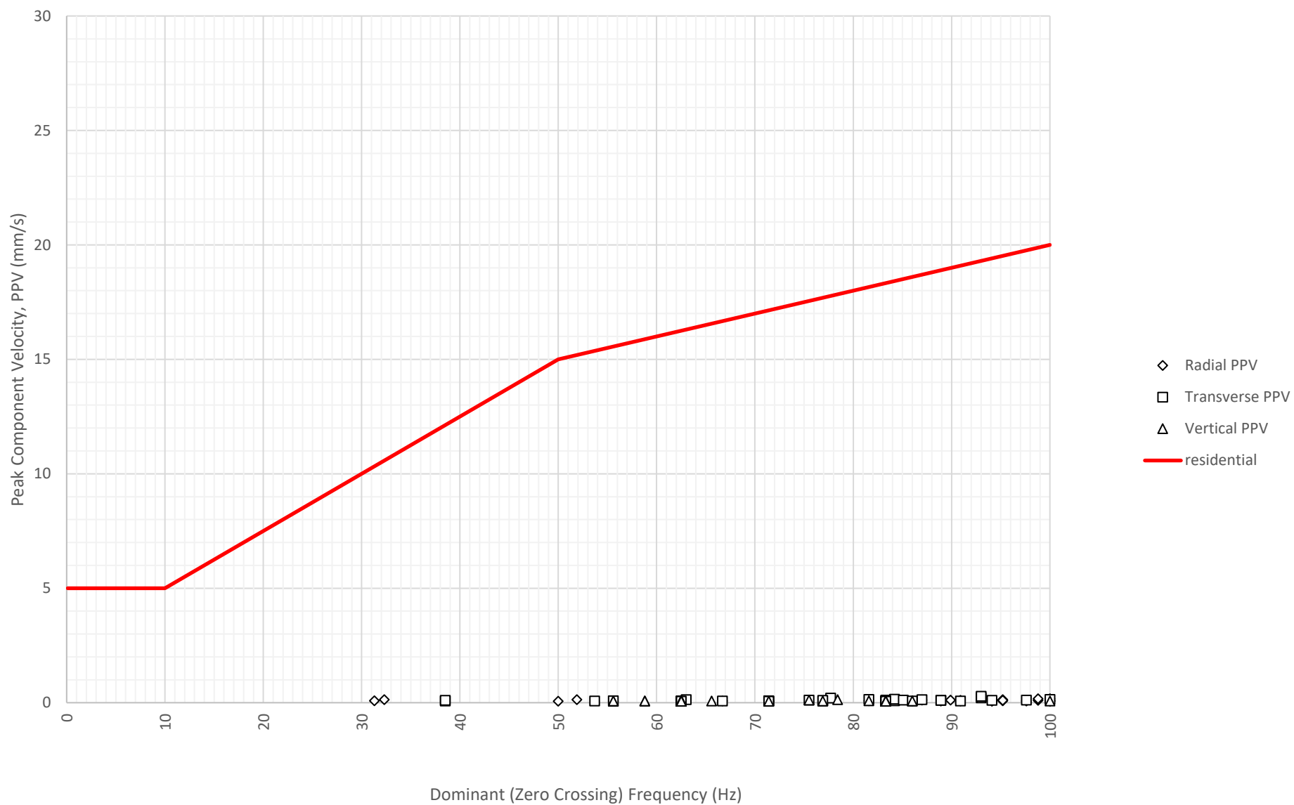
Frequency Content of Vibration Levels at North Boundary Near Block A and B (ETM7687) on 13-08-2024
