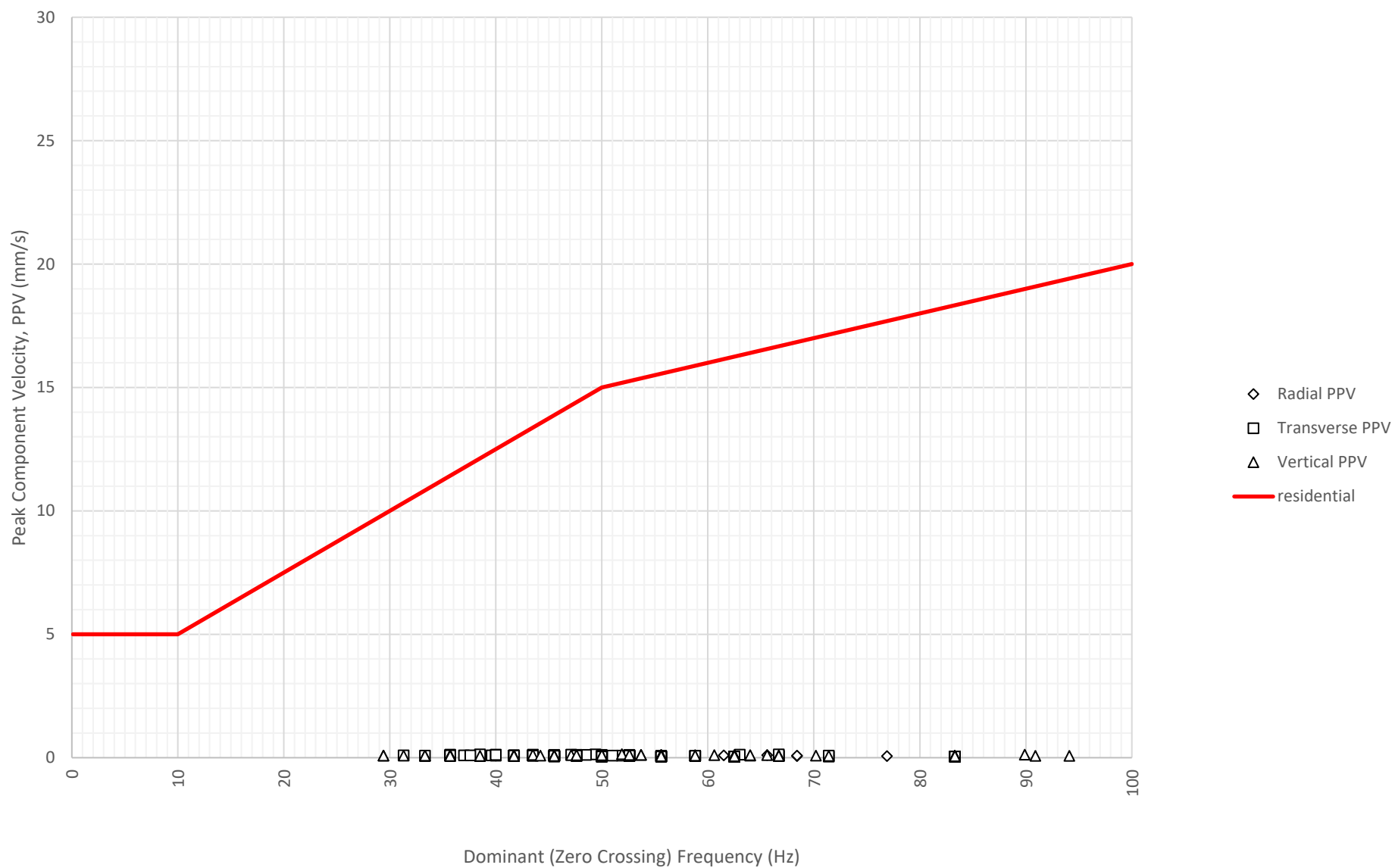
Frequency Content of Vibration Levels at East Boundary Opposite Shoalhaven Street (ETM7326) on 29-08-2024
