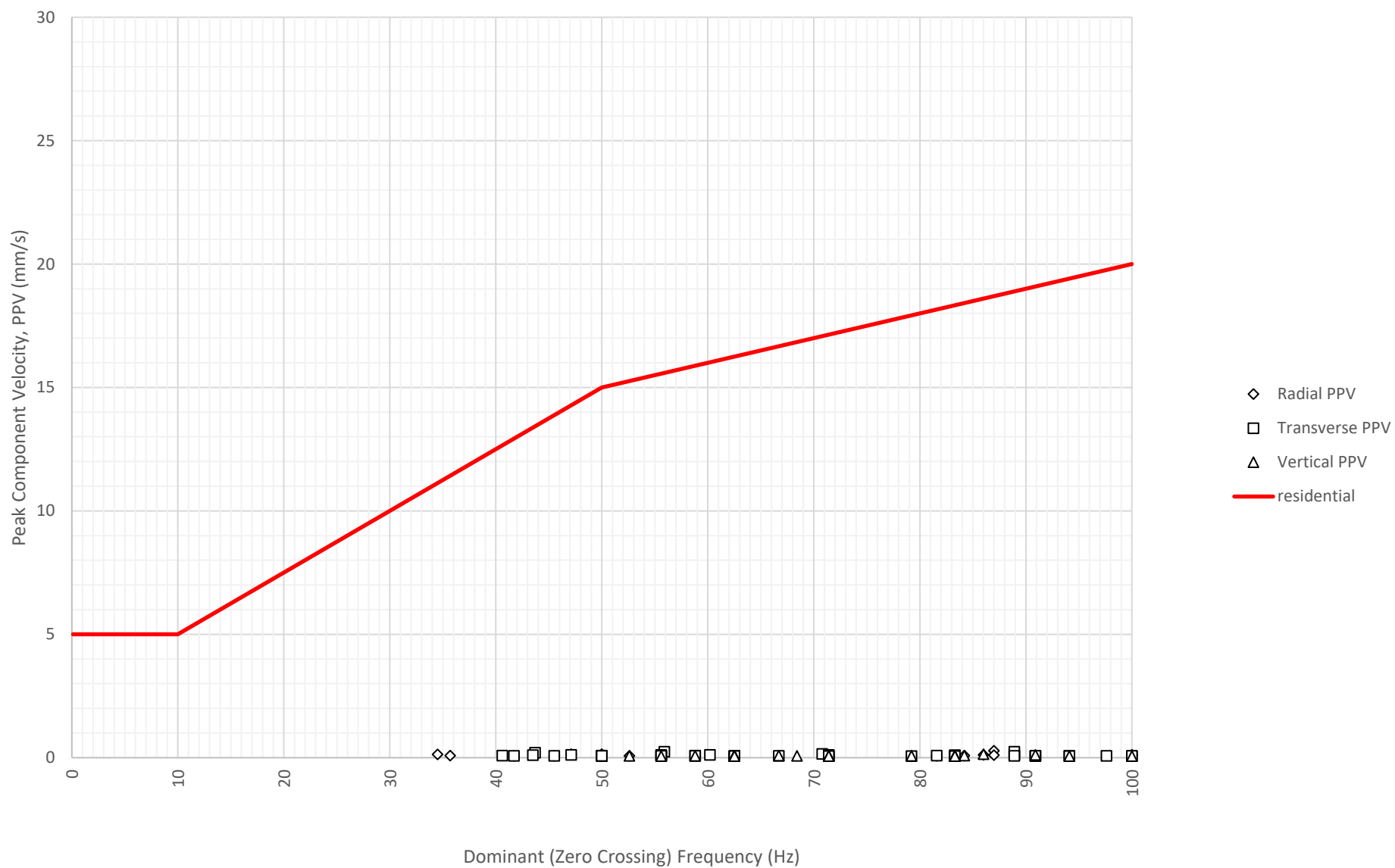
Frequency Content of Vibration Levels at North Boundary Near Block A and B (ETM7687) on 26-08-2024
