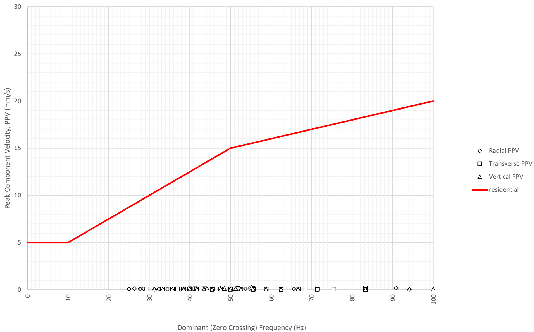
Frequency Content of Vibration Levels at East Boundary Opposite Shoalhaven Street (ETM7326) on 15-08-2024
