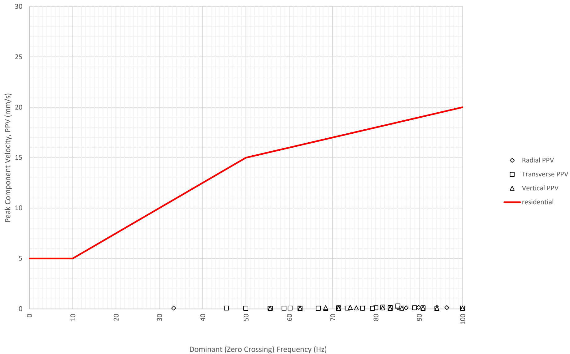
Frequency Content of Vibration Levels at North Boundary Near Block A and B (ETM7687) on 14-08-2024
