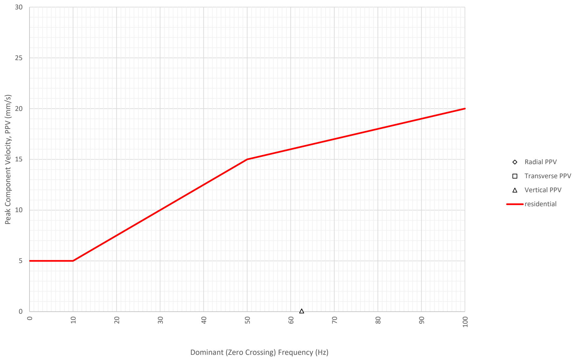
Frequency Content of Vibration Levels at East Boundary Opposite Shoalhaven Street (ETM7326) on 18-08-2024
