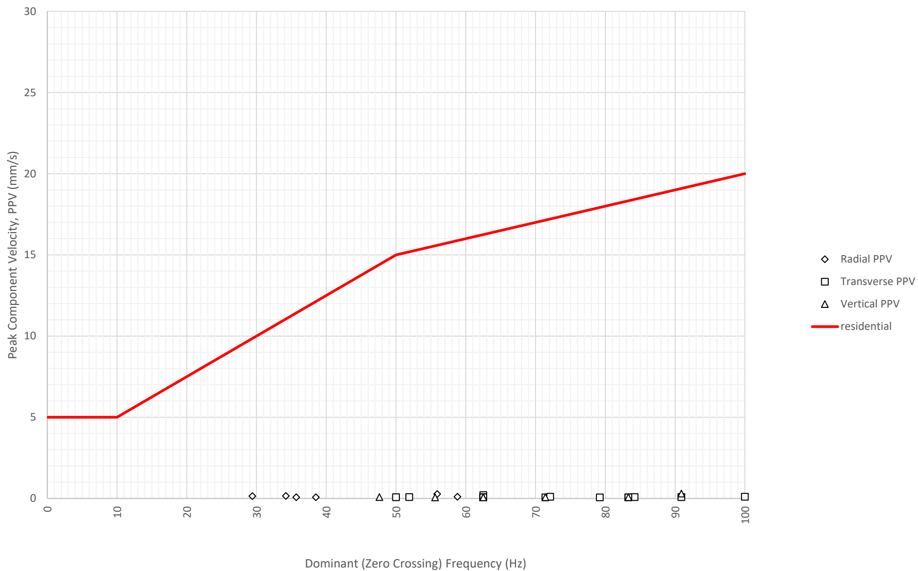
Frequency Content of Vibration Levels at North Boundary Near Block A and B (ETM7687) on 24-08-2024
