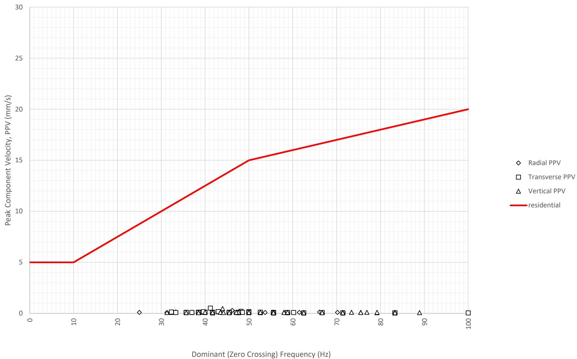
Frequency Content of Vibration Levels at East Boundary Opposite Shoalhaven Street (ETM7326) on 27-08-2024
