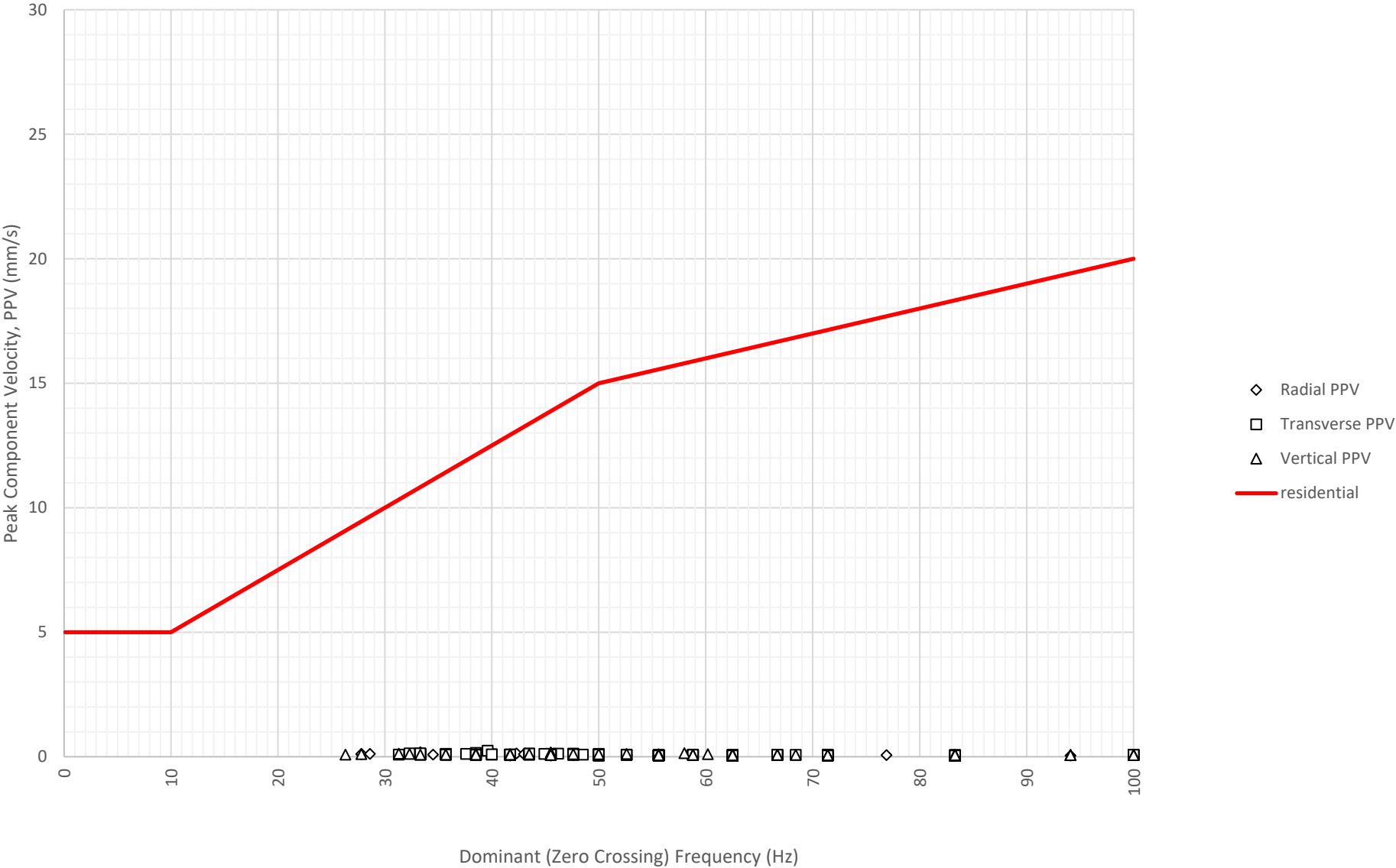
Frequency Content of Vibration Levels at East Boundary Opposite Shoalhaven Street (ETM7326) on 6-08-2024
