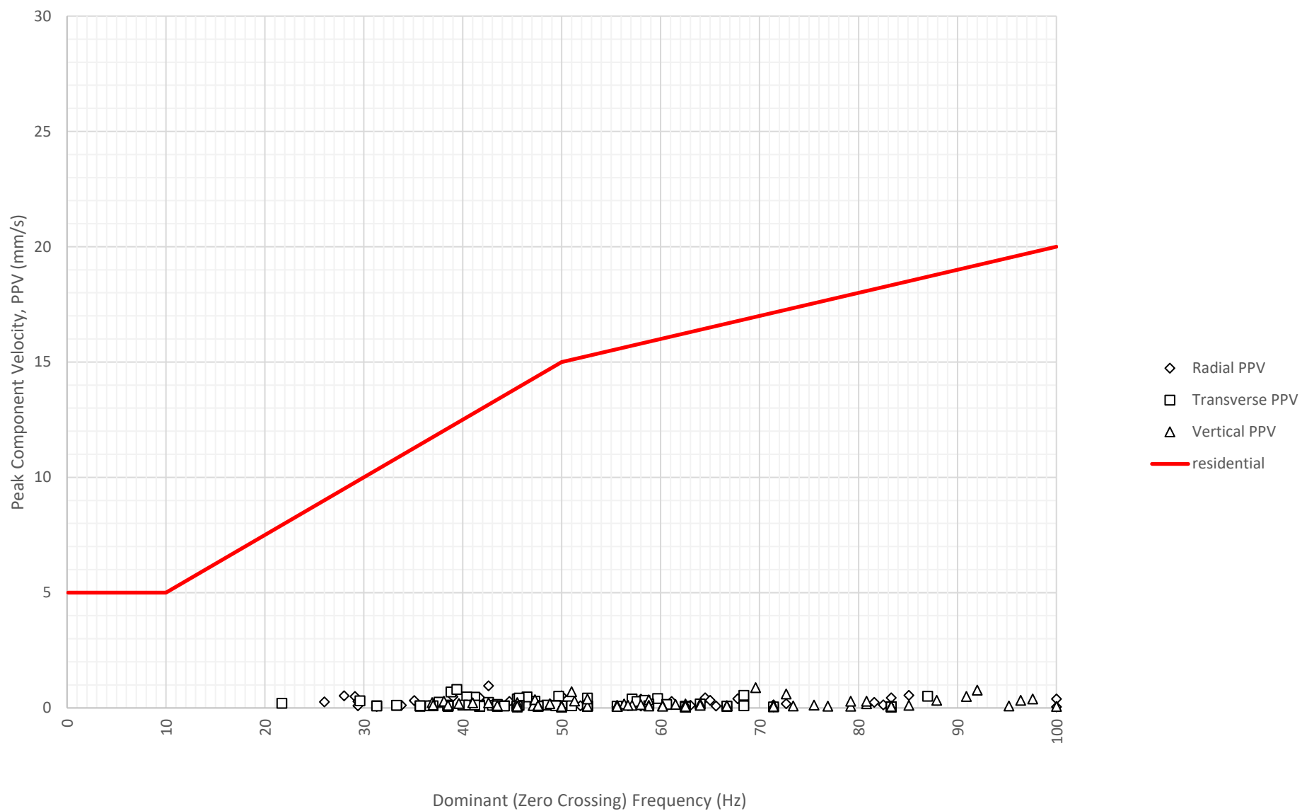
Frequency Content of Vibration Levels at East Boundary Opposite Shoalhaven Street (ETM7326) on 30-08-2024
