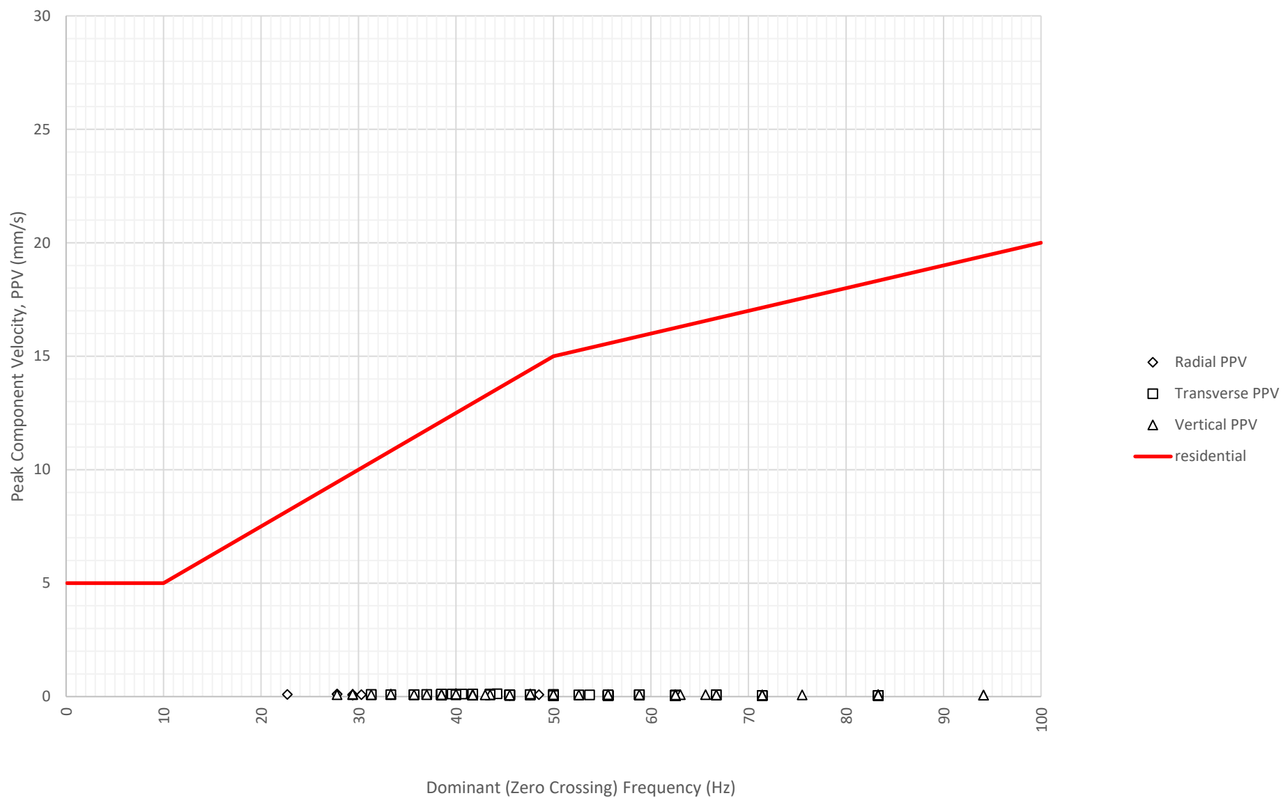
Frequency Content of Vibration Levels at East Boundary Opposite Shoalhaven Street (ETM7326) on 17-08-2024
