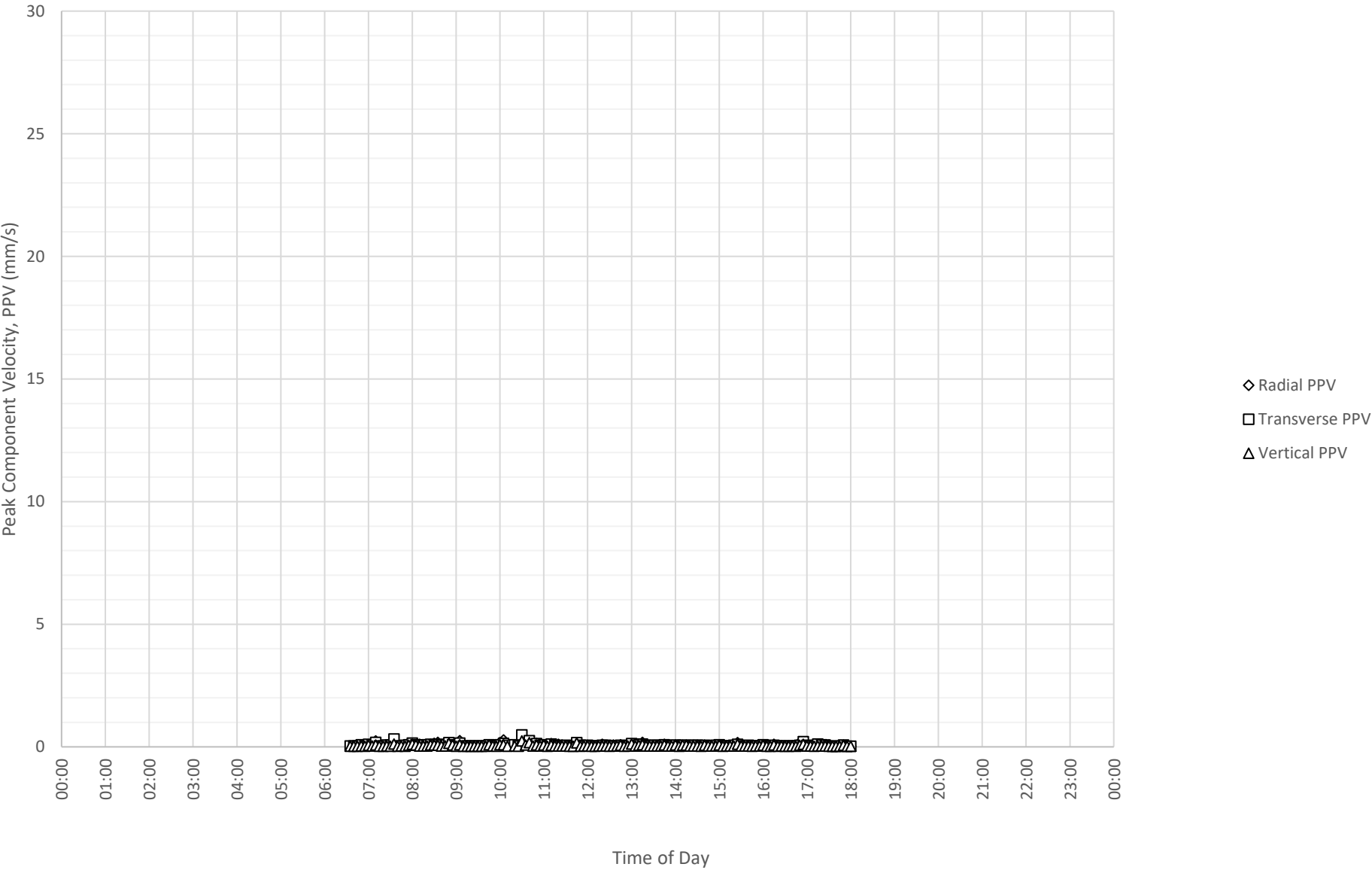
Daily Monitored Vibration Levels at North Boundary Near Block A and B (ETM7687) on 22-08-2024
