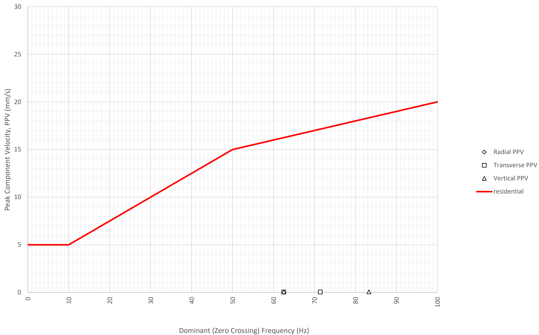
Frequency Content of Vibration Levels at East Boundary Opposite Shoalhaven Street (ETM7326) on 11-08-2024
