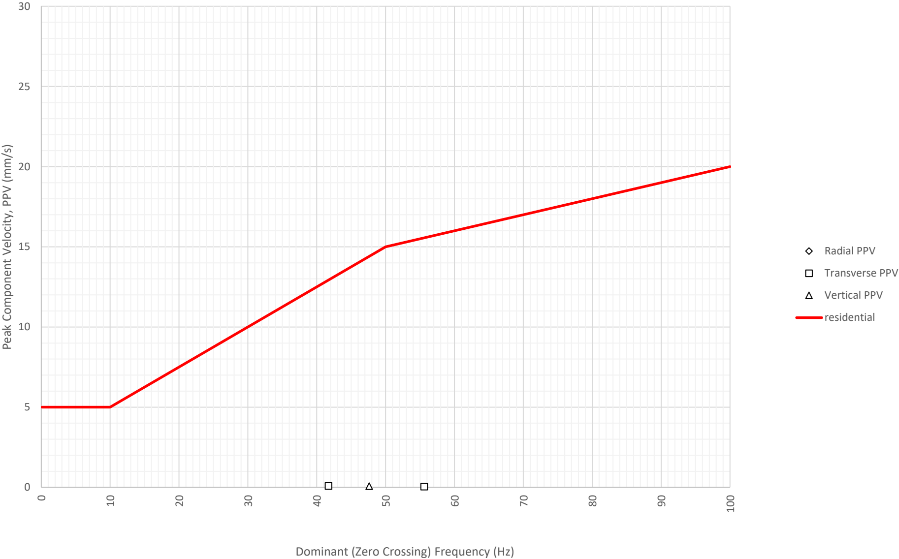
Frequency Content of Vibration Levels at East Boundary Opposite Shoalhaven Street (ETM7326) on 4-08-2024
