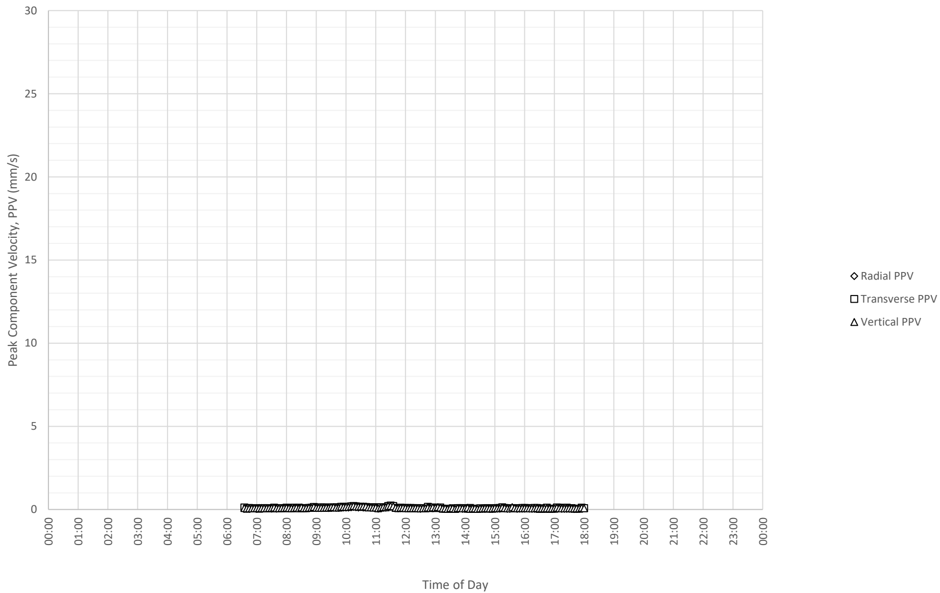
Daily Monitored Vibration Levels at East Boundary Opposite Shoalhaven Street (ETM7326) on 8-08-2024
