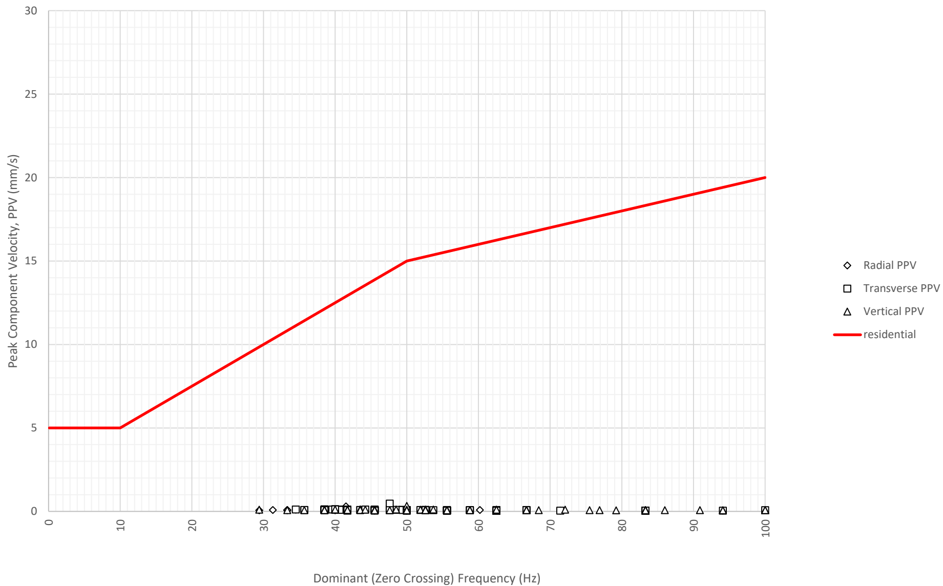
Frequency Content of Vibration Levels at East Boundary Opposite Shoalhaven Street (ETM7326) on 7-08-2024
