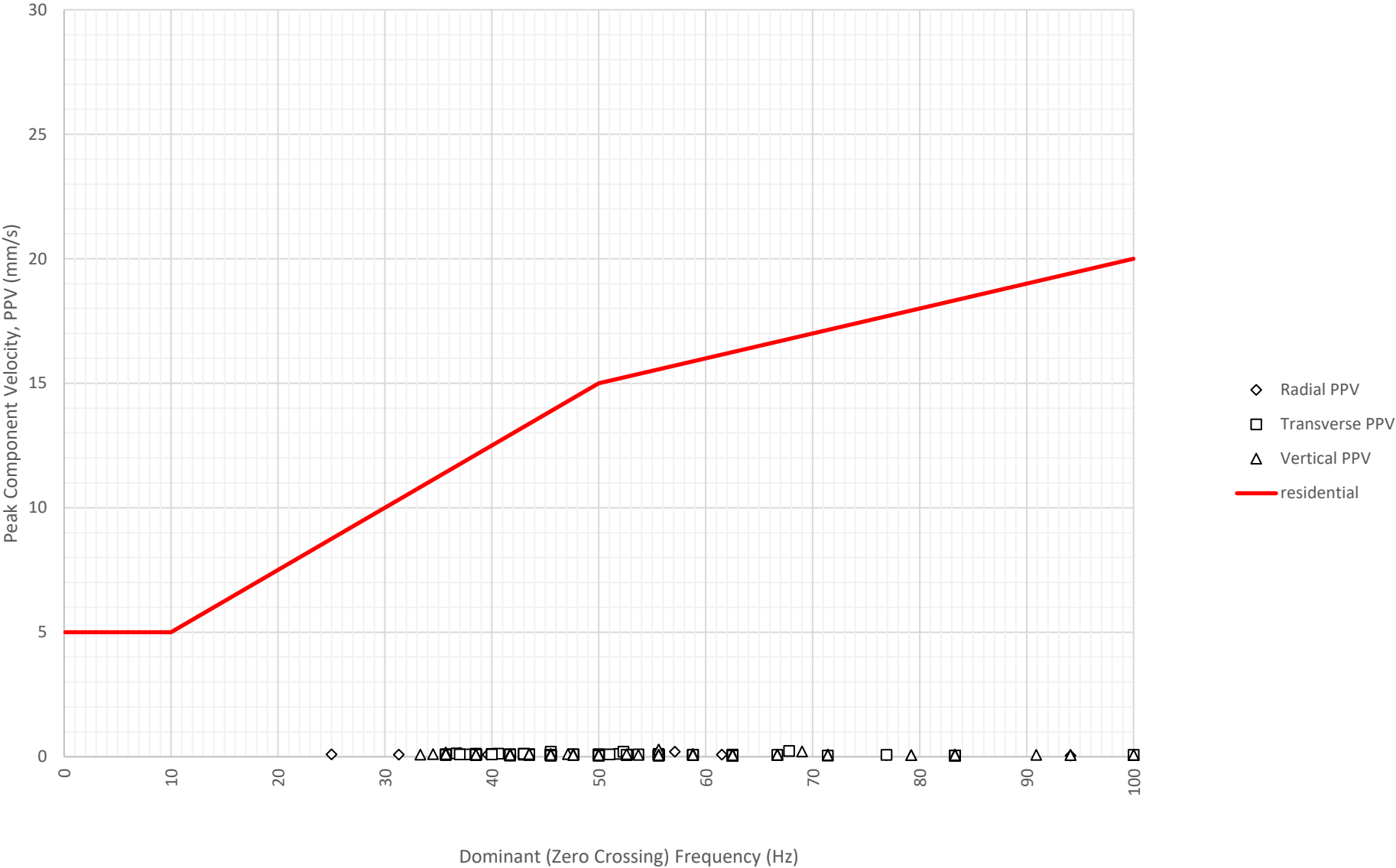
Frequency Content of Vibration Levels at East Boundary Opposite Shoalhaven Street (ETM7326) on 1-08-2024
