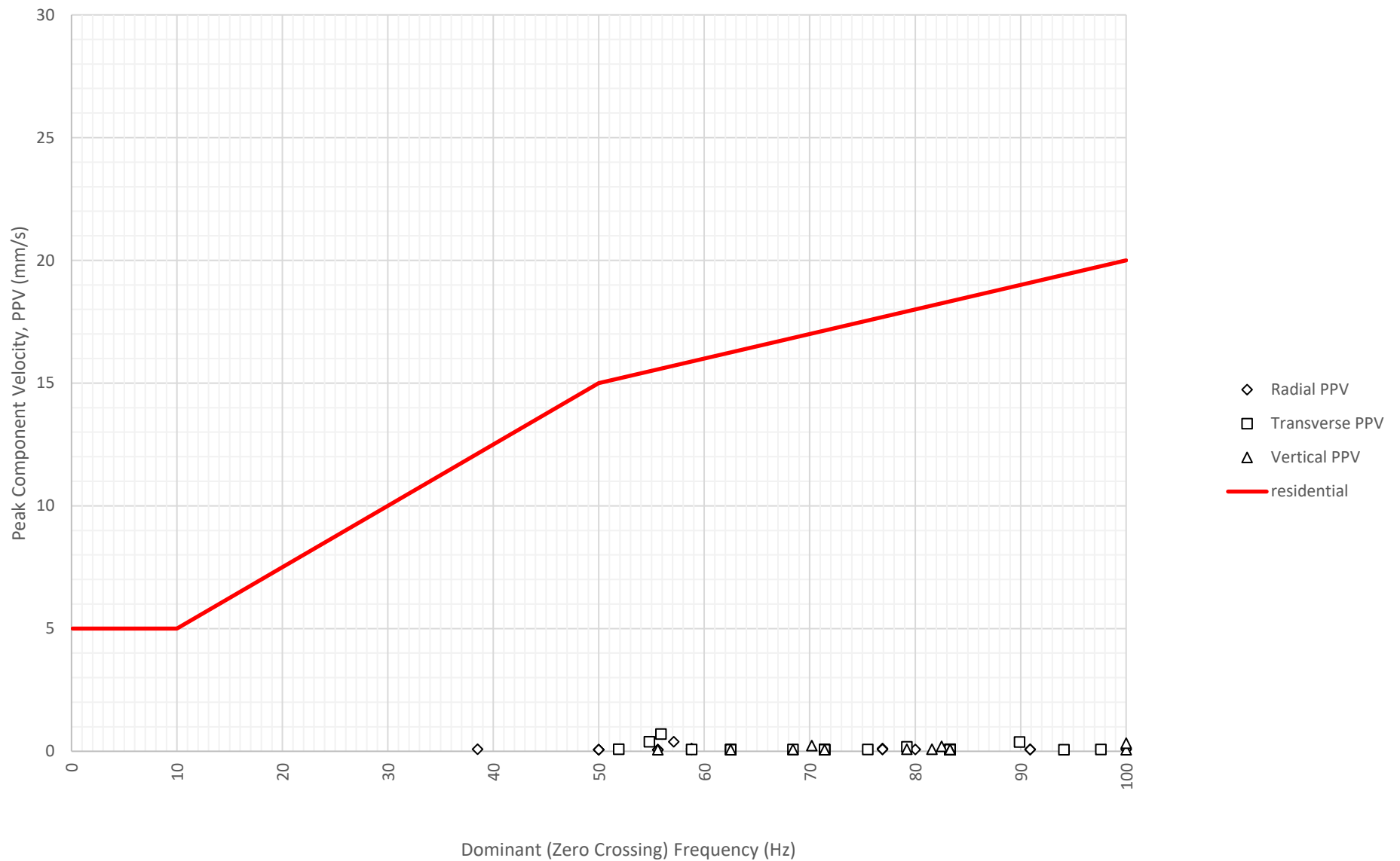
Frequency Content of Vibration Levels at North Boundary Near Block A and B (ETM7687) on 5-08-2024
