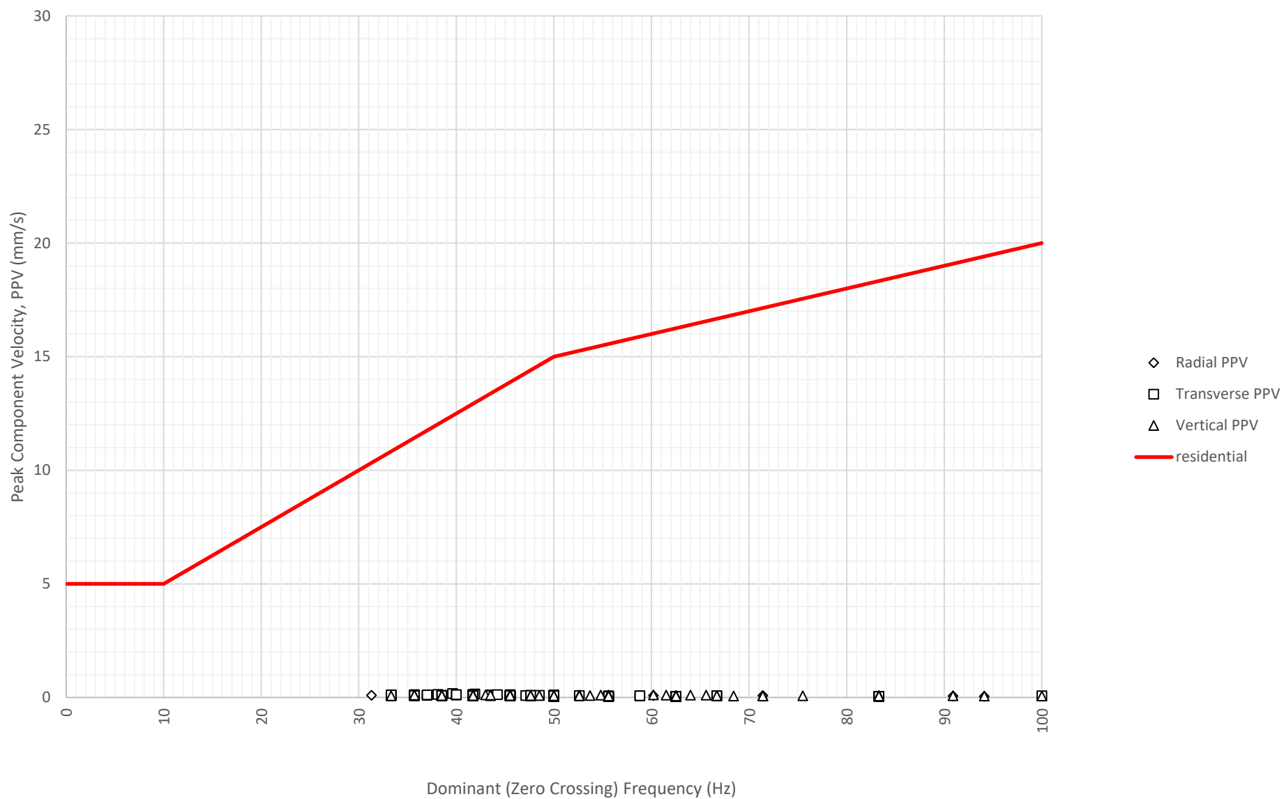
Frequency Content of Vibration Levels at East Boundary Opposite Shoalhaven Street (ETM7326) on 23-08-2024
