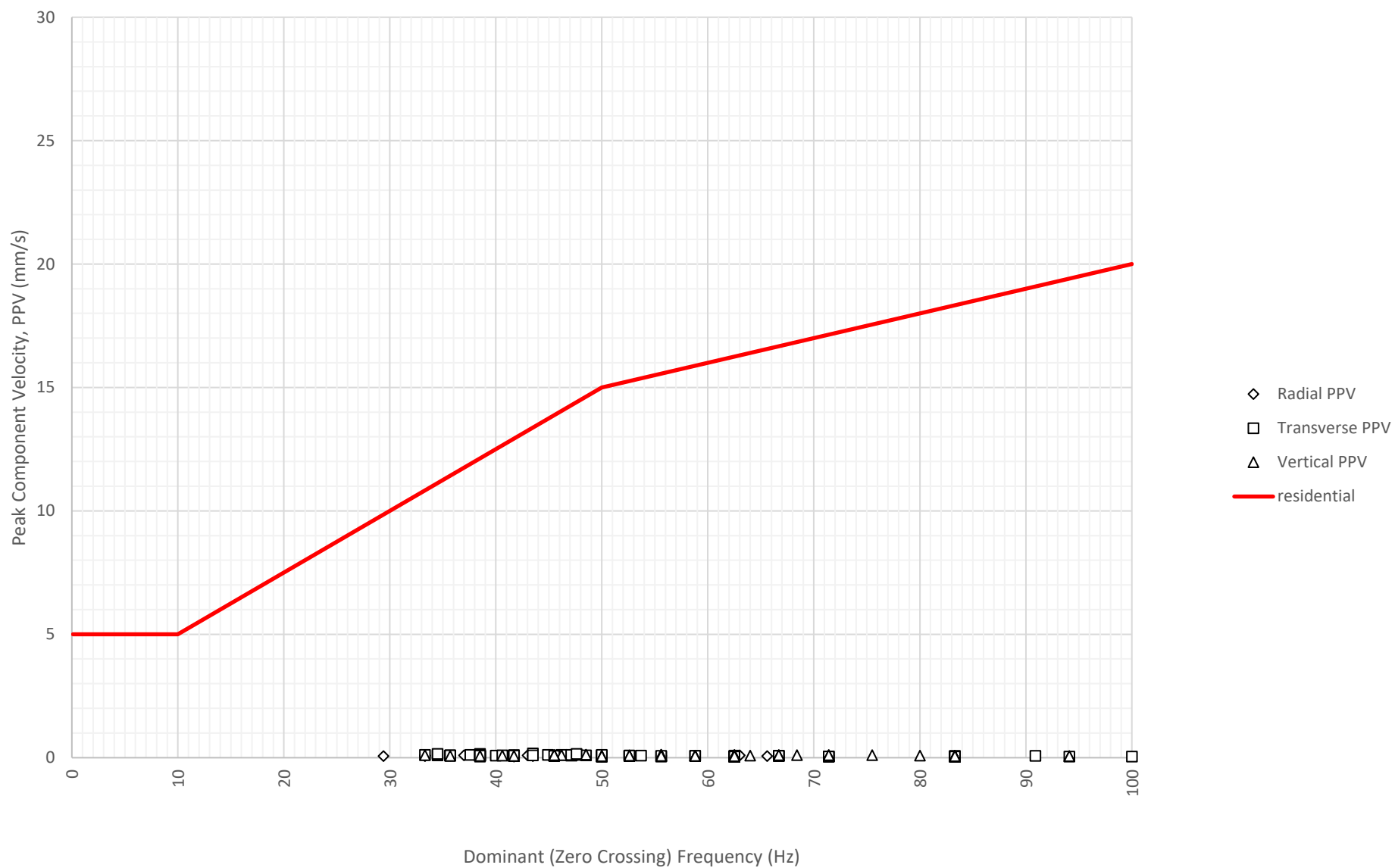
Frequency Content of Vibration Levels at East Boundary Opposite Shoalhaven Street (ETM7326) on 10-08-2024
