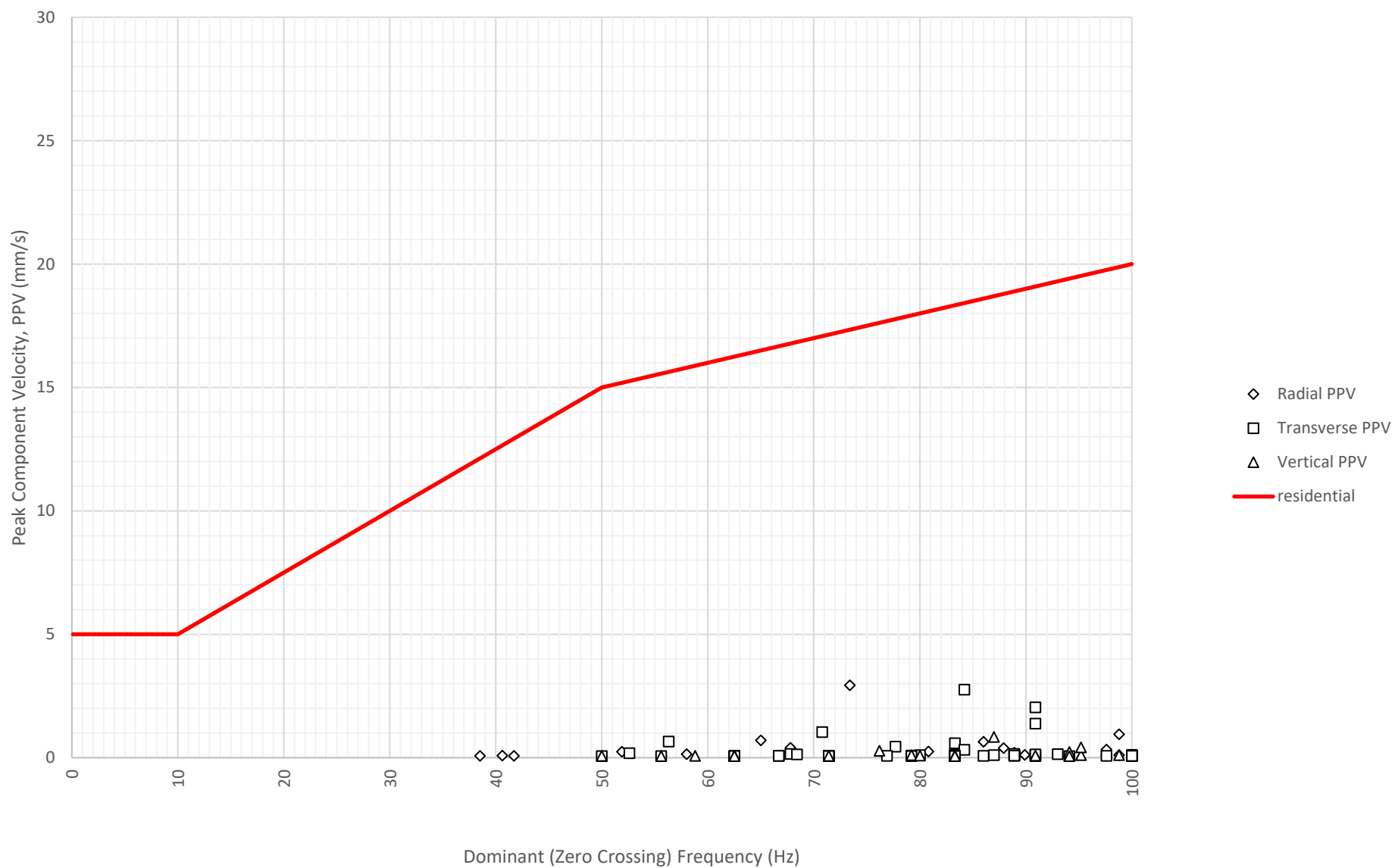
Frequency Content of Vibration Levels at North Boundary Near Block A and B (ETM7687) on 21-08-2024
