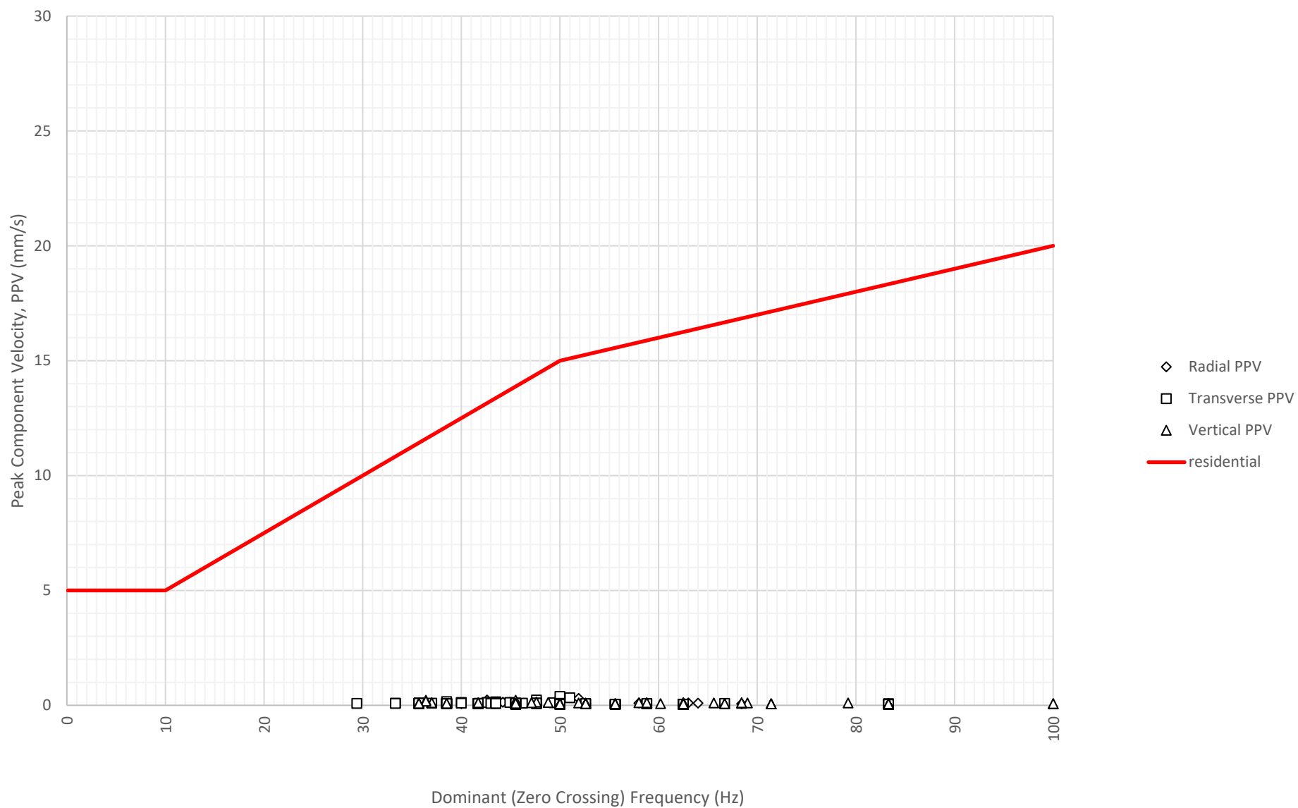
Frequency Content of Vibration Levels at East Boundary Opposite Shoalhaven Street (ETM7326) on 28-08-2024
