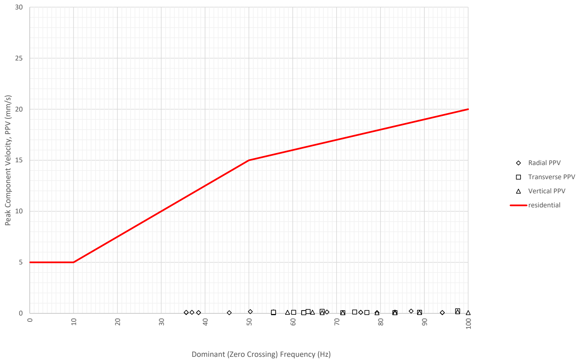
Frequency Content of Vibration Levels at North Boundary Near Block A and B (ETM7687) on 12-08-2024
