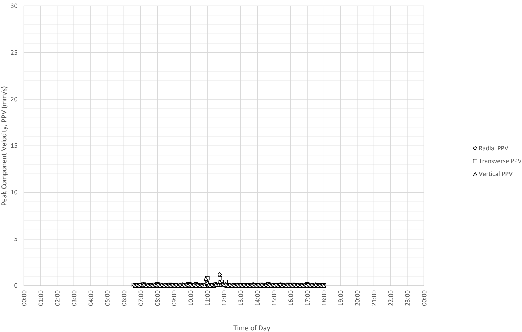
Daily Monitored Vibration Levels at North Boundary Near Block A and B (ETM7687) on 15-08-2024
