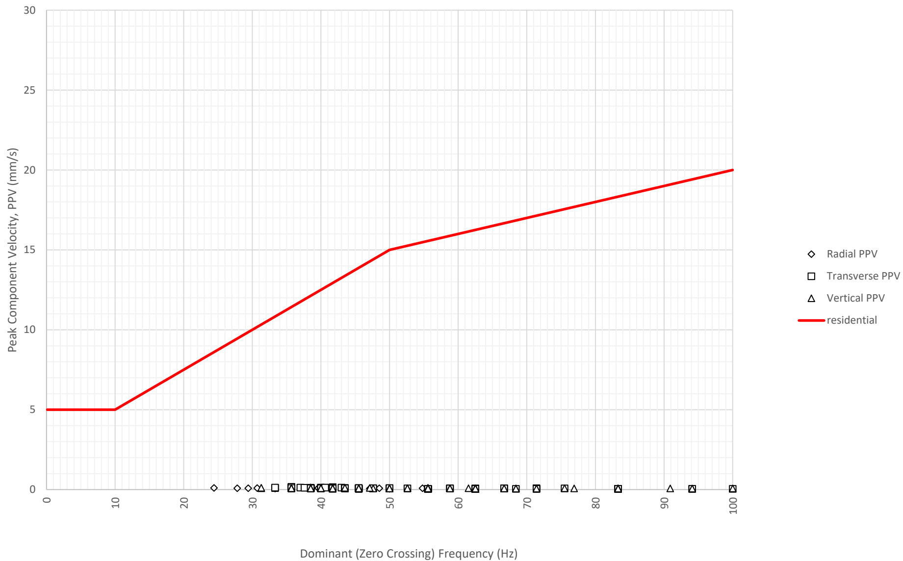
Frequency Content of Vibration Levels at East Boundary Opposite Shoalhaven Street (ETM7326) on 13-08-2024
