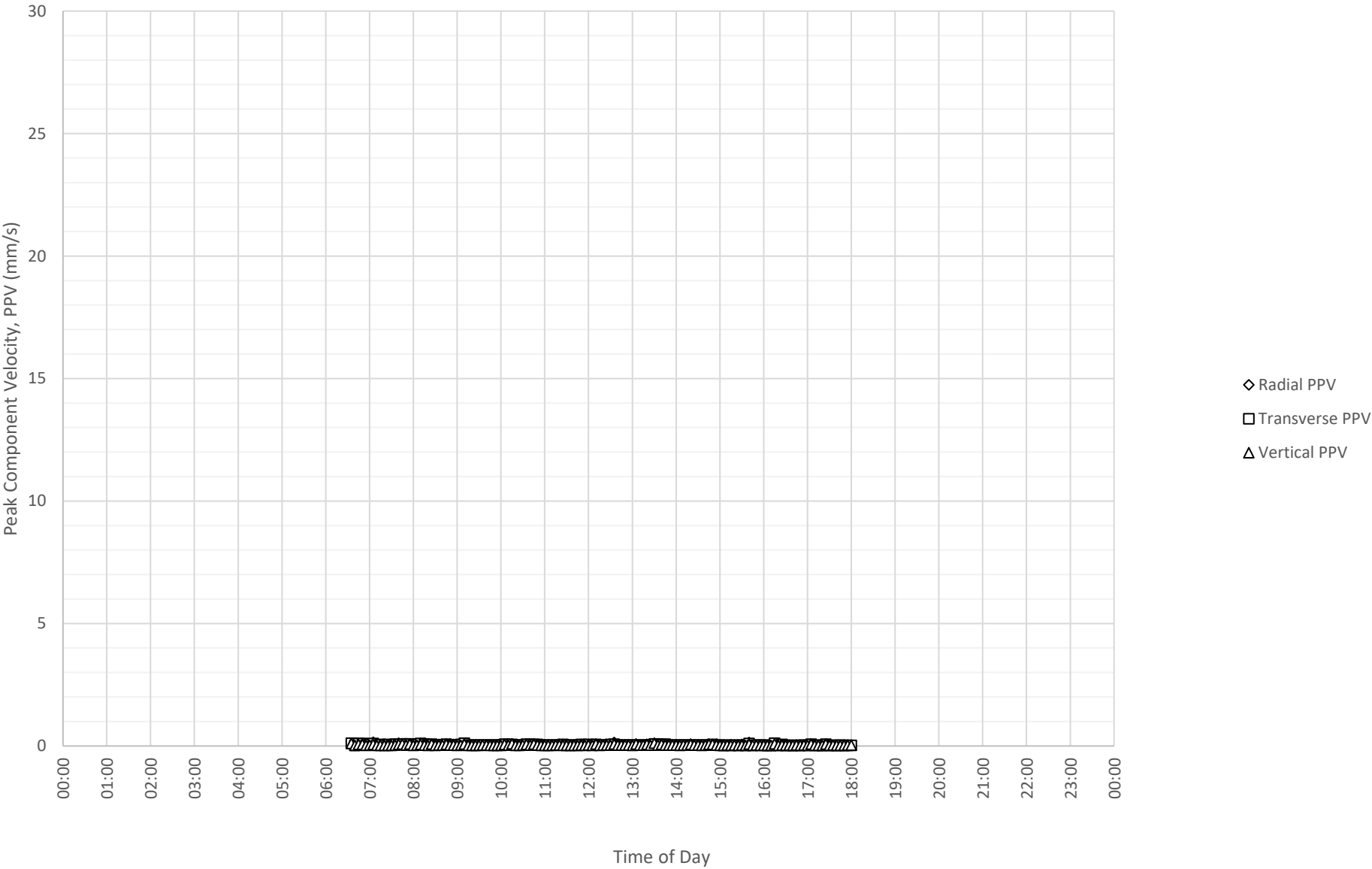
Daily Monitored Vibration Levels at North Boundary Near Block A and B (ETM7687) on 27-08-2024
