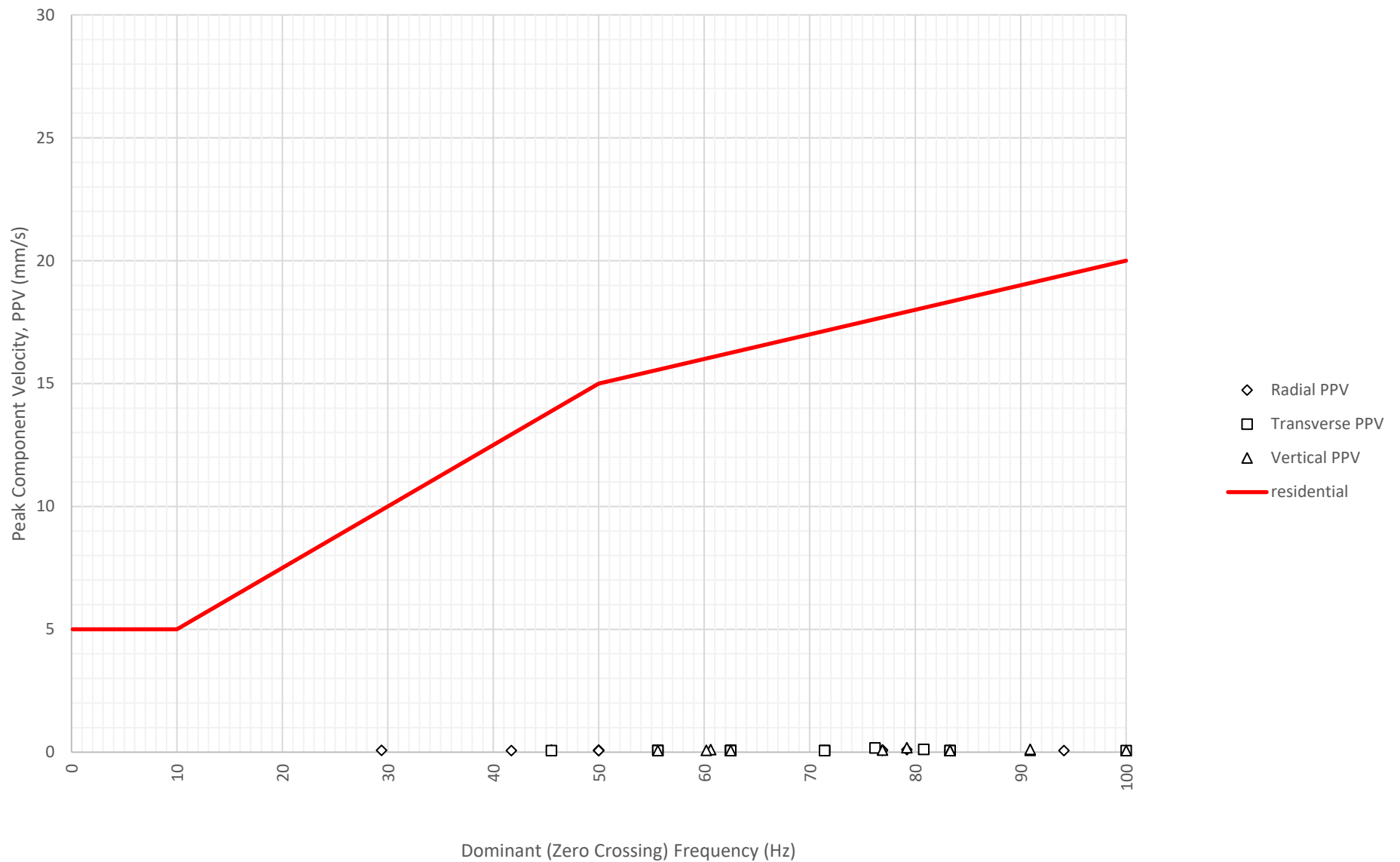
Frequency Content of Vibration Levels at North Boundary Near Block A and B (ETM7687) on 2-08-2024
