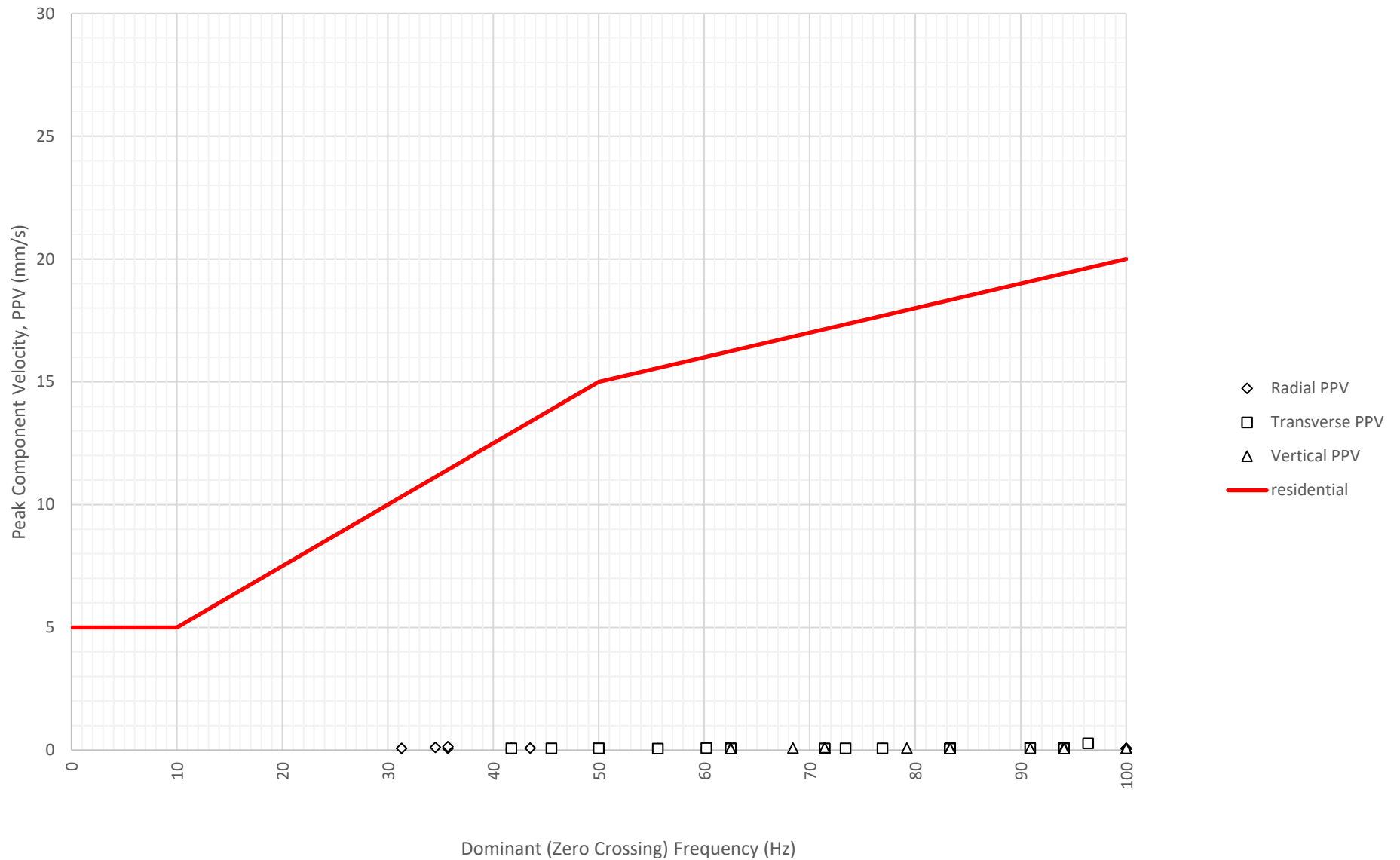
Frequency Content of Vibration Levels at North Boundary Near Block A and B (ETM7687) on 6-08-2024
