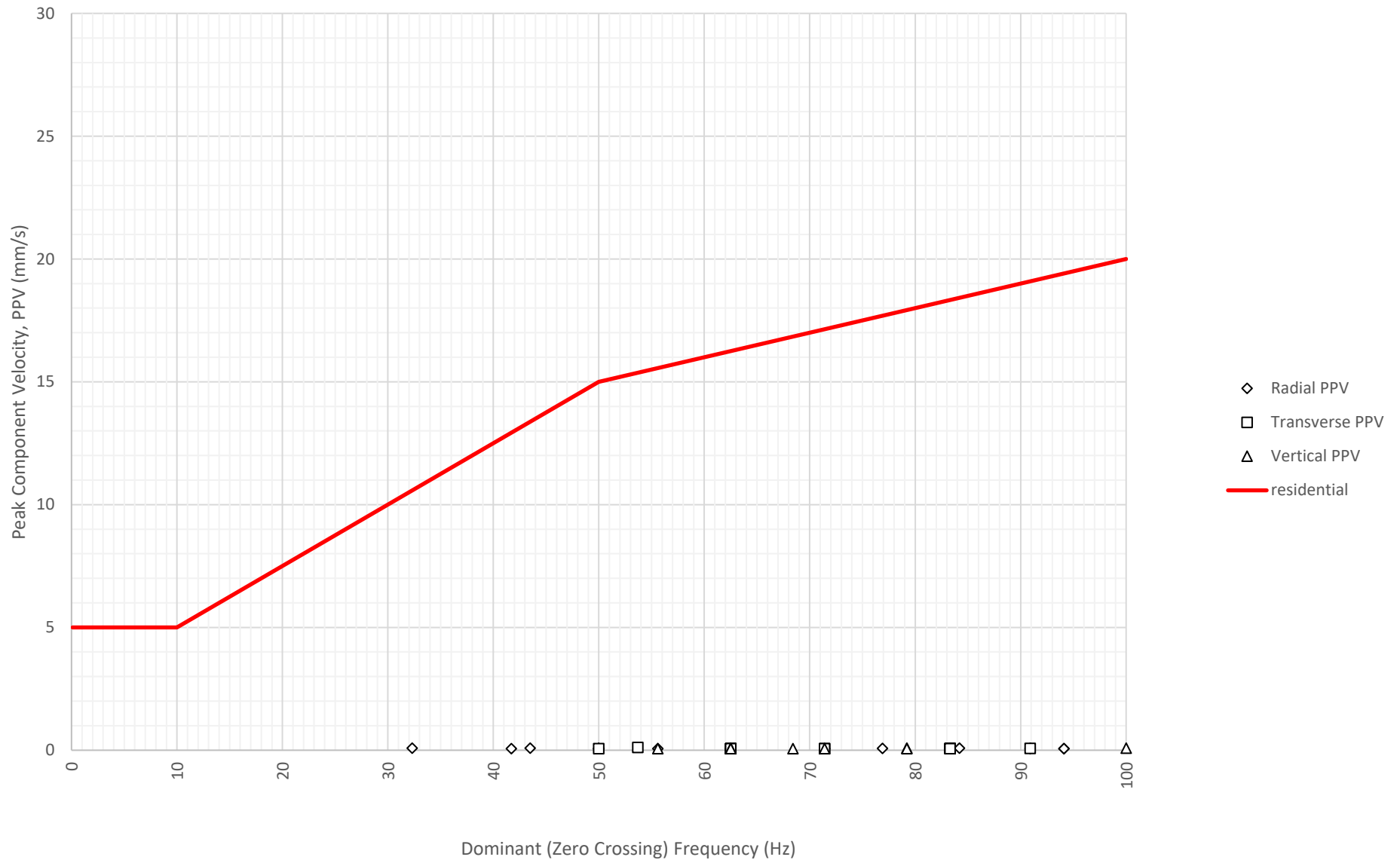
Frequency Content of Vibration Levels at North Boundary Near Block A and B (ETM7687) on 9-08-2024
