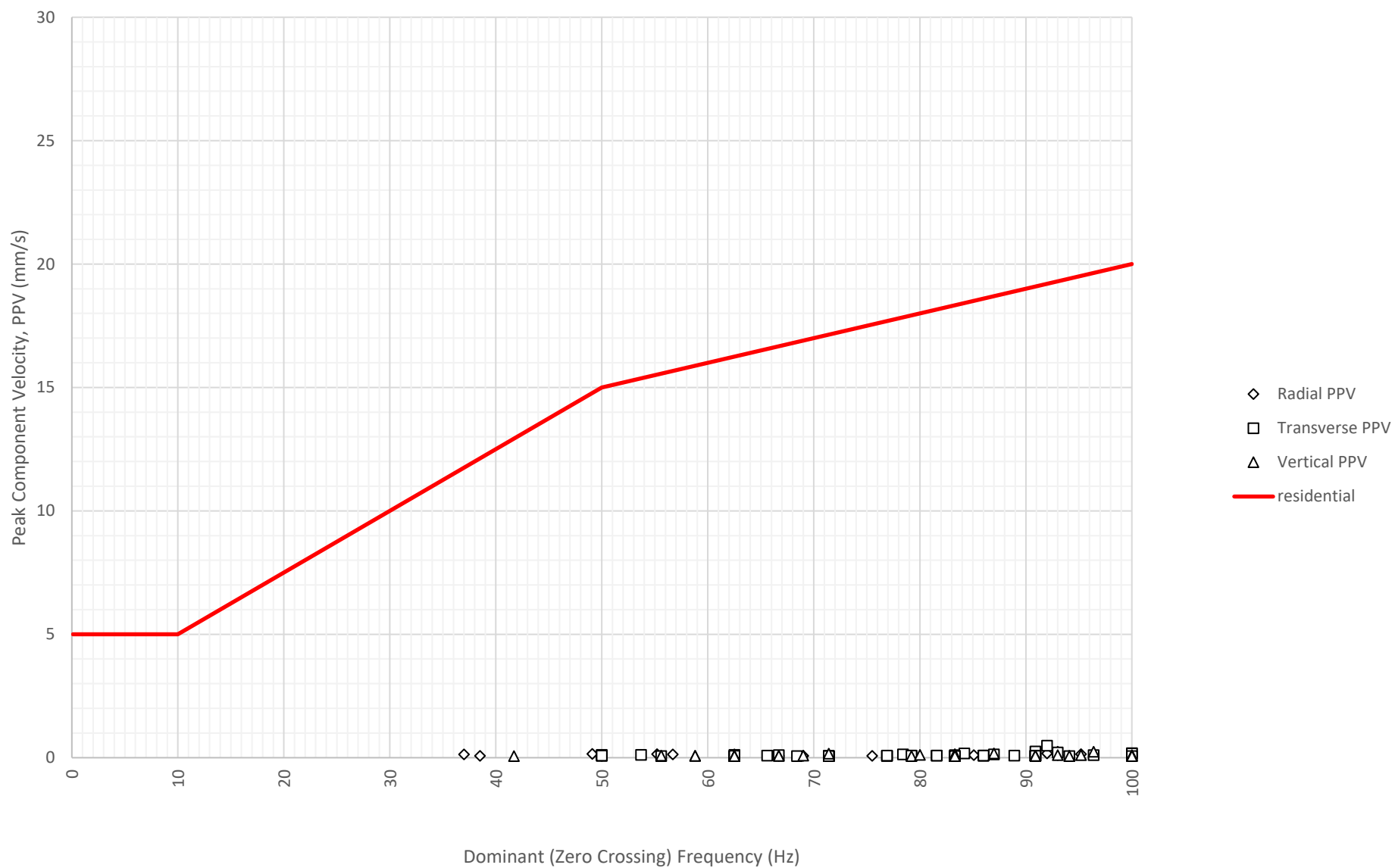
Frequency Content of Vibration Levels at North Boundary Near Block A and B (ETM7687) on 22-08-2024
