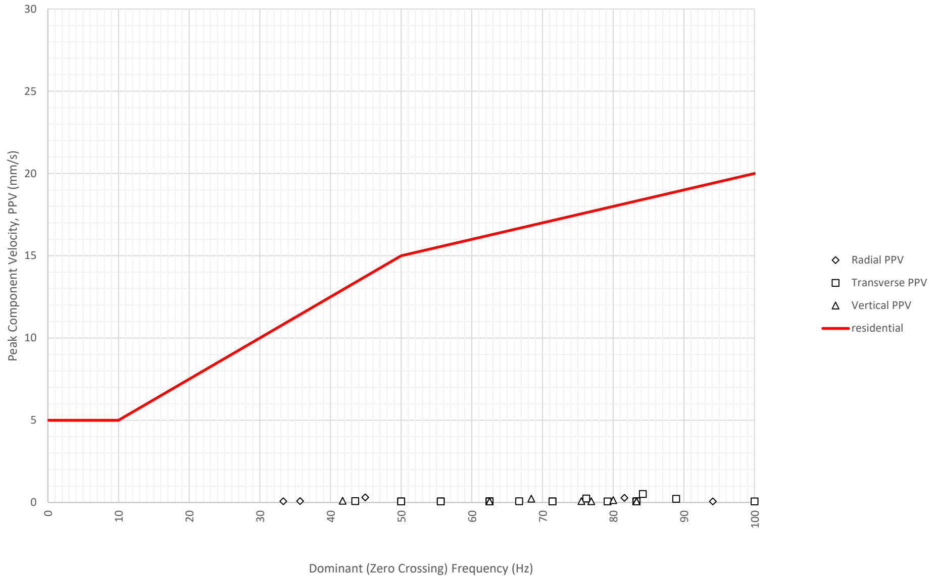
Frequency Content of Vibration Levels at North Boundary Near Block A and B (ETM7687) on 7-08-2024
