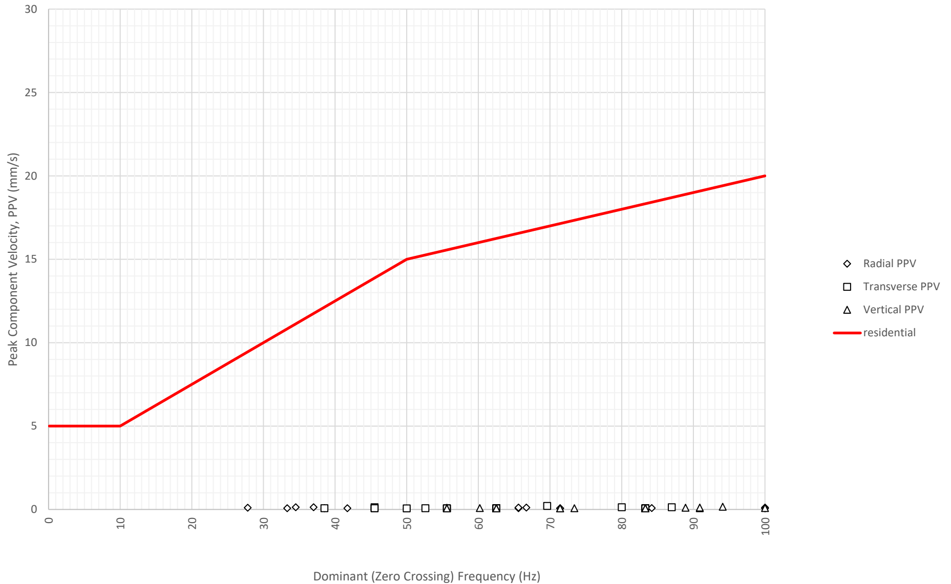
Frequency Content of Vibration Levels at North Boundary Near Block A and B (ETM7687) on 1-08-2024
