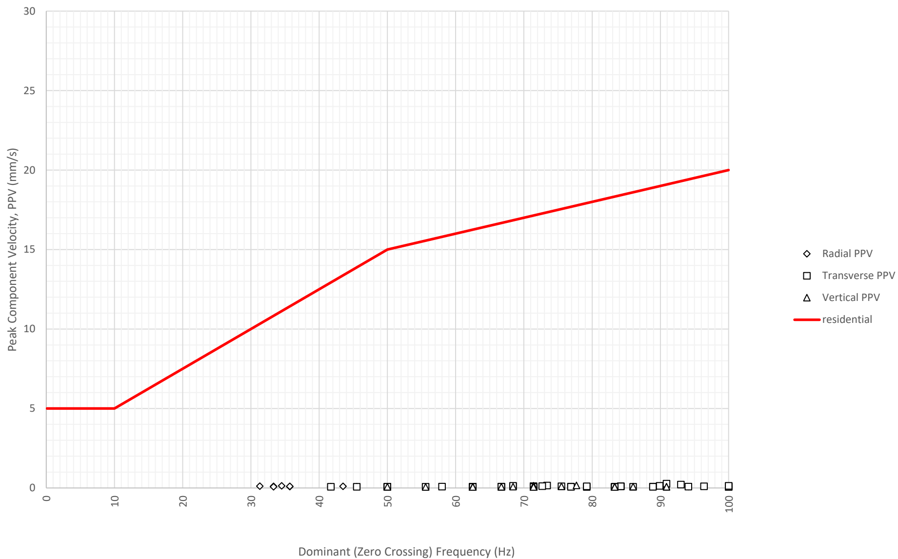
Frequency Content of Vibration Levels at North Boundary Near Block A and B (ETM7687) on 19-08-2024
