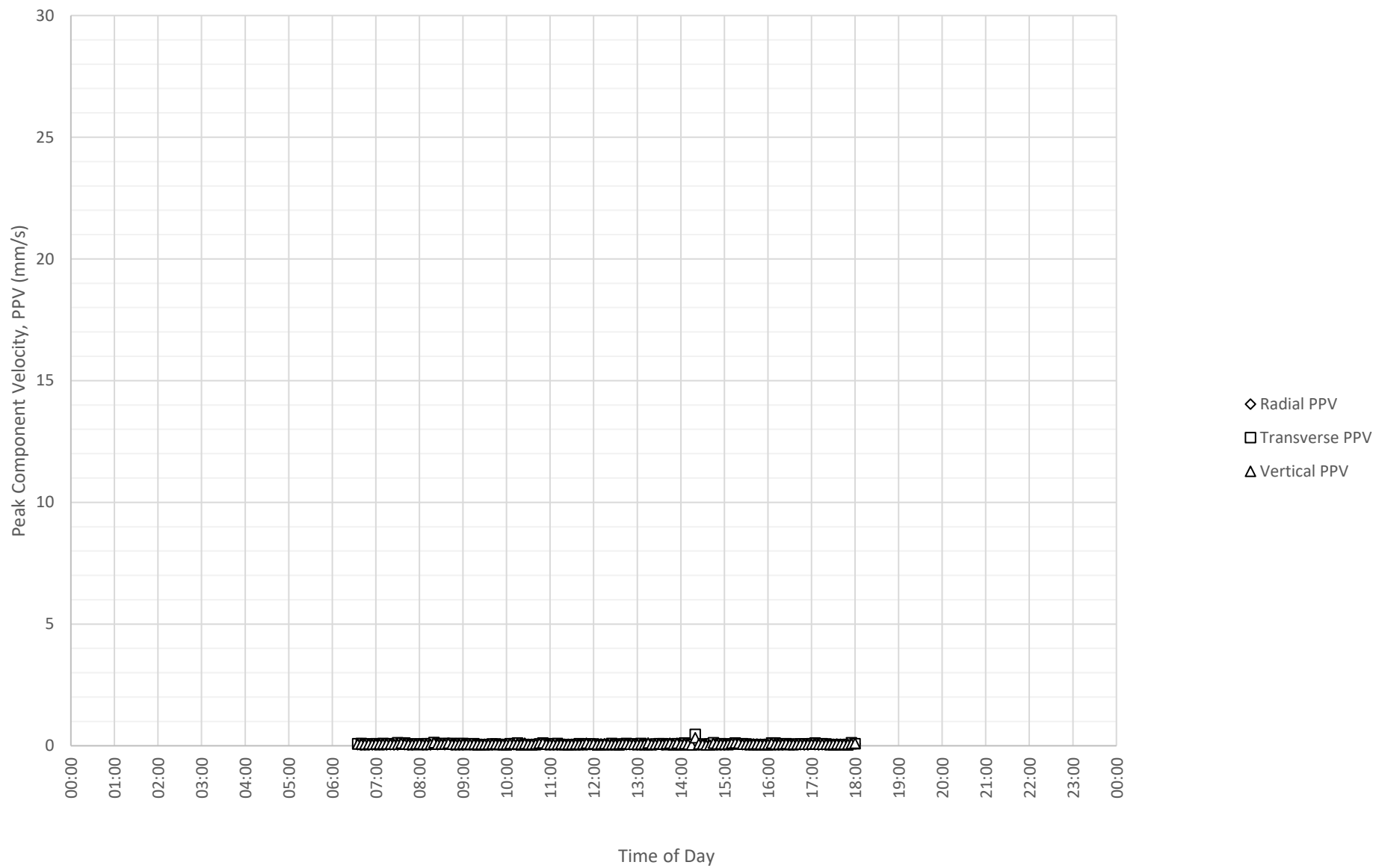
Daily Monitored Vibration Levels at East Boundary Opposite Shoalhaven Street (ETM7326) on 7-08-2024
