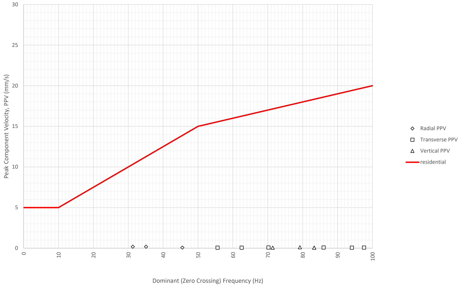
Frequency Content of Vibration Levels at North Boundary Near Block A and B (ETM7687) on 3-08-2024
