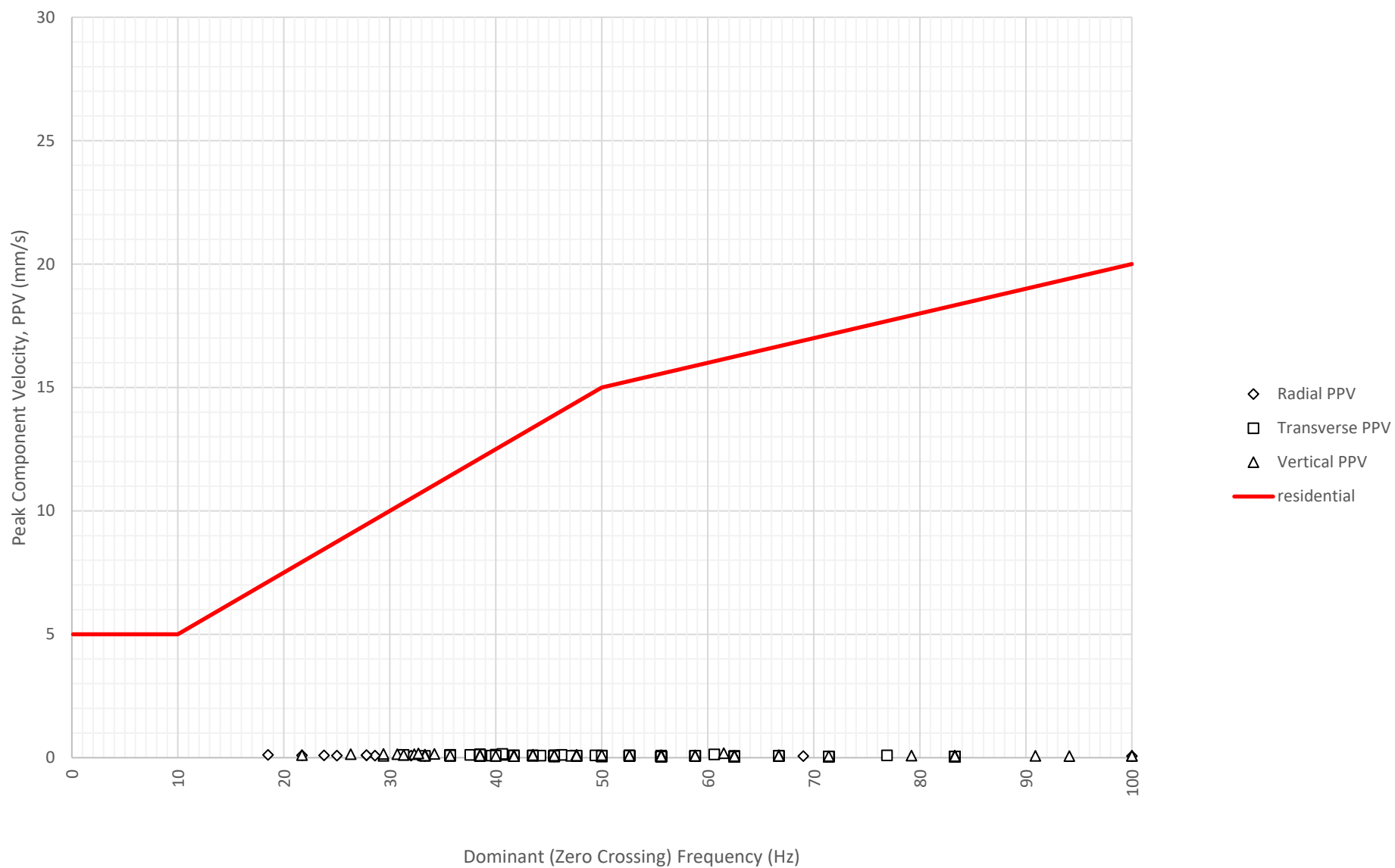
Frequency Content of Vibration Levels at East Boundary Opposite Shoalhaven Street (ETM7326) on 19-08-2024
