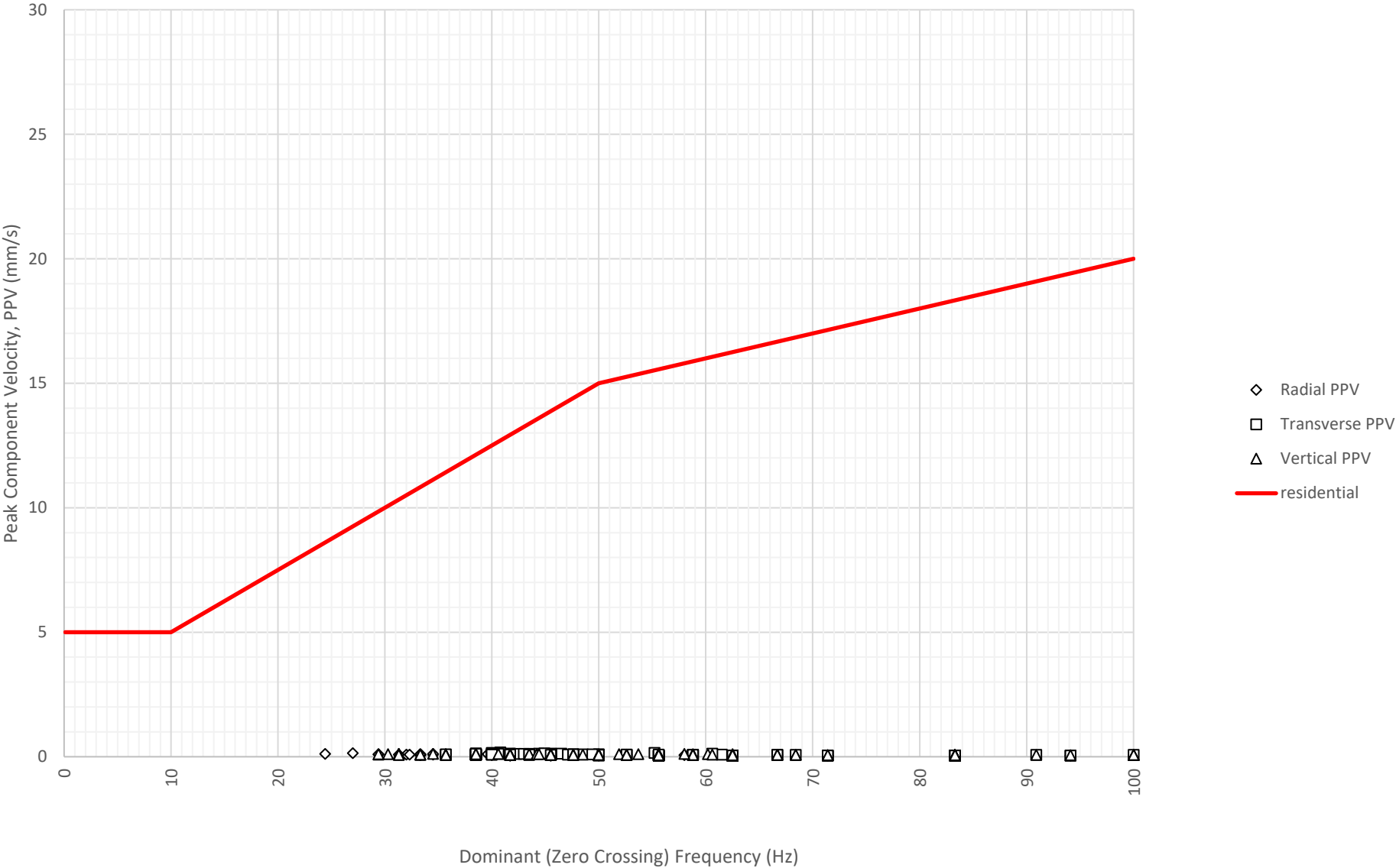
Frequency Content of Vibration Levels at East Boundary Opposite Shoalhaven Street (ETM7326) on 2-08-2024
