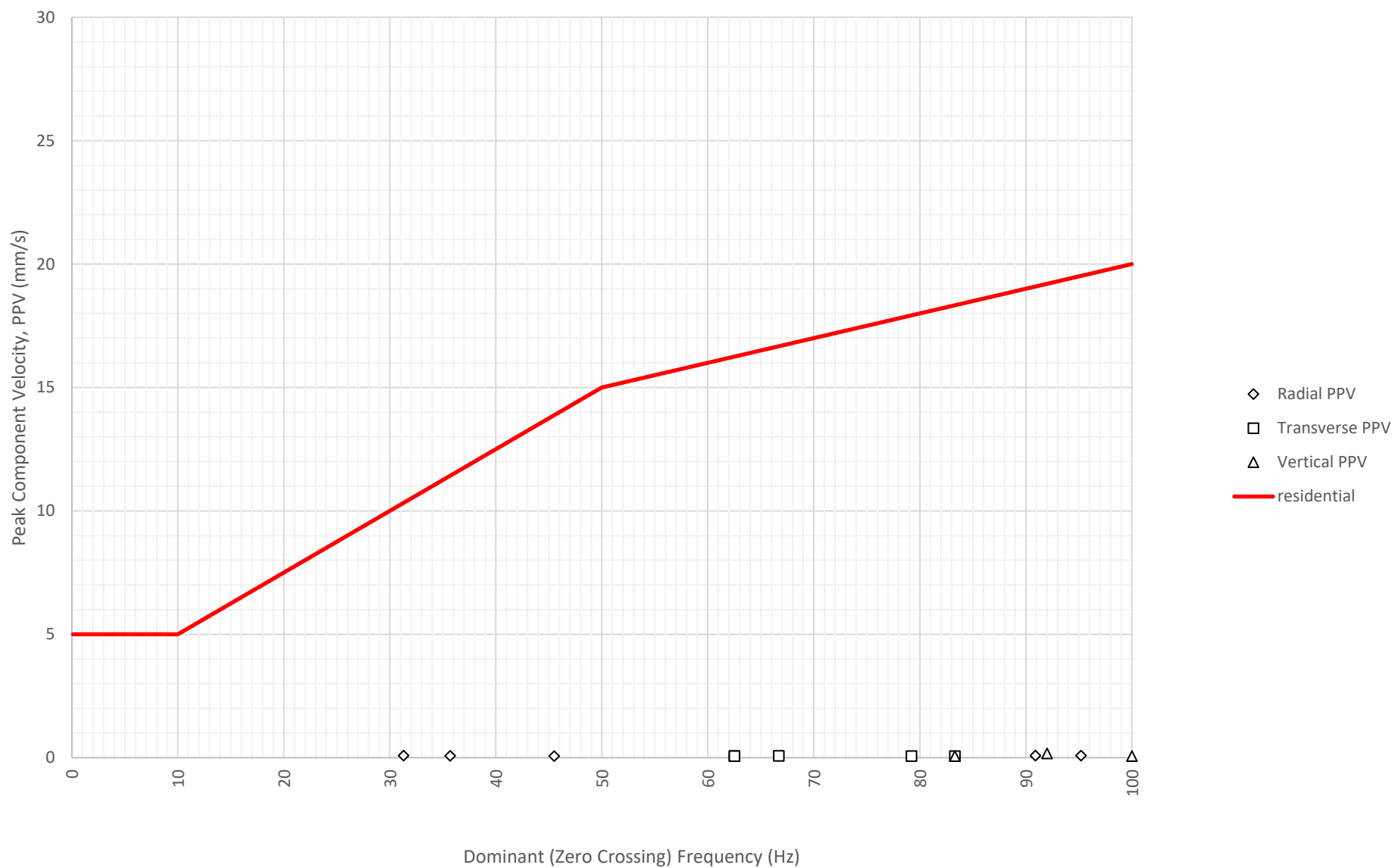
Frequency Content of Vibration Levels at North Boundary Near Block A and B (ETM7687) on 31-08-2024
