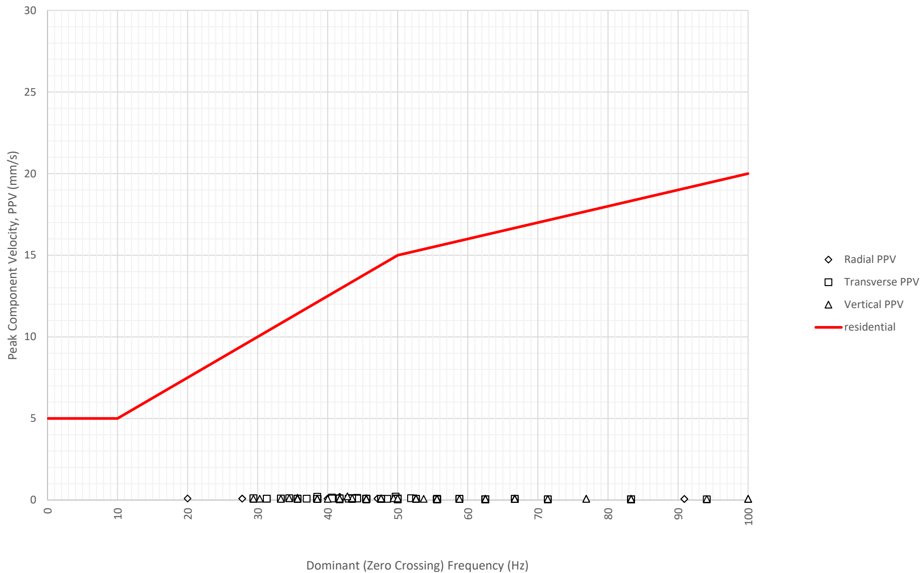
Frequency Content of Vibration Levels at East Boundary Opposite Shoalhaven Street (ETM7326) on 22-08-2024
