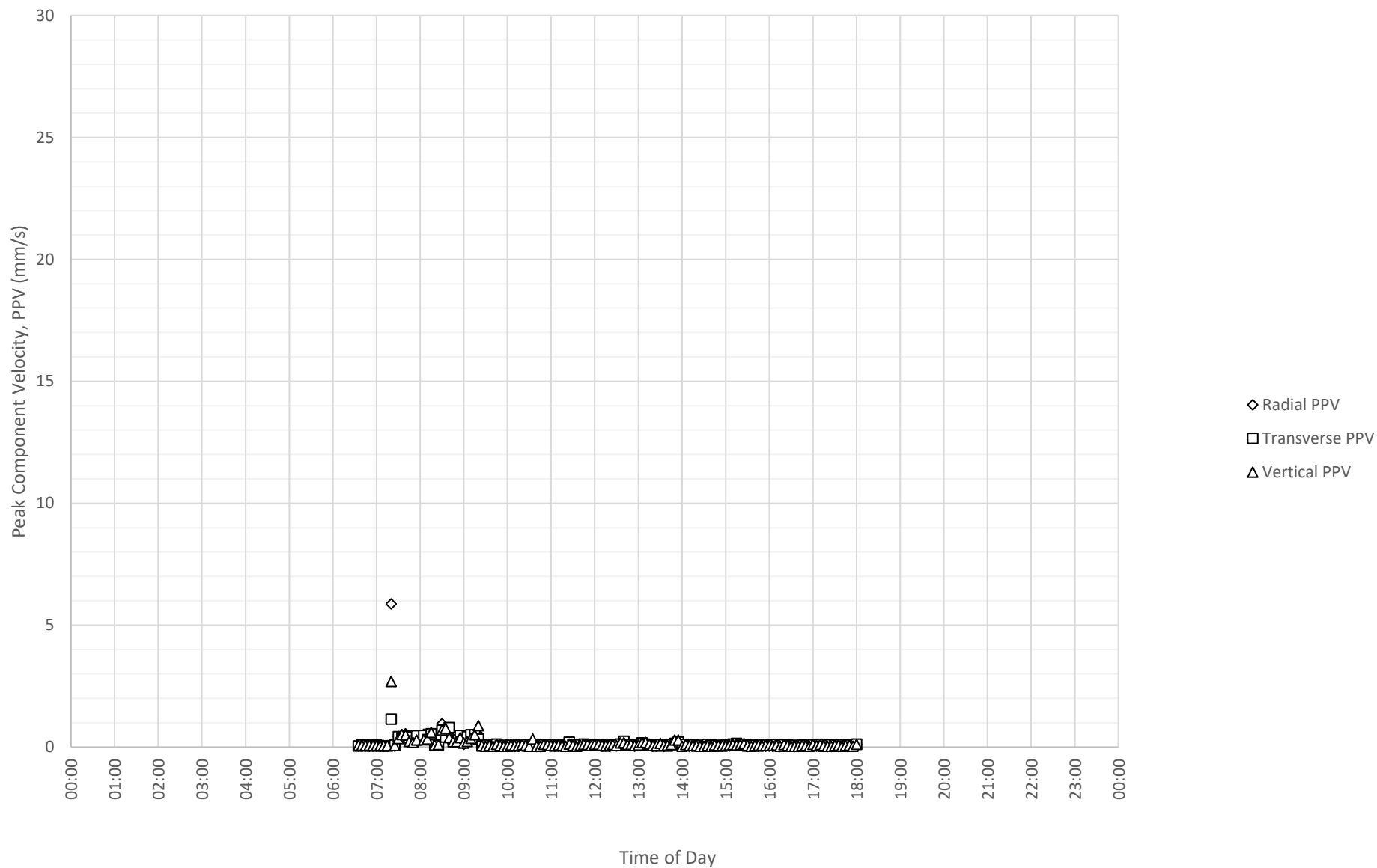
Daily Monitored Vibration Levels at East Boundary Opposite Shoalhaven Street (ETM7326) on 30-08-2024
