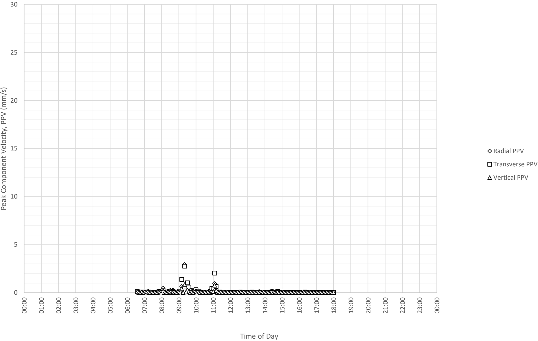
Daily Monitored Vibration Levels at North Boundary Near Block A and B (ETM7687) on 21-08-2024
