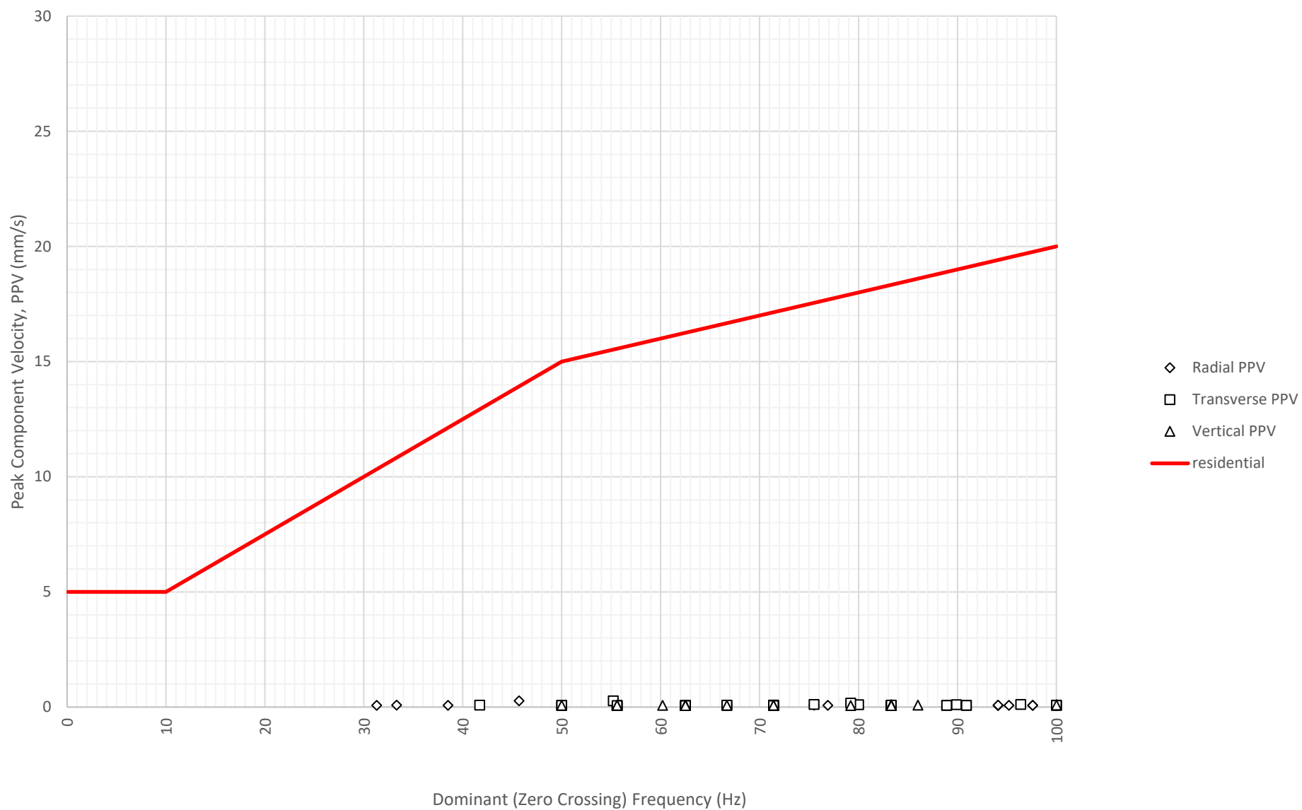
Frequency Content of Vibration Levels at North Boundary Near Block A and B (ETM7687) on 23-08-2024
