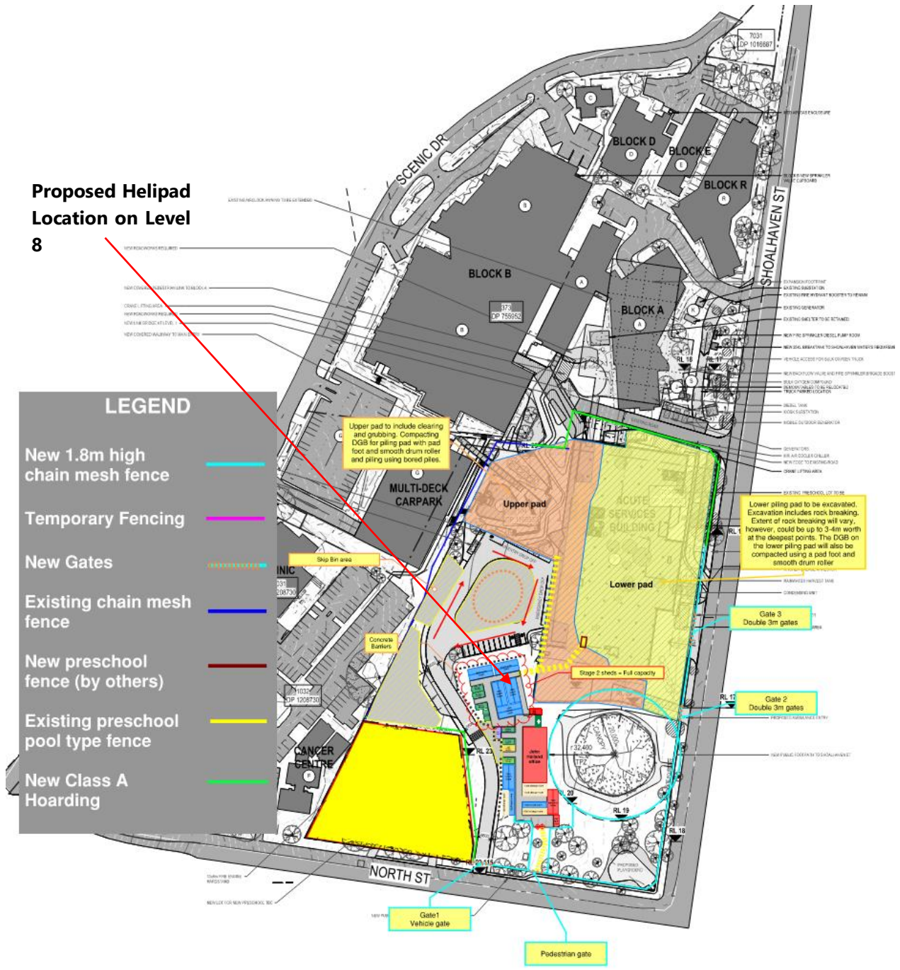
Figure 2 –Site Plan of Proposed Development (Refer also – Appendix B)
