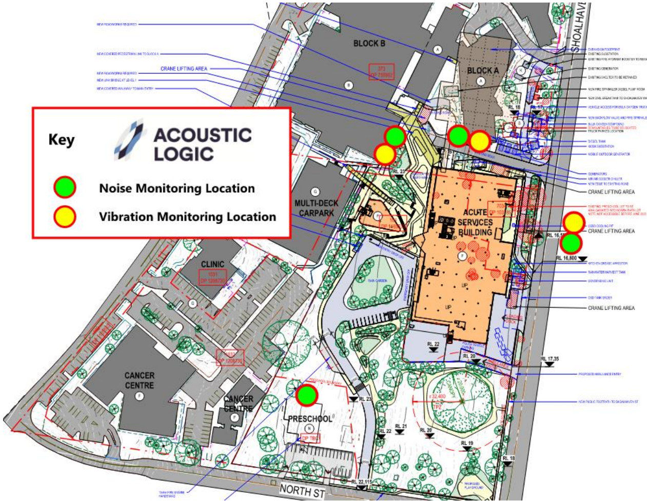
Figure 5 – Recommended Noise and Vibration Monitoring Locations (Preliminary)
