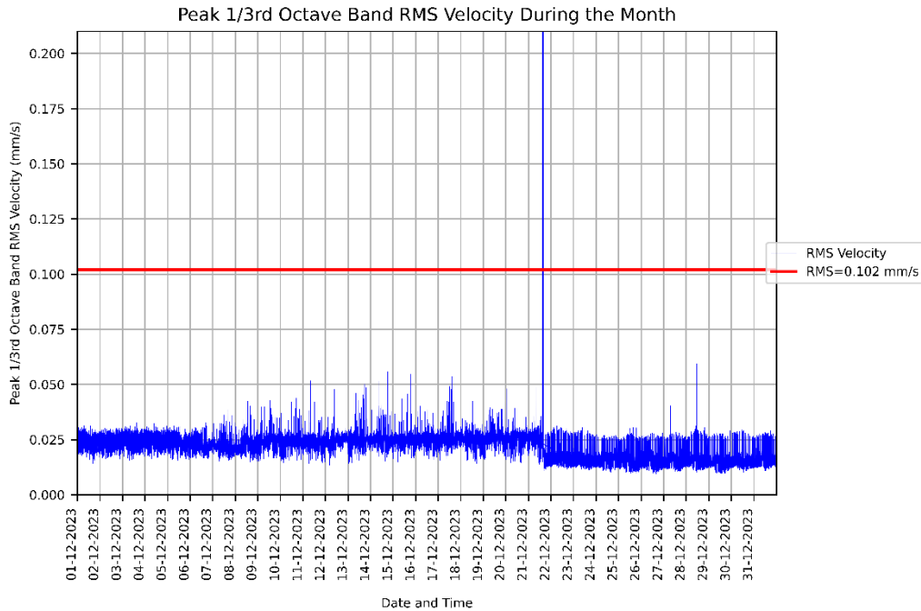
Figure 4: Measured RMSV vibration levels for 01/12/2023 to 31/12/2023 at the KR - Gait Lab.
