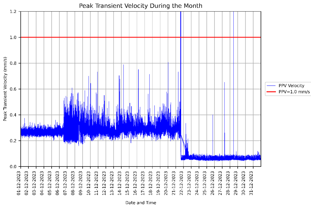
Figure 5: Measured PPV vibration levels for 01/12/2023 to 31/12/2023 at the KR - Gait Lab.
