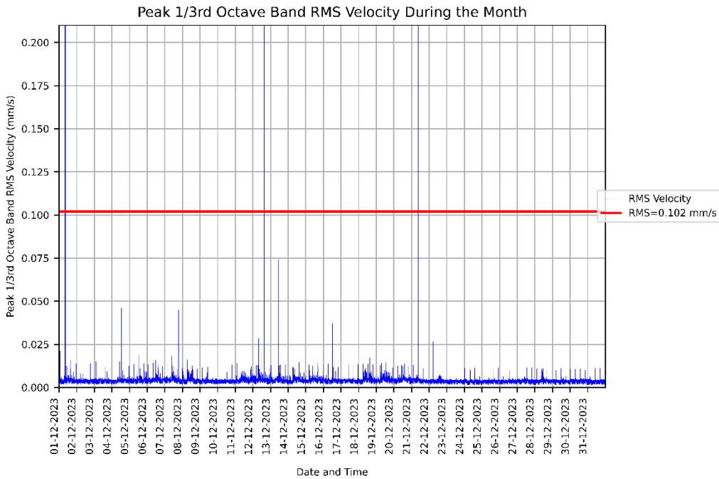
Figure 4: Measured RMSV vibration levels for 01/12/2023 to 31/12/2023 at the SCHN L1 Endocrinology Lab.
