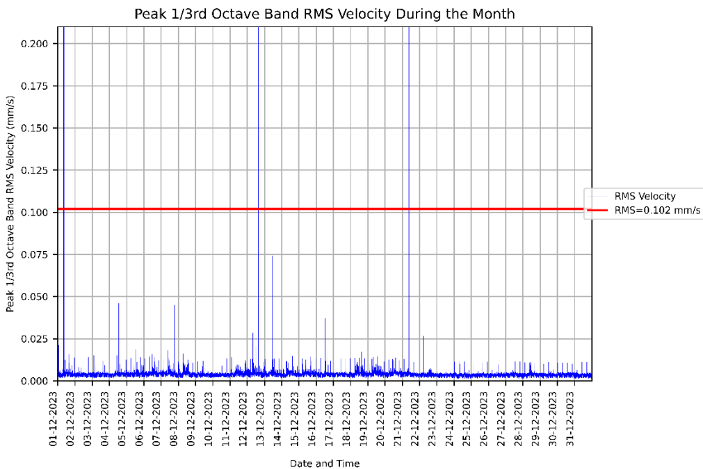
Figure 1: Measured RMSV vibration levels for 01/12/2023 to 31/12/2023 at the SCHN L1 Endocrinology Lab.
