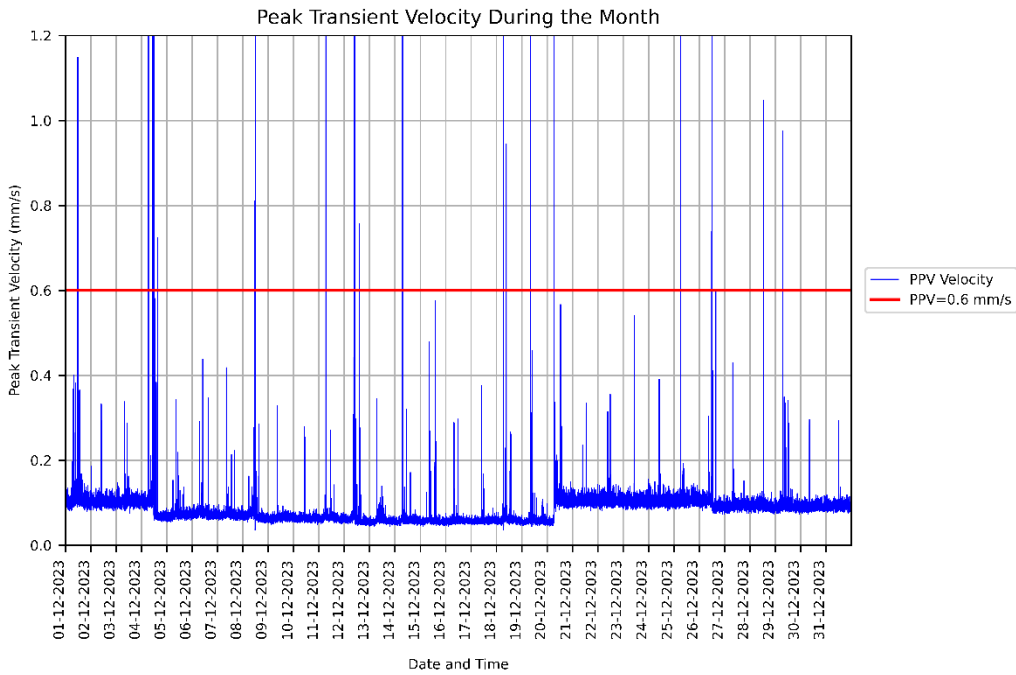
Figure 2: Measured vibration levels for 01/12/2023 to 31/12/2023 at the WIMR - BSF Mice Holding Room - Rack.
