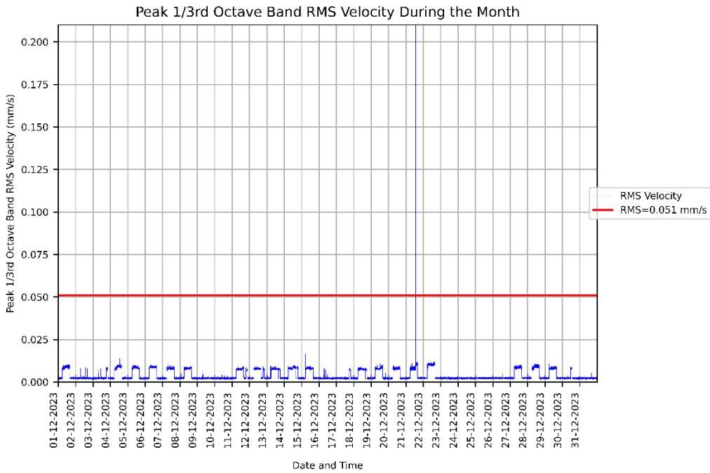
Figure 4: Measured RMSV vibration levels for 01/12/2023 to 31/12/2023 at the CMRI Animal Holding Facility.
