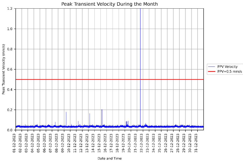
Figure 2: Measured vibration levels for 01/12/2023 to 31/12/2023 at the CMRI Animal Holding Facility.
