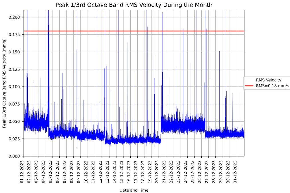
Figure 1: Measured RMSV vibration levels for 01/12/2023 to 31/12/2023 at the WIMR - BSF Mice Holding Room - Rack.
