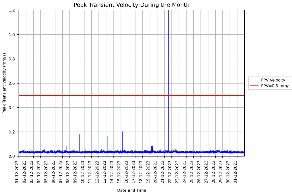
Figure 5: Measured PPV vibration levels for 01/12/2023 to 31/12/2023 at the CMRI Animal Holding Facility.
