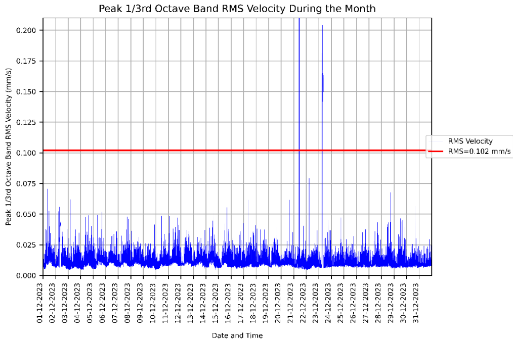
Figure 4: Measured RMSV vibration levels for 01/12/2023 to 31/12/2023 at the CASB level 3 Surgical Suite.
