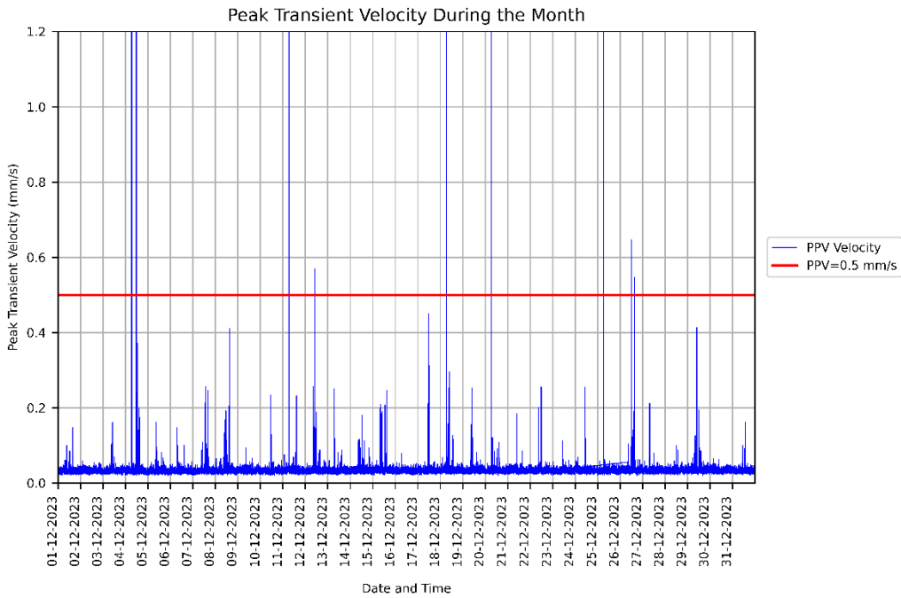
Figure 2: Measured vibration levels for 01/12/2023 to 31/12/2023 at the WIMR - BSF Mice Holding Room - Floor.
