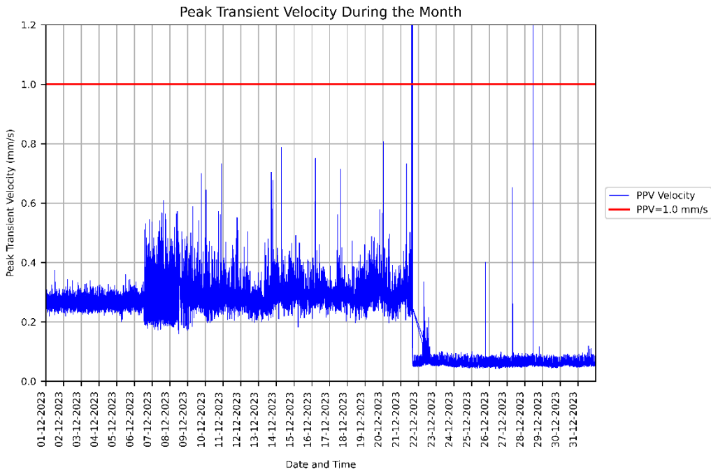
Figure 2: Measured vibration levels for 01/12/2023 to 31/12/2023 at the KR - Gait Lab.
