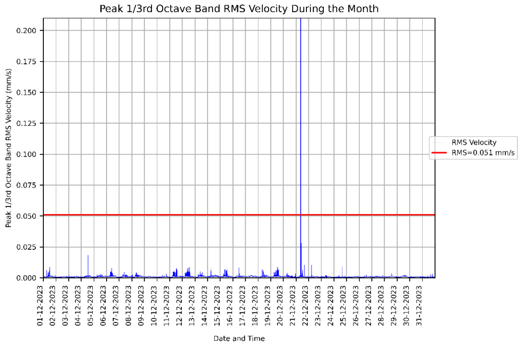
Figure 4: Measured RMSV vibration levels for 01/12/2023 to 31/12/2023 at the SCHN - 1.5t MRI.
