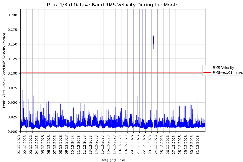
Figure 1: Measured RMSV vibration levels for 01/12/2023 to 31/12/2023 at the CASB level 3 Surgical Suite.
