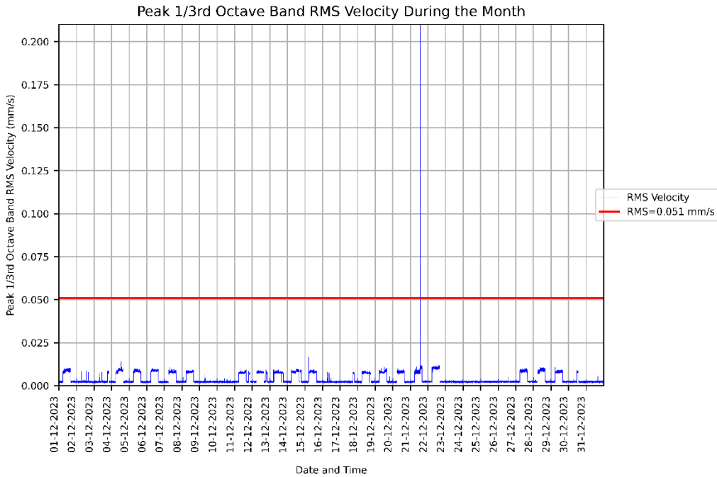
Figure 1: Measured RMSV vibration levels for 01/12/2023 to 31/12/2023 at the CMRI Animal Holding Facility.
