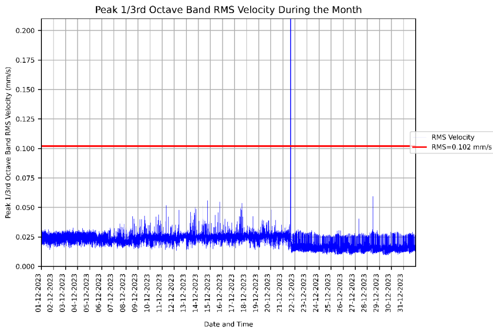
Figure 1: Measured RMSV vibration levels for 01/12/2023 to 31/12/2023 at the KR - Gait Lab.
