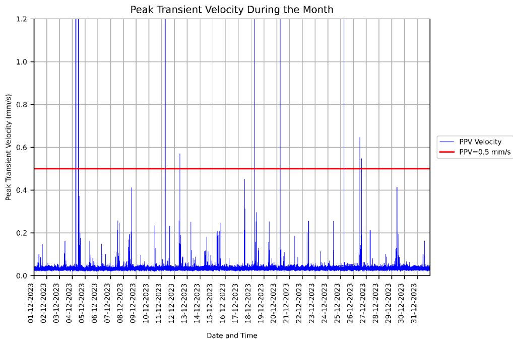
Figure 5: Measured PPV vibration levels for 01/12/2023 to 31/12/2023 at the WIMR - BSF Mice Holding Room - Floor.
