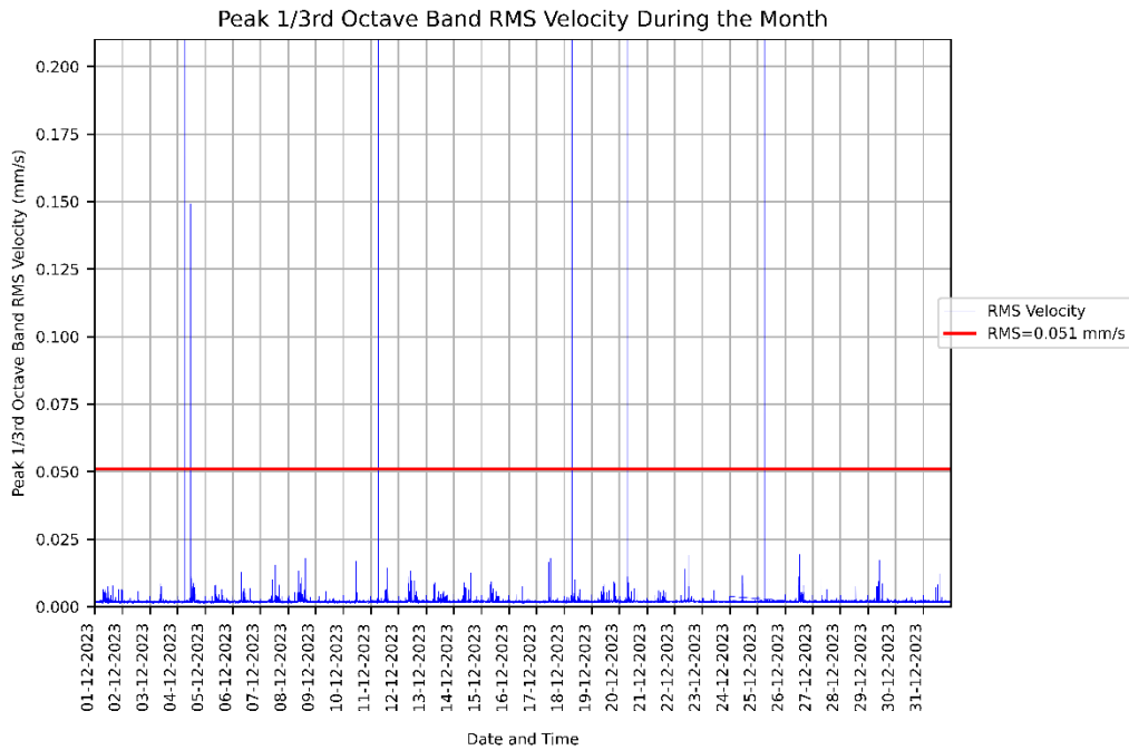
Figure 1: Measured RMSV vibration levels for 01/12/2023 to 31/12/2023 at the WIMR - BSF Mice Holding Room - Floor.
