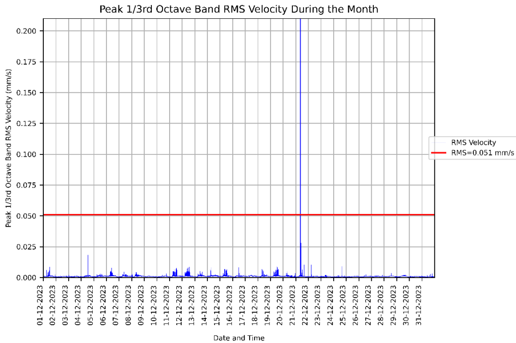
Figure 1: Measured RMSV vibration levels for 01/12/2023 to 31/12/2023 at the SCHN - 1.5t MRI.
