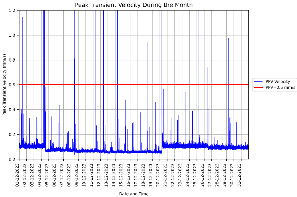
Figure 5: Measured PPV vibration levels for 01/12/2023 to 31/12/2023 at the WIMR - BSF Mice Holding Room - Rack.
