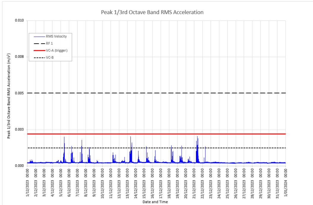
Figure 3: Measured RMS acceleration vibration levels for 01/12/2023 to 31/12/2023 at KR – L4.
