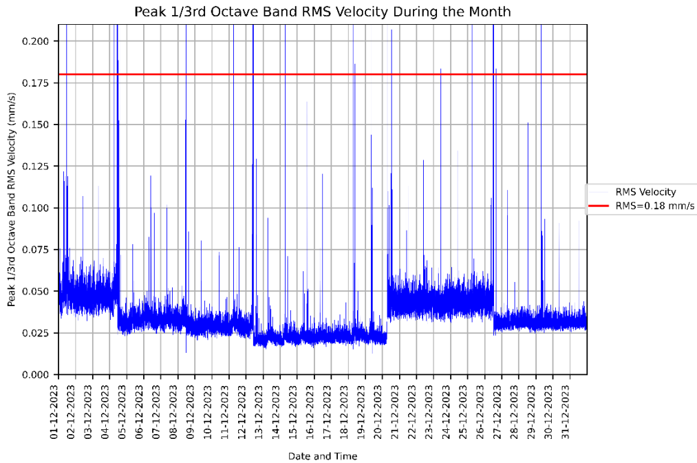
Figure 4: Measured RMSV vibration levels for 01/12/2023 to 31/12/2023 at the WIMR - BSF Mice Holding Room - Rack.
