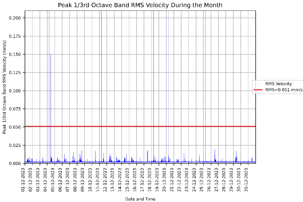
Figure 4: Measured RMSV vibration levels for 01/12/2023 to 31/12/2023 at the WIMR - BSF Mice Holding Room - Floor.
